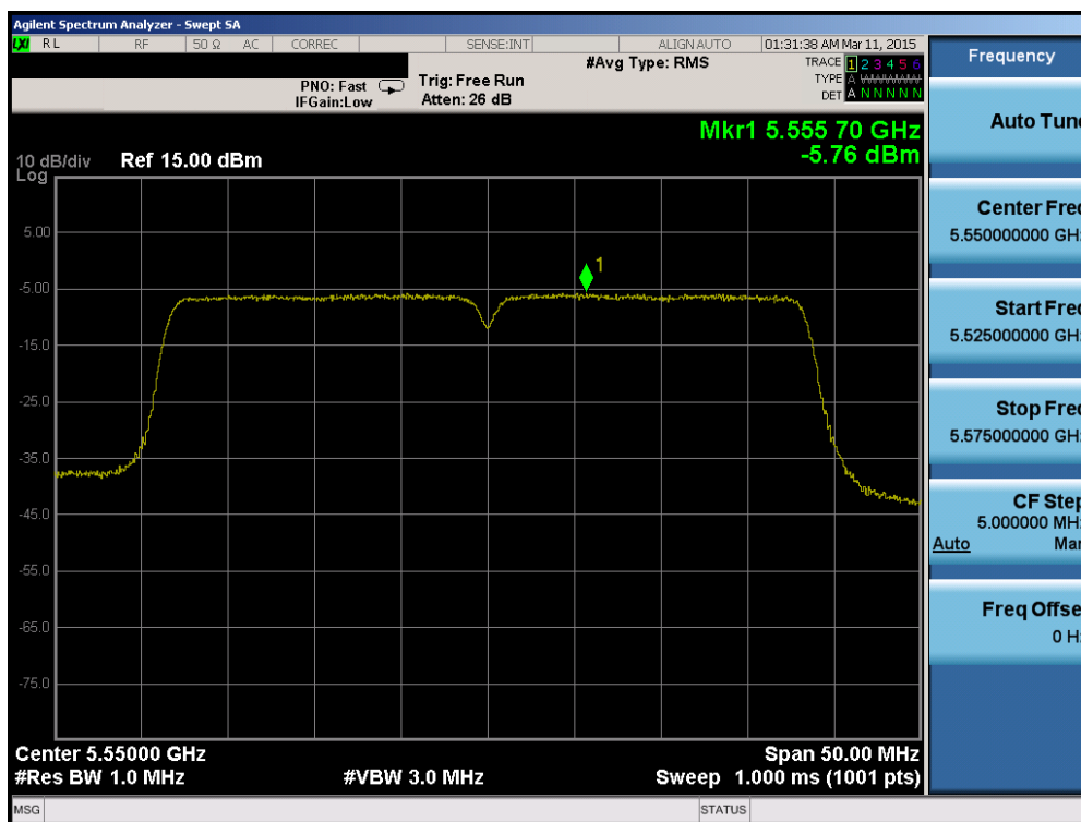
Plot 6-140. Power Spectral Density Plot (40MHz BW 802.11n (UNII Band 2C) – Ch. 110)
