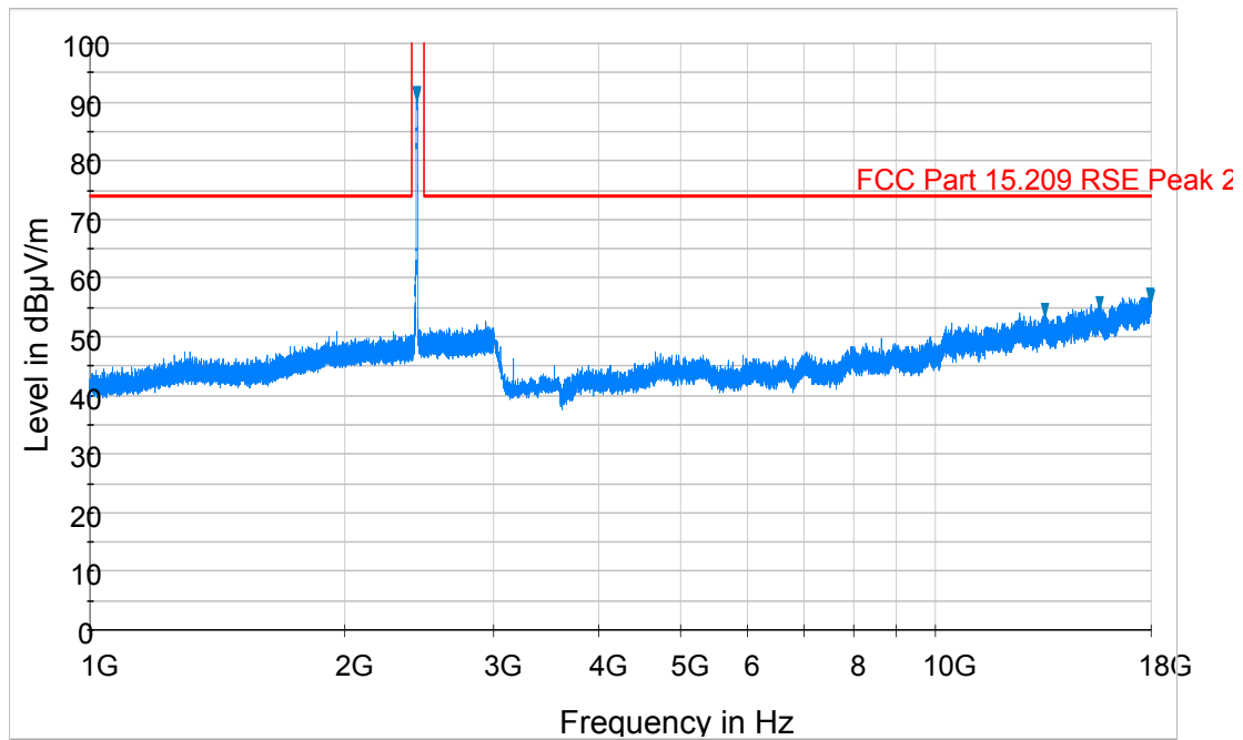
Plot 6-72. Radiated Spurious Plot above 1GHz (802.11b – Ch. 11, Ant. Pol. V)
