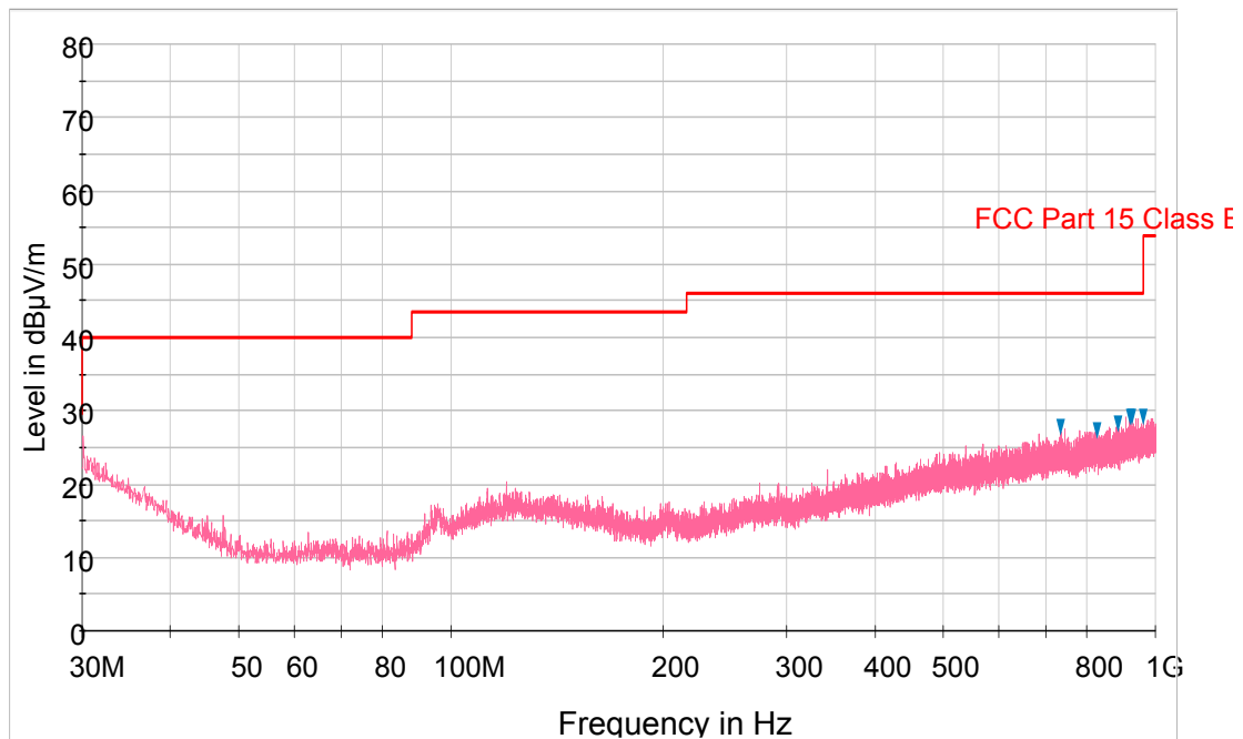
Plot 6-90. Radiated Spurious Plot below 1GHz (Pol. V)
