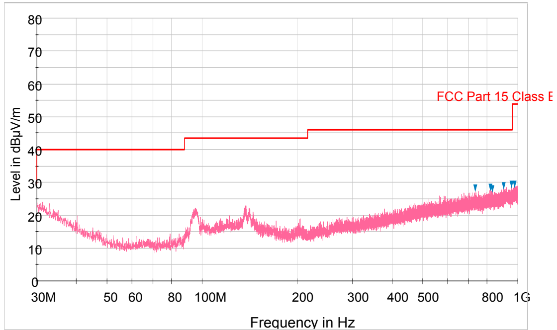
Plot 6-91. Radiated Spurious Plot below 1GHz (Pol. H)
