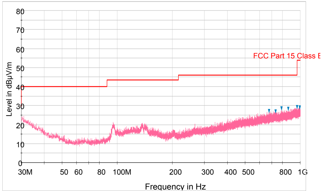
Plot 6-89. Radiated Spurious Plot below 1GHz (Pol. H)
