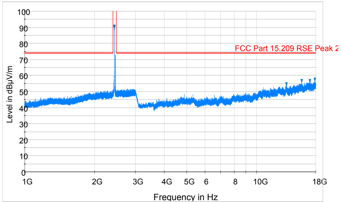
Plot 6-69. Radiated Spurious Plot above 1GHz (802.11b – Ch. 6, Ant. Pol. H)
