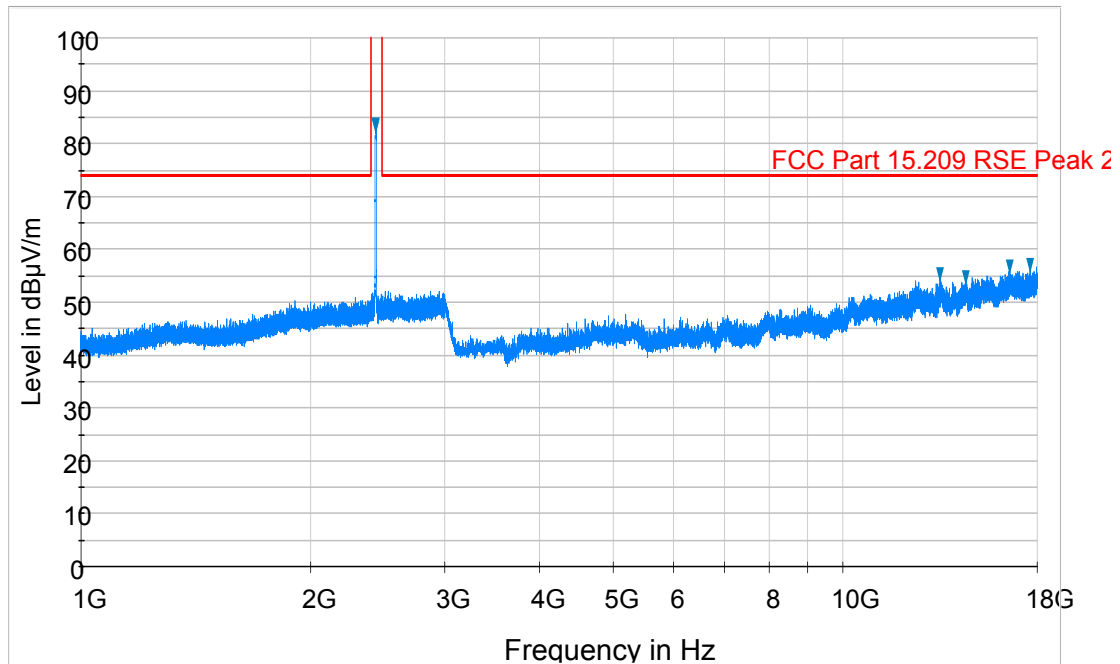
Plot 6-70. Radiated Spurious Plot above 1GHz (802.11b – Ch. 6, Ant. Pol. V)
