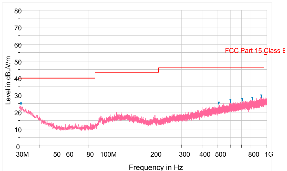
Plot 6-92. Radiated Spurious Plot below 1GHz (Pol. V)
