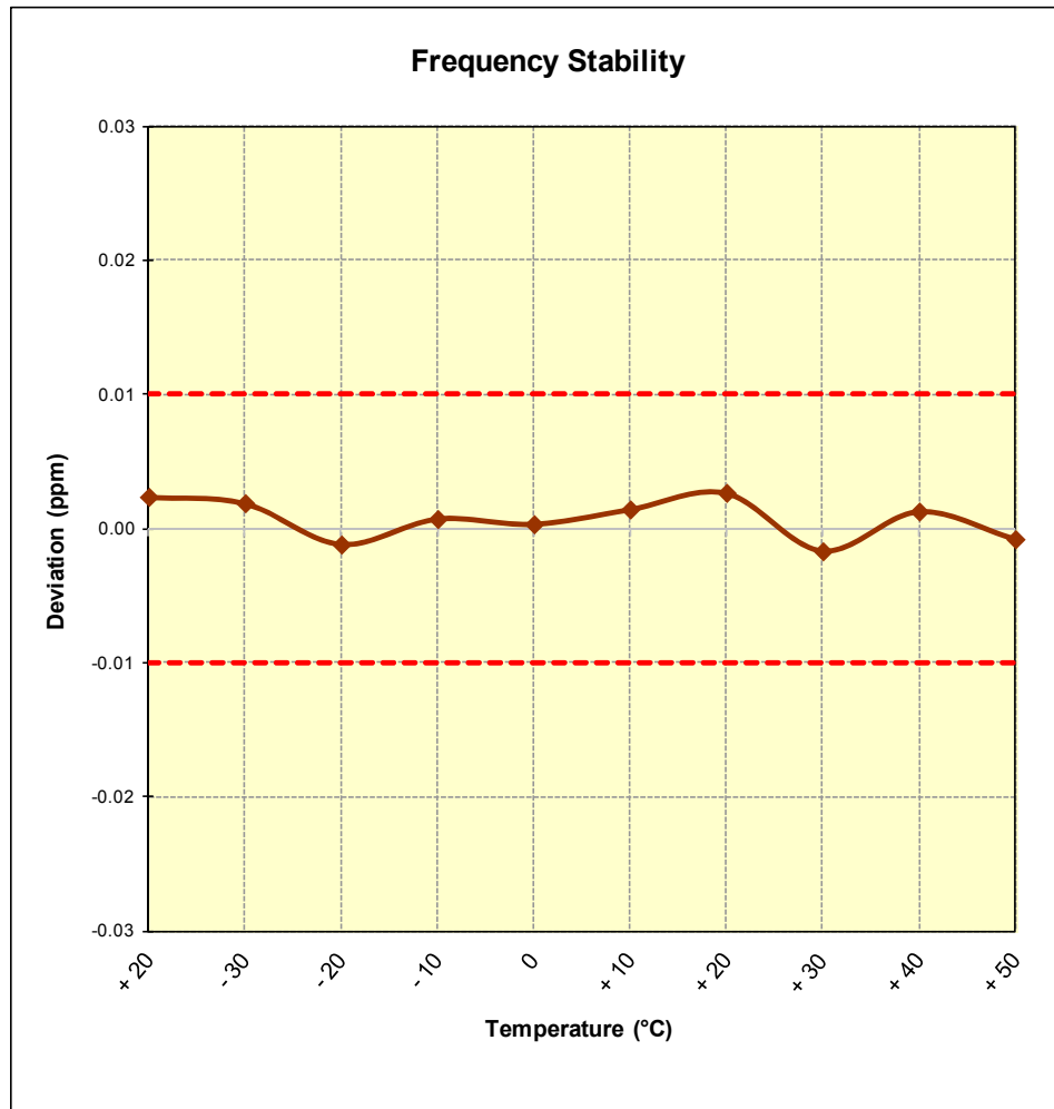
Figure 8-3. Frequency Stability Plot
