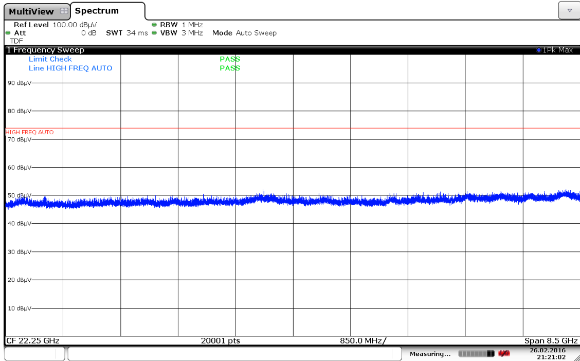
Plot 7-183. Radiated Spurious Plot 18GHz – 26GHz (2.4 GHz – 5 GHz, Ant. Pol. V)
