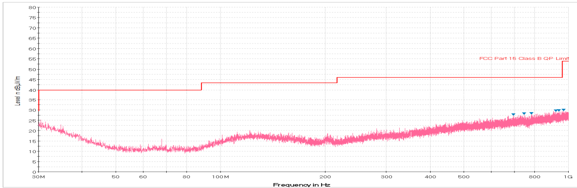
Plot 7-272. Radiated Spurious Plot below 1GHz (802.11a – U3 Ch. 157, Ant. Pol. H)
