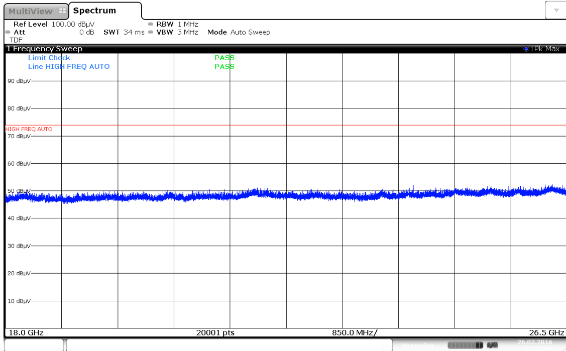
Plot 7-181. Radiated Spurious Plot 18GHz – 26GHz (2.4 GHz – 5 GHz, Ant. Pol. H)
