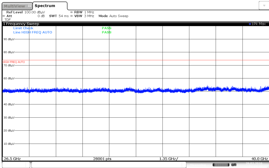
Plot 7-184. Radiated Spurious Plot above 26GHz (2.4 GHz – 5 GHz, Ant. Pol. V)
