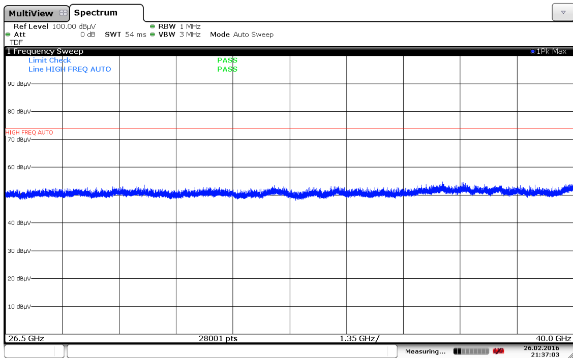
Plot 7-182. Radiated Spurious Plot above 26GHz (2.4 GHz – 5 GHz, Ant. Pol. H)
