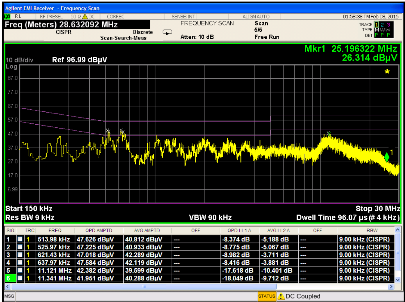
Plot 7-99. Line Conducted Plot with 802.11b (L1)
