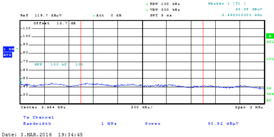
Plot A4-3. Radiated Restricted Upper Band Edge Measurement (Average)
