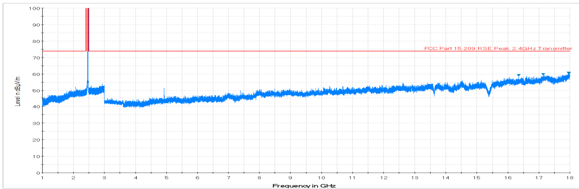
Plot 7-66. Radiated Spurious Plot above 1GHz (802.11b – Ch. 11, Ant. Pol. V)
