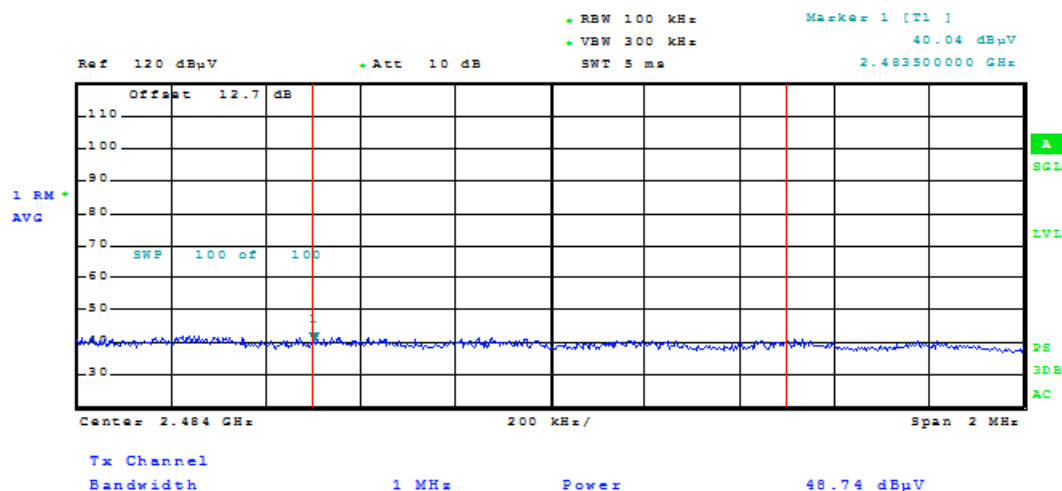
Plot 7-85. Radiated Restricted Upper Band Edge Measurement (Average)
