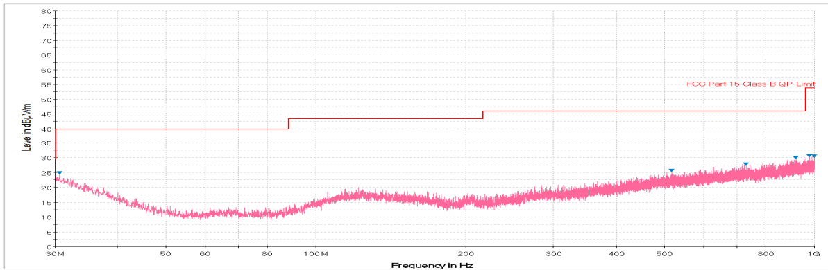
Plot 7-97. Radiated Spurious Plot below 1GHz (Pol. H)
