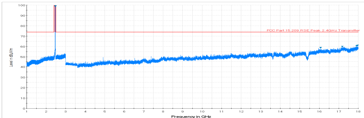
Plot 7-74. Radiated Spurious Plot above 1GHz (802.11b – Ch. 11, Ant. Pol. V)
