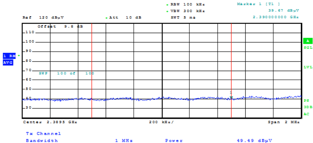
Plot 7-93. Radiated Restricted Band Edge Measurement with WCP (Average)
