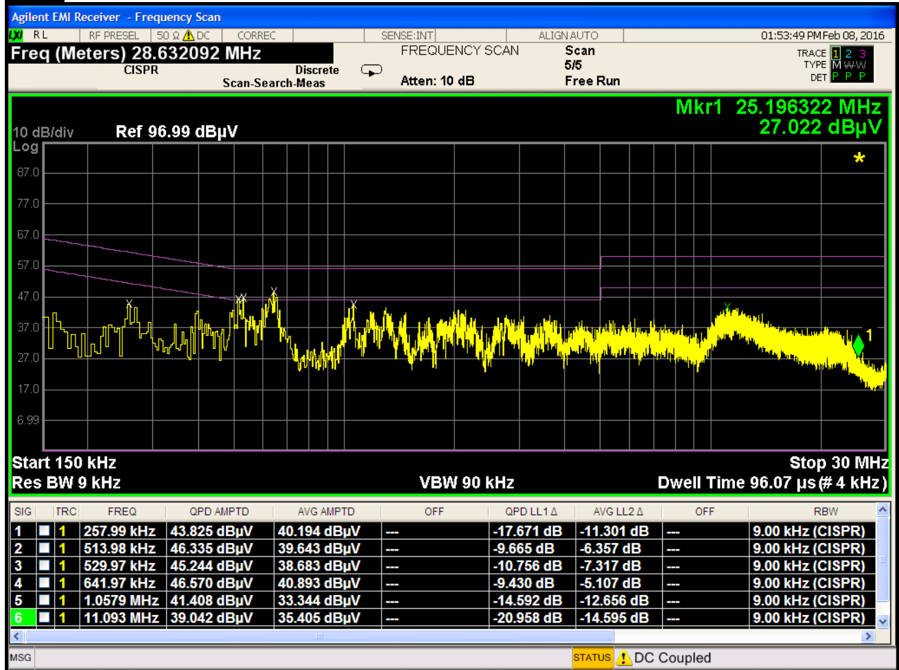
Plot 7-100. Line Conducted Plot with 802.11b (N)
