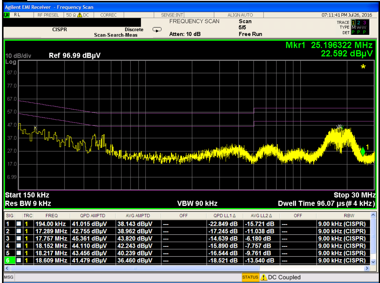
Plot 8-4. Line-Conducted Test Plot with 50Ohm Termination (N)
