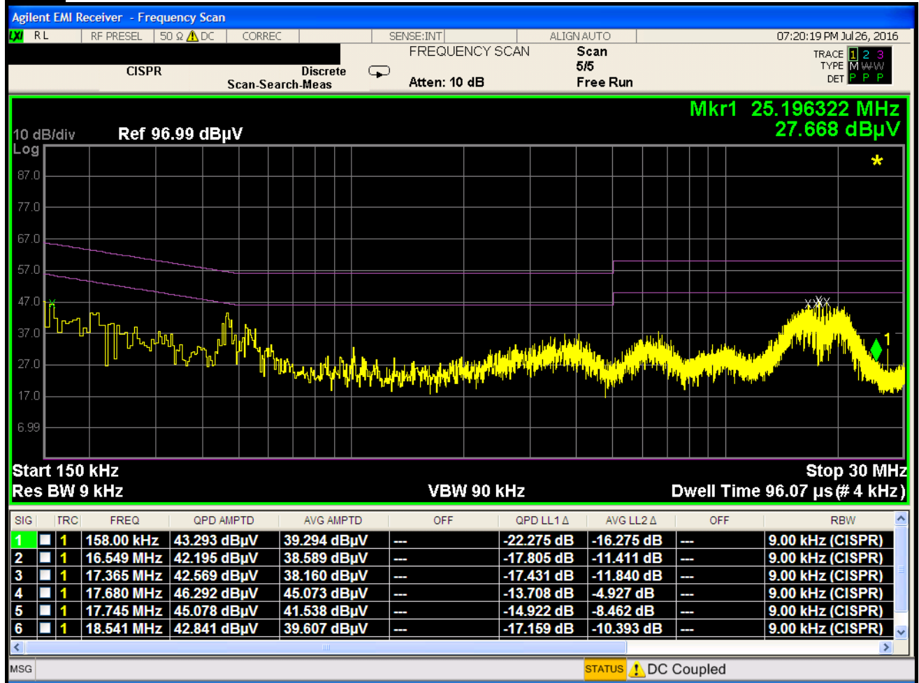
Plot 8-3. Line-Conducted Test Plot with 50Ohm Termination (L1)
