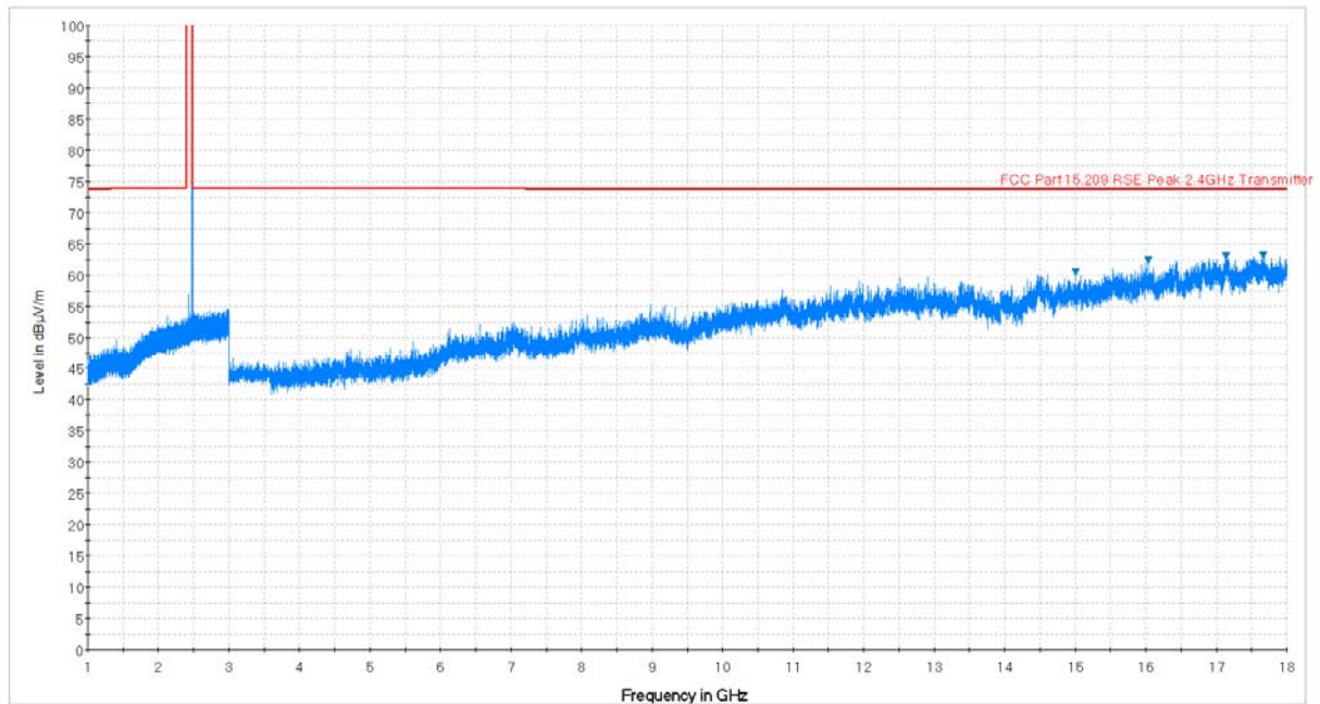
Plot 7-47. Radiated Spurious Plot above 1GHz (BT – Ch. 78, Ant. Pol. V)
