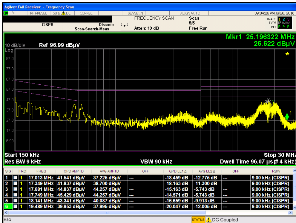
Plot 7-249. Line Conducted Plot with 802.11a UNII Band 3 (L1)
