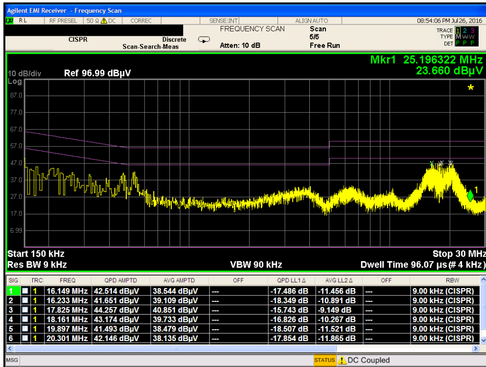
Plot 7-248. Line Conducted Plot with 802.11a UNII Band 2C (N)
