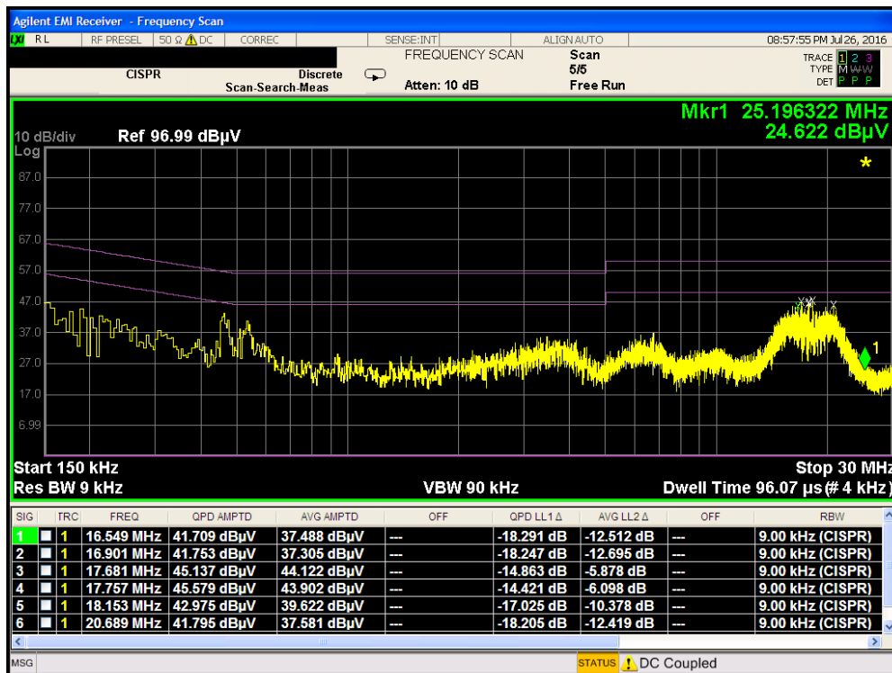
Plot 7-247. Line Conducted Plot with 802.11a UNII Band 2C (L1)
