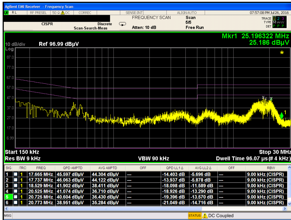
Plot 7-243. Line Conducted Plot with 802.11a UNII Band 1 (L1)
