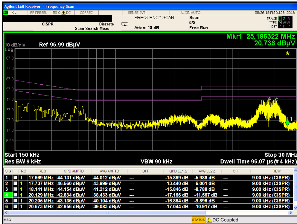
Plot 7-244. Line Conducted Plot with 802.11a UNII Band 1 (N)
