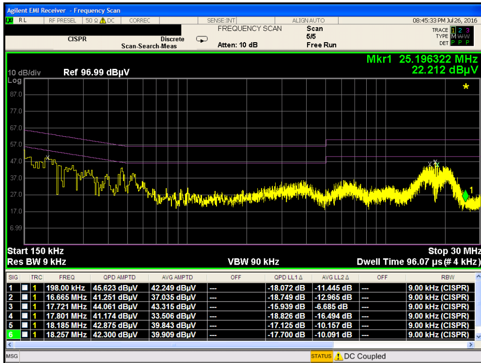
Plot 7-245. Line Conducted Plot with 802.11a UNII Band 2A (L1)
