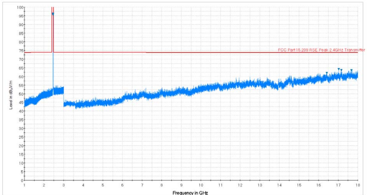
Plot 7-73. Radiated Spurious Plot above 1GHz (802.11b – Ch. 11, Ant. Pol. H)
