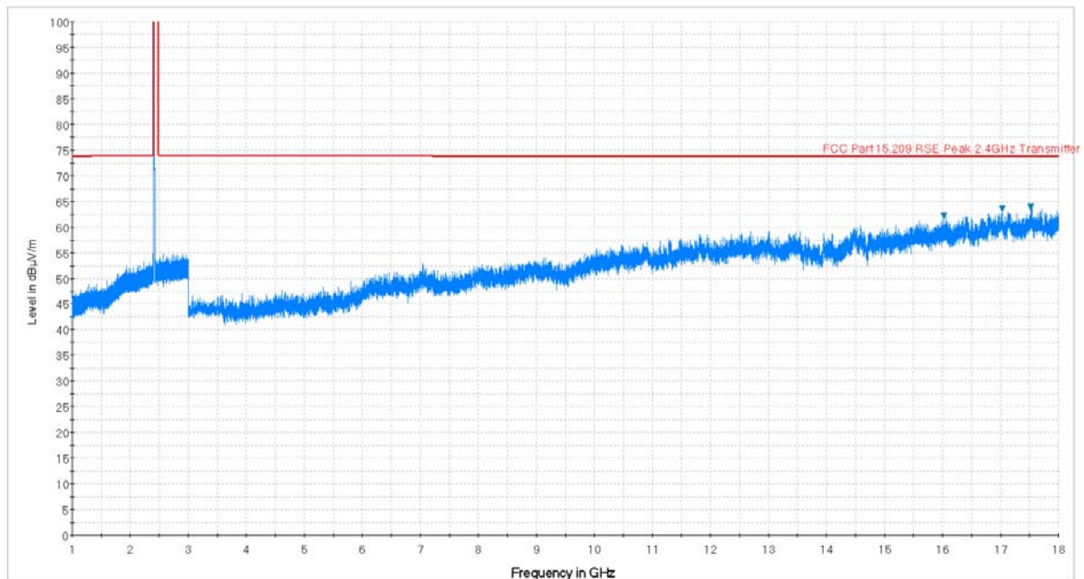
Plot 7-61. Radiated Spurious Plot above 1GHz (802.11b – Ch. 1, Ant. Pol. H)
