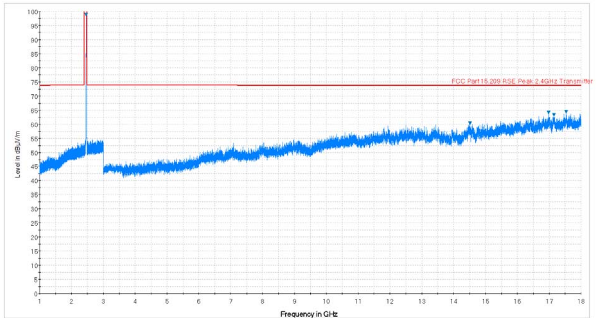
Plot 7-74. Radiated Spurious Plot above 1GHz (802.11b – Ch. 11, Ant. Pol. V)
