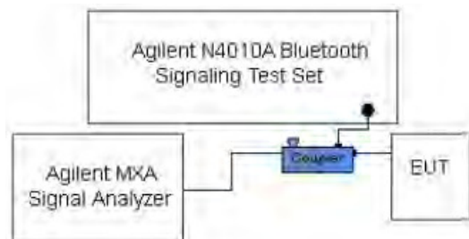
Figure 9-8 Power Measurement Setup
