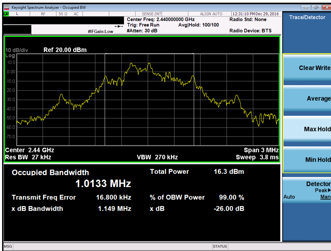
Plot 7-1. Occupied Bandwidth Plot (ANT+ – Ch. 39)
