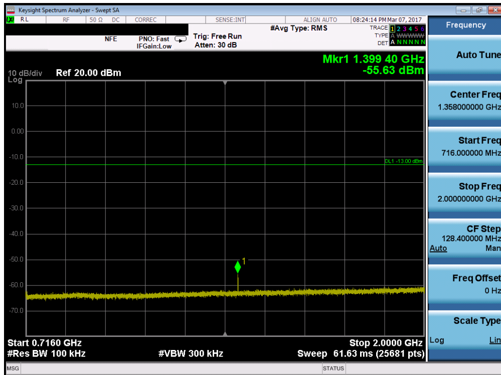
Plot 7-41. Conducted Spurious Plot (Band 17 – 10.0MHz QPSK – RB Size 1, RB Offset 0 – Low Channel)
