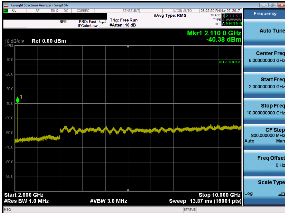
Plot 7-45. Conducted Spurious Plot (Band 17 – 10.0MHz QPSK – RB Size 1, RB Offset 0 – Mid Channel)
