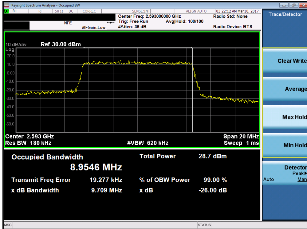
Plot 7-33. Occupied Bandwidth Plot (Band 41 – 10.0MHz 64-QAM – RB Size 50)
