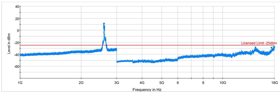
Plot 7-26. Radiated Spurious Plot (ULCA B41 PCC: RB 100 Offset 0, SCC: RB 100 Offset 0, Ant. Pol. V)
