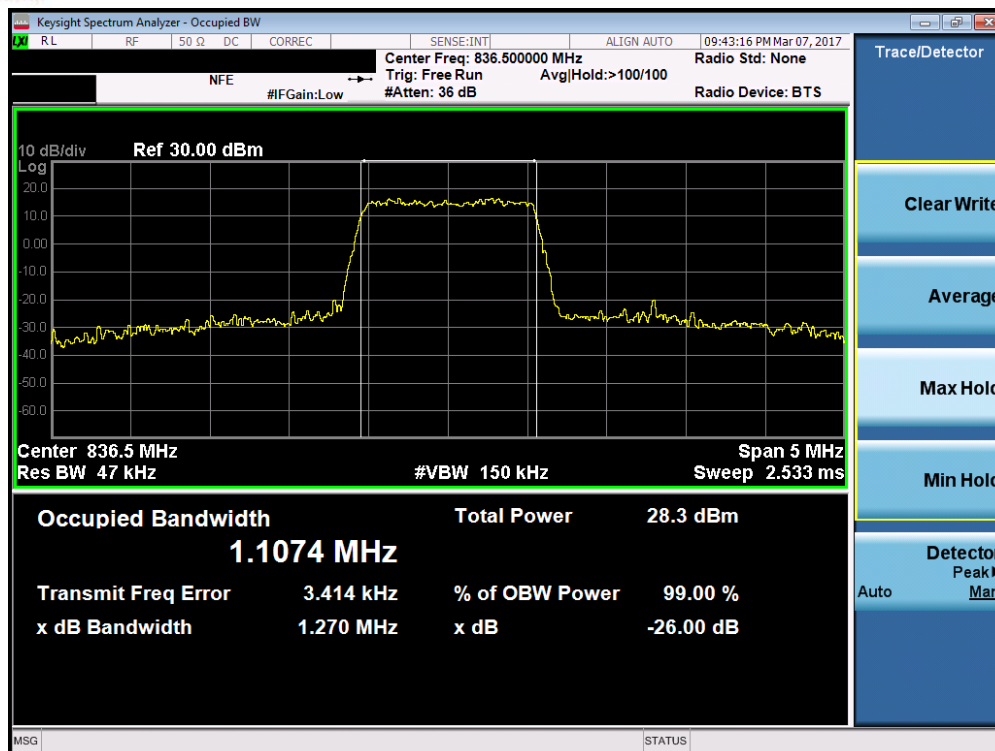
Plot 7-15. Occupied Bandwidth Plot (Band 5/26 – 1.4MHz 64-QAM – RB Size 6)
