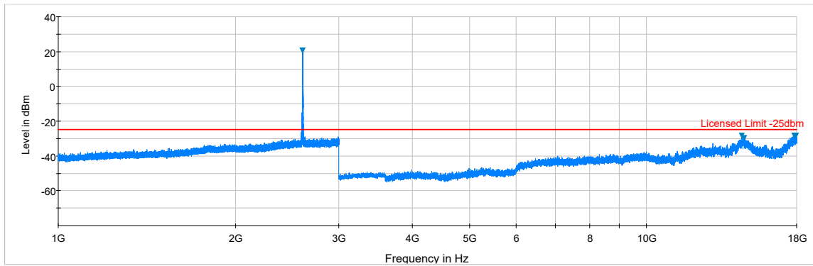
Plot 7-27. Radiated Spurious Plot (ULCA B41 PCC: RB 1 Offset 99, SCC: RB 1 Offset 0, Ant. Pol. H)
