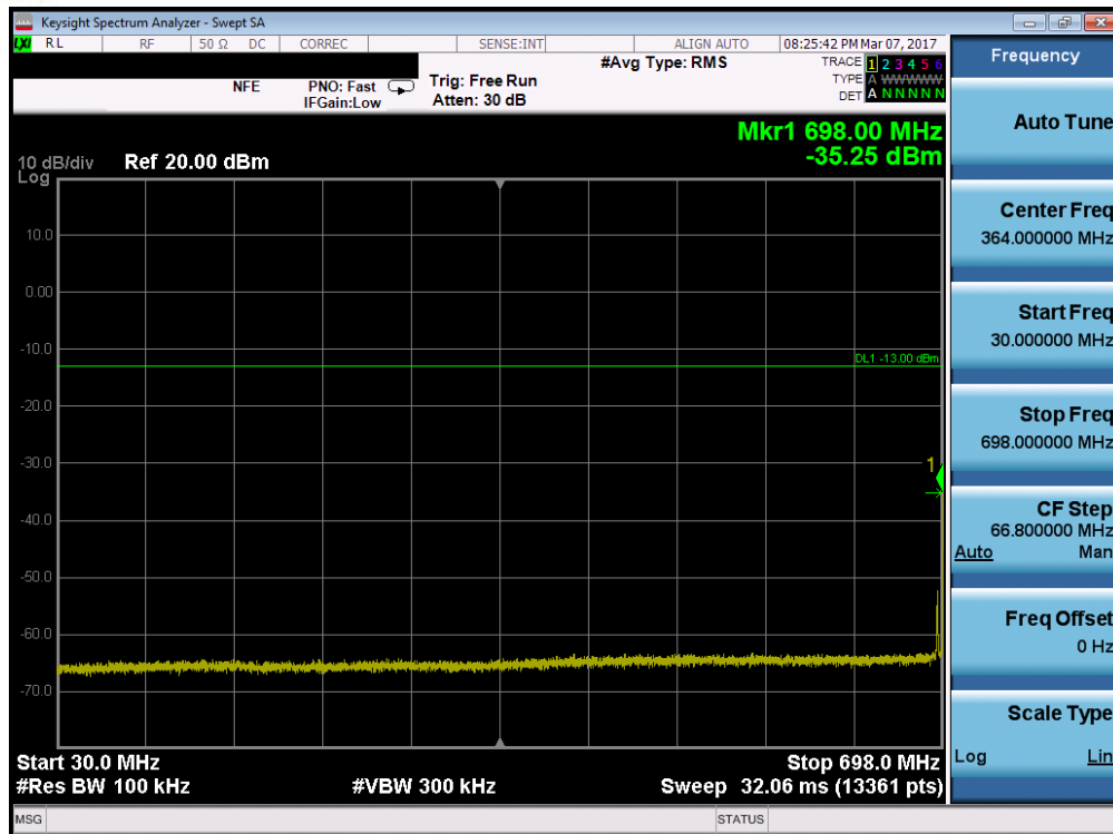
Plot 7-46. Conducted Spurious Plot (Band 17 – 10.0MHz QPSK – RB Size 1, RB Offset 0 – High Channel)
