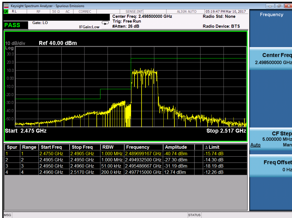
Plot 7-92. Lower ACP Plot (Band 41 – 5.0MHz QPSK – RB Size 25)
