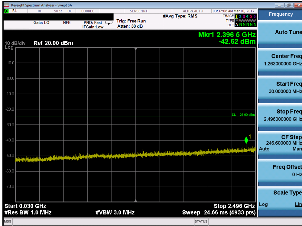
Plot 7-64. Conducted Spurious Plot (Band 41 – 20.0MHz QPSK – RB Size 1, RB Offset 0 – Mid Channel)
