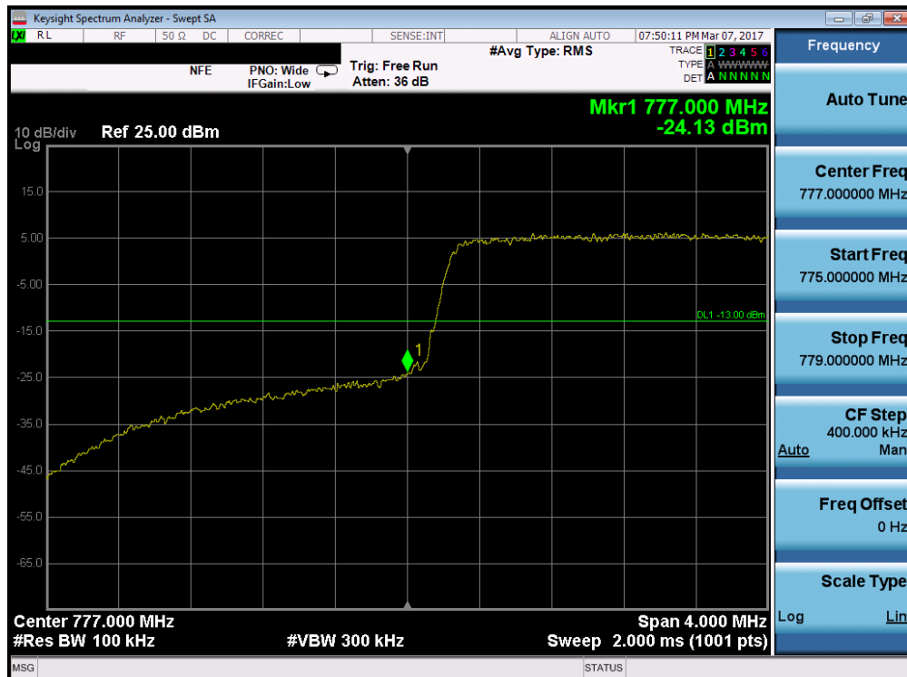
Plot 7-74. Lower Band Edge Plot (Band 13 – 5.0MHz QPSK – RB Size 25)
