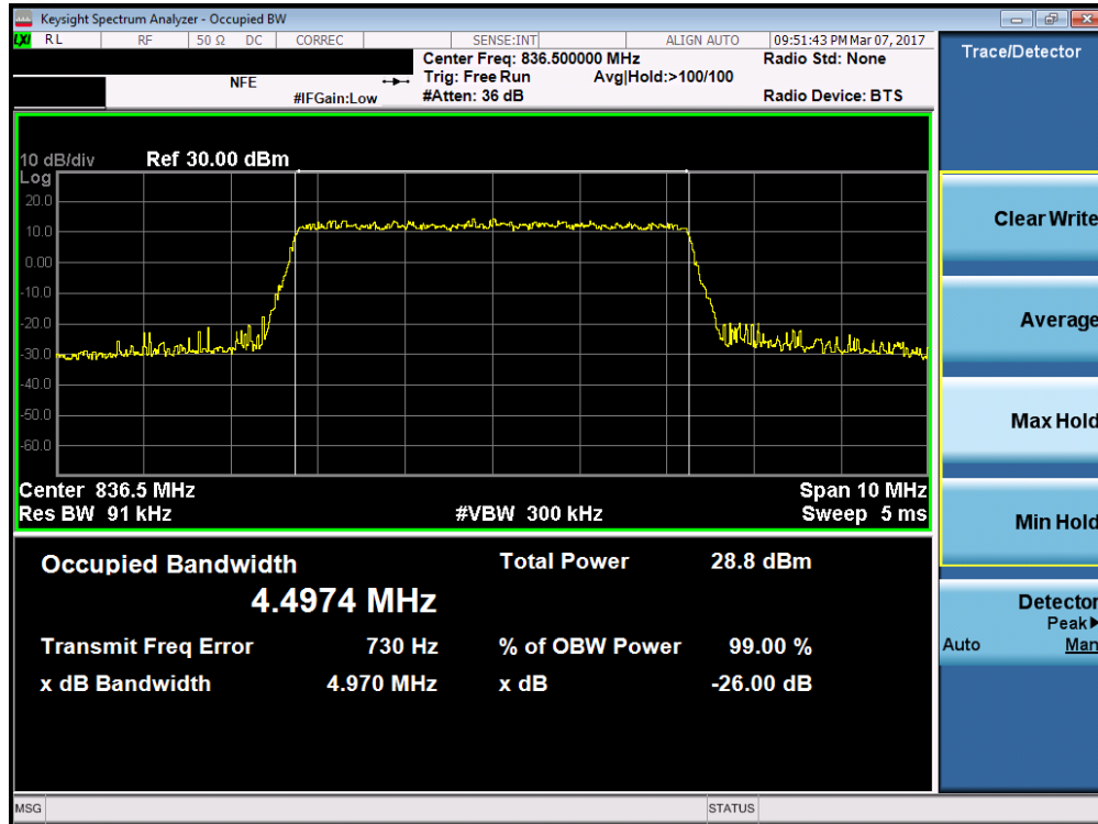
Plot 7-21. Occupied Bandwidth Plot (Band 5/26 - 5.0MHz 64-QAM - RB Size 25)
