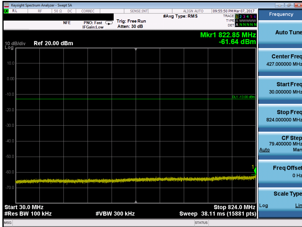
Plot 7-58. Conducted Spurious Plot (Band 5/26 – 10.0MHz QPSK – RB Size 1, RB Offset 0 – High Channel)
