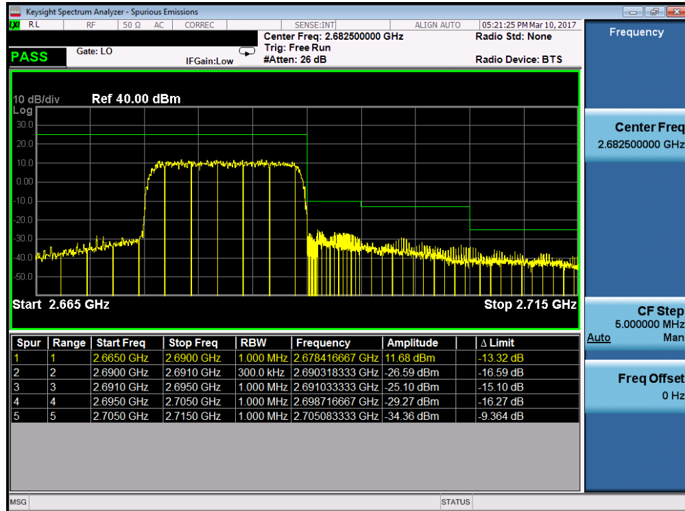
Plot 7-97. Upper ACP Plot (Band 41 – 15.0MHz QPSK – RB Size 75)
