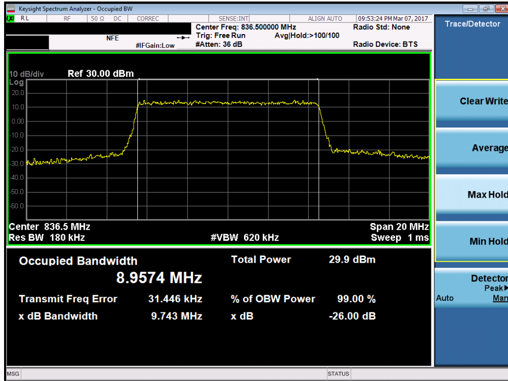
Plot 7-23. Occupied Bandwidth Plot (Band 5/26 – 10.0MHz 16-QAM – RB Size 50)
