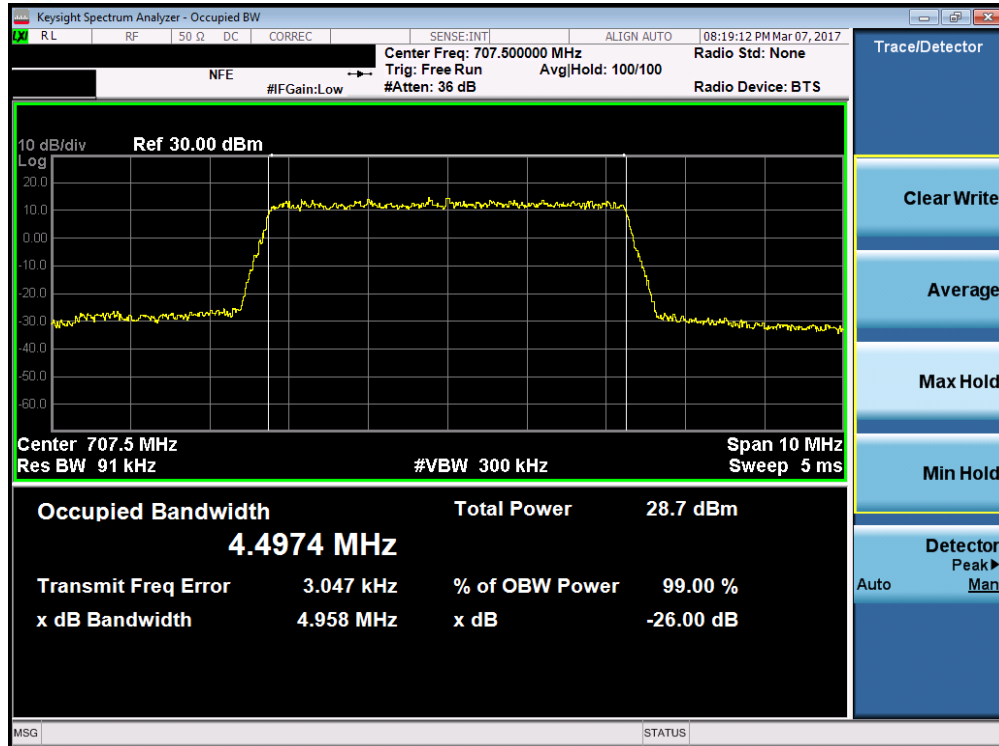
Plot 7-3. Occupied Bandwidth Plot (Band 17 – 5.0MHz 64-QAM – RB Size 25)
