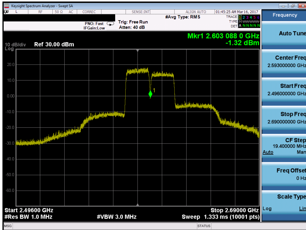
Plot 7-105. Conducted Spurious Plot (Band 41 – 20.0MHz QPSK – PCC 100/0, SCC 100/0 – Mid Channel)
