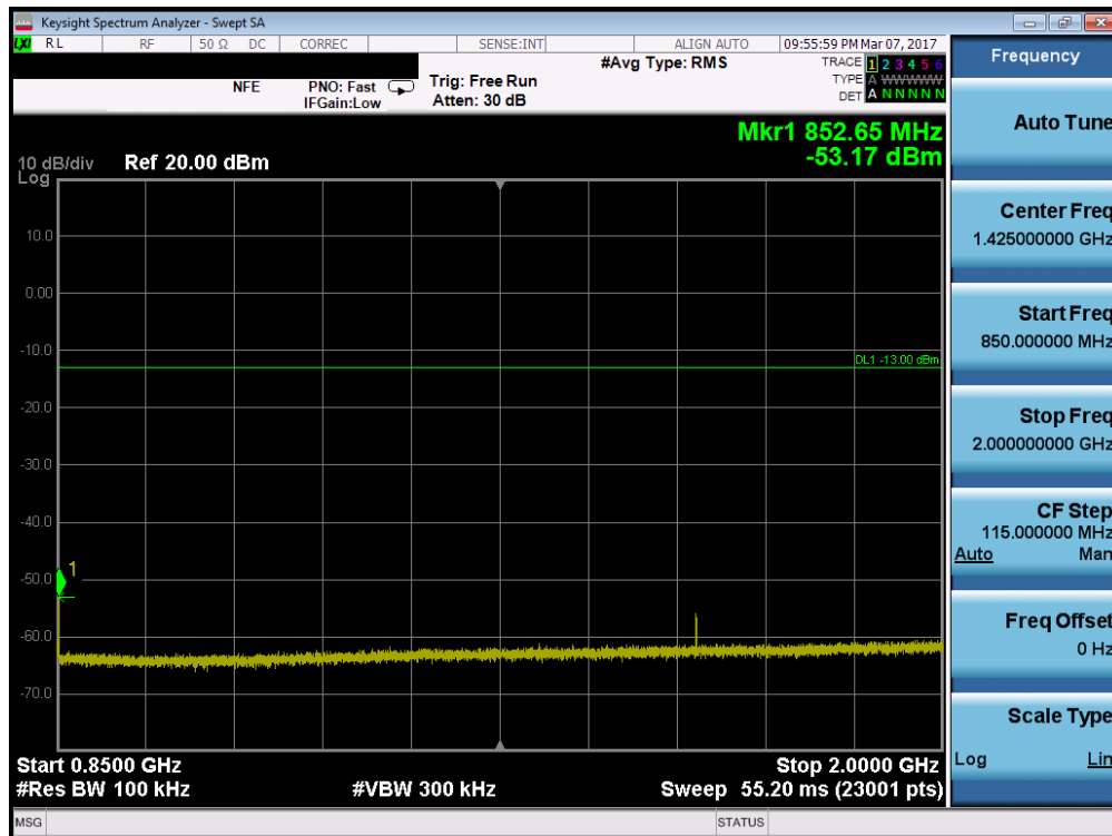
Plot 7-59. Conducted Spurious Plot (Band 5/26 – 10.0MHz QPSK – RB Size 1, RB Offset 0 – High Channel)
