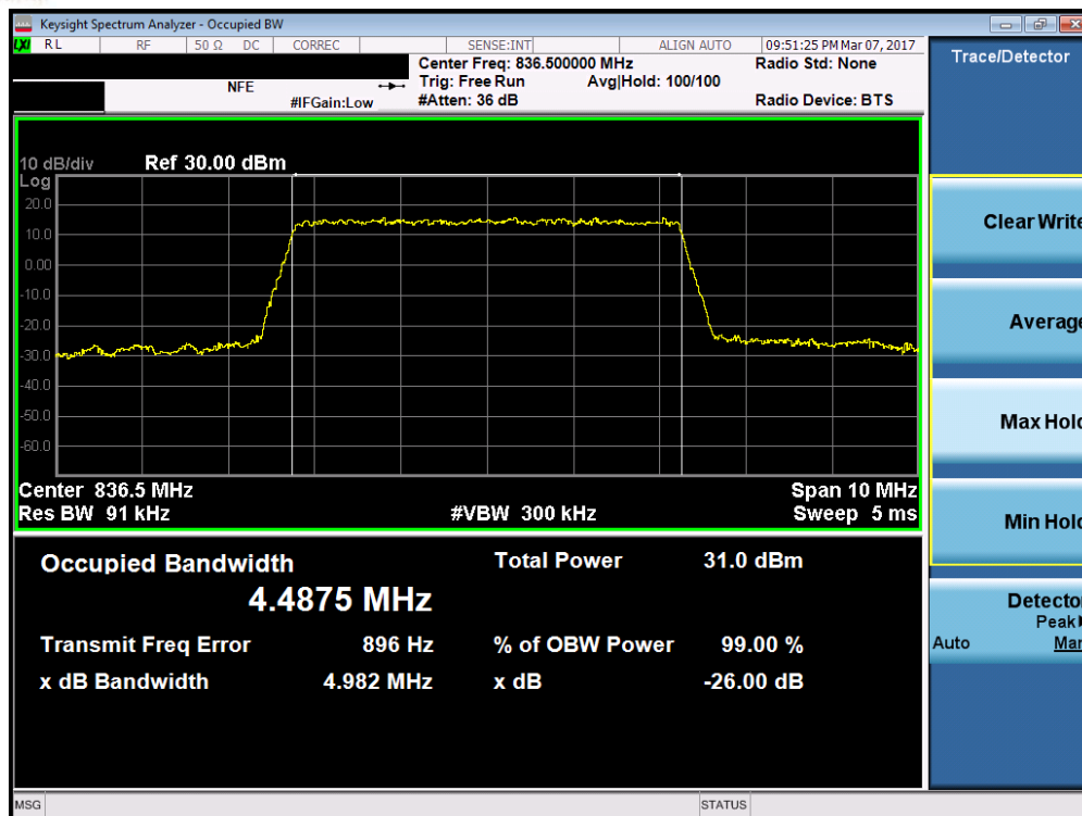
Plot 7-19. Occupied Bandwidth Plot (Band 5/26 - 5.0MHz QPSK - RB Size 25)
