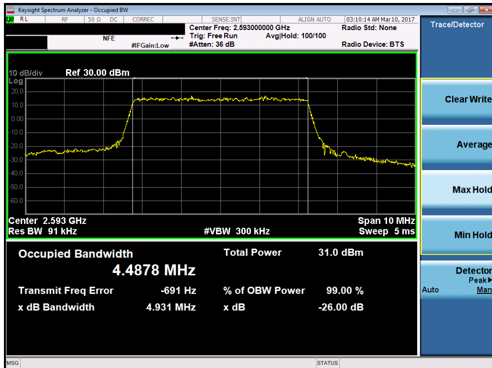
Plot 7-28. Occupied Bandwidth Plot (Band 41 – 5.0MHz QPSK – RB Size 25)
