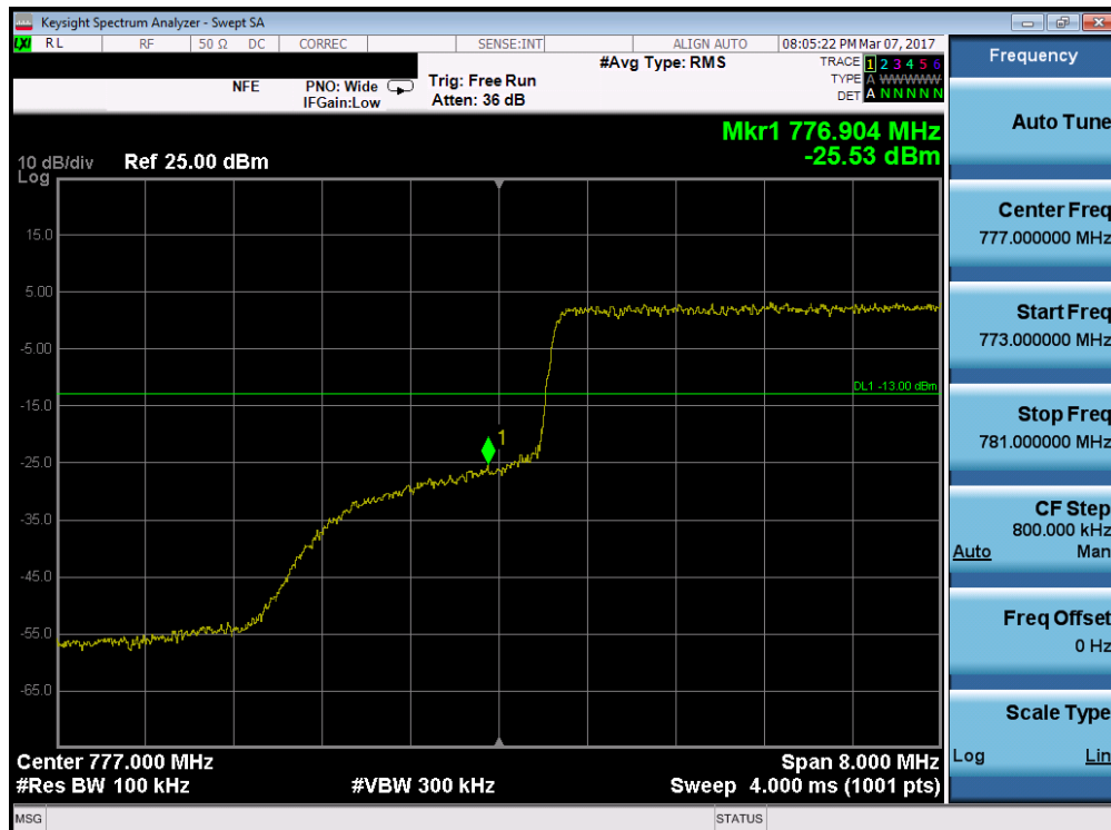
Plot 7-78. Lower Band Edge Plot (Band 13 – 10.0MHz QPSK – RB Size 50)
