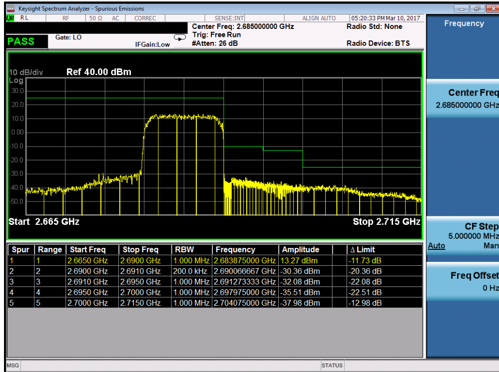
Plot 7-95. Upper ACP Plot (Band 41 – 10.0MHz QPSK – RB Size 50)
