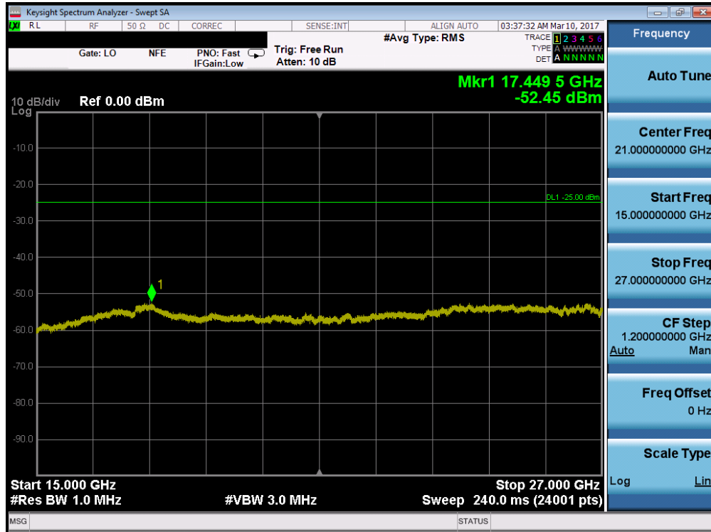
Plot 7-66. Conducted Spurious Plot (Band 41 – 20.0MHz QPSK – RB Size 1, RB Offset 0 – Mid Channel)
