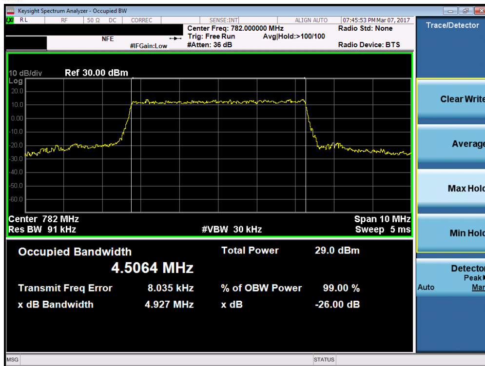
Plot 7-7. Occupied Bandwidth Plot (Band 13 – 5.0MHz QPSK – RB Size 25)
