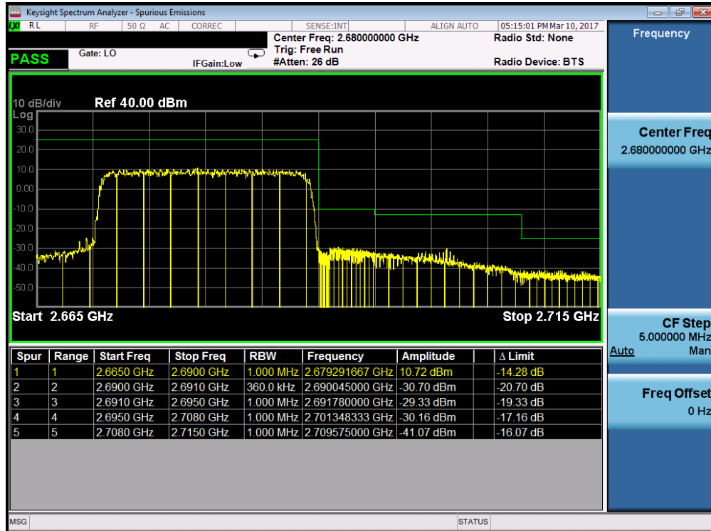
Plot 7-99. Upper ACP Plot (Band 41 – 20.0MHz QPSK – RB Size 100)
