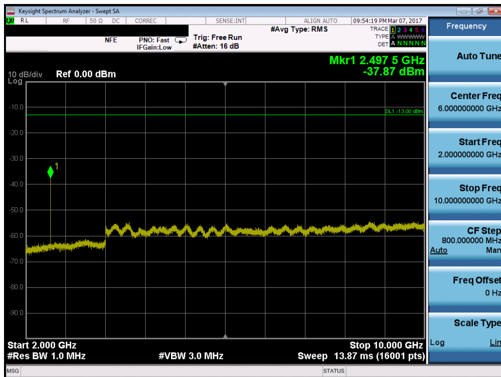
Plot 7-57. Conducted Spurious Plot (Band 5/26 – 10.0MHz QPSK – RB Size 1, RB Offset 0 – Mid Channel)
