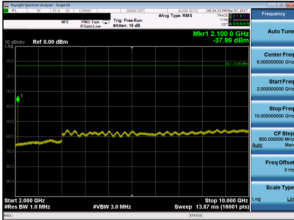
Plot 7-42. Conducted Spurious Plot (Band 17 – 10.0MHz QPSK – RB Size 1, RB Offset 0 – Low Channel)
