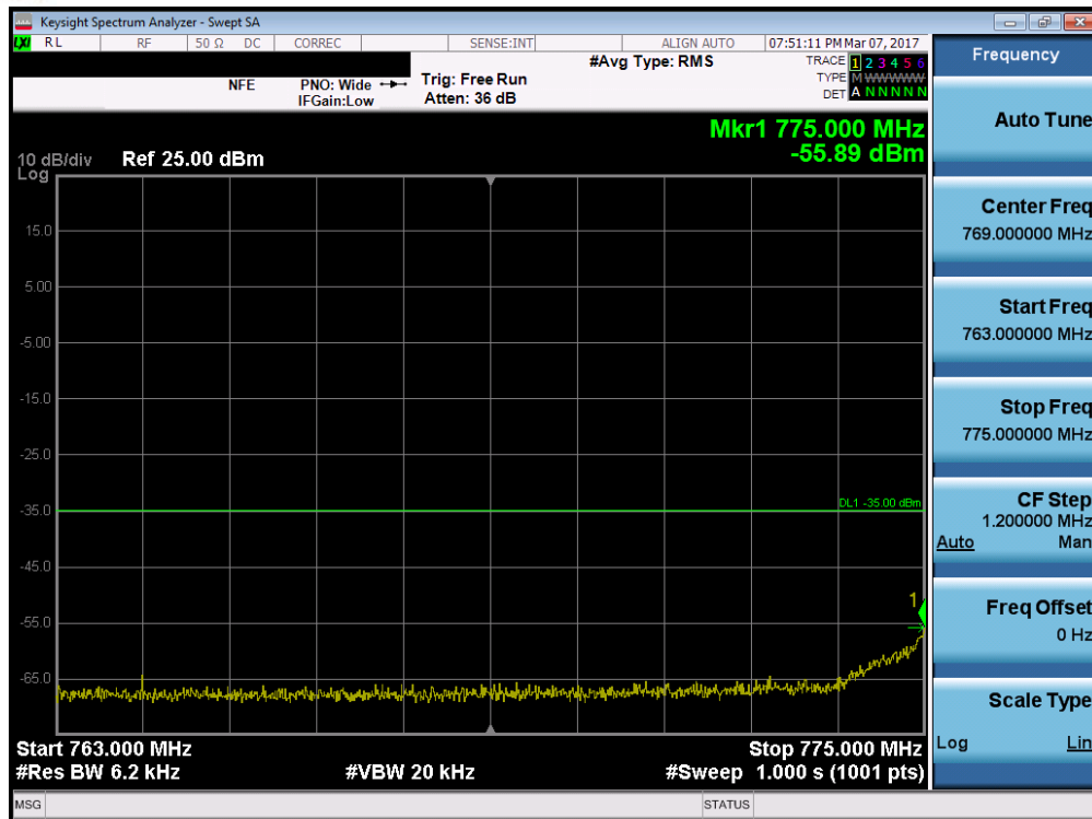
Plot 7-75. Lower Emission Mask Edge Plot (Band 13 - 5.0MHz QPSK - RB Size 25)
