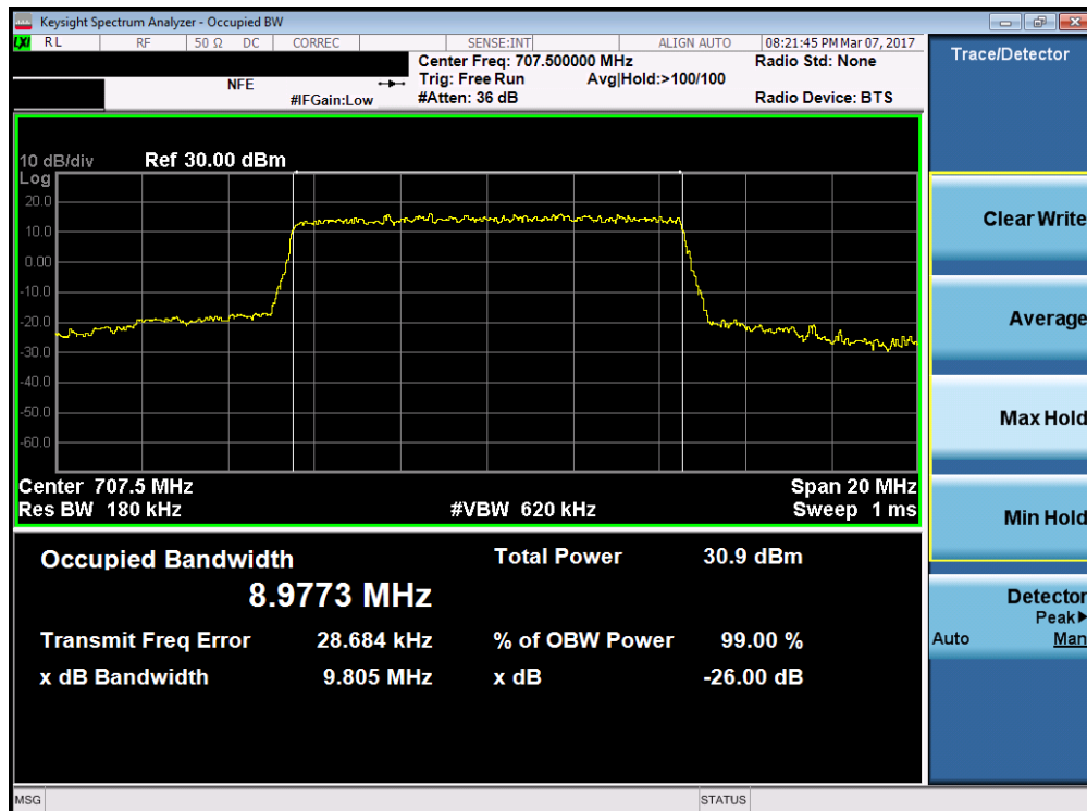
Plot 7-4. Occupied Bandwidth Plot (Band 17 – 10.0MHz QPSK – RB Size 50)
