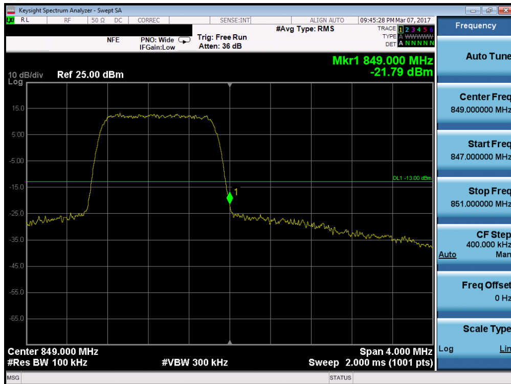
Plot 7-83. Upper Band Edge Plot (Band 5/26 - 1.4MHz QPSK - RB Size 6)
