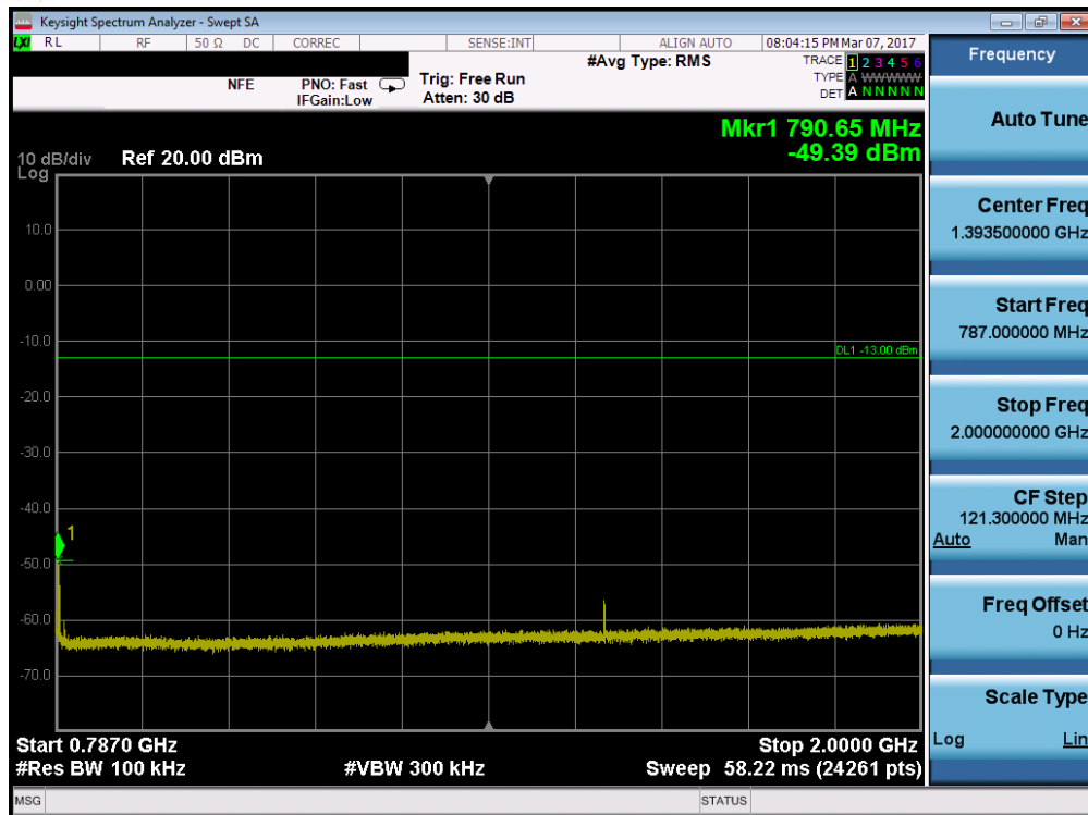
Plot 7-50. Conducted Spurious Plot (Band 13 – 10.0MHz QPSK – RB Size 1, RB Offset 0)
