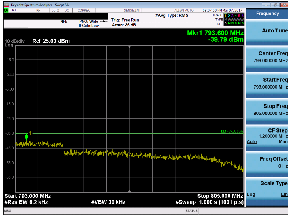
Plot 7-81. Upper Emission Mask Edge Plot (Band 13 – 10.0MHz QPSK – RB Size 50)
