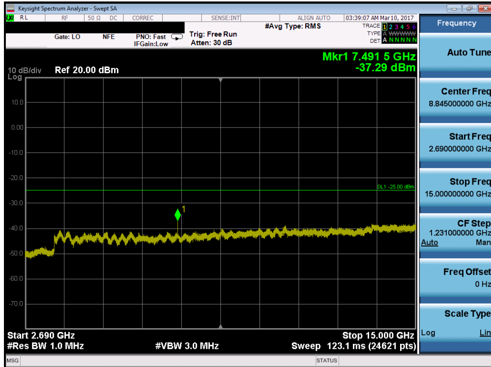
Plot 7-62. Conducted Spurious Plot (Band 41 – 20.0MHz QPSK – RB Size 1, RB Offset 0 – Low Channel)
