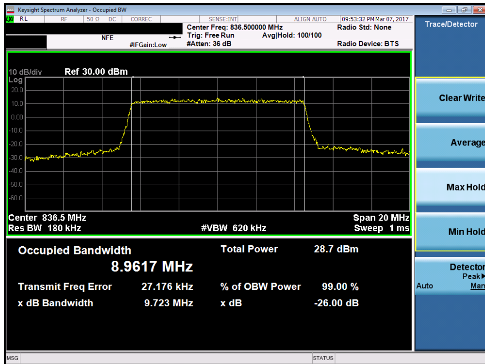
Plot 7-24. Occupied Bandwidth Plot (Band 5/26 – 10.0MHz 64-QAM – RB Size 50)
