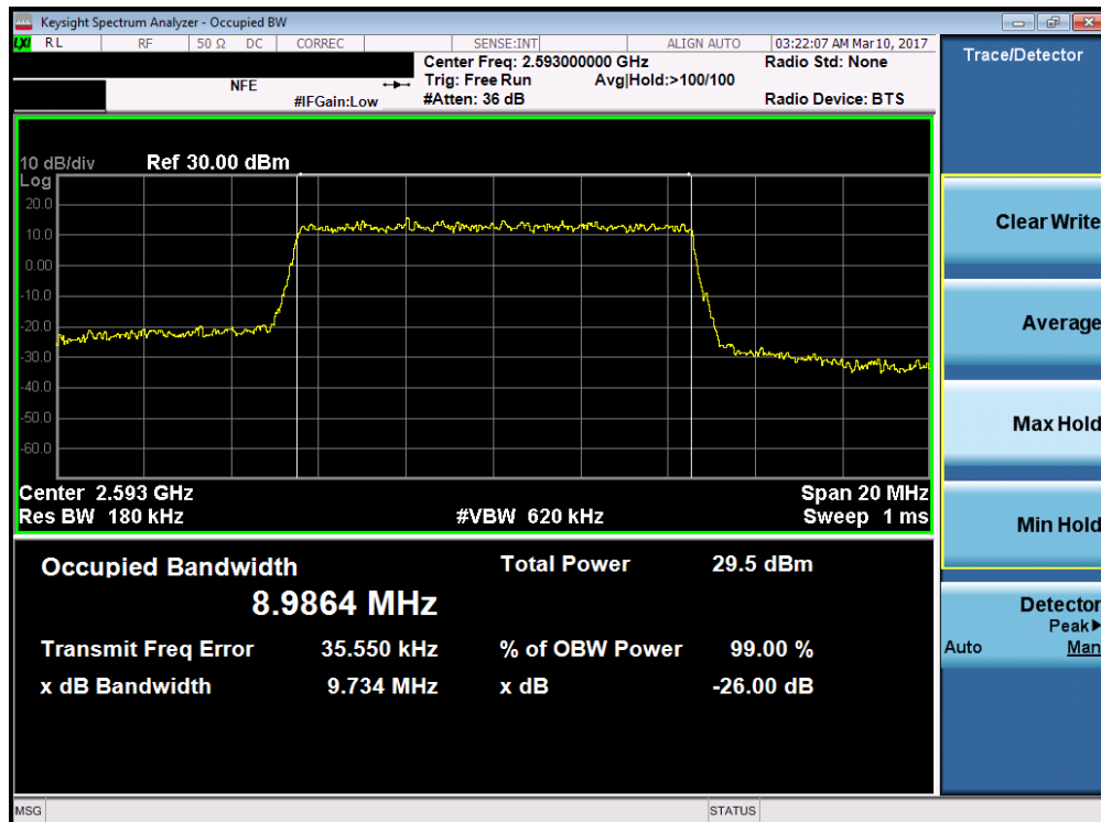
Plot 7-32. Occupied Bandwidth Plot (Band 41 – 10.0MHz 16-QAM – RB Size 50)
