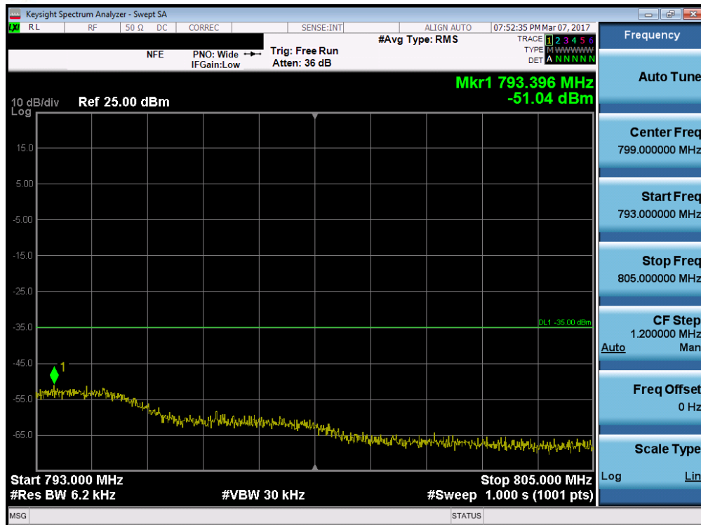
Plot 7-77. Upper Emission Mask Edge Plot (Band 13 – 5.0MHz QPSK – RB Size 25)
