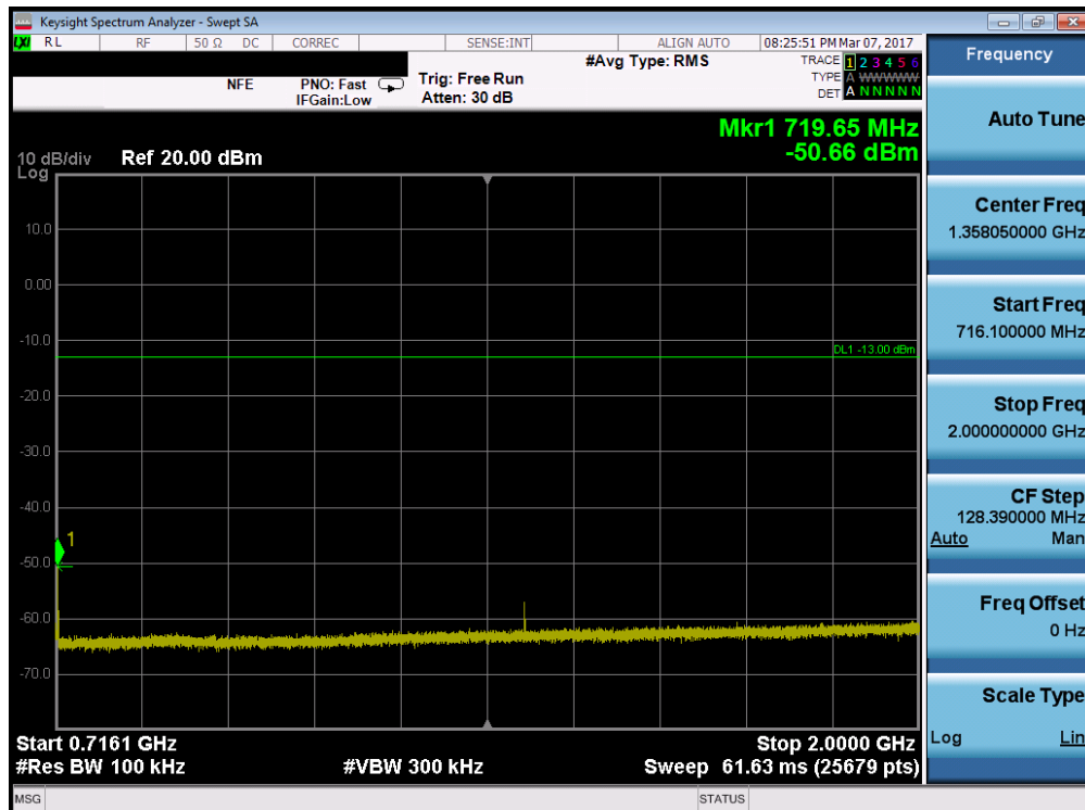
Plot 7-47. Conducted Spurious Plot (Band 17 – 10.0MHz QPSK – RB Size 1, RB Offset 0 – High Channel)
