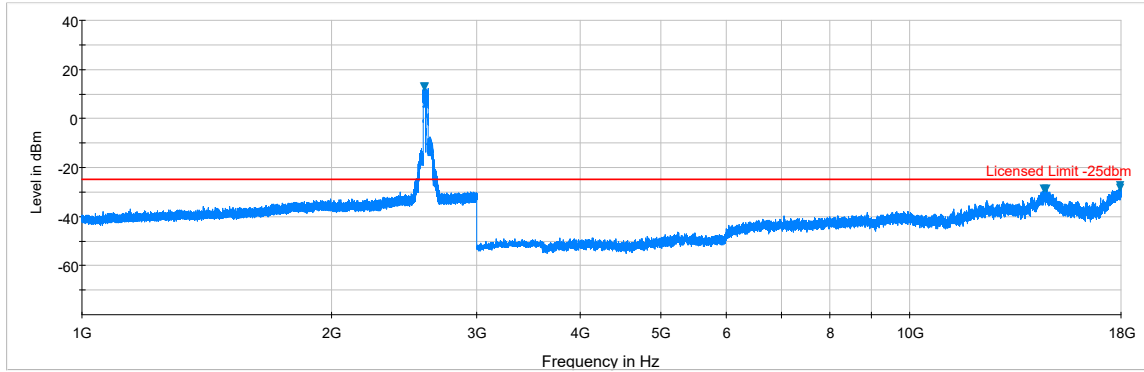
Plot 7-25. Radiated Spurious Plot (ULCA B41 PCC: RB 100 Offset 0, SCC: RB 100 Offset 0, Ant. Pol. H)
