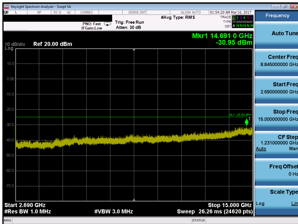
Plot 7-106. Conducted Spurious Plot (Band 41 – 20.0MHz QPSK – PCC 100/0, SCC 100/0 – Mid Channel)
