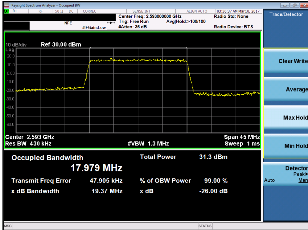
Plot 7-37. Occupied Bandwidth Plot (Band 41 – 20.0MHz QPSK – RB Size 100)
