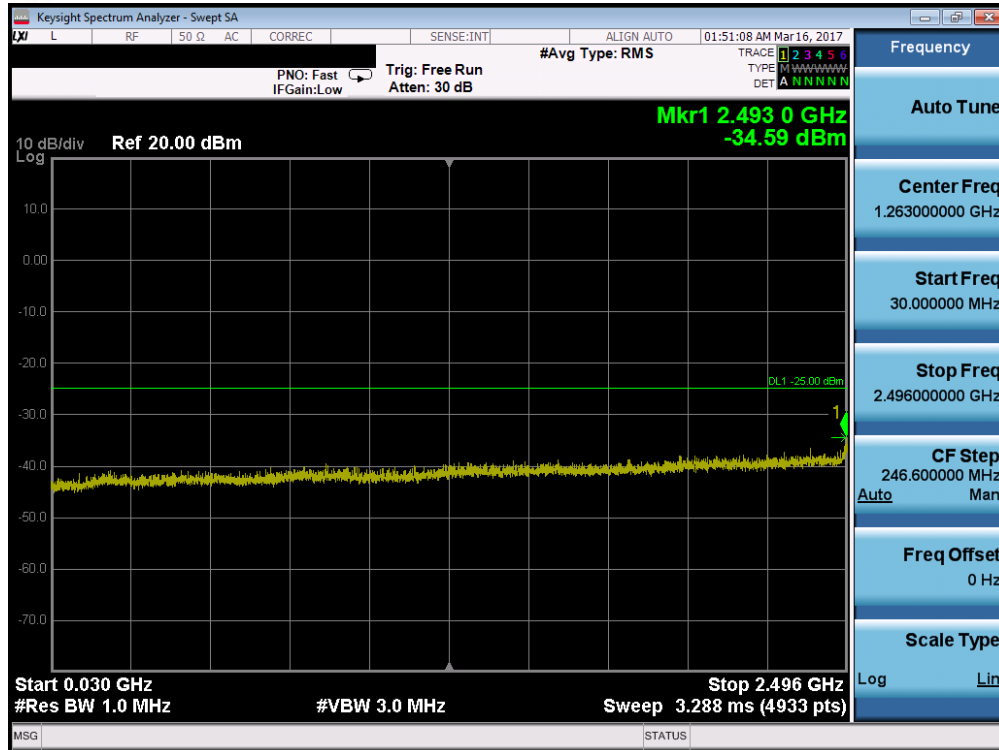
Plot 7-104. Conducted Spurious Plot (Band 41 – 20.0MHz QPSK – PCC 100/0, SCC 100/0 – Mid Channel)
