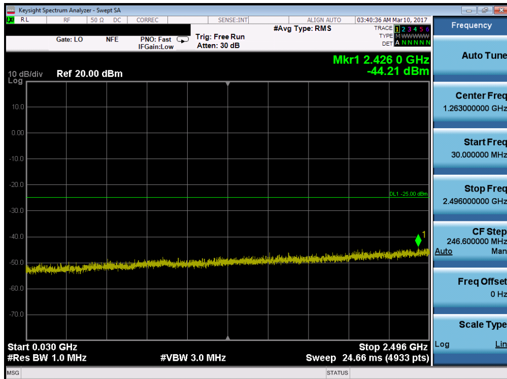
Plot 7-67. Conducted Spurious Plot (Band 41 – 20.0MHz QPSK – RB Size 1, RB Offset 0 – High Channel)
