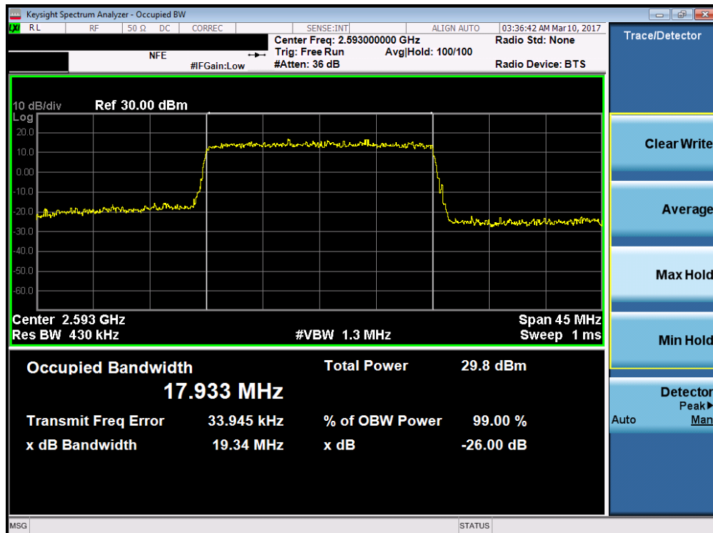
Plot 7-38. Occupied Bandwidth Plot (Band 41 – 20.0MHz 16-QAM – RB Size 100)
