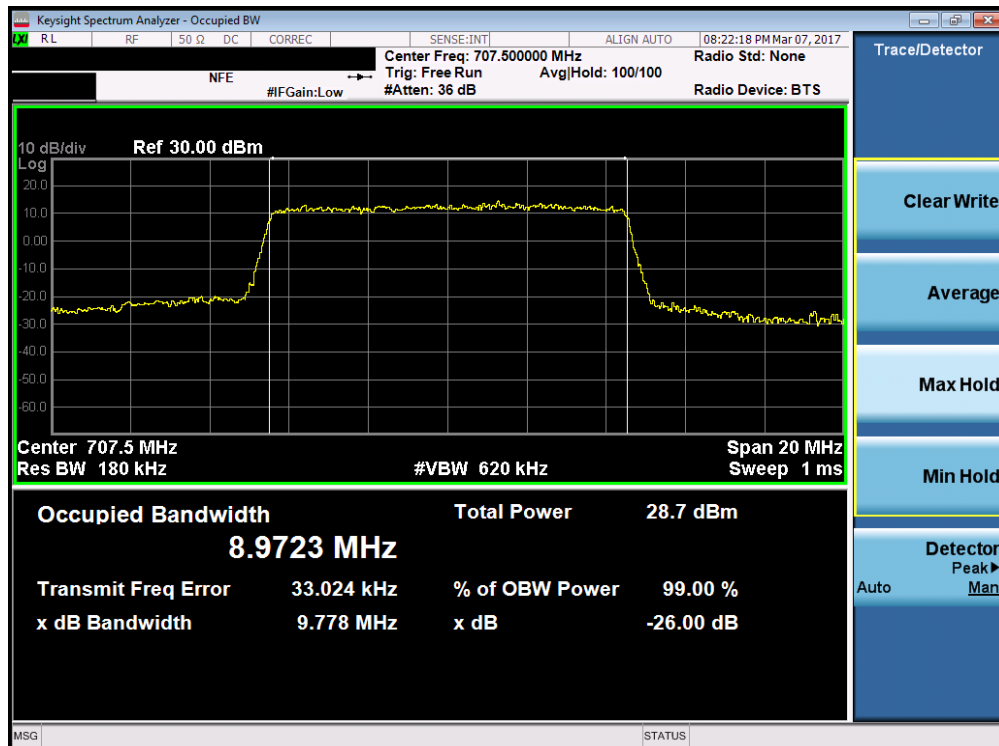
Plot 7-6. Occupied Bandwidth Plot (Band 17 – 10.0MHz 64-QAM – RB Size 50)
