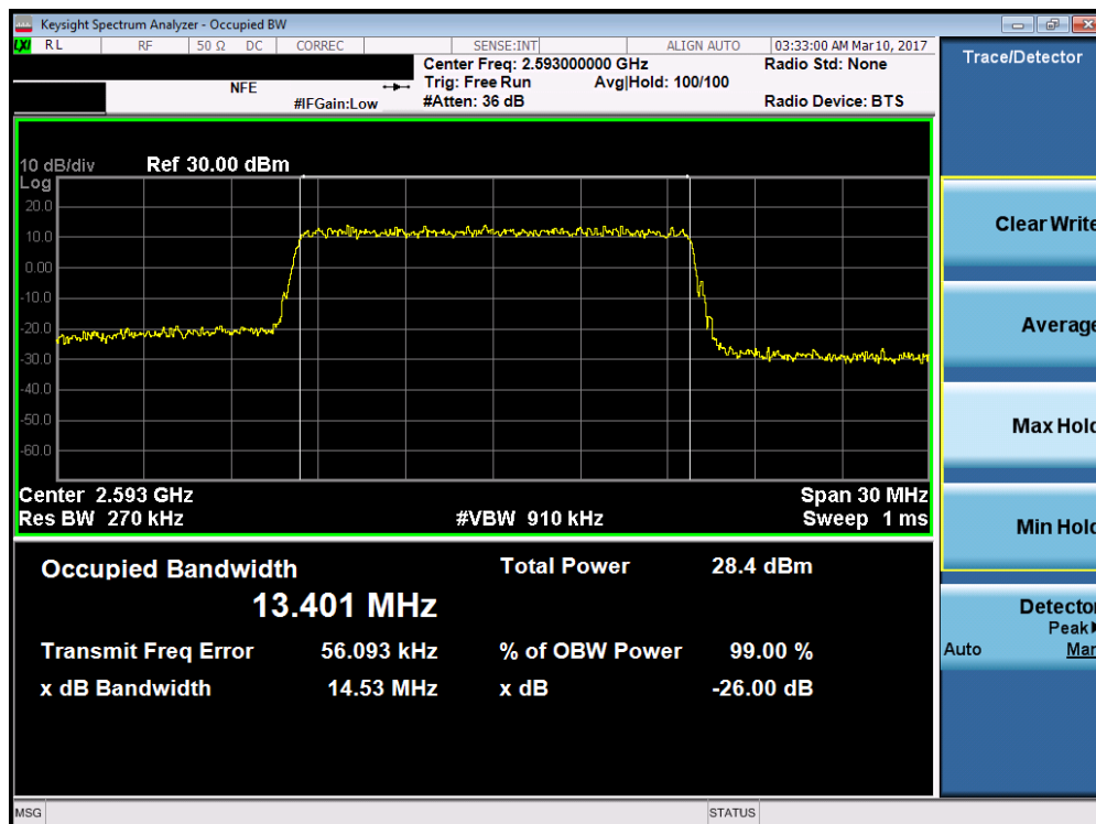
Plot 7-36. Occupied Bandwidth Plot (Band 41 – 15.0MHz 64-QAM – RB Size 75)
