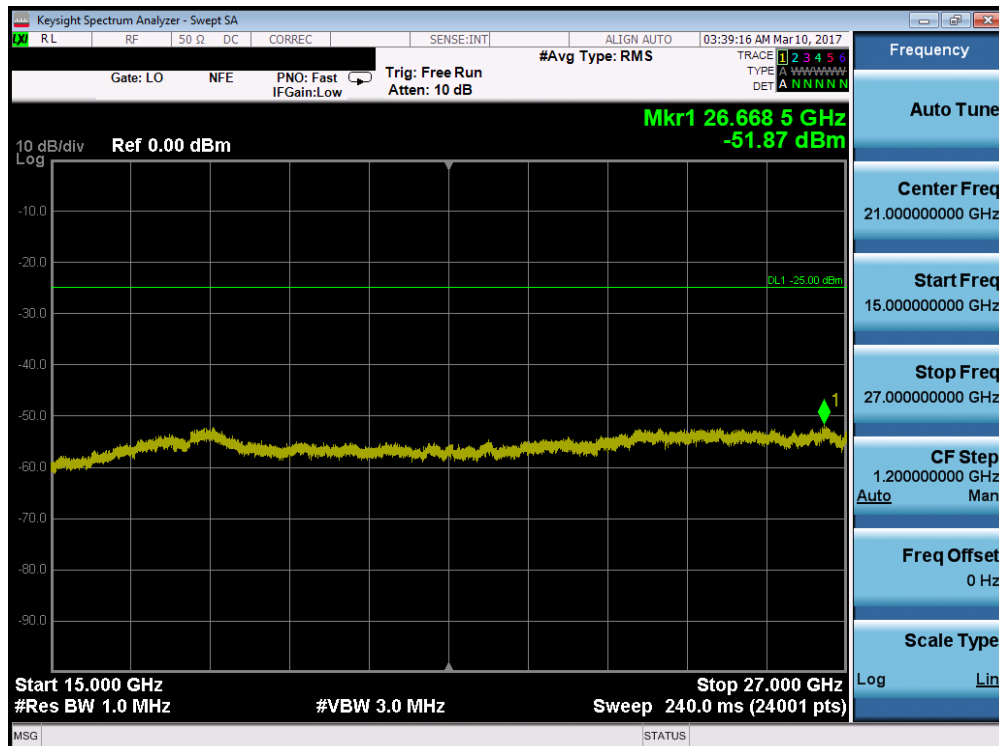
Plot 7-63. Conducted Spurious Plot (Band 41 – 20.0MHz QPSK – RB Size 1, RB Offset 0 – Low Channel)
