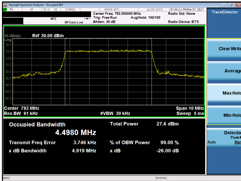
Plot 7-8. Occupied Bandwidth Plot (Band 13 – 5.0MHz 16-QAM – RB Size 25)
