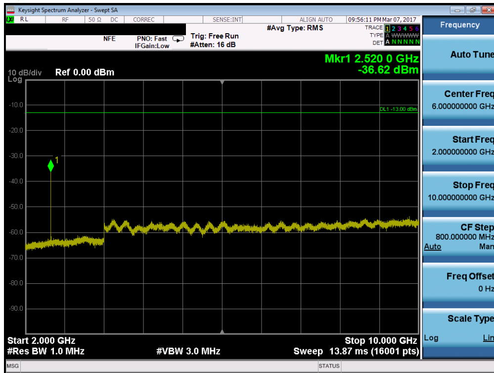
Plot 7-60. Conducted Spurious Plot (Band 5/26 – 10.0MHz QPSK – RB Size 1, RB Offset 0 – High Channel)
