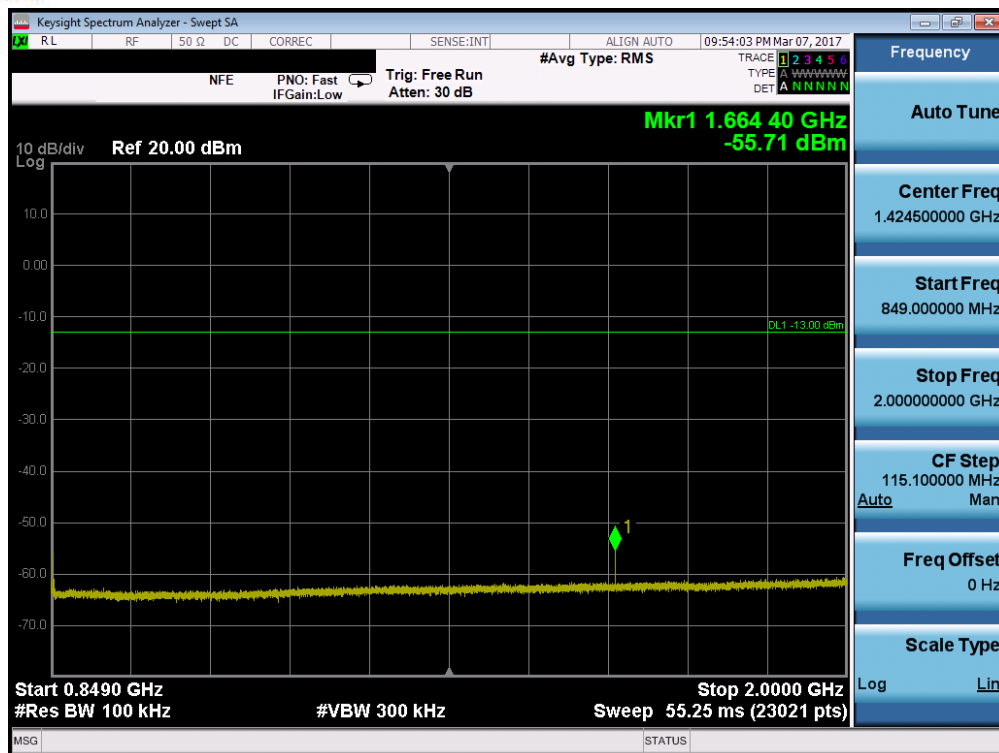
Plot 7-56. Conducted Spurious Plot (Band 5/26 – 10.0MHz QPSK – RB Size 1, RB Offset 0 – Mid Channel)
