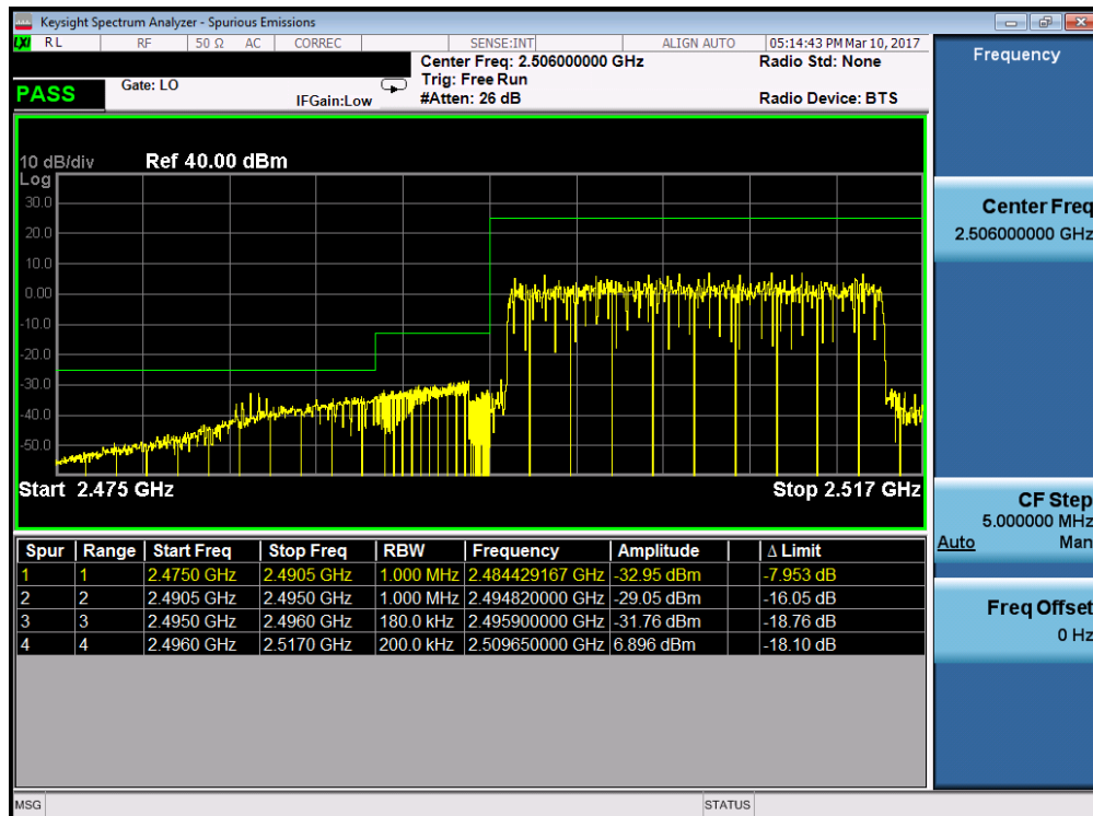
Plot 7-98. Lower ACP Plot (Band 41 – 20.0MHz QPSK – RB Size 100)
