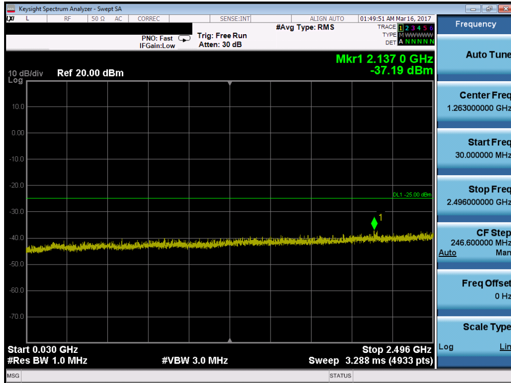
Plot 7-100. Conducted Spurious Plot (Band 41 – 20.0MHz QPSK – PCC 1/99 SCC 1/0 – Mid Channel)
