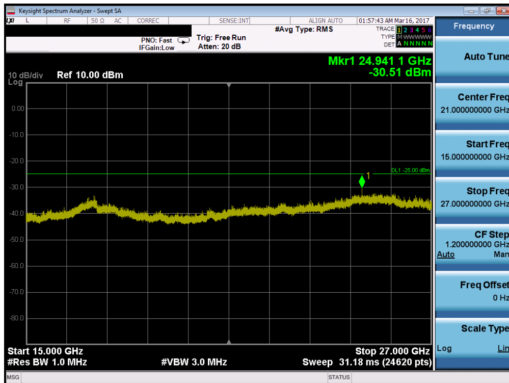
Plot 7-103. Conducted Spurious Plot (Band 41 – 20.0MHz QPSK – PCC 1/99, SCC 1/0 – Mid Channel)
