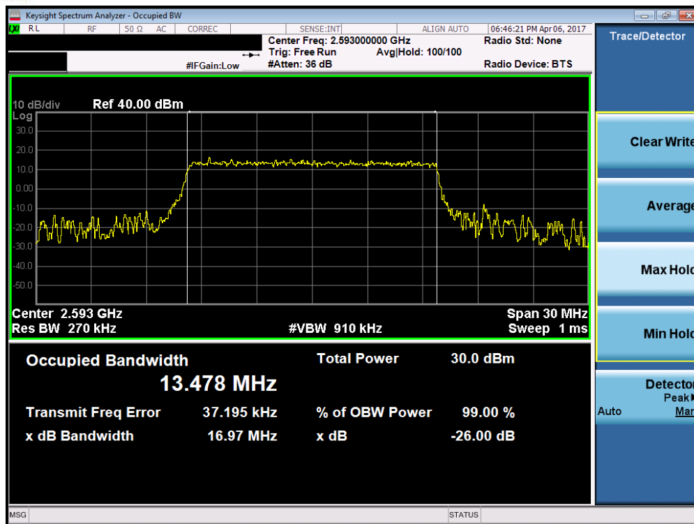
Plot 7-35. Occupied Bandwidth Plot (Band 41 – 15.0MHz 16-QAM – RB Size 75)
