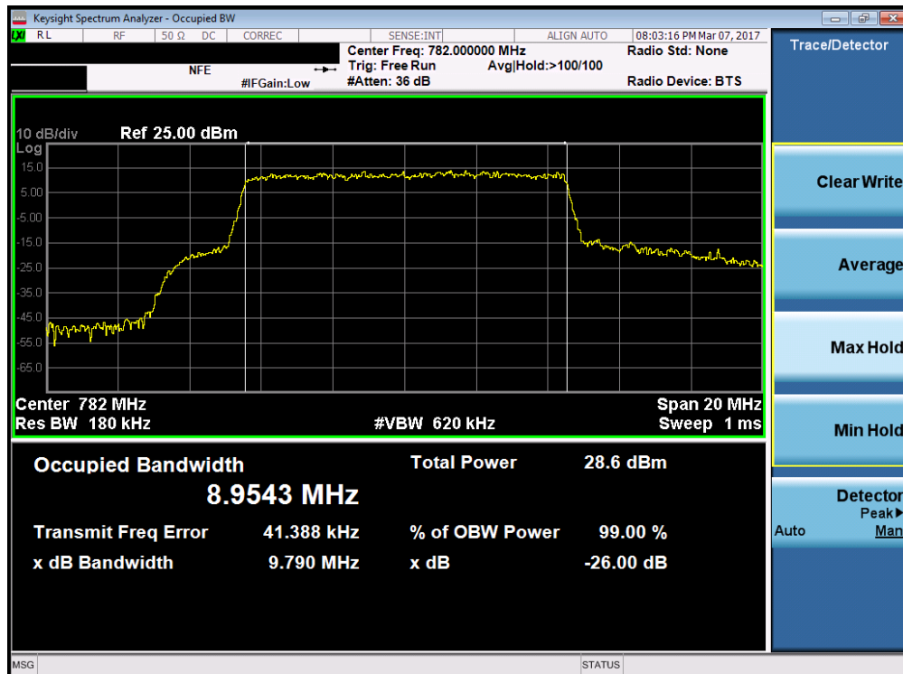
Plot 7-12. Occupied Bandwidth Plot (Band 13 – 10.0MHz 64-QAM – RB Size 50)
