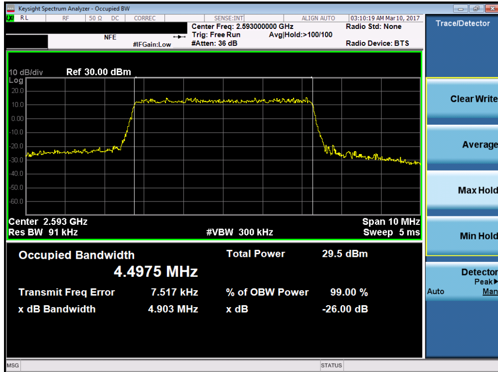
Plot 7-29. Occupied Bandwidth Plot (Band 41 – 5.0MHz 16-QAM – RB Size 25)
