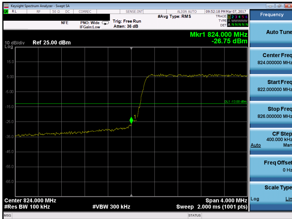
Plot 7-86. Lower Band Edge Plot (Band 5/26 – 5.0MHz QPSK – RB Size 25)
