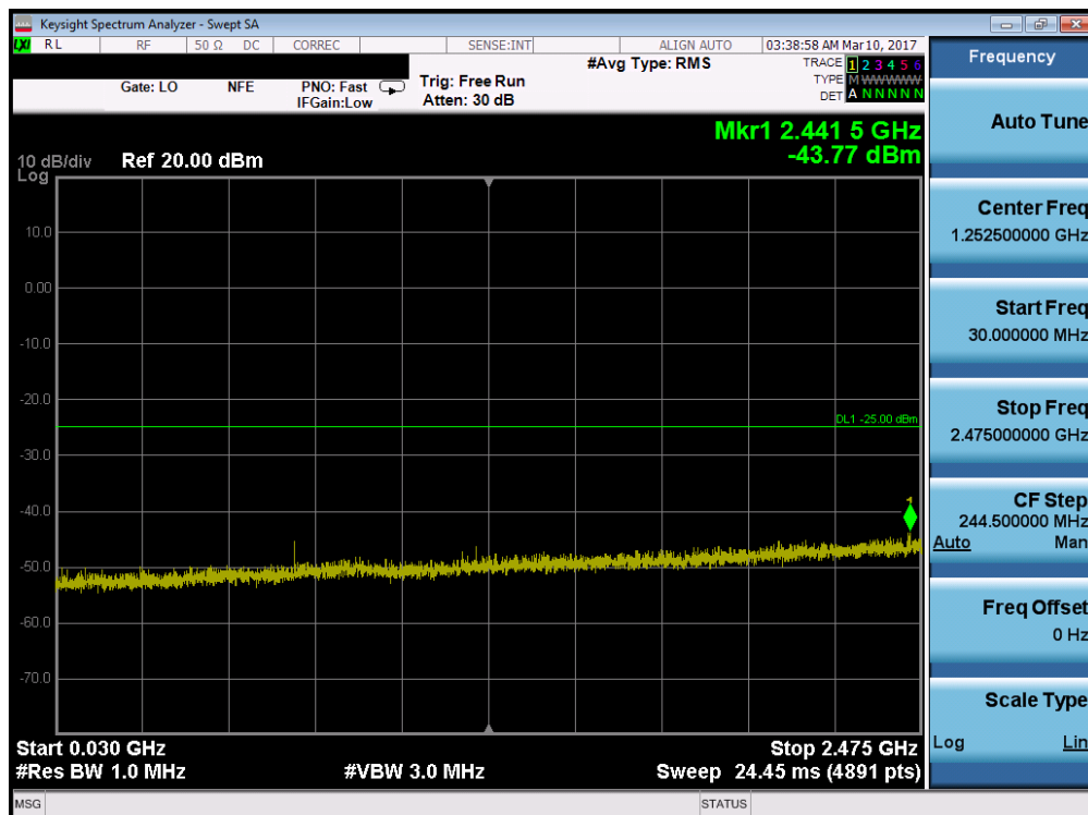
Plot 7-61. Conducted Spurious Plot (Band 41 – 20.0MHz QPSK – RB Size 1, RB Offset 0– Low Channel)
