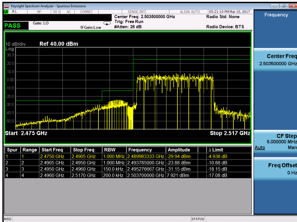
Plot 7-96. Lower ACP Plot (Band 41 – 15.0MHz QPSK – RB Size 75)
