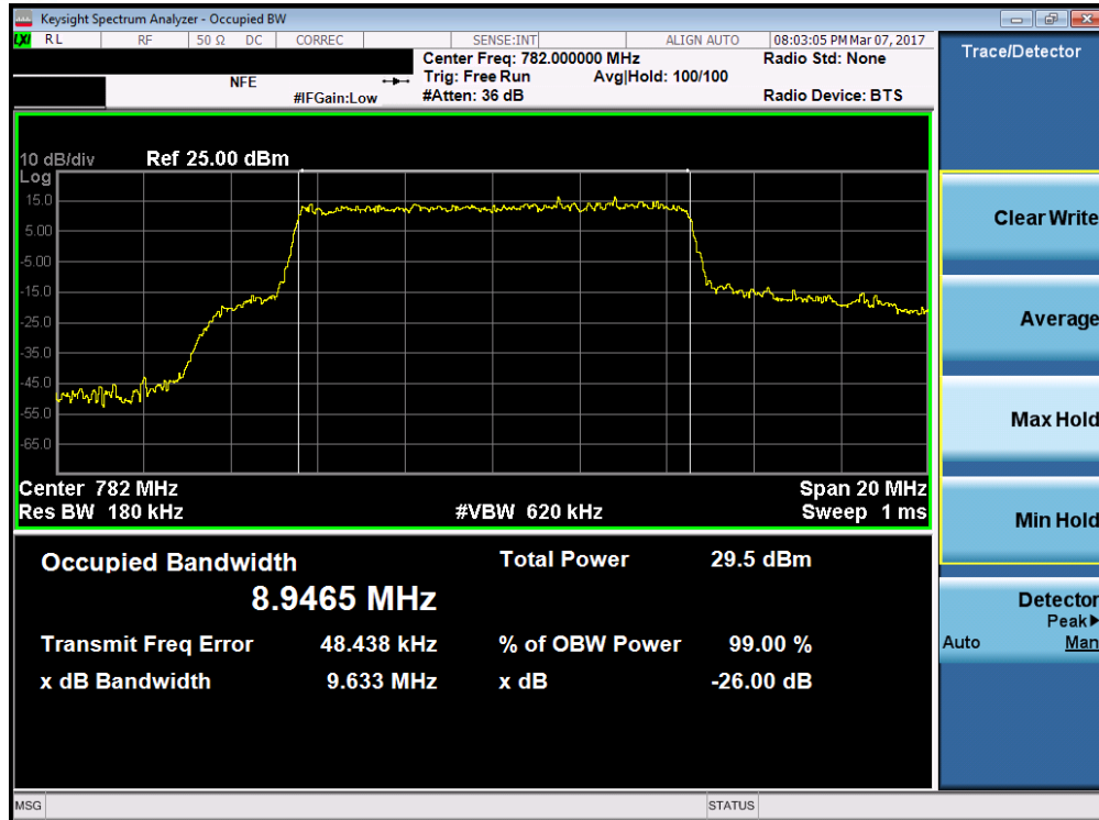
Plot 7-11. Occupied Bandwidth Plot (Band 13 – 10.0MHz 16-QAM – RB Size 50)
