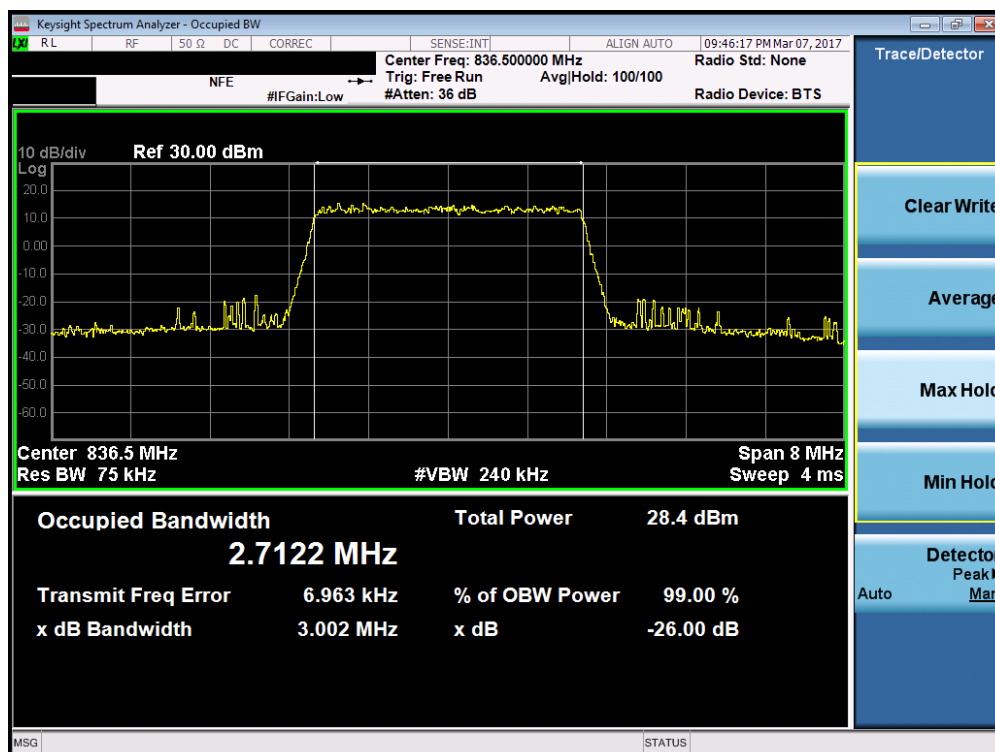
Plot 7-18. Occupied Bandwidth Plot (Band 5/26 – 3.0MHz 64-QAM – RB Size 15)
