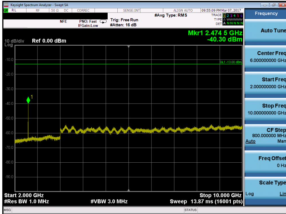
Plot 7-54. Conducted Spurious Plot (Band 5/26 – 10.0MHz QPSK – RB Size 1, RB Offset 0 – Low Channel)
