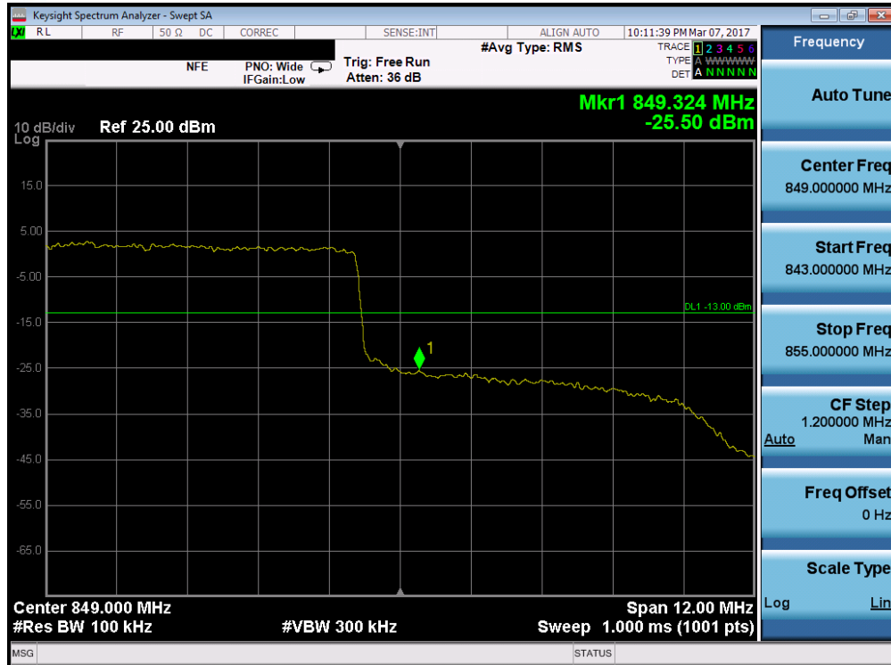
Plot 7-91. Upper Band Edge Plot (Band 26 – 15.0MHz QPSK – RB Size 75)
