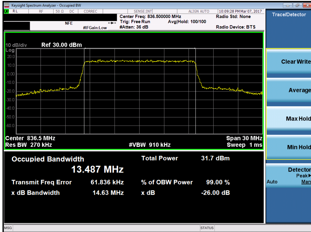
Plot 7-25. Occupied Bandwidth Plot (Band 26 – 15.0MHz QPSK – RB Size 75)
