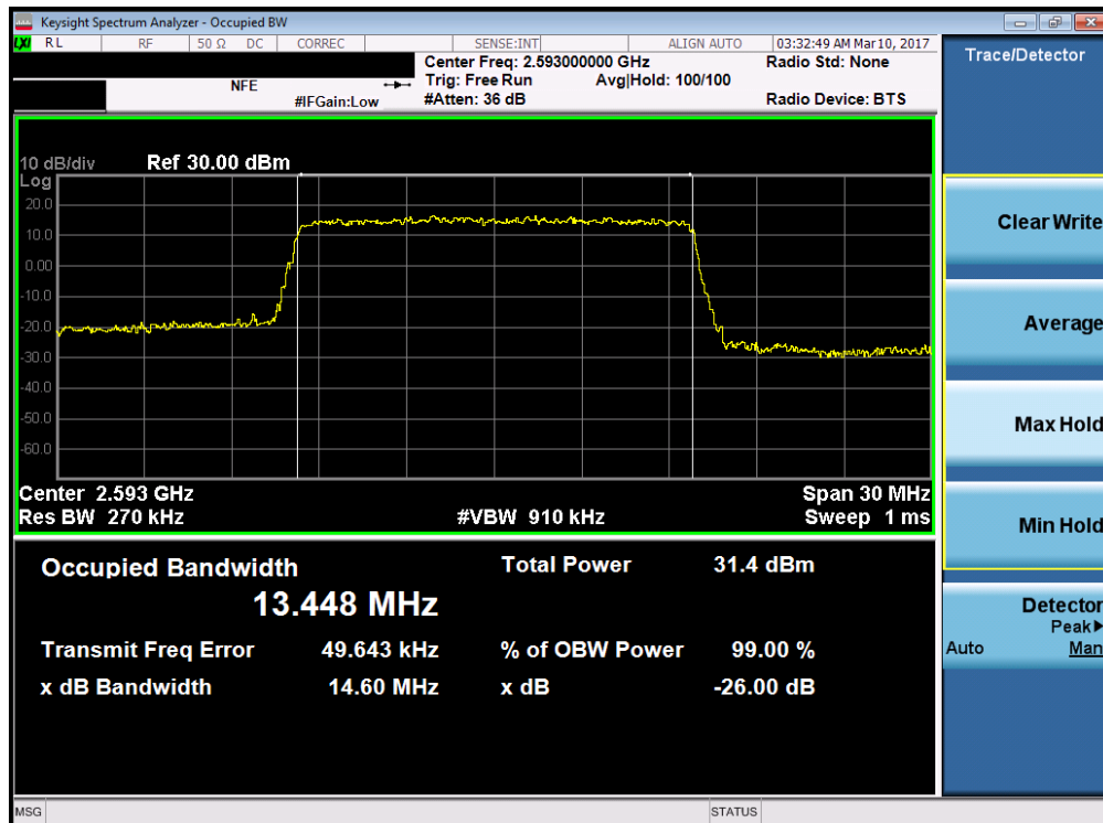
Plot 7-34. Occupied Bandwidth Plot (Band 41 – 15.0MHz QPSK – RB Size 75)
