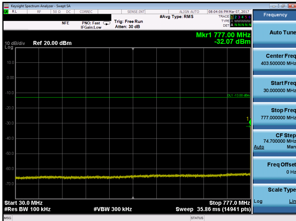
Plot 7-49. Conducted Spurious Plot (Band 13 – 10.0MHz QPSK – RB Size 1, RB Offset 0)
