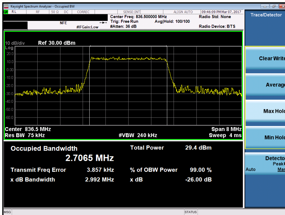
Plot 7-17. Occupied Bandwidth Plot (Band 5/26 – 3.0MHz 16-QAM – RB Size 15)
