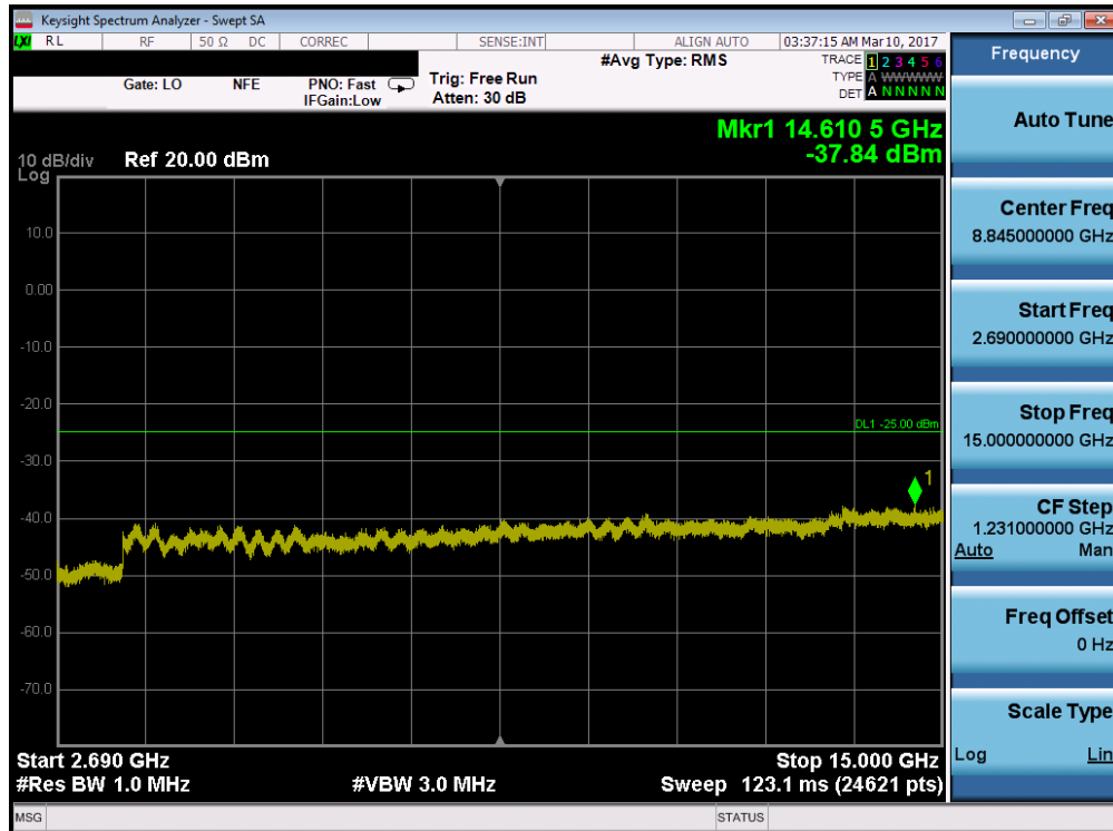
Plot 7-65. Conducted Spurious Plot (Band 41 – 20.0MHz QPSK – RB Size 1, RB Offset 0 – Mid Channel)
