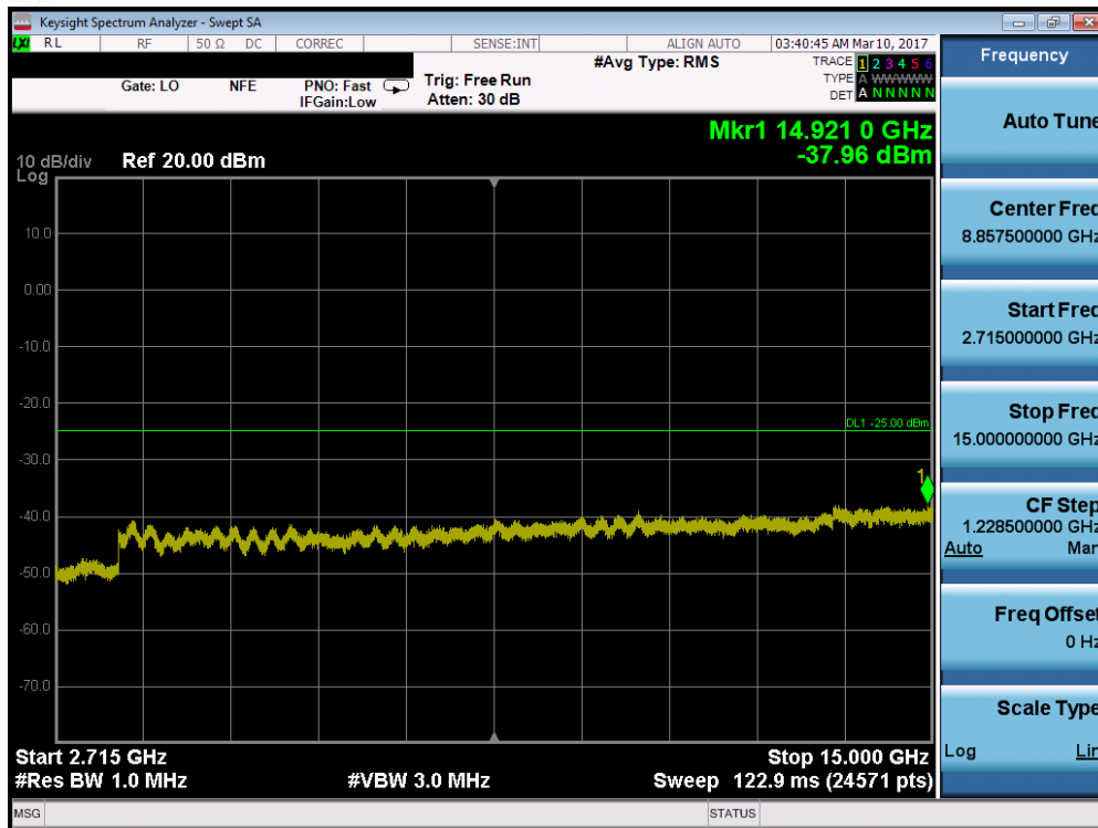
Plot 7-68. Conducted Spurious Plot (Band 41 – 20.0MHz QPSK – RB Size 1, RB Offset 0 – High Channel)
