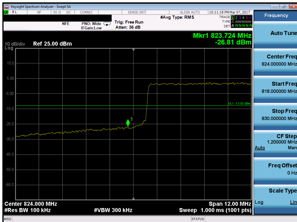
Plot 7-90. Lower Band Edge Plot (Band 26 – 15.0MHz QPSK – RB Size 75)
