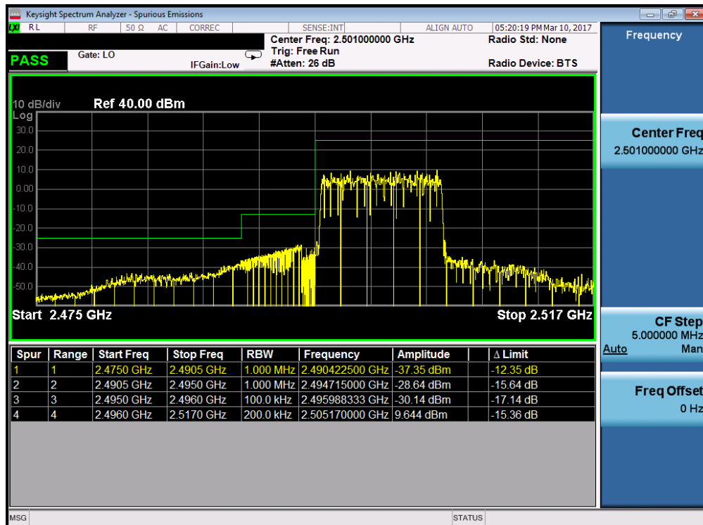
Plot 7-94. Lower ACP Plot (Band 41 – 10.0MHz QPSK – RB Size 50)
