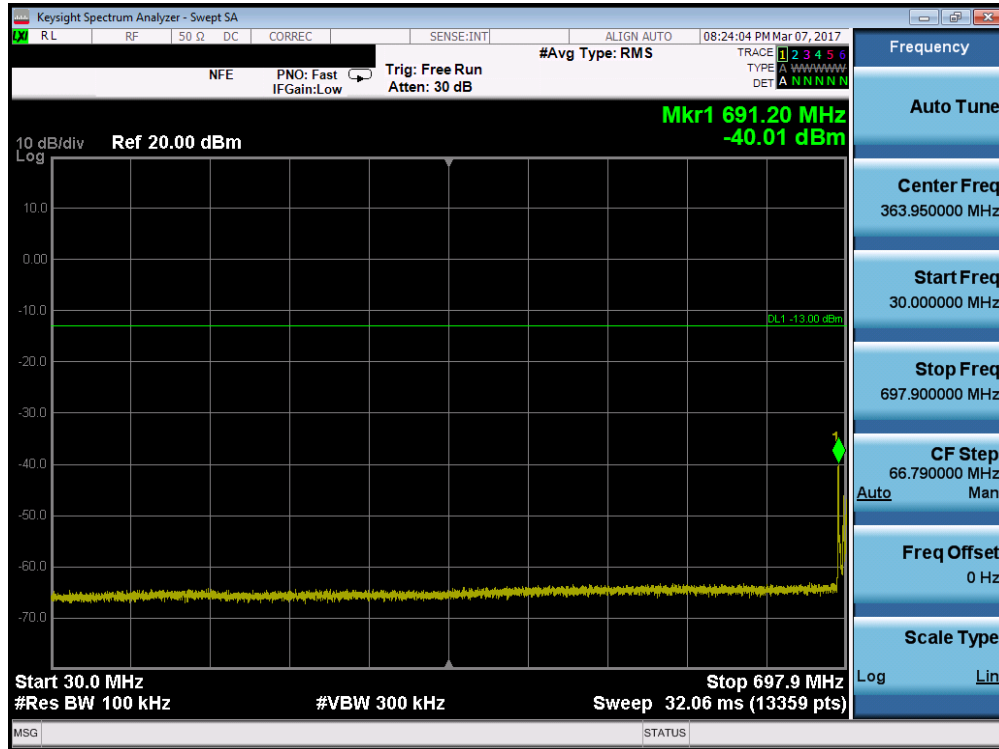
Plot 7-40. Conducted Spurious Plot (Band 17 – 10.0MHz QPSK – RB Size 1, RB Offset 0– Low Channel)
