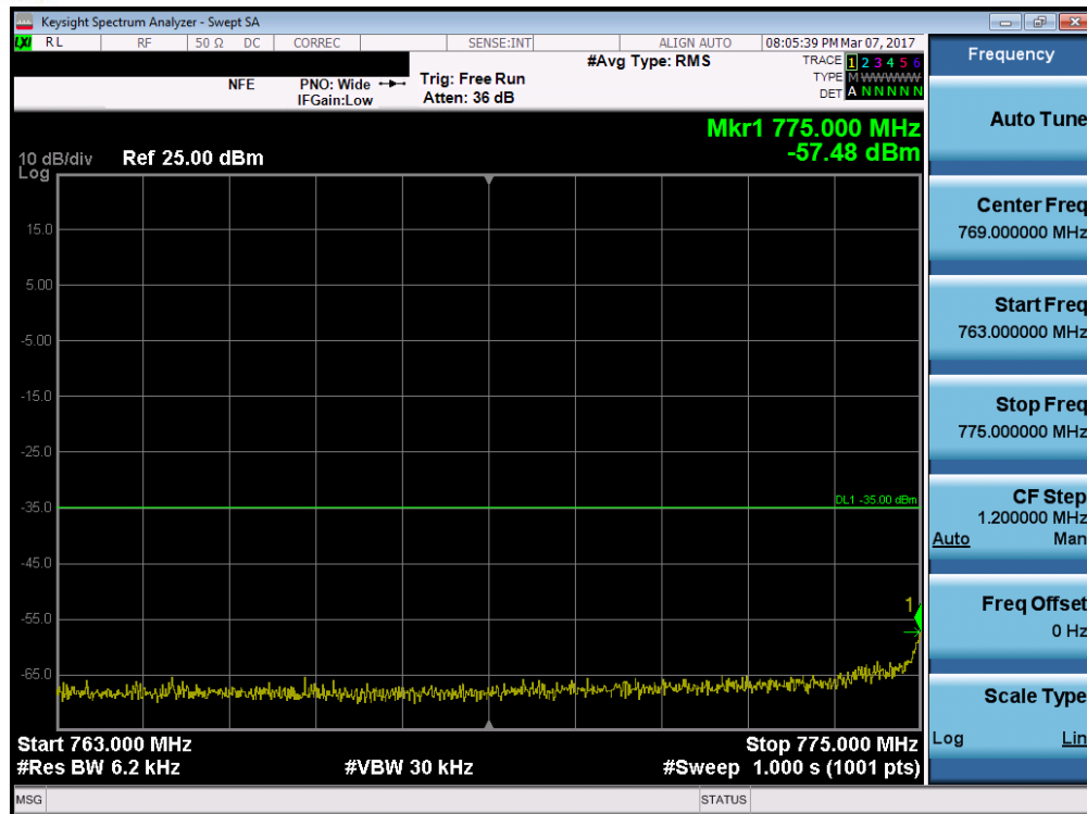
Plot 7-79. Lower Emission Mask Edge Plot (Band 13 – 10.0MHz QPSK – RB Size 50)
