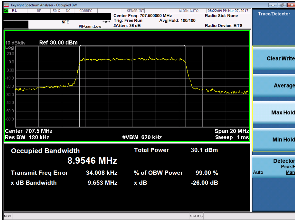
Plot 7-5. Occupied Bandwidth Plot (Band 17 – 10.0MHz 16-QAM – RB Size 50)
