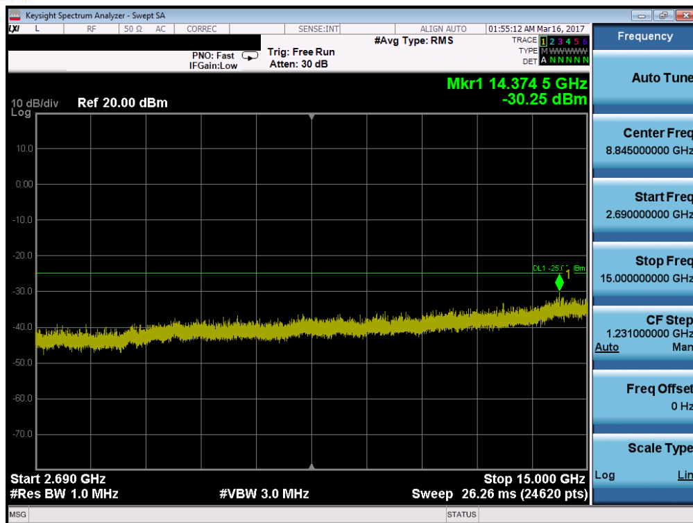
Plot 7-102. Conducted Spurious Plot (Band 41 – 20.0MHz QPSK – PCC 1/99 ,SCC 1/0 – Mid Channel)
