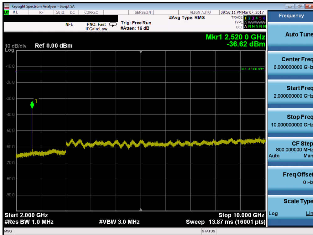
Plot 7-53. Conducted Spurious Plot (Band 5/26 – 10.0MHz QPSK – RB Size 1, RB Offset 0 – Low Channel)
