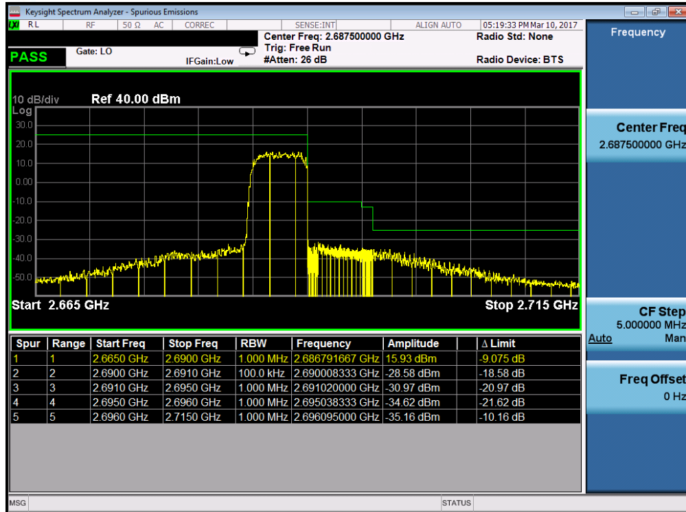
Plot 7-93. Upper ACP Plot (Band 41 – 5.0MHz QPSK – RB Size 25)
