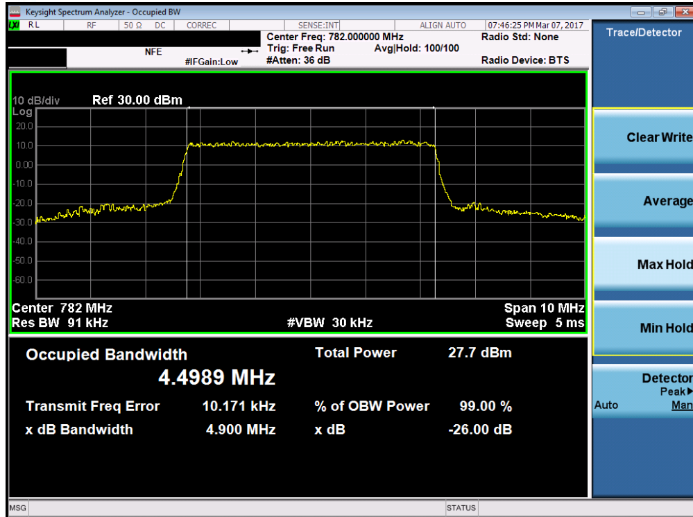
Plot 7-9. Occupied Bandwidth Plot (Band 13 – 5.0MHz 64-QAM – RB Size 25)
