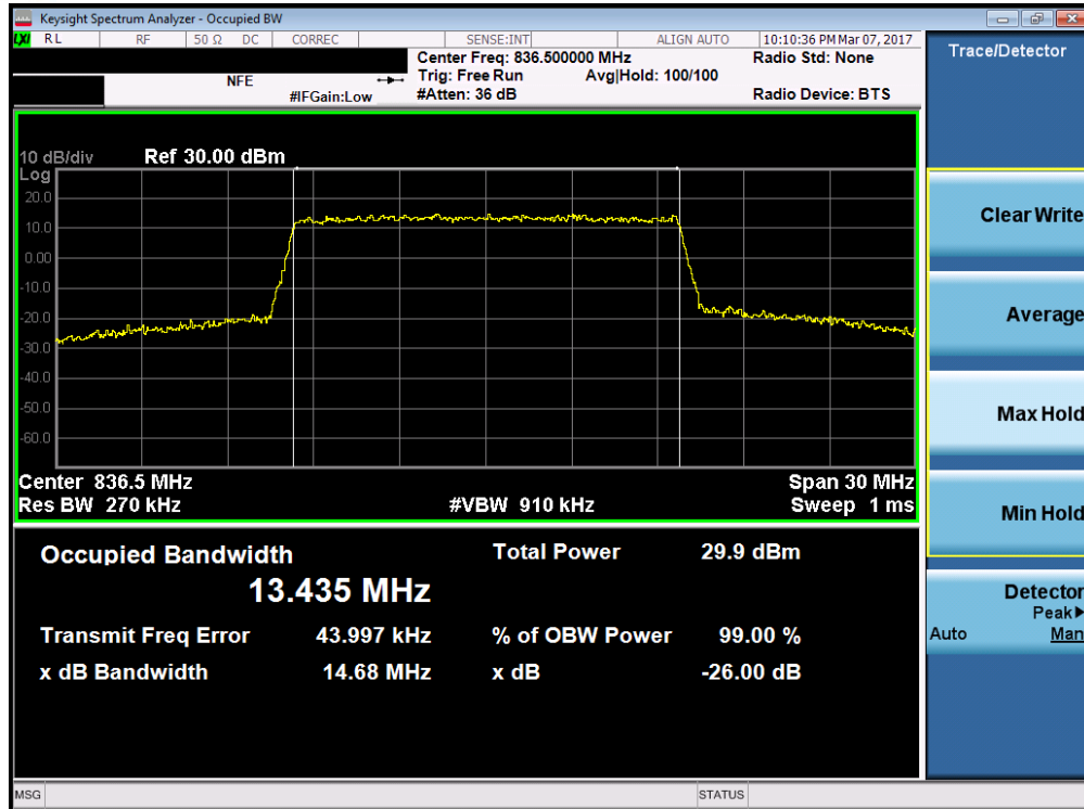
Plot 7-27. Occupied Bandwidth Plot (Band 26 – 15.0MHz 64-QAM – RB Size 75)
