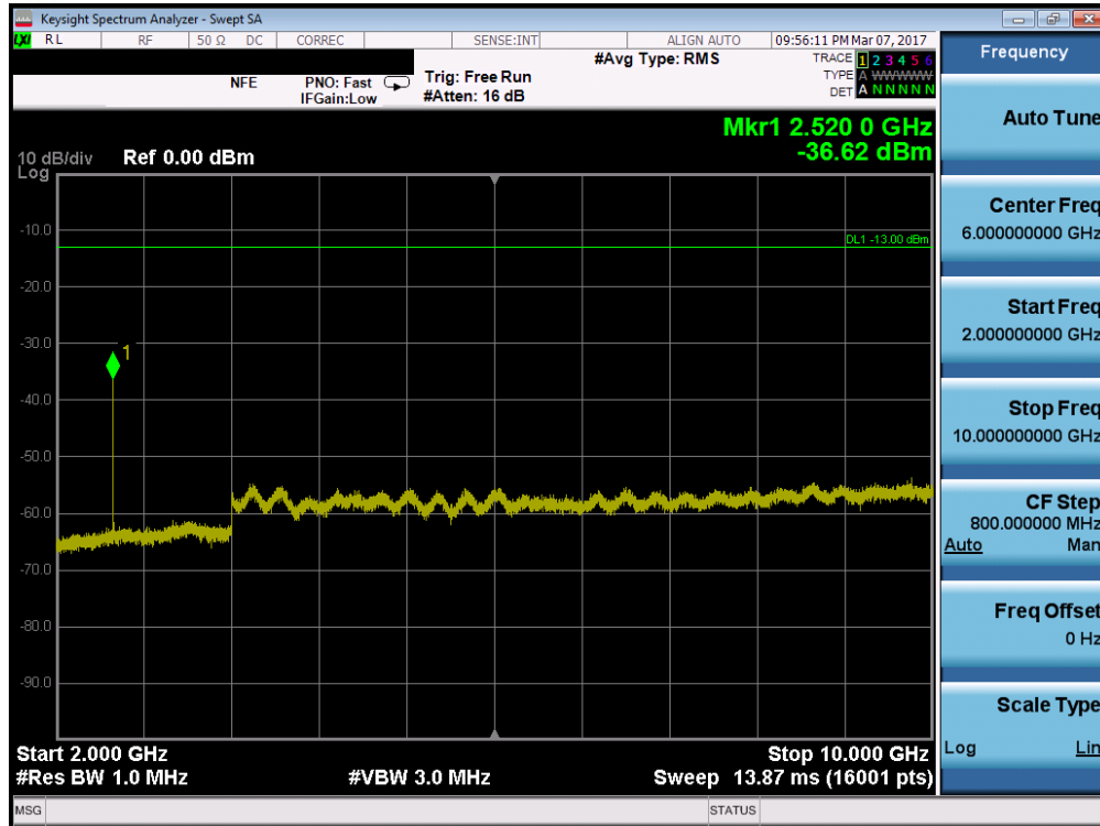
Plot 7-52. Conducted Spurious Plot (Band 5/26 – 10.0MHz QPSK – RB Size 1, RB Offset 0– Low Channel)
