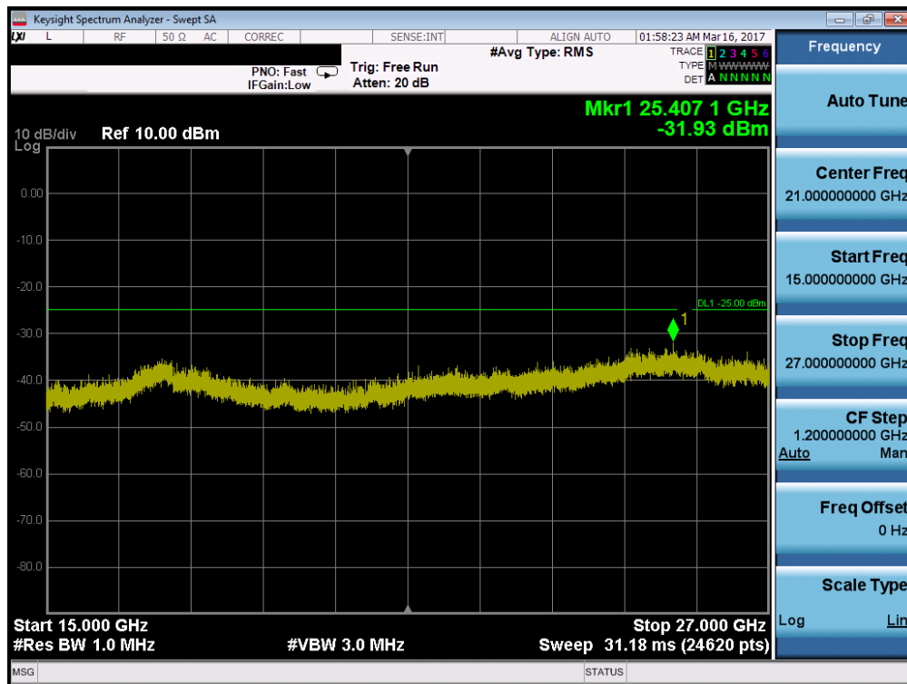
Plot 7-107. Conducted Spurious Plot (Band 41 – 20.0MHz QPSK – PCC 100/0, SCC 100/0 – Mid Channel)
