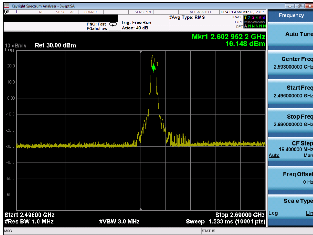
Plot 7-101. Conducted Spurious Plot (Band 41 – 20.0MHz QPSK – PCC 1/99 SCC 1/0 – Mid Channel)
