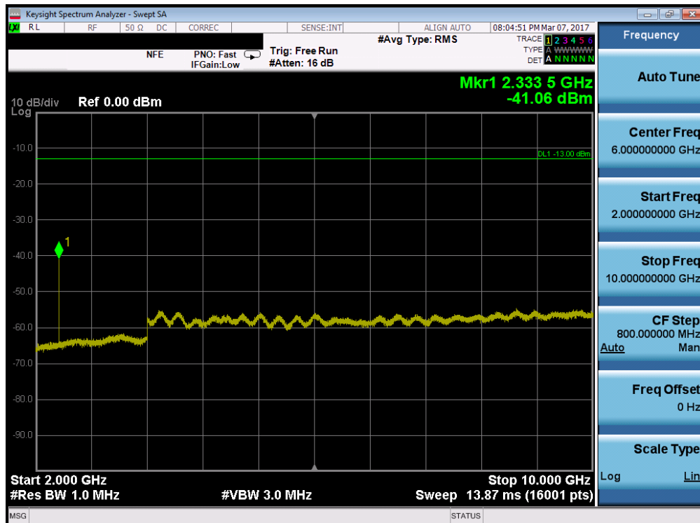
Plot 7-51. Conducted Spurious Plot (Band 13 – 10.0MHz QPSK – RB Size 1, RB Offset 0)
