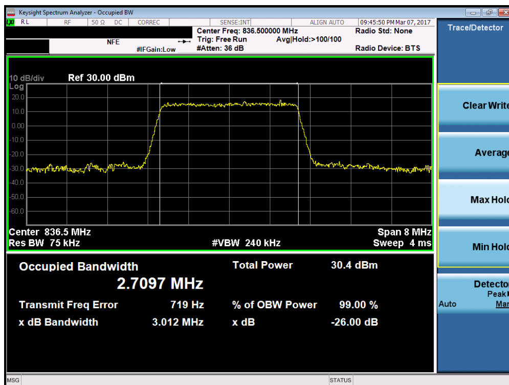
Plot 7-16. Occupied Bandwidth Plot (Band 5/26 – 3.0MHz QPSK – RB Size 15)
