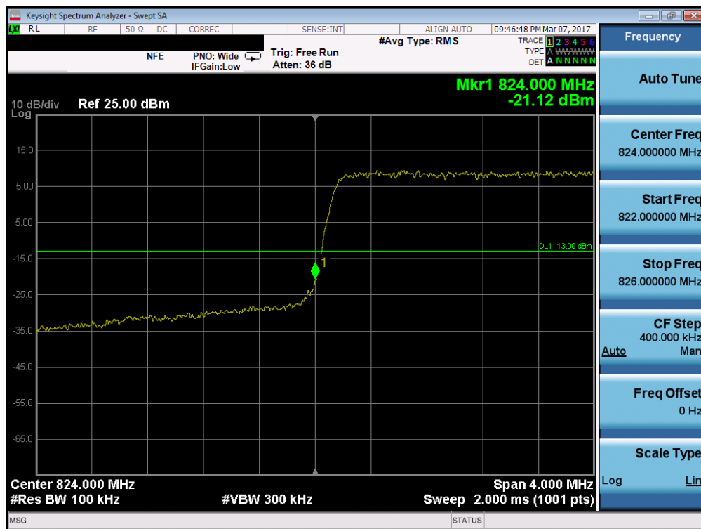
Plot 7-84. Lower Band Edge Plot (Band 5/26 - 3.0MHz QPSK - RB Size 15)
