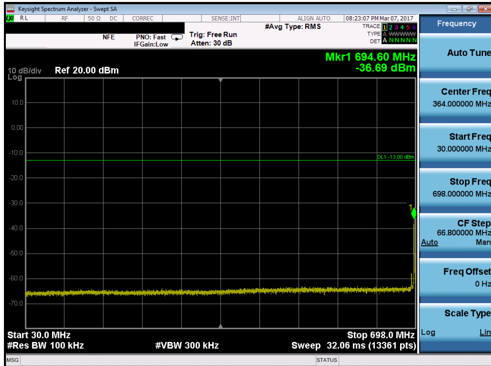
Plot 7-43. Conducted Spurious Plot (Band 17 – 10.0MHz QPSK – RB Size 1, RB Offset 0 – Mid Channel)
