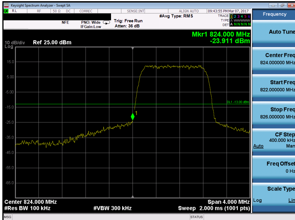
Plot 7-82. Lower Band Edge Plot (Band 5/26 – 1.4MHz QPSK – RB Size 6)
