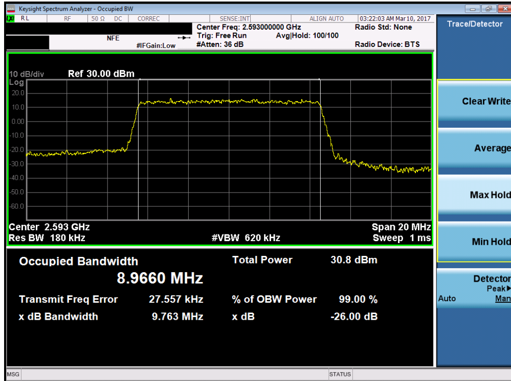
Plot 7-31. Occupied Bandwidth Plot (Band 41 – 10.0MHz QPSK – RB Size 50)
