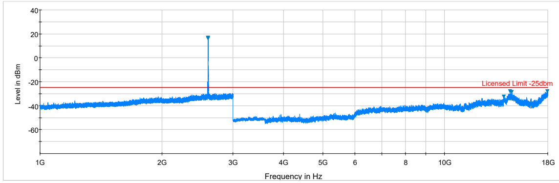
Plot 7-28. Radiated Spurious Plot (ULCA B41 PCC: RB 1 Offset 99, SCC: RB 1 Offset 0, Ant. Pol. V)
