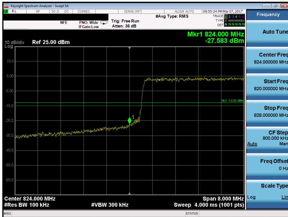
Plot 7-88. Lower Band Edge Plot (Band 5/26 - 10.0MHz QPSK - RB Size 50)
