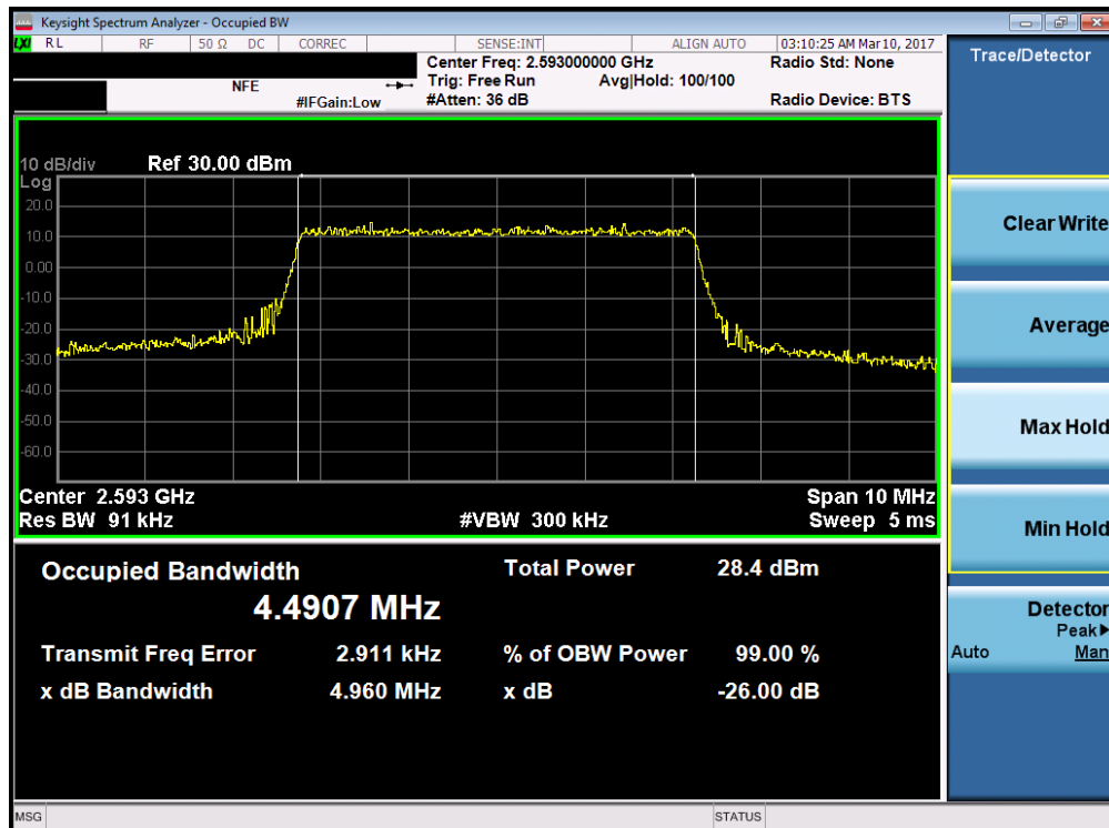
Plot 7-30. Occupied Bandwidth Plot (Band 41 – 5.0MHz 64-QAM – RB Size 25)
