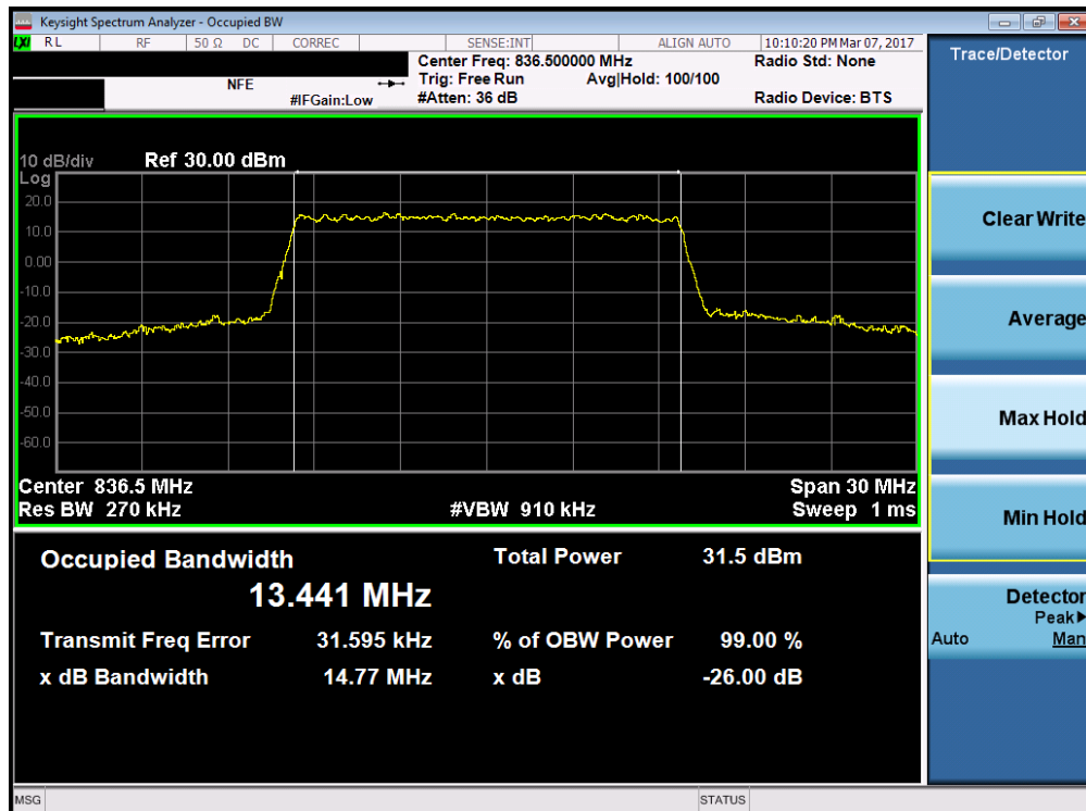
Plot 7-26. Occupied Bandwidth Plot (Band 26 – 15.0MHz 16-QAM – RB Size 75)
