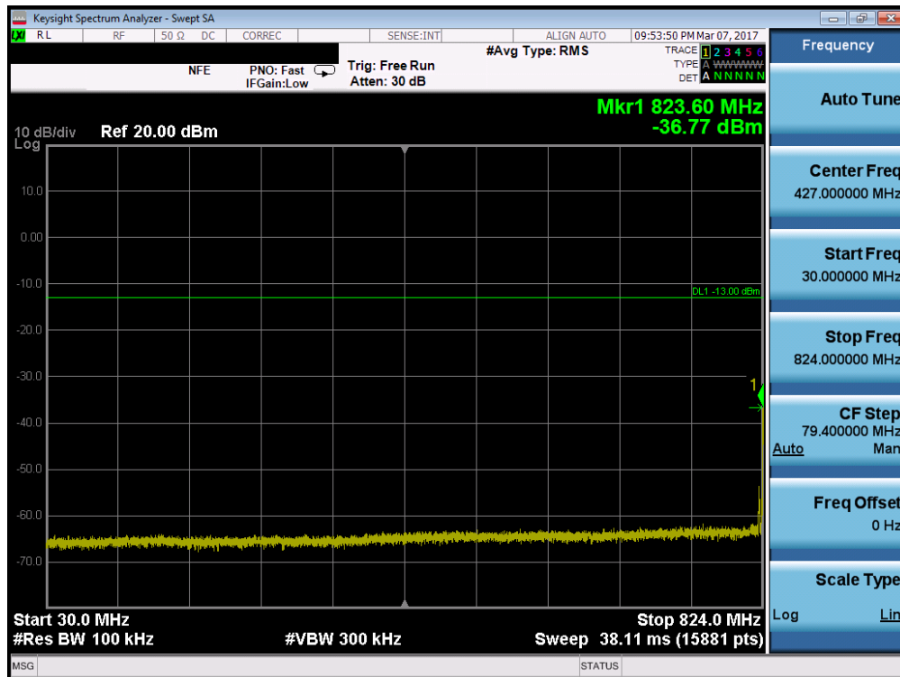
Plot 7-55. Conducted Spurious Plot (Band 5/26 – 10.0MHz QPSK – RB Size 1, RB Offset 0 – Mid Channel)
