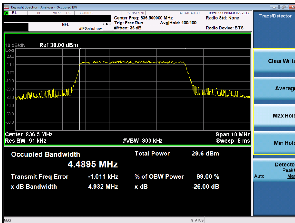
Plot 7-20. Occupied Bandwidth Plot (Band 5/26 - 5.0MHz 16-QAM - RB Size 25)
