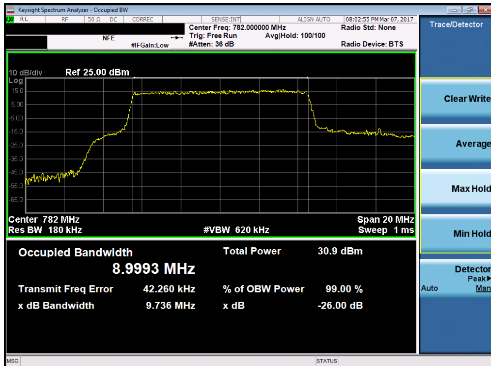
Plot 7-10. Occupied Bandwidth Plot (Band 13 – 10.0MHz QPSK – RB Size 50)
