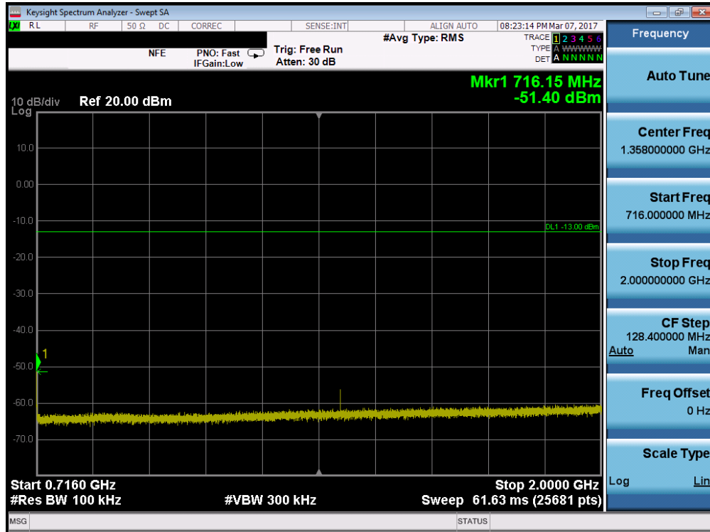
Plot 7-44. Conducted Spurious Plot (Band 17 – 10.0MHz QPSK – RB Size 1, RB Offset 0 – Mid Channel)
