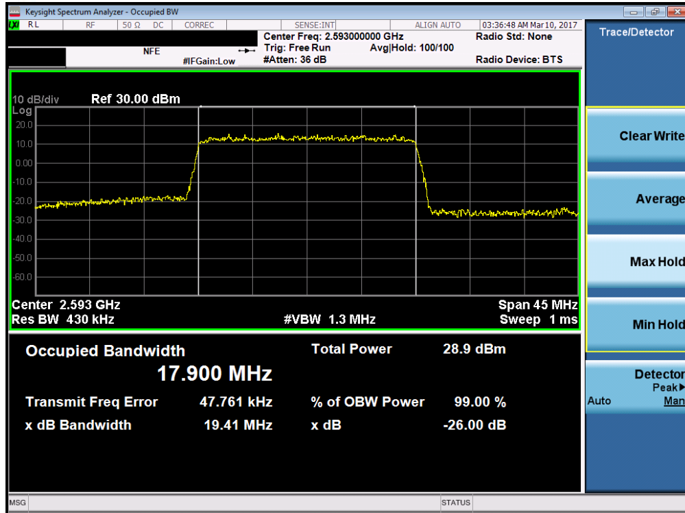
Plot 7-39. Occupied Bandwidth Plot (Band 41 – 20.0MHz 64-QAM – RB Size 100)
