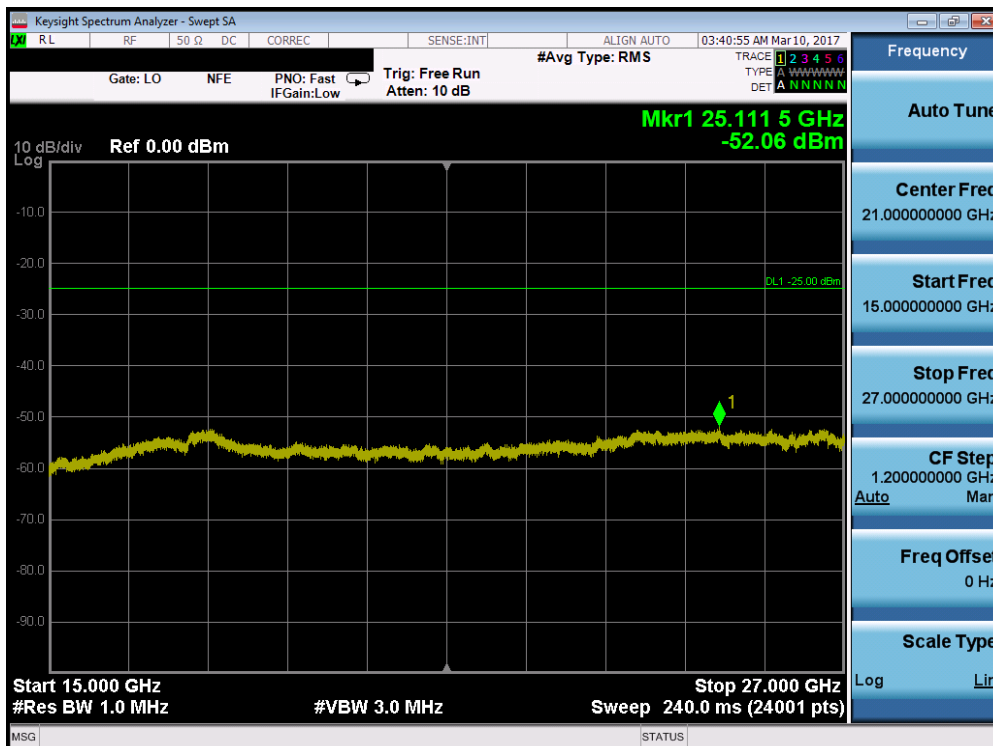
Plot 7-69. Conducted Spurious Plot (Band 41 – 20.0MHz QPSK – RB Size 1, RB Offset 0 – High Channel)
