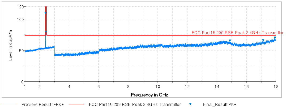
Plot 7-43. Radiated Spurious Plot above 1GHz (BT – Ch. 0, Ant. Pol. V)
