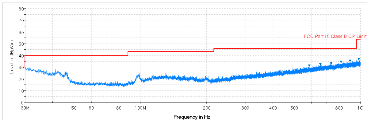
Plot 7-55. Radiated Spurious Plot below 1GHz (Pol. V)
