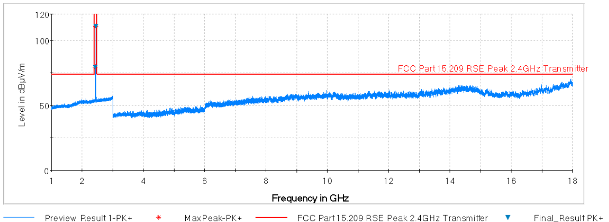
Plot 7-44. Radiated Spurious Plot above 1GHz (BT – Ch. 39, Ant. Pol. H)
