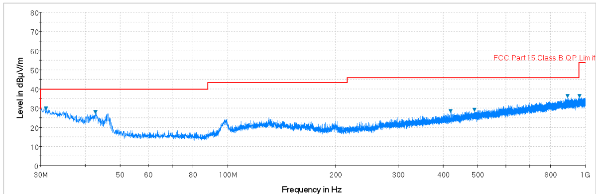
Plot 7-54. Radiated Spurious Plot below 1GHz (Pol. H)
