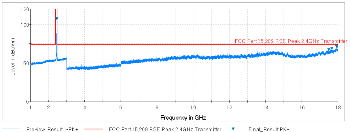
Plot 7-65. Radiated Spurious Plot above 1GHz (802.11b – Ch. 11, Ant. Pol. H)
