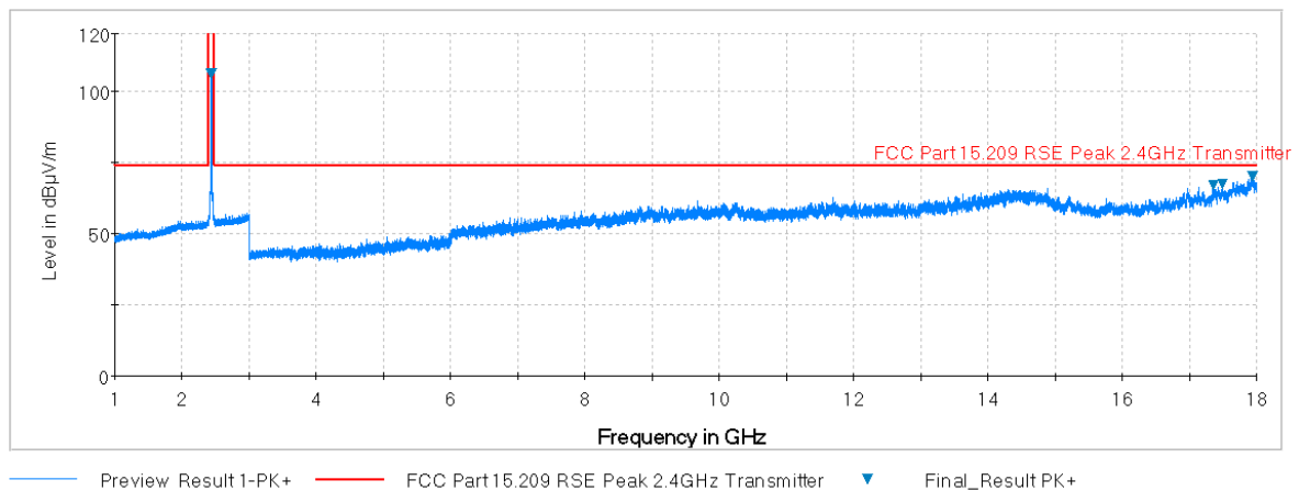
Plot 7-63. Radiated Spurious Plot above 1GHz (802.11b – Ch. 6, Ant. Pol. H)
