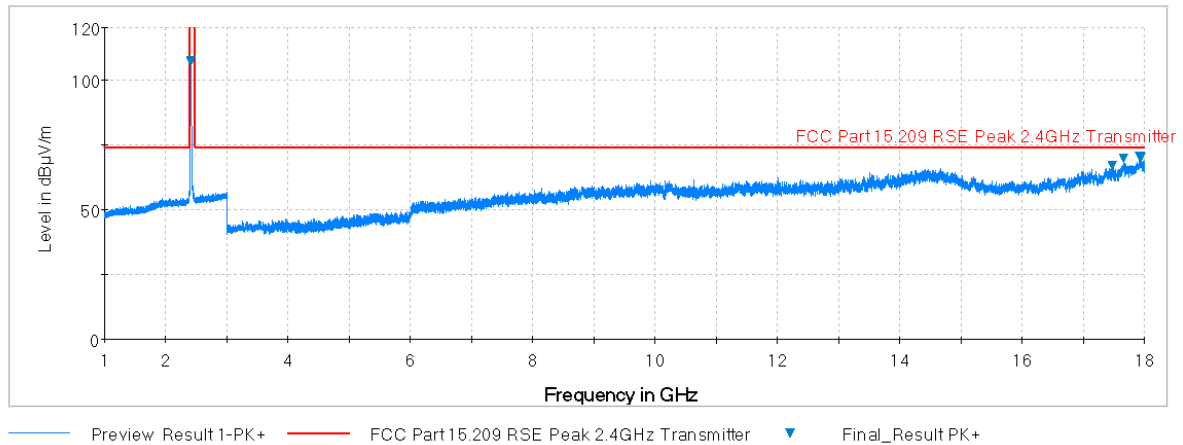
Plot 7-62. Radiated Spurious Plot above 1GHz (802.11b – Ch. 1, Ant. Pol. V)
