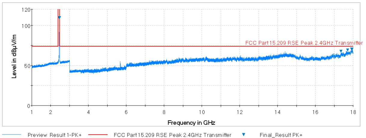
Plot 7-74. Radiated Spurious Plot above 1GHz (802.11b – Ch. 11, Ant. Pol. V)
