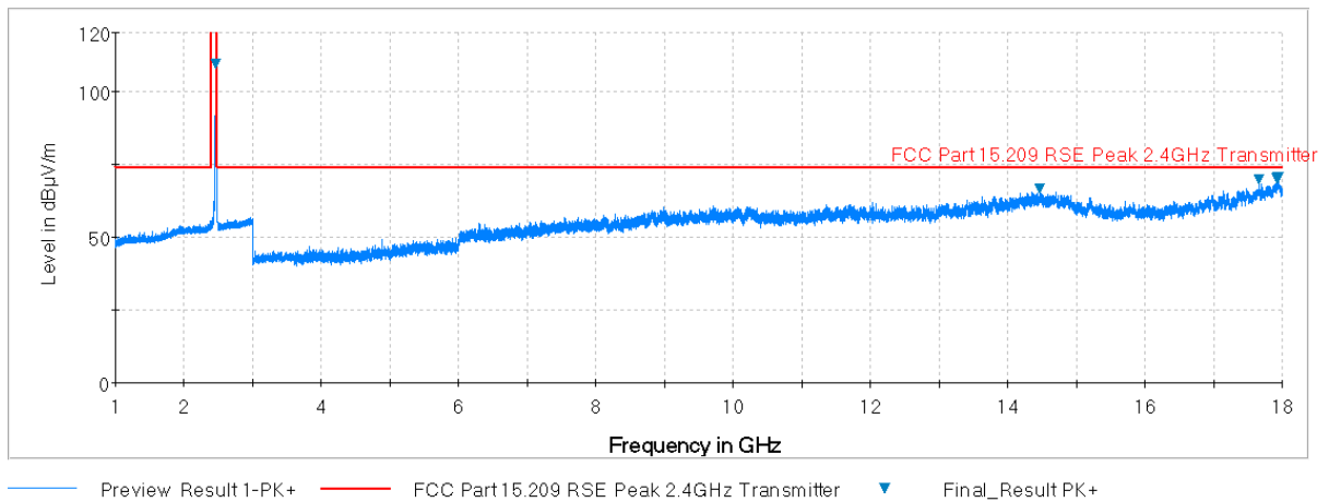
Plot 7-73. Radiated Spurious Plot above 1GHz (802.11b – Ch. 11, Ant. Pol. H)
