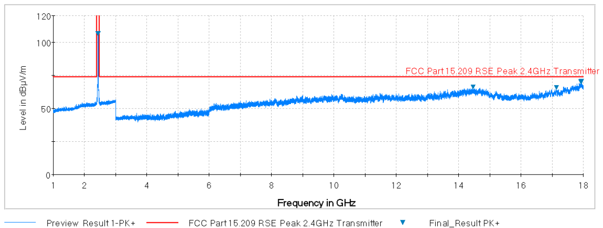
Plot 7-71. Radiated Spurious Plot above 1GHz (802.11b – Ch. 6, Ant. Pol. H)
