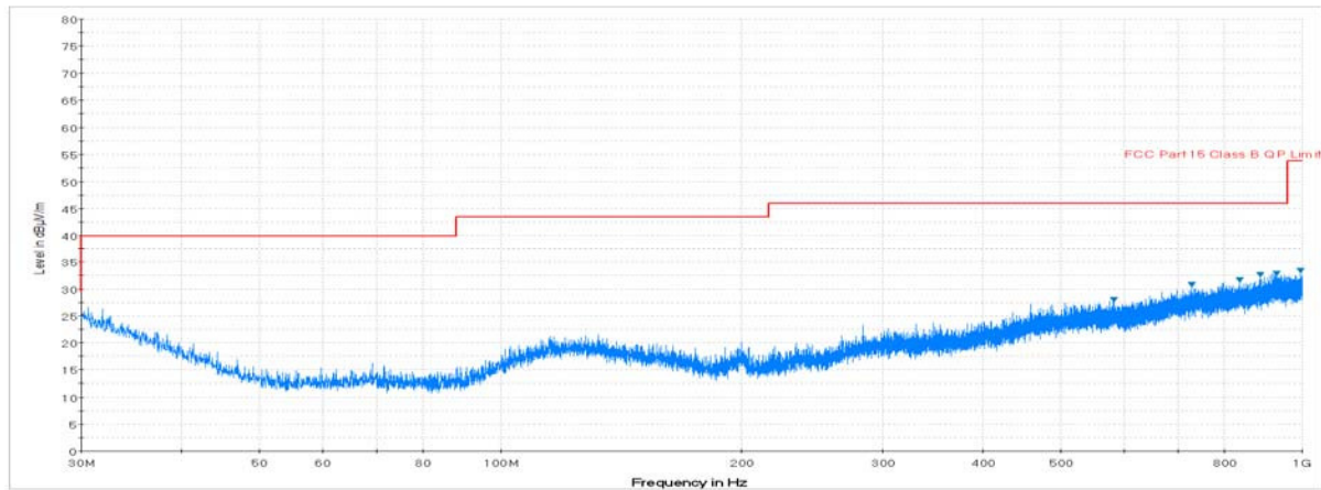
Plot 7-55. Radiated Spurious Plot below 1GHz (Pol. V)
