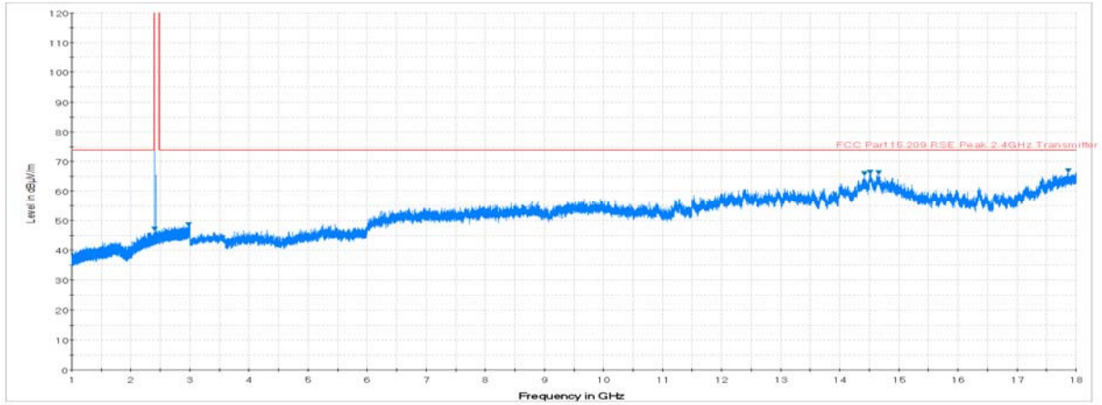
Plot 7-42. Radiated Spurious Plot above 1GHz (BT – Ch. 0, Ant. Pol. H)
