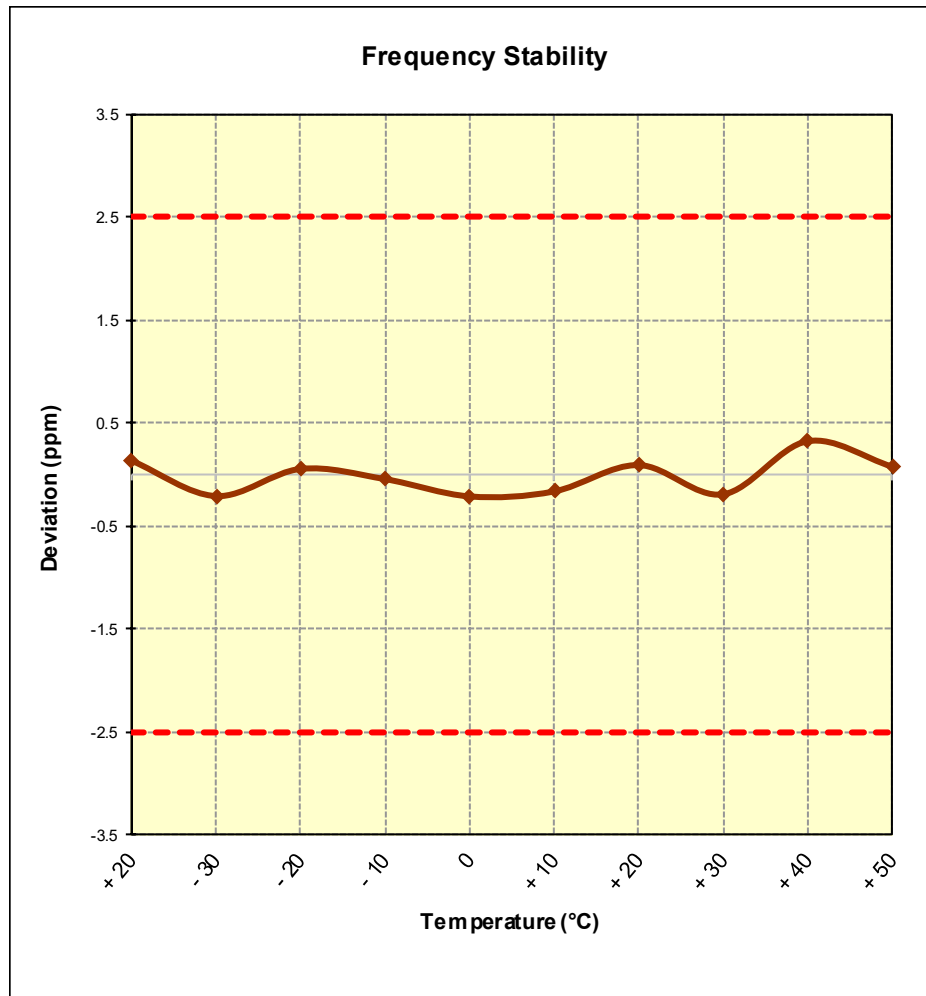
Figure 7-11. Frequency Stability Graph (Band 5/26)
