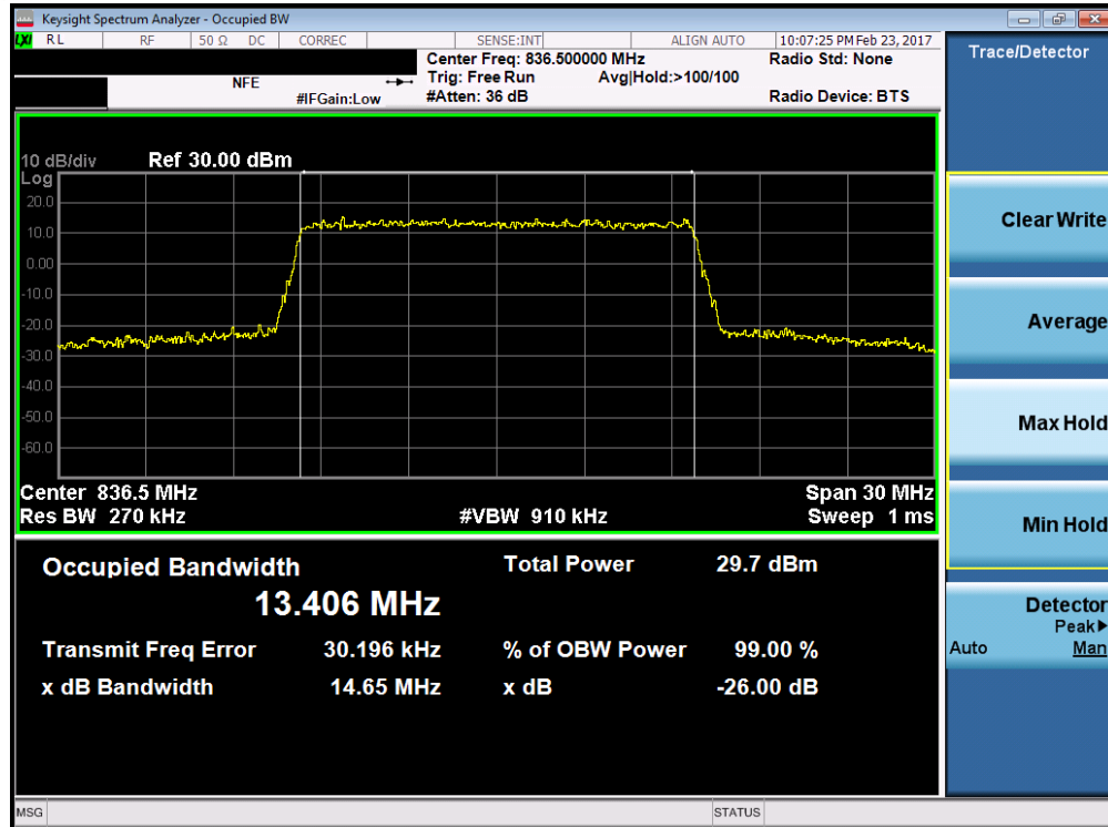
Plot 7-27. Occupied Bandwidth Plot (Band 5/26 – 15.0MHz 64-QAM – RB Size 75)
