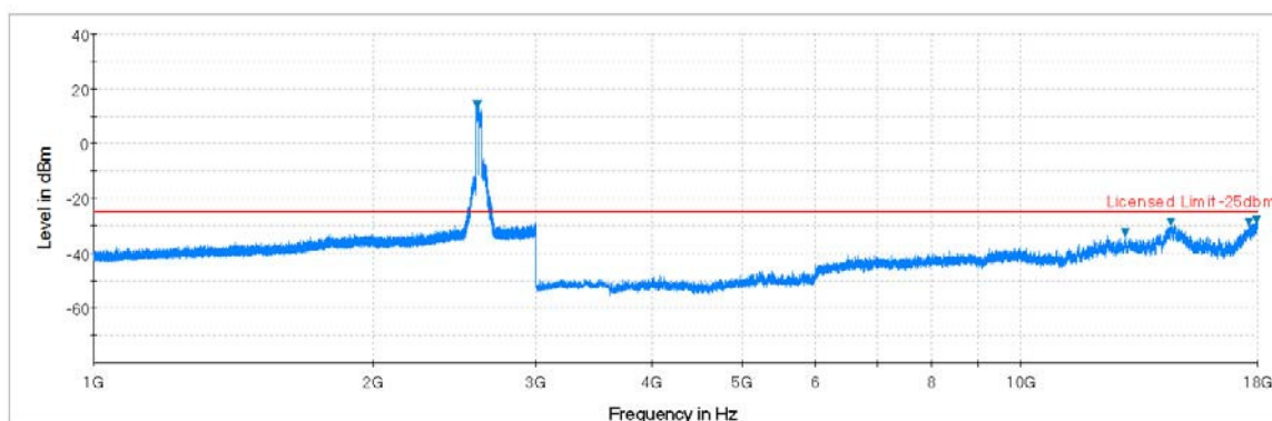
Plot 7-110. Radiated Spurious Plot (ULCA B41 PCC: RB 100 Offset 0, SCC: RB 100 Offset 0, Ant. Pol. H)
