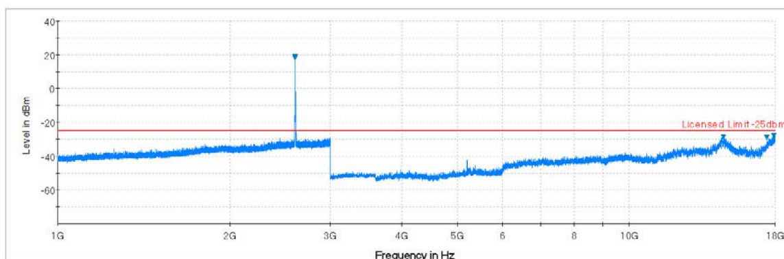
Plot 7-109. Radiated Spurious Plot (ULCA B41 PCC: RB 1 Offset 99, SCC: RB 1 Offset 0, Ant. Pol. V)
