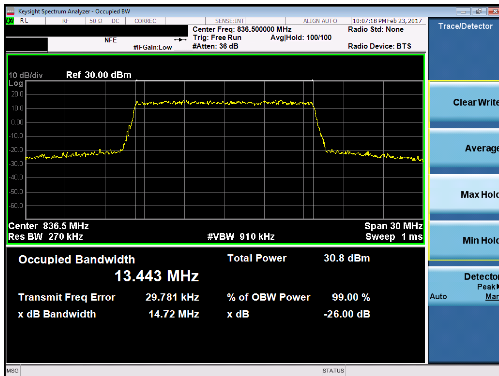
Plot 7-26. Occupied Bandwidth Plot (Band 5/26 – 15.0MHz 16-QAM – RB Size 75)
