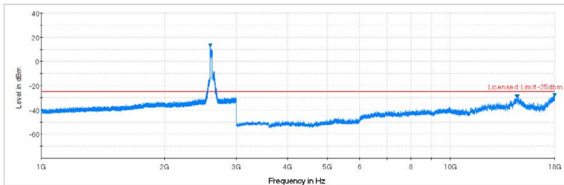
Plot 7-111. Radiated Spurious Plot (ULCA B41 PCC: RB 100 Offset 0, SCC: RB 100 Offset 0, Ant. Pol. V)
