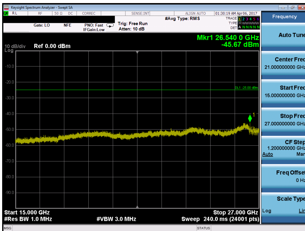
Plot 7-63. Conducted Spurious Plot (Band 41 – 10.0MHz QPSK – RB Size 1, RB Offset 0 – Low Channel)
