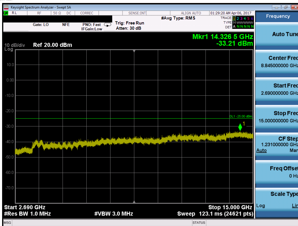
Plot 7-62. Conducted Spurious Plot (Band 41 – 10.0MHz QPSK – RB Size 1, RB Offset 0 – Low Channel)
