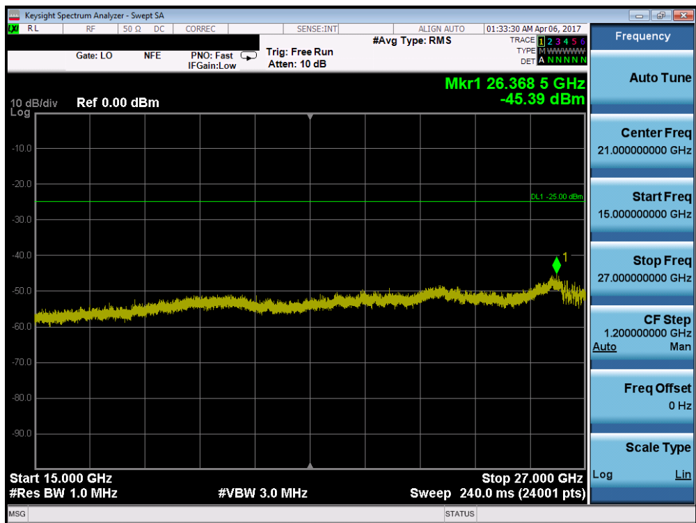
Plot 7-69. Conducted Spurious Plot (Band 41 – 10.0MHz QPSK – RB Size 1, RB Offset 0 – High Channel)
