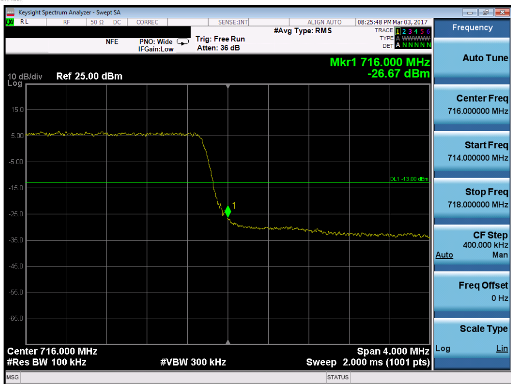
Plot 7-71. Upper Band Edge Plot (Band 17 – 5.0MHz QPSK – RB Size 25)
