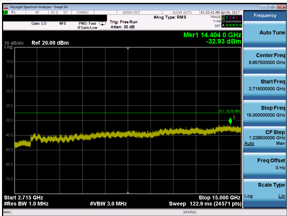
Plot 7-68. Conducted Spurious Plot (Band 41 – 10.0MHz QPSK – RB Size 1, RB Offset 0 – High Channel)
