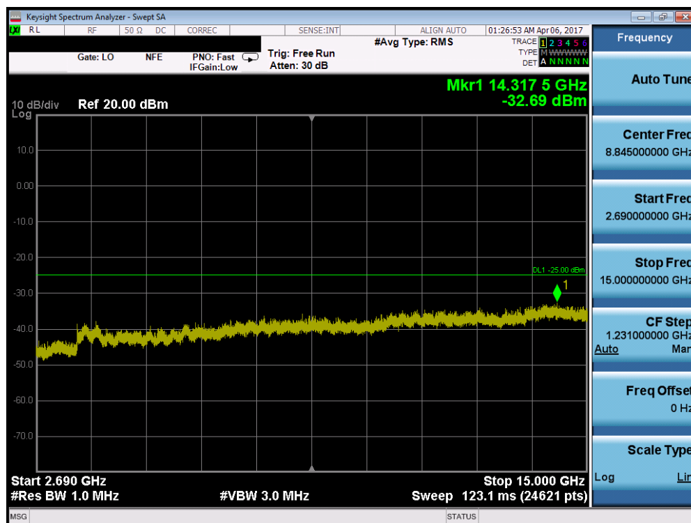
Plot 7-65. Conducted Spurious Plot (Band 41 – 10.0MHz QPSK – RB Size 1, RB Offset 0 – Mid Channel)
