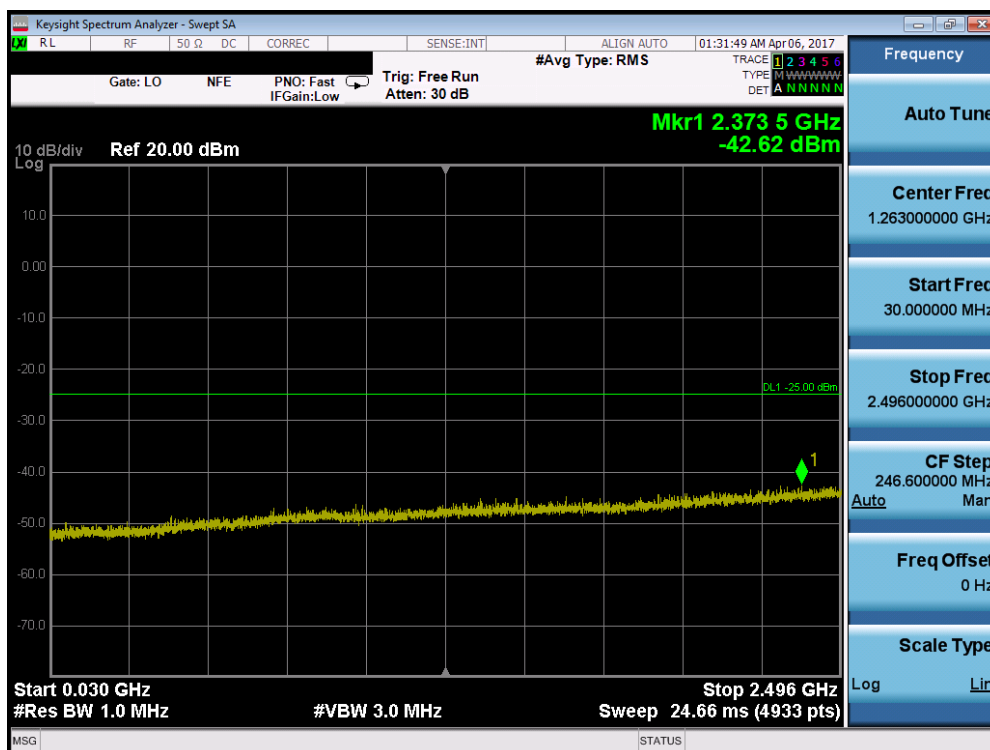
Plot 7-67. Conducted Spurious Plot (Band 41 – 10.0MHz QPSK – RB Size 1, RB Offset 0 – High Channel)
