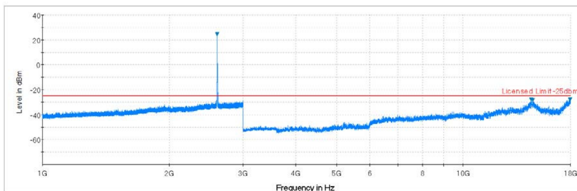
Plot 7-108. Radiated Spurious Plot (ULCA B41 PCC: RB 1 Offset 99, SCC: RB 1 Offset 0, Ant. Pol. H)
