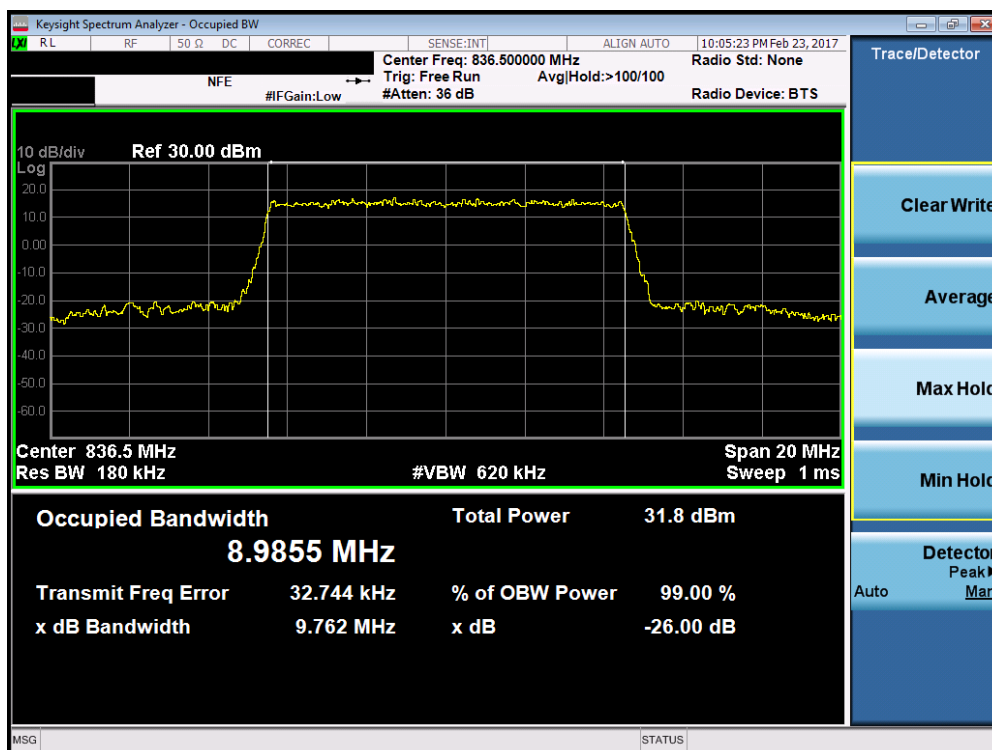
Plot 7-22. Occupied Bandwidth Plot (Band 5/26 – 10.0MHz QPSK – RB Size 50)
