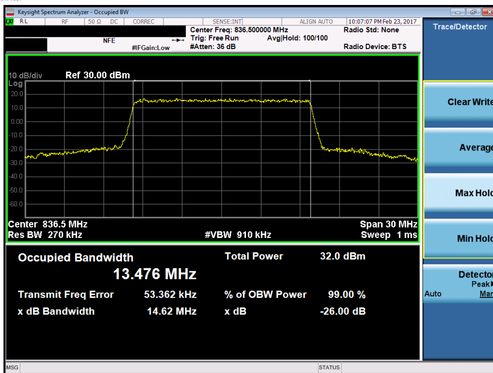
Plot 7-25. Occupied Bandwidth Plot (Band 5/26 – 15.0MHz QPSK – RB Size 75)
