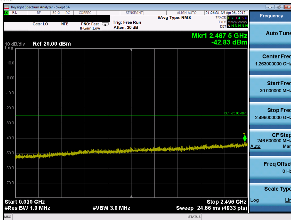
Plot 7-64. Conducted Spurious Plot (Band 41 – 10.0MHz QPSK – RB Size 1, RB Offset 0 – Mid Channel)
