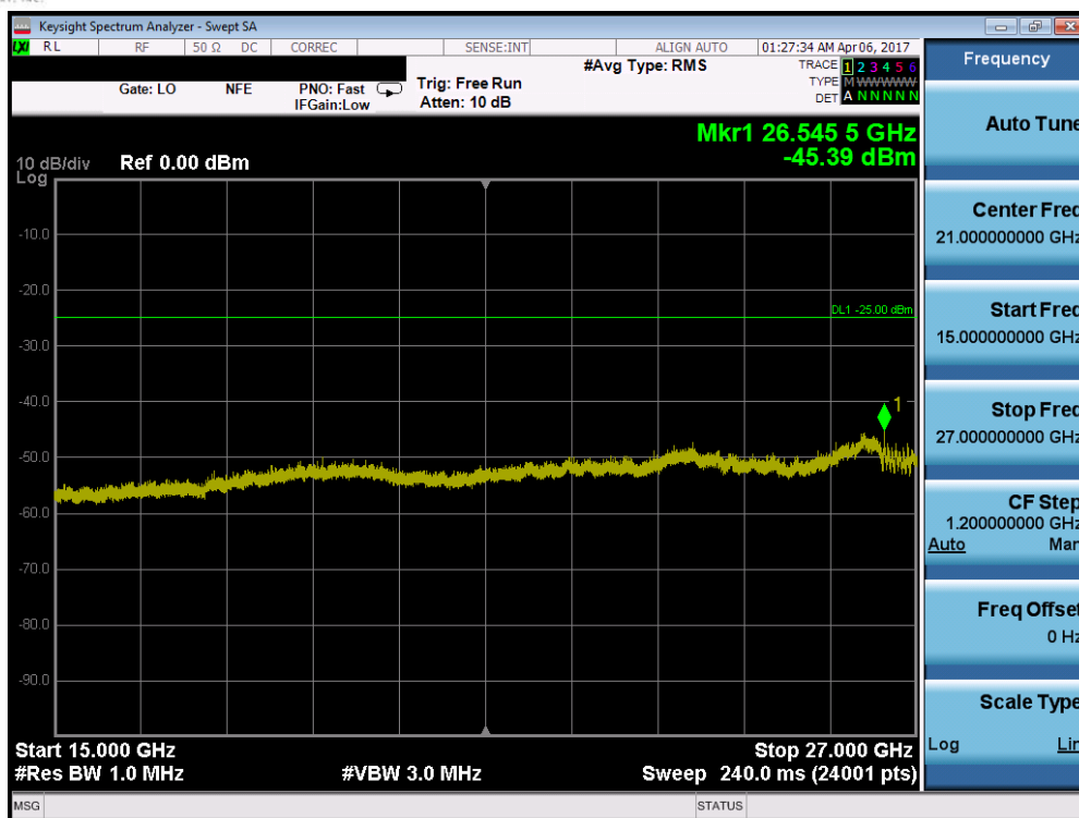
Plot 7-66. Conducted Spurious Plot (Band 41 – 10.0MHz QPSK – RB Size 1, RB Offset 0 – Mid Channel)
