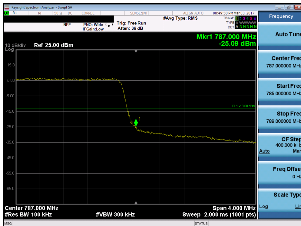
Plot 7-76. Upper Band Edge Plot (Band 13 – 5.0MHz QPSK – RB Size 25)
