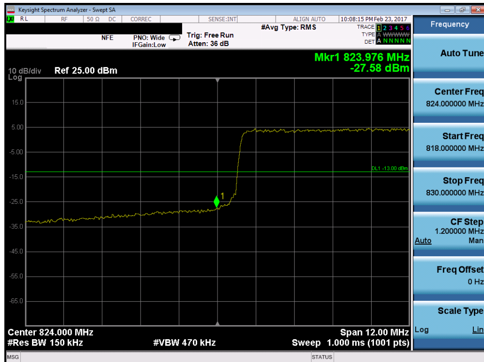
Plot 7-90. Lower Band Edge Plot (Band 5/26 – 15.0MHz QPSK – RB Size 75)
