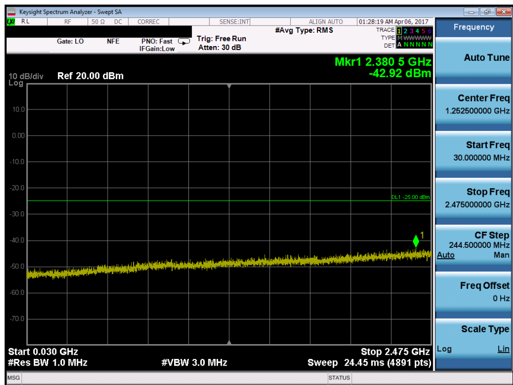
Plot 7-61. Conducted Spurious Plot (Band 41 – 10.0MHz QPSK – RB Size 1, RB Offset 0– Low Channel)
