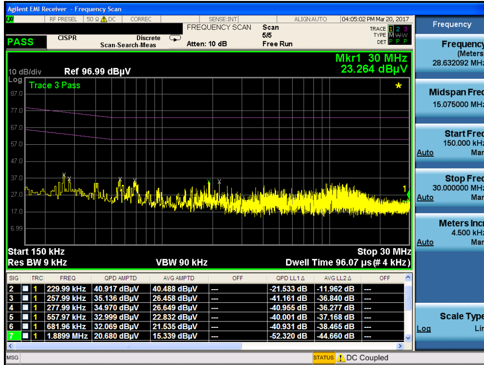
Plot 8-3. Line-Conducted Test Plot (L1) – Terminated in 50 Ω
