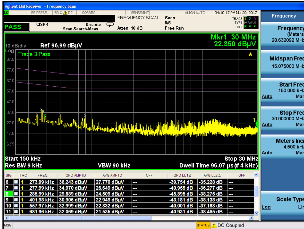
Plot 8-4. Line-Conducted Test Plot (N) – Terminated in 50 Ω
