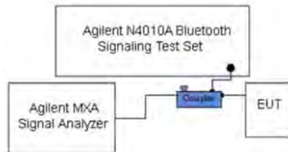
Figure 9-7 Power Measurement Setup
