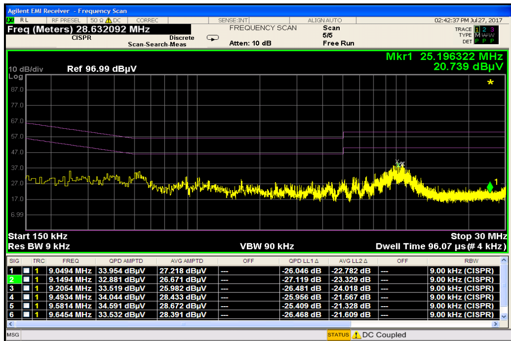
Plot 7-9. Line-Conducted Test Plot (N)
