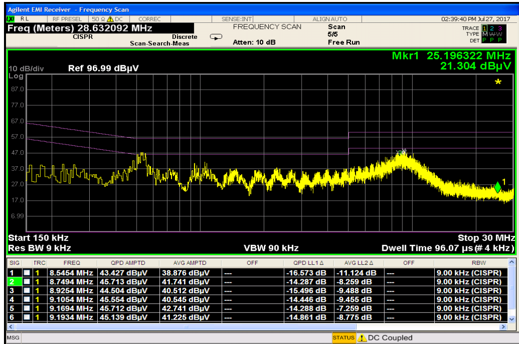
Plot 7-8. Line-Conducted Test Plot (L1)
