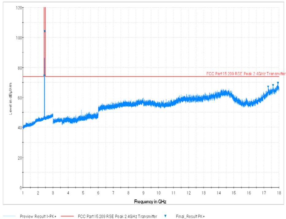
Plot 7-44. Radiated Spurious Plot above 1GHz (BT – Ch. 39, Ant. Pol. H)
