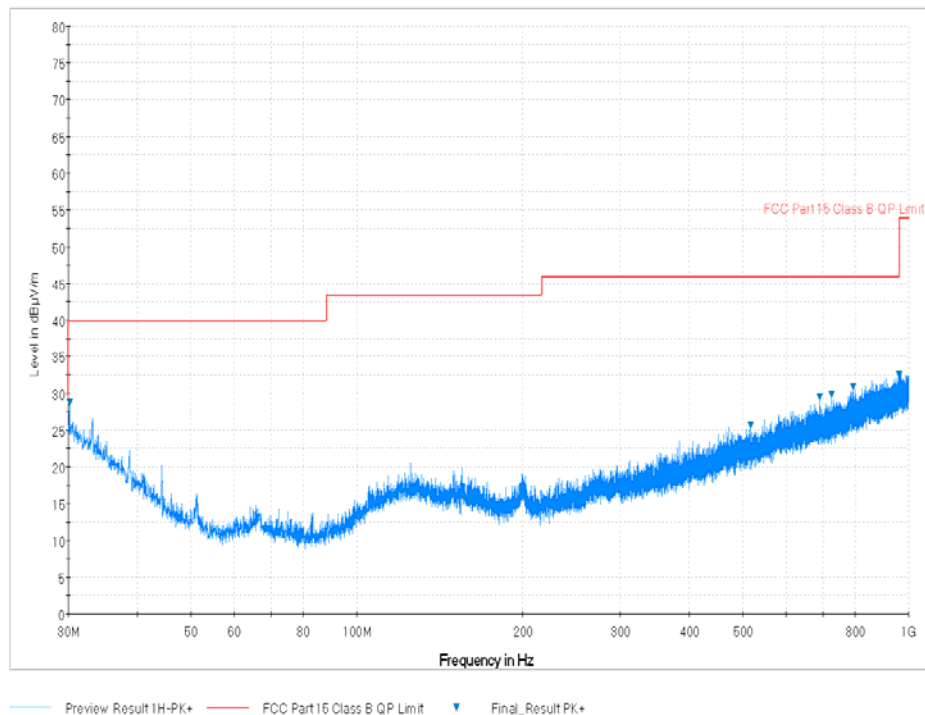
Plot 7-55. Radiated Spurious Plot below 1GHz (Pol. V)
