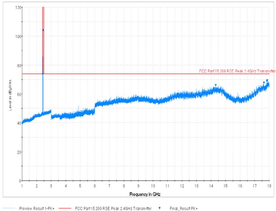
Plot 7-45. Radiated Spurious Plot above 1GHz (BT – Ch. 39, Ant. Pol. V)
