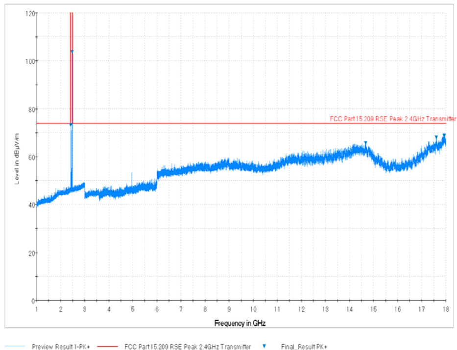
Plot 7-47. Radiated Spurious Plot above 1GHz (BT – Ch. 78, Ant. Pol. V)
