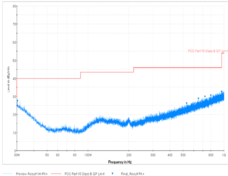
Plot 7-54. Radiated Spurious Plot below 1GHz (Pol. H)
