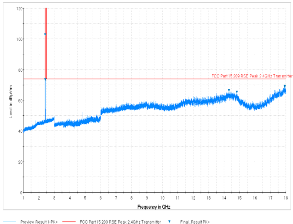
Plot 7-43. Radiated Spurious Plot above 1GHz (BT – Ch. 0, Ant. Pol. V)
