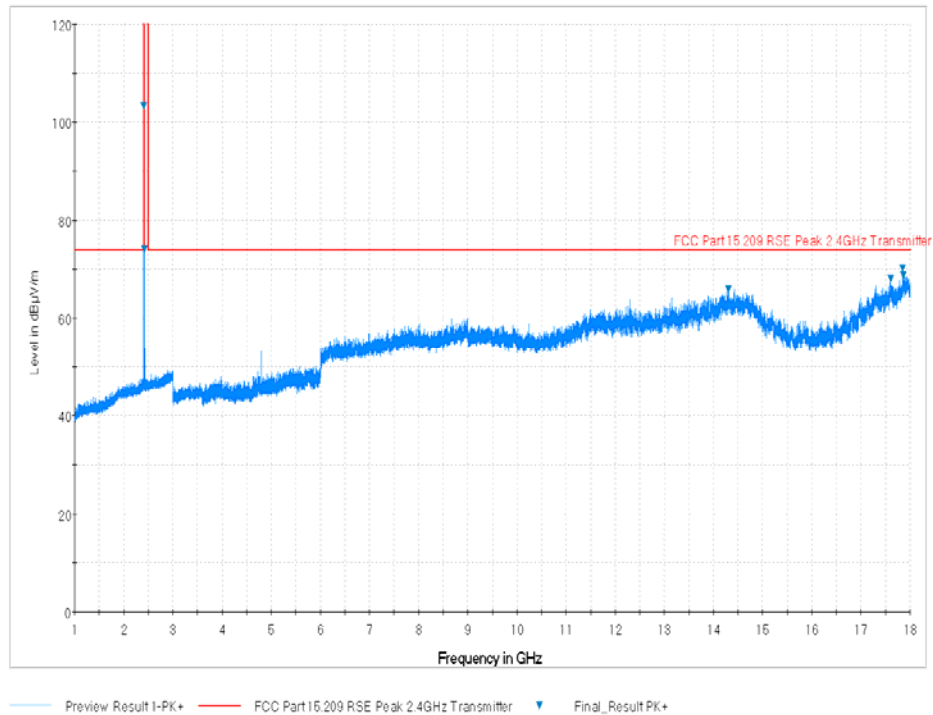
Plot 7-42. Radiated Spurious Plot above 1GHz (BT – Ch. 0, Ant. Pol. H)
