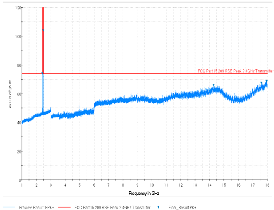
Plot 7-46. Radiated Spurious Plot above 1GHz (BT – Ch. 78, Ant. Pol. H)
