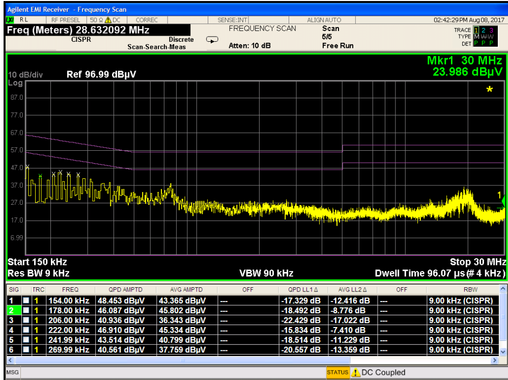
Plot 7-3. Line-Conducted Test Plot (L1) – Terminated in 50Ω
