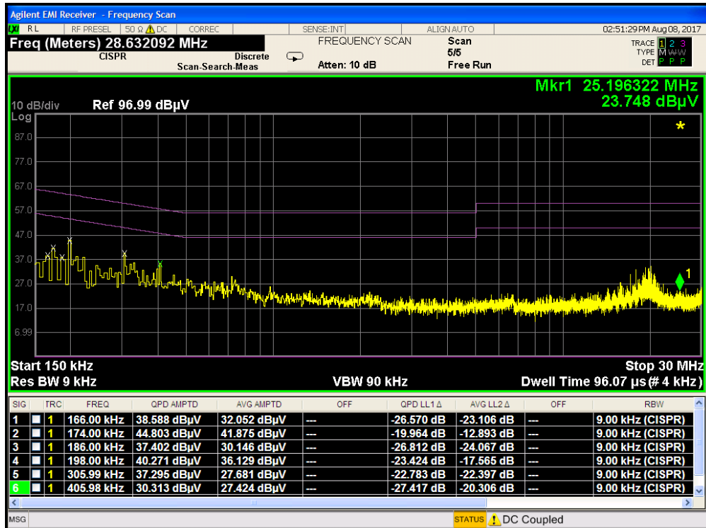
Plot 7-4. Line-Conducted Test Plot (N) – Terminated in 50Ω
