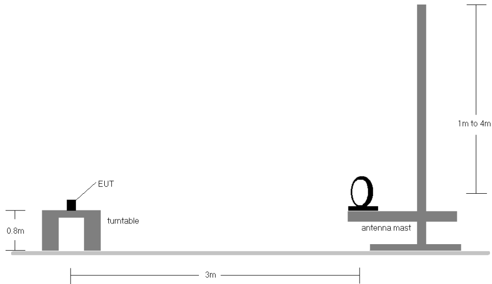
Figure 7-5. Radiated Test Setup < 30MHz
