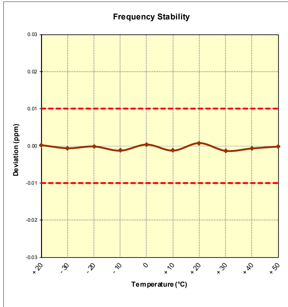
Figure 7-3. Frequency Stability Plot
