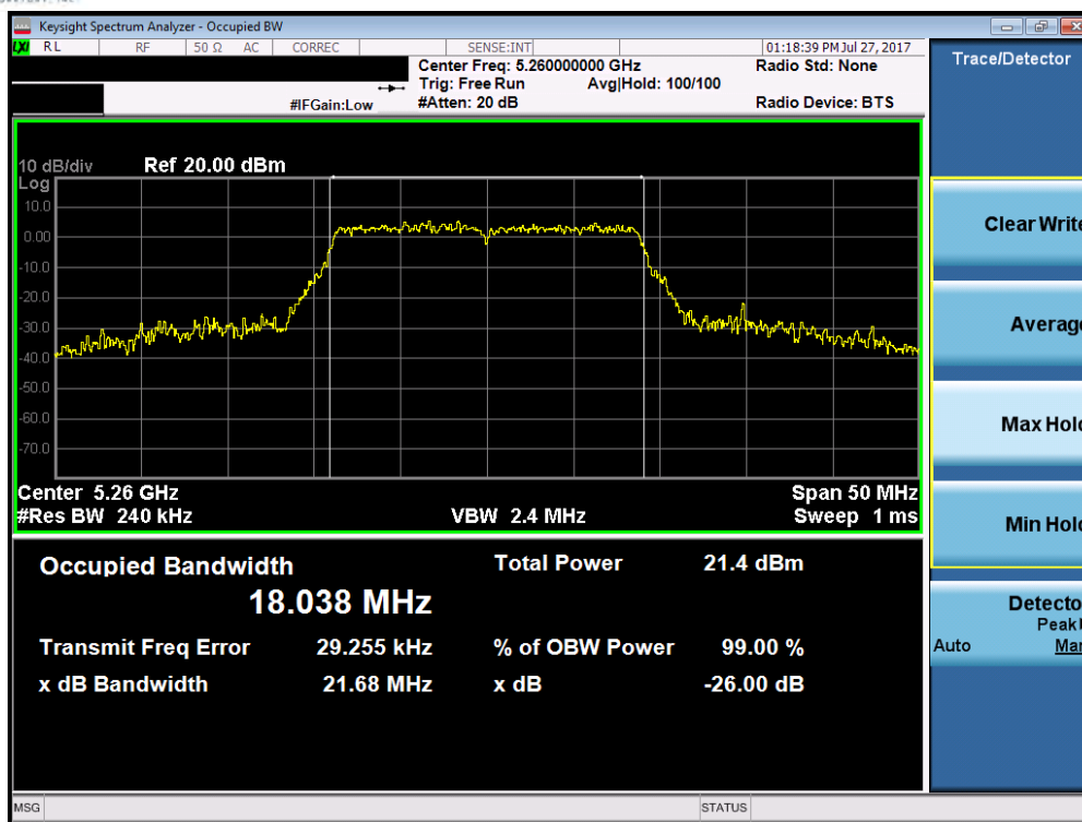
Plot 7-43. 26dB Bandwidth Plot (20MHz BW 802.11n (UNII Band 2A) – Ch. 52)
