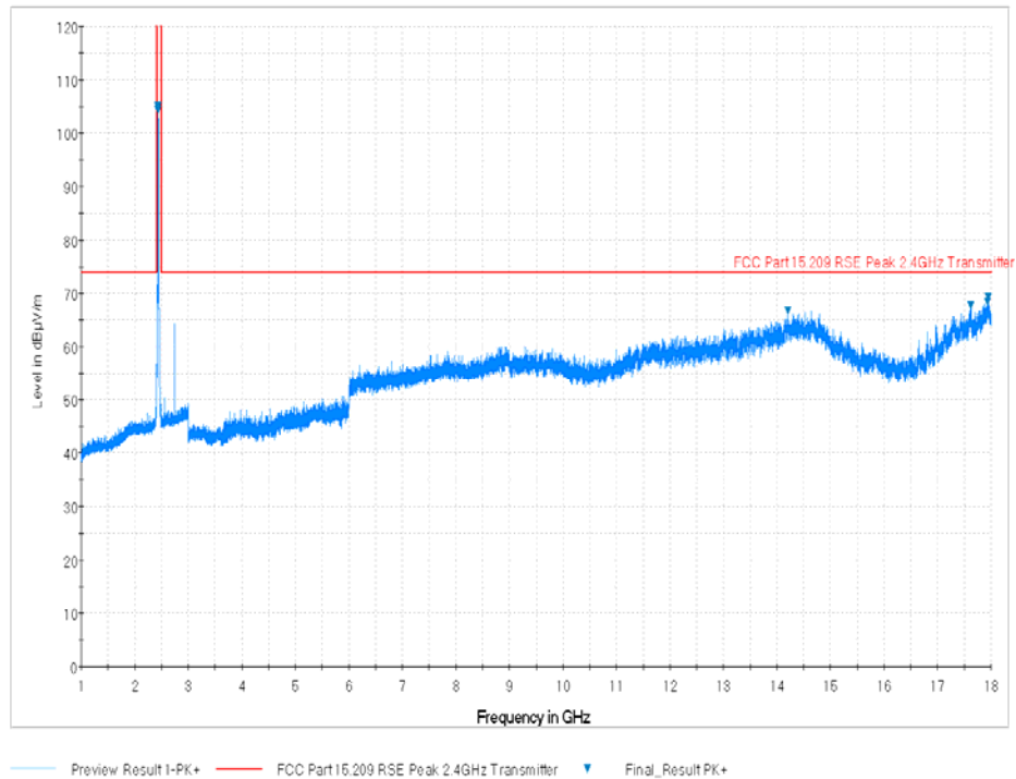
Plot 7-75. Radiated Spurious Plot above 1GHz (802.11b – Ch. 6, Ant. Pol. H)
