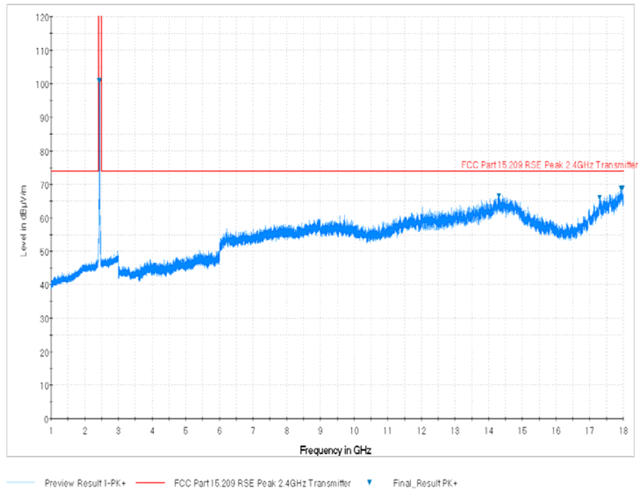
Plot 7-76. Radiated Spurious Plot above 1GHz (802.11b – Ch. 6, Ant. Pol. V)
