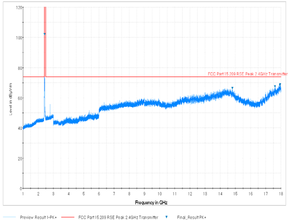
Plot 7-74. Radiated Spurious Plot above 1GHz (802.11b – Ch. 1, Ant. Pol. V)
