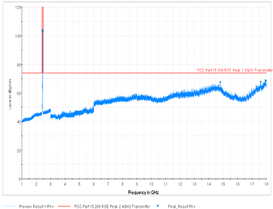
Plot 7-83. Radiated Spurious Plot above 1GHz (802.11b – Ch. 6, Ant. Pol. H)
