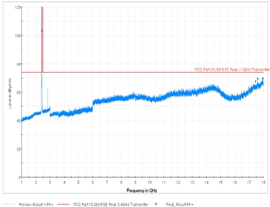
Plot 7-81. Radiated Spurious Plot above 1GHz (802.11b – Ch. 1, Ant. Pol. H)
