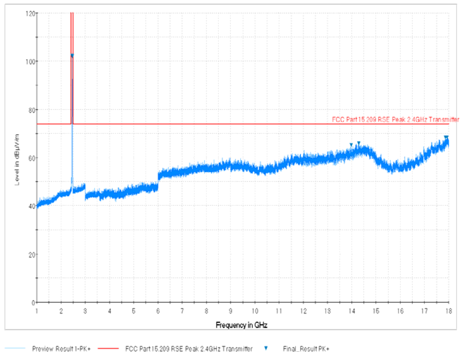
Plot 7-86. Radiated Spurious Plot above 1GHz (802.11b – Ch. 11, Ant. Pol. V)
