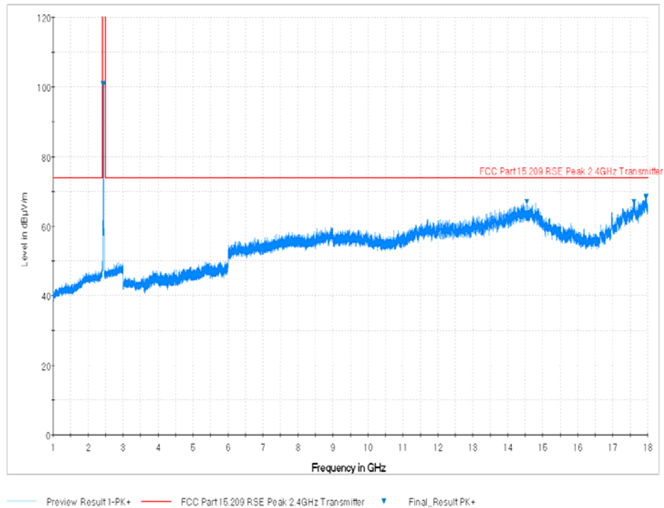
Plot 7-84. Radiated Spurious Plot above 1GHz (802.11b – Ch. 6, Ant. Pol. V)
