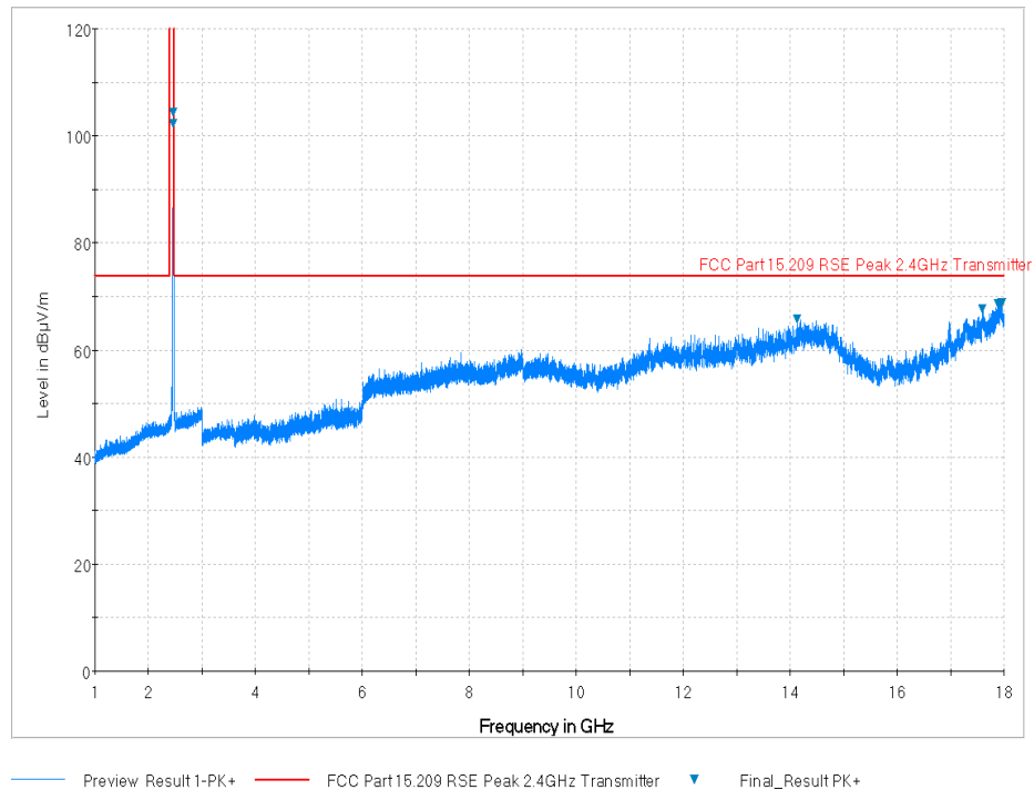
Plot 7-85. Radiated Spurious Plot above 1GHz (802.11b – Ch. 11, Ant. Pol. H)
