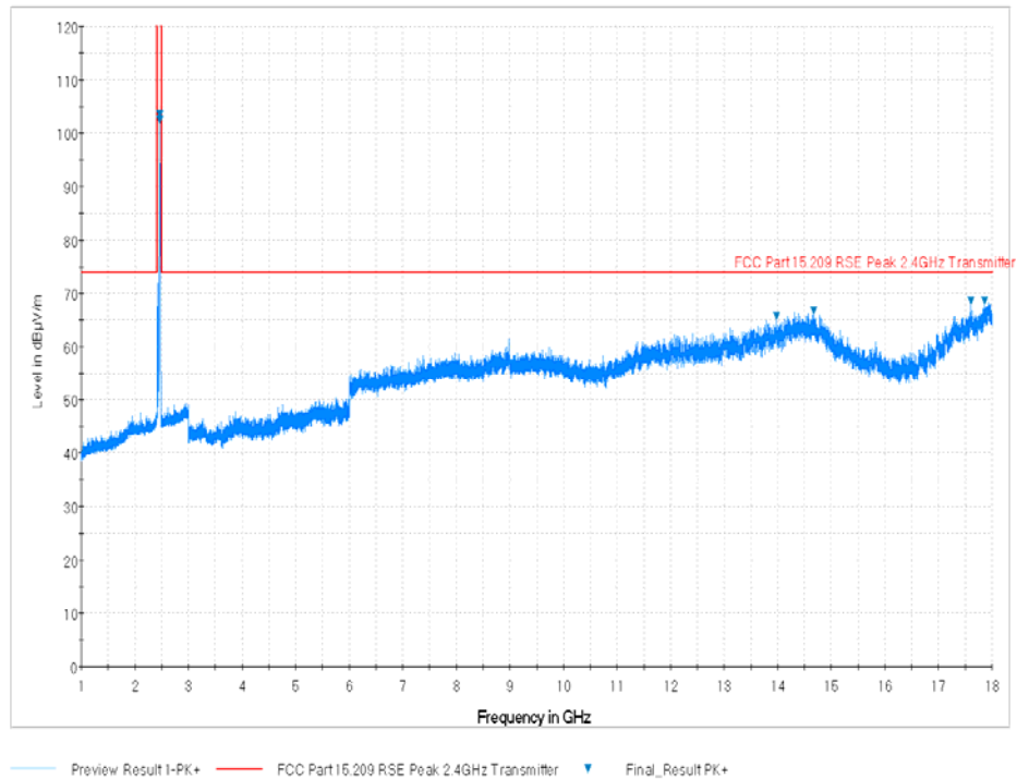
Plot 7-78. Radiated Spurious Plot above 1GHz (802.11b – Ch. 11, Ant. Pol. V)
