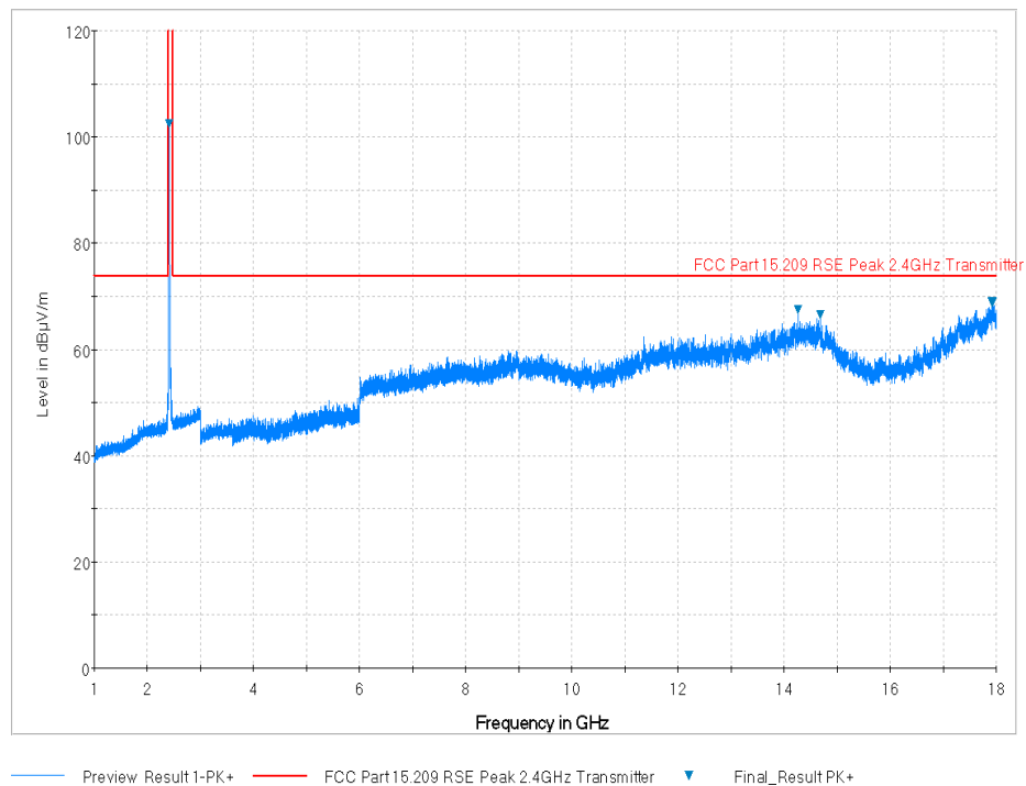
Plot 7-82. Radiated Spurious Plot above 1GHz (802.11b – Ch. 1, Ant. Pol. V)
