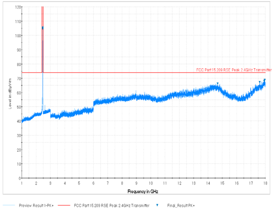
Plot 7-77. Radiated Spurious Plot above 1GHz (802.11b – Ch. 11, Ant. Pol. H)
