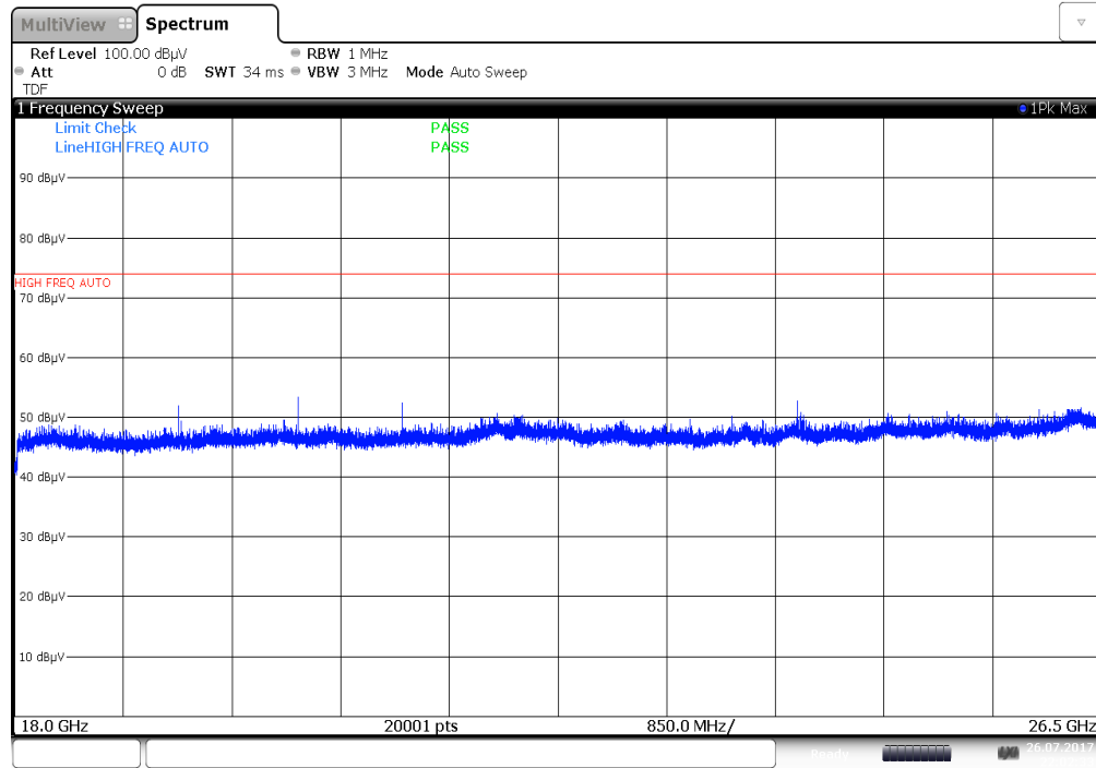
Plot 7-87. Radiated Spurious Plot above 18GHz (Pol. H)
