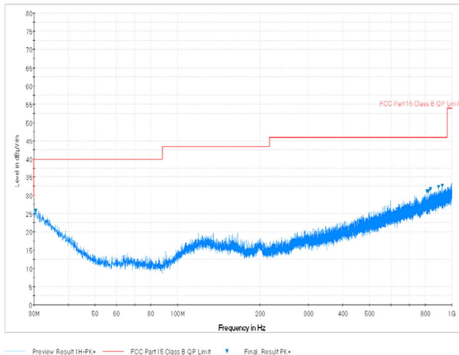
Plot 7-120. Radiated Spurious Plot below 1GHz (Pol. V)
