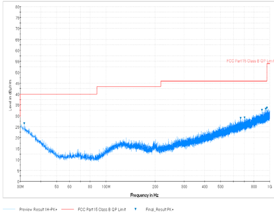
Plot 7-121. Radiated Spurious Plot below 1GHz (Pol. H)
