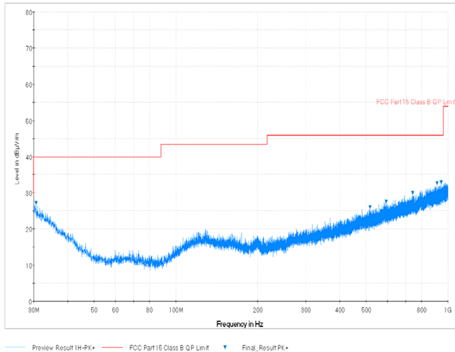
Plot 7-119. Radiated Spurious Plot below 1GHz (Pol. H)
