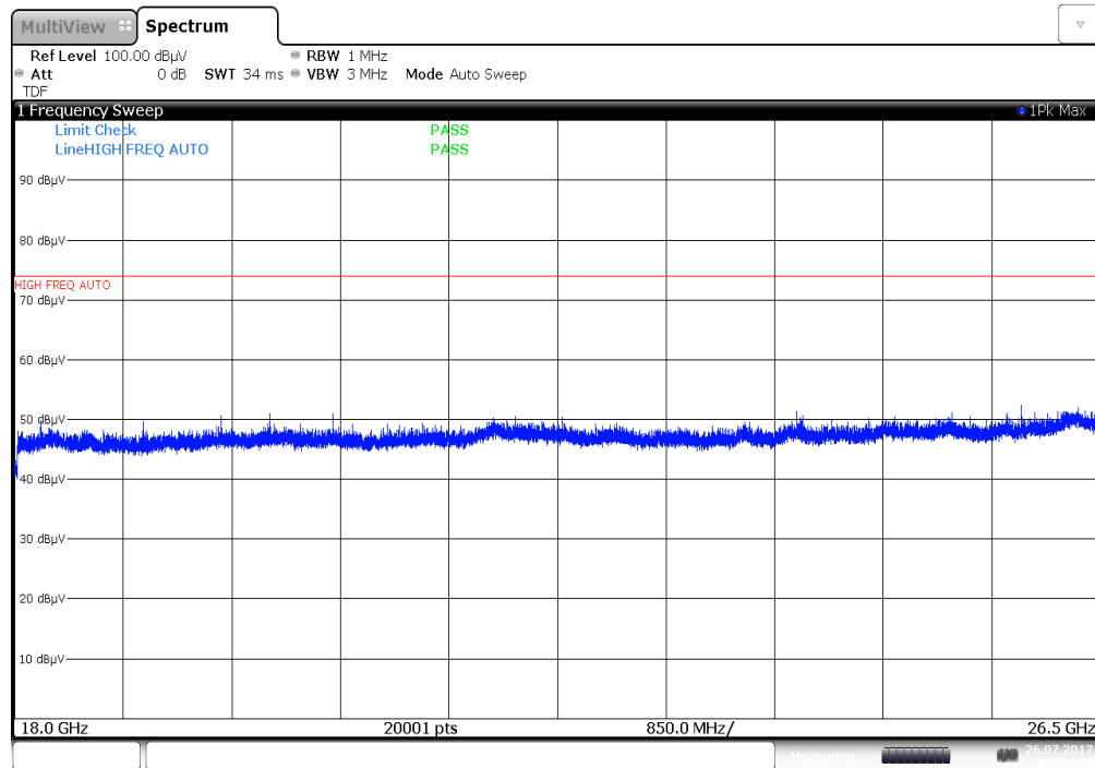
Plot 7-88. Radiated Spurious Plot above 18GHz (Pol. V)
