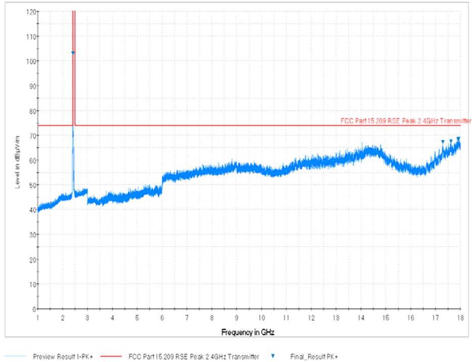
Plot 7-73. Radiated Spurious Plot above 1GHz (802.11b – Ch. 1, Ant. Pol. H)
