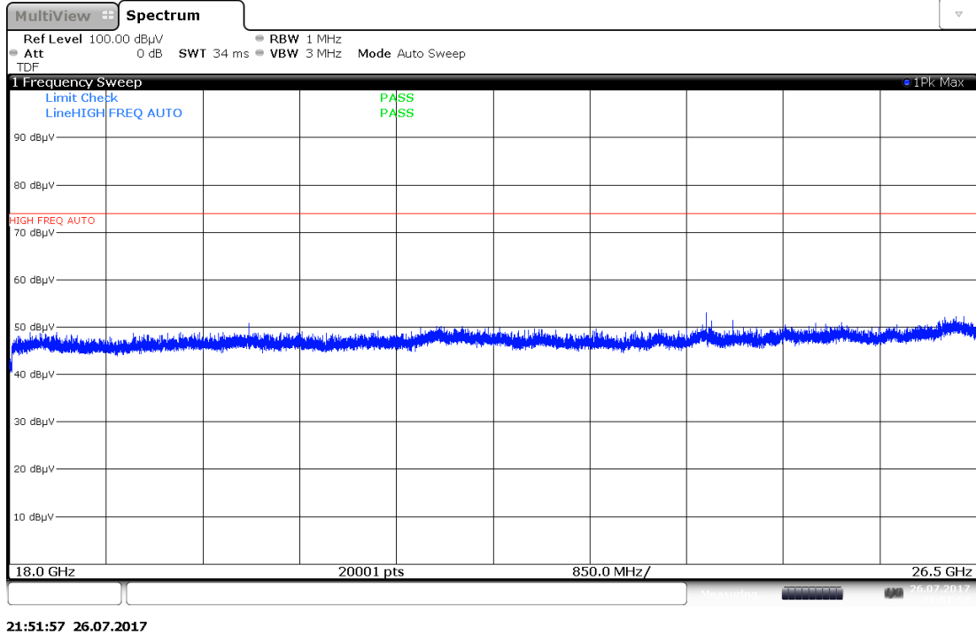
Plot 7-79. Radiated Spurious Plot above 18GHz (Pol. H)
