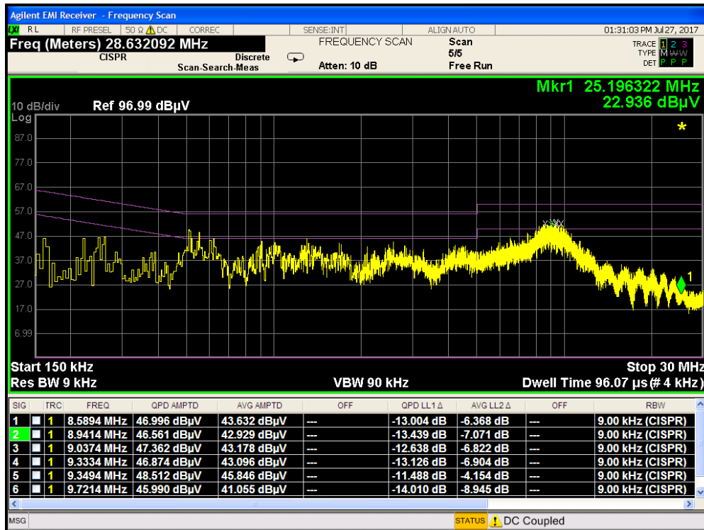
Plot 7-123. Line Conducted Plot with 802.11b (L1)
