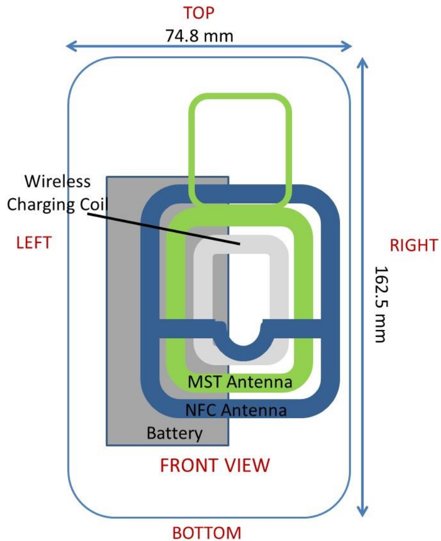
Figure F-2 NFC Antenna Locations
