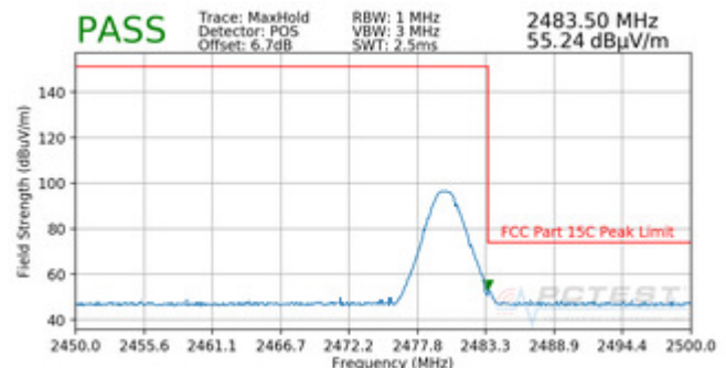
Plot 7-5. Radiated Restricted Upper Band Edge Measurement (Peak)
