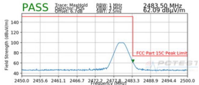
Plot 7-30. Radiated Restricted Upper Band Edge Measurement with WCP (Peak)
