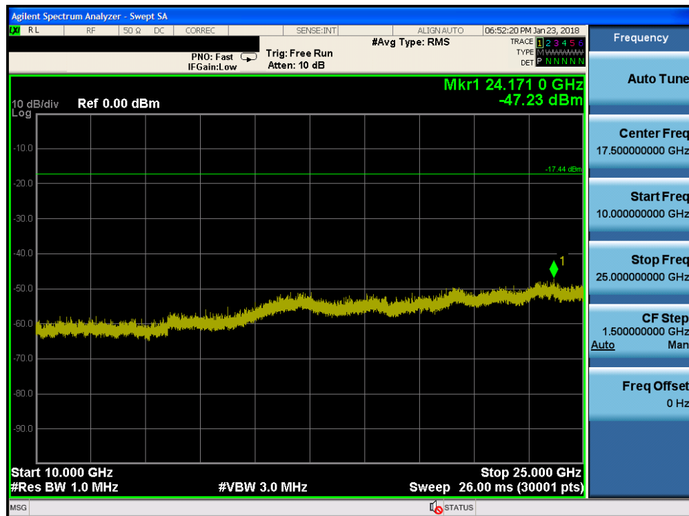
Plot 7-22. Conducted Spurious Plot (Bluetooth (LE), 1Mbps - Ch. 0)
