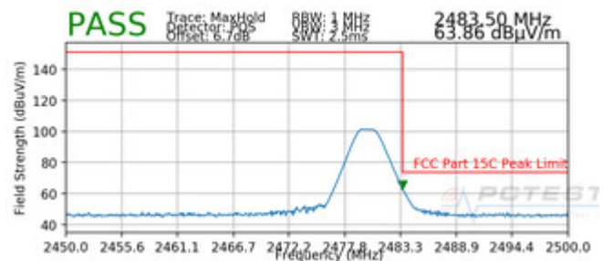
Plot 7-28. Radiated Restricted Upper Band Edge Measurement (Peak)
