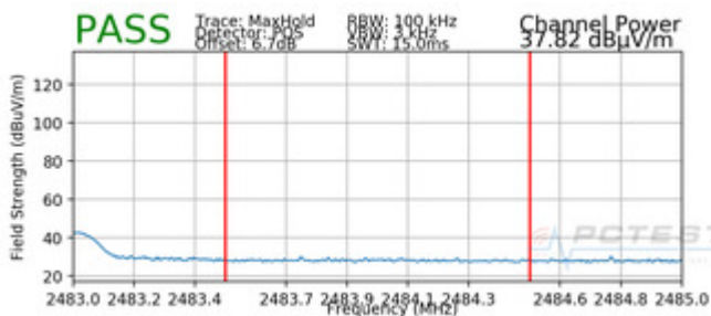
Plot 7-27. Radiated Restricted Upper Band Edge Measurement (Average)
