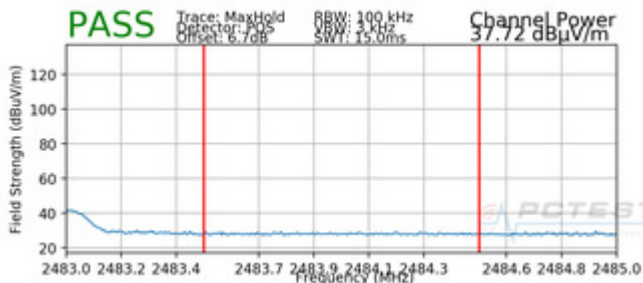
Plot 7-29. Radiated Restricted Upper Band Edge Measurement with WCP (Average)
