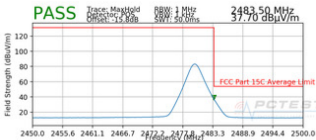
Plot 7-48. Radiated Restricted Upper Band Edge Measurement with WCP (Average)
