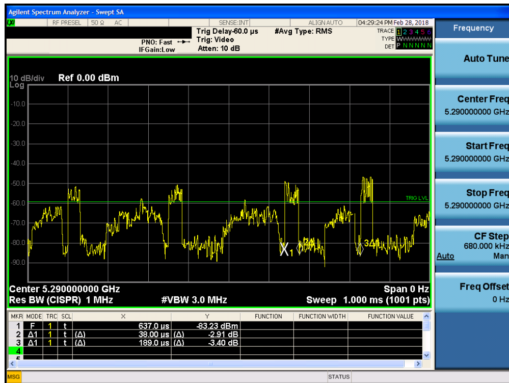
Figure 5-1. Band 2A Duty Cycle
