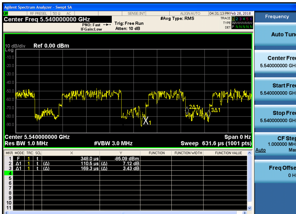
Figure 5-2. Band 2C Duty Cycle
