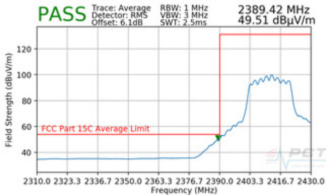
Plot 7-101. Radiated Restricted Lower Band Edge Measurement (Average)
