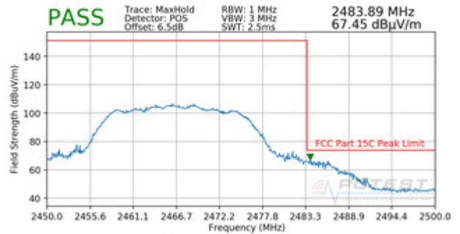
Plot 7-106. Radiated Restricted Upper Band Edge Measurement (Peak)
