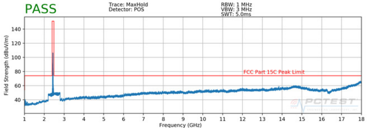
Plot 7-78. Radiated Spurious Plot above 1GHz (802.11b – Ch. 6)
