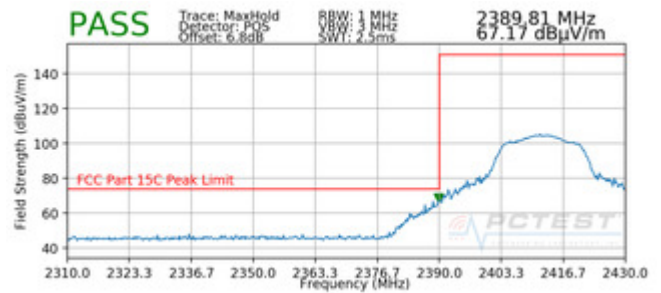
Plot 7-90. Radiated Restricted Band Edge Measurement with WCP (Peak)
