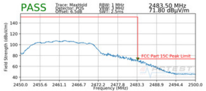
Plot 7-110. Radiated Restricted Band Edge Measurement with WCP (Peak)
