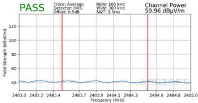
Plot 7-95. Radiated Restricted Upper Band Edge Measurement (Average)
