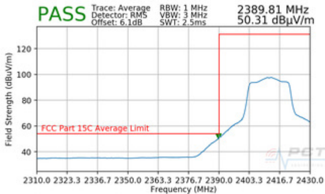
Plot 7-91. Radiated Restricted Lower Band Edge Measurement (Average)
