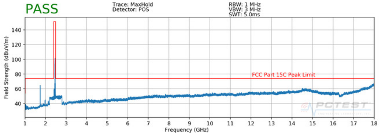
Plot 7-75. Radiated Spurious Plot above 1GHz (802.11b – Ch. 11)
