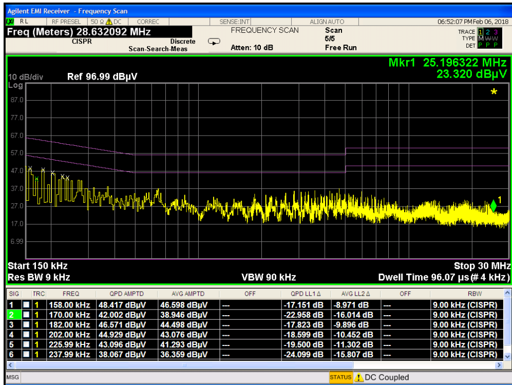
Plot 7-113. Line Conducted Plot with 802.11b (L1)
