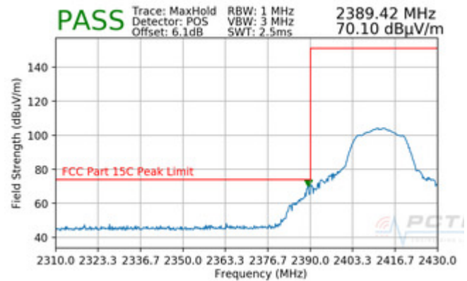
Plot 7-82. Radiated Restricted Lower Band Edge Measurement (Peak)
