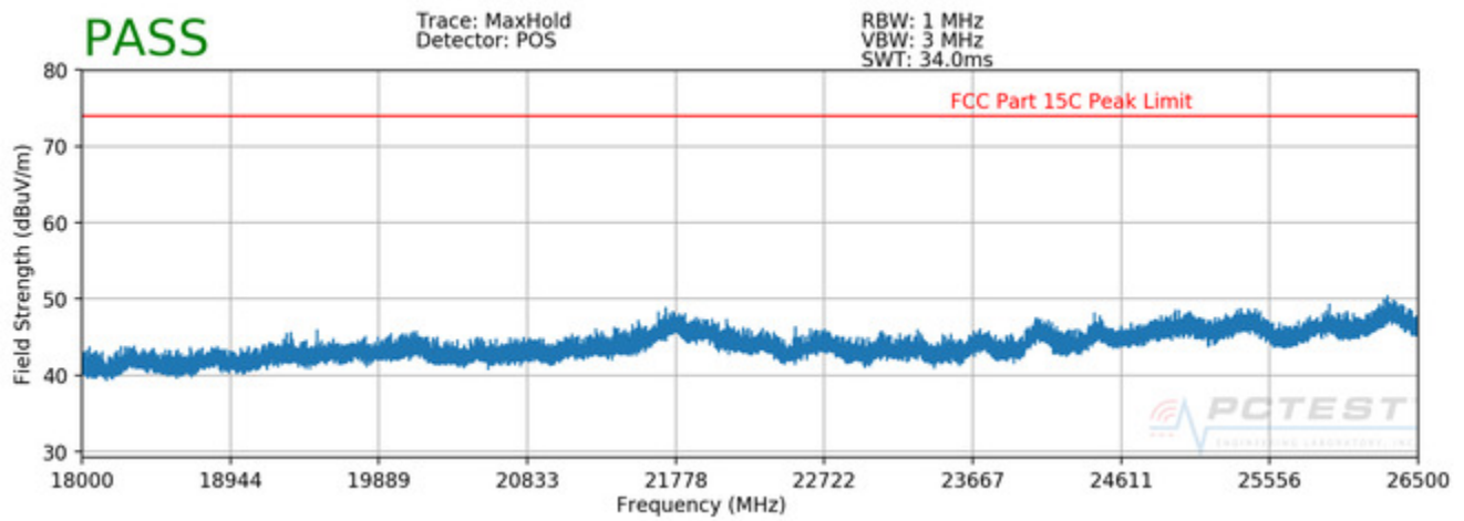
Plot 7-76. Radiated Spurious Plot above 18GHz
