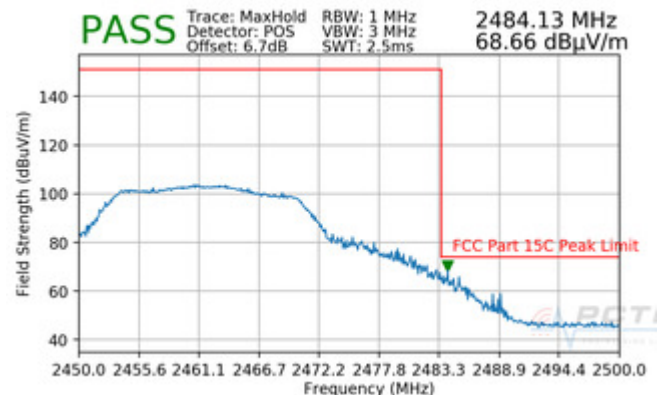
Plot 7-84. Radiated Restricted Upper Band Edge Measurement (Peak)
