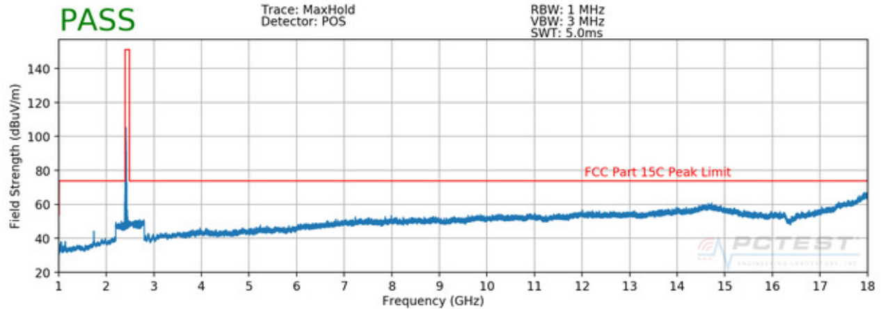
Plot 7-77. Radiated Spurious Plot above 1GHz (802.11b – Ch. 1)
