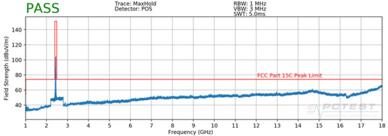
Plot 7-74. Radiated Spurious Plot above 1GHz (802.11b – Ch. 6)
