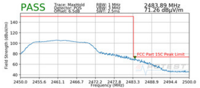
Plot 7-100. Radiated Restricted Band Edge Measurement with WCP (Peak)
