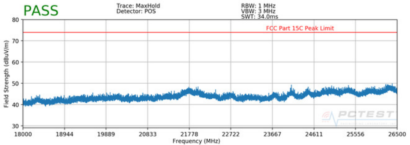
Plot 7-80. Radiated Spurious Plot above 18GHz
