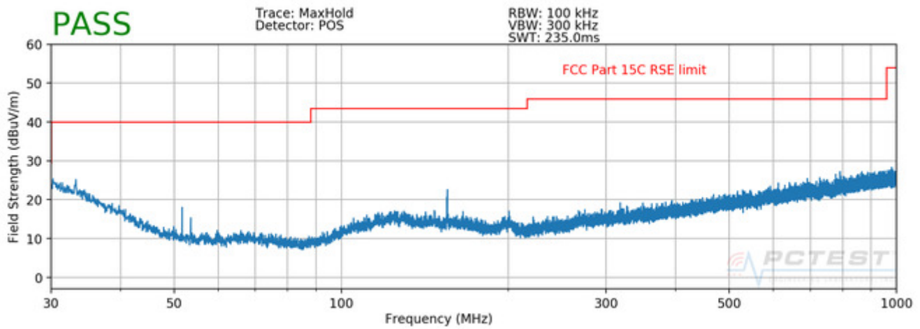
Plot 7-111. Radiated Spurious Plot below 1GHz
