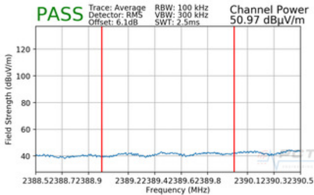
Plot 7-81. Radiated Restricted Lower Band Edge Measurement (Average)
