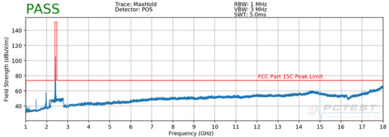
Plot 7-73. Radiated Spurious Plot above 1GHz (802.11b – Ch. 1)
