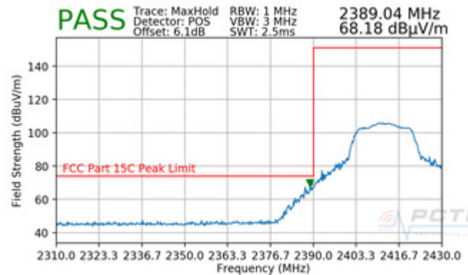
Plot 7-92. Radiated Restricted Lower Band Edge Measurement (Peak)
