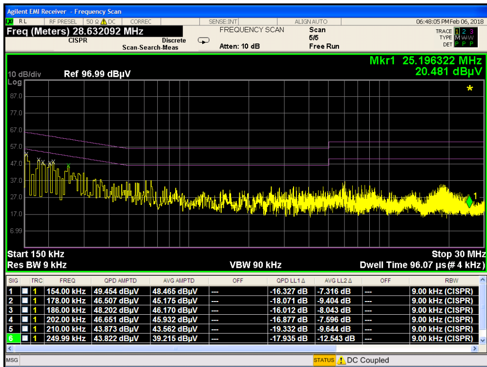
Plot 7-114. Line Conducted Plot with 802.11b (N)
