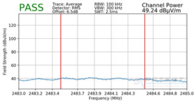
Plot 7-105. Radiated Restricted Upper Band Edge Measurement (Average)
