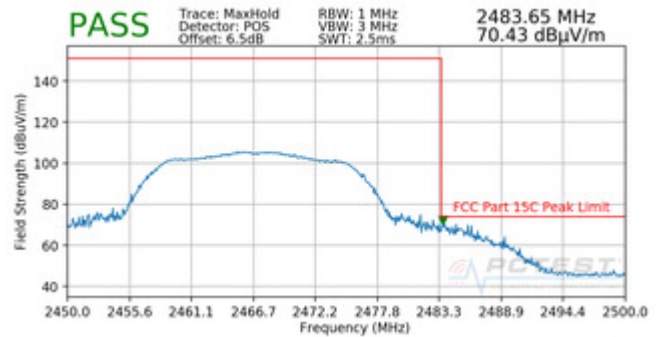
Plot 7-96. Radiated Restricted Upper Band Edge Measurement (Peak)
