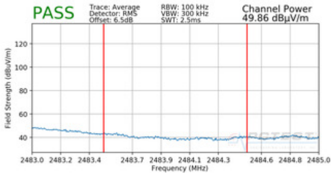
Plot 7-107. Radiated Restricted Upper Band Edge Measurement (Average)
