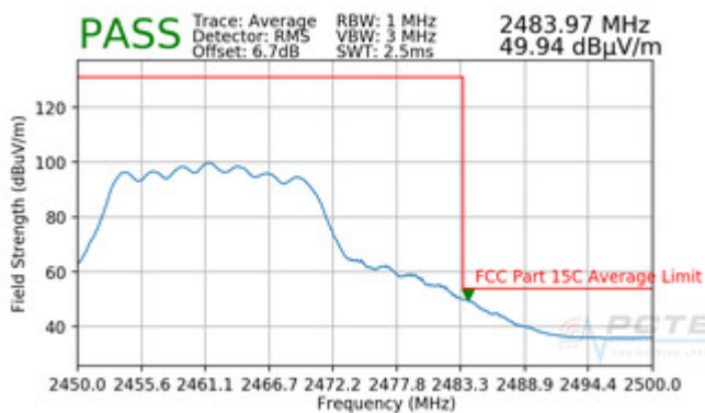
Plot 7-103. Radiated Restricted Upper Band Edge Measurement (Average)
