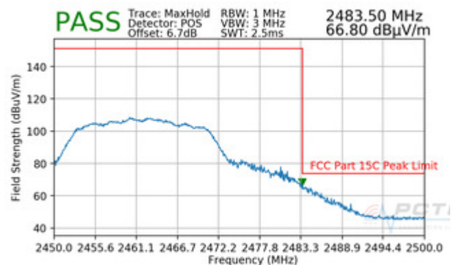
Plot 7-104. Radiated Restricted Upper Band Edge Measurement (Peak)
