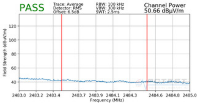
Plot 7-87. Radiated Restricted Upper Band Edge Measurement (Average)
