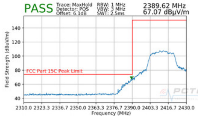
Plot 7-102. Radiated Restricted Lower Band Edge Measurement (Peak)
