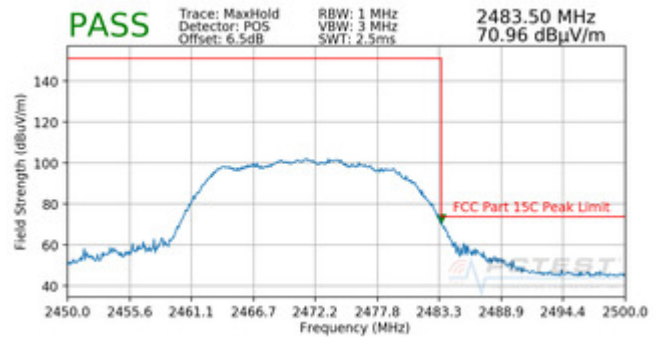
Plot 7-108. Radiated Restricted Upper Band Edge Measurement (Peak)
