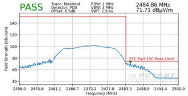
Plot 7-88. Radiated Restricted Upper Band Edge Measurement (Peak)
