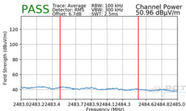
Plot 7-93. Radiated Restricted Upper Band Edge Measurement (Average)
