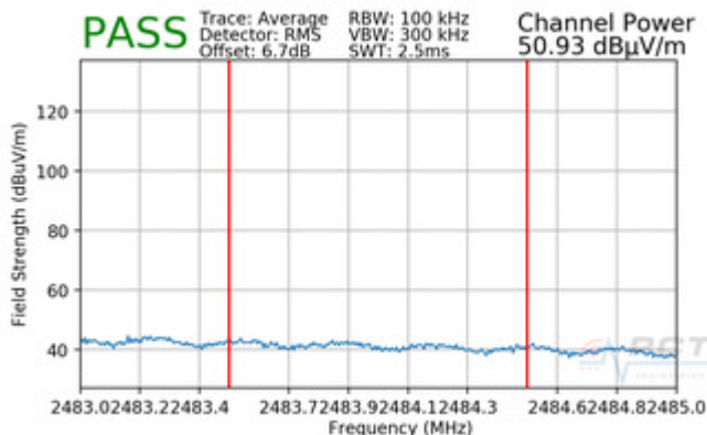
Plot 7-83. Radiated Restricted Upper Band Edge Measurement (Average)
