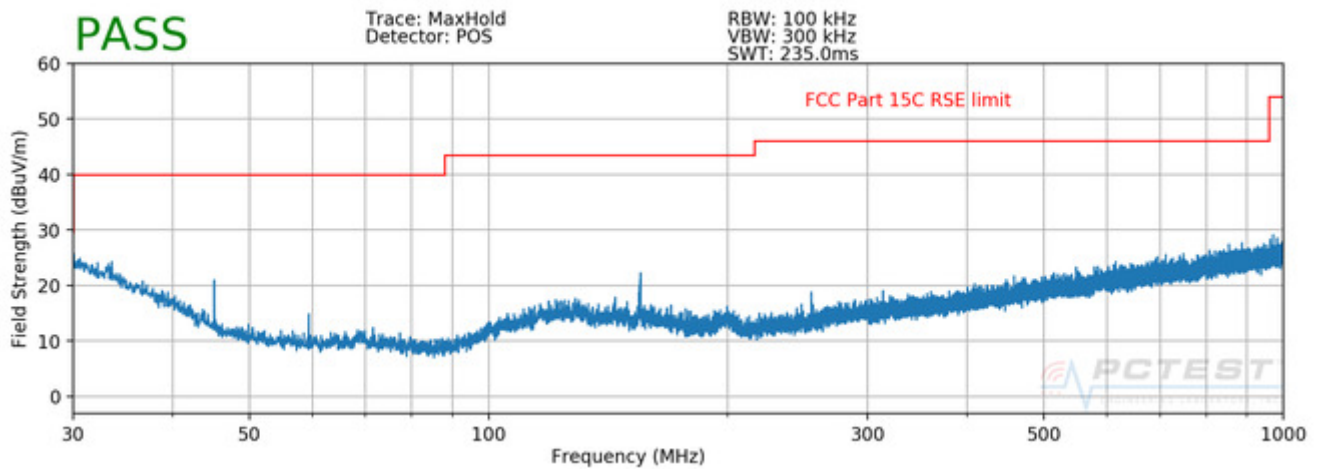
Plot 7-112. Radiated Spurious Plot below 1GHz
