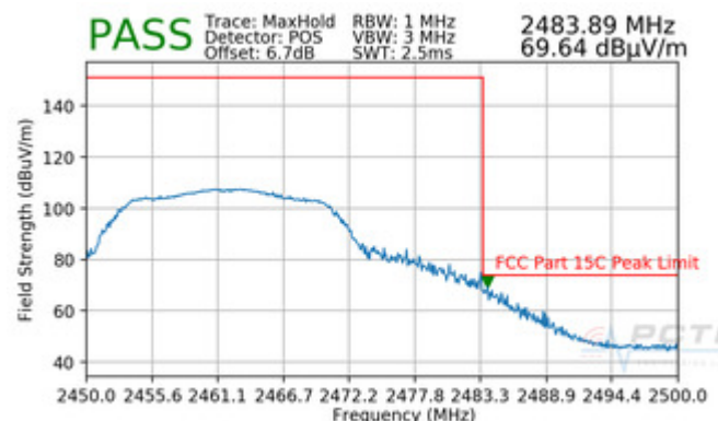
Plot 7-94. Radiated Restricted Upper Band Edge Measurement (Peak)
