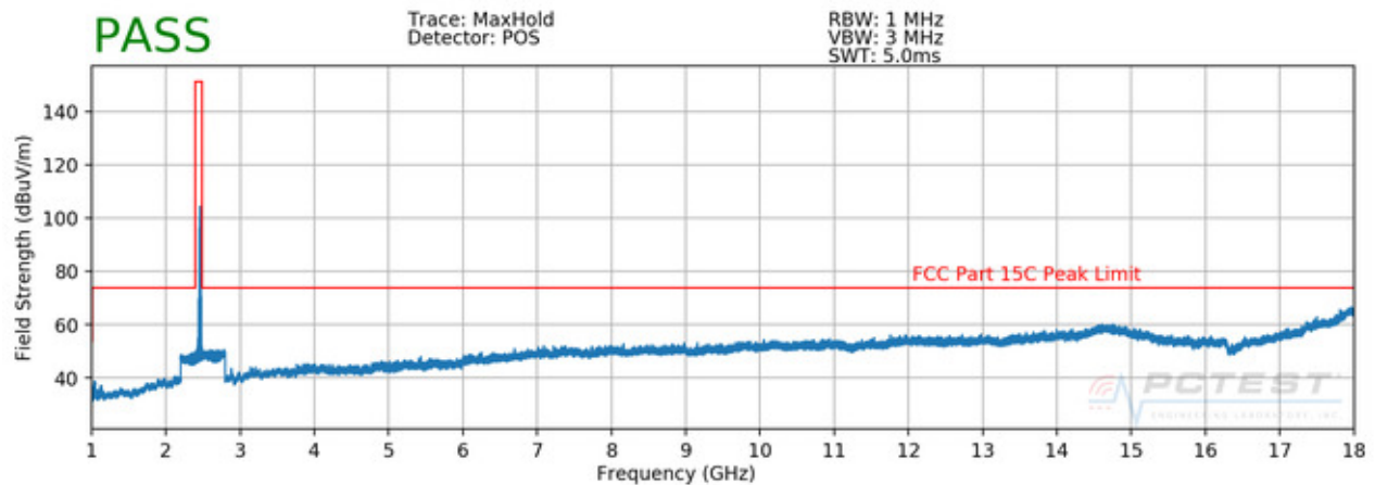
Plot 7-79. Radiated Spurious Plot above 1GHz (802.11b – Ch. 11)
