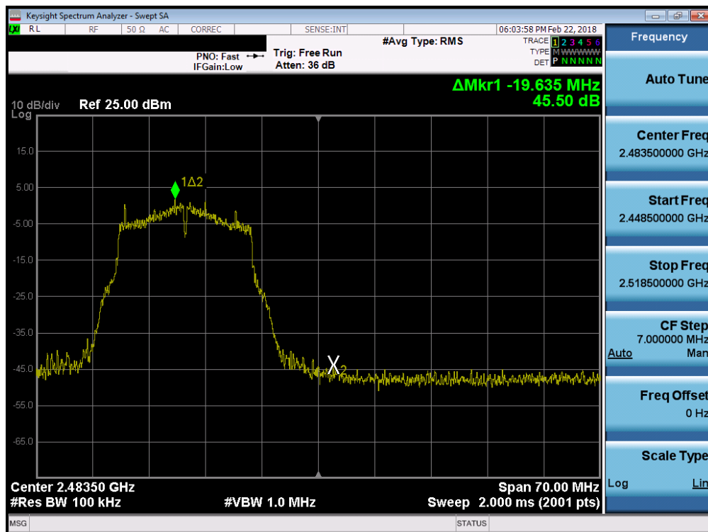
Plot 7-43. Band Edge Plot (802.11g - Ch. 12)
