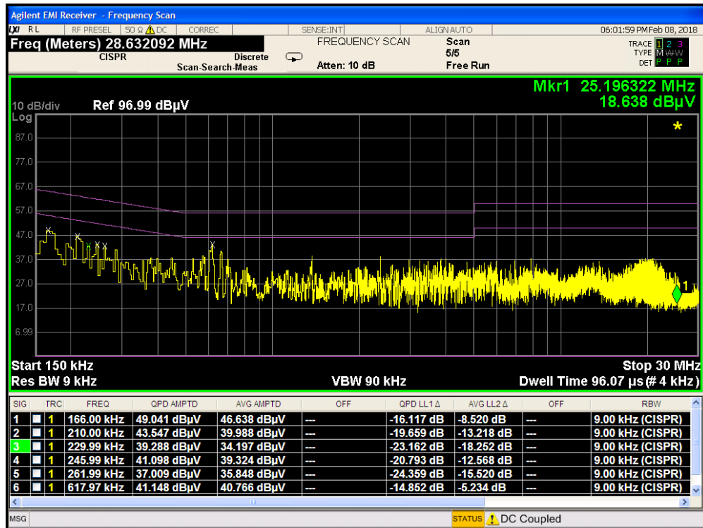
Plot 7-42. Line Conducted Plot with Bluetooth LE with WCP (N)
