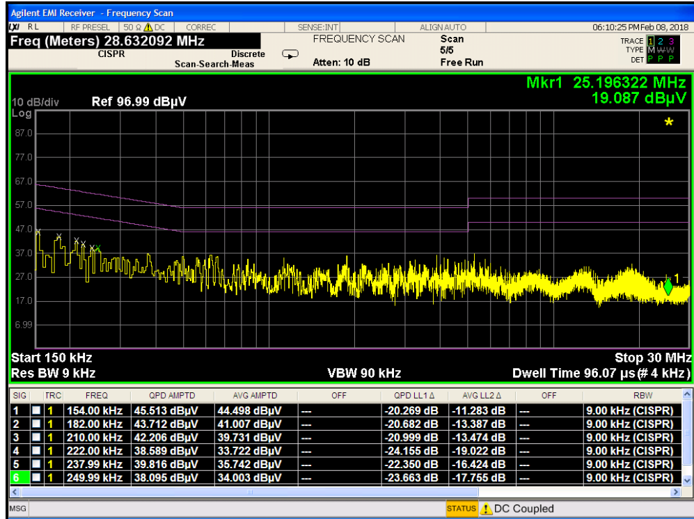
Plot 7-41. Line Conducted Plot with Bluetooth LE with WCP (L1)
