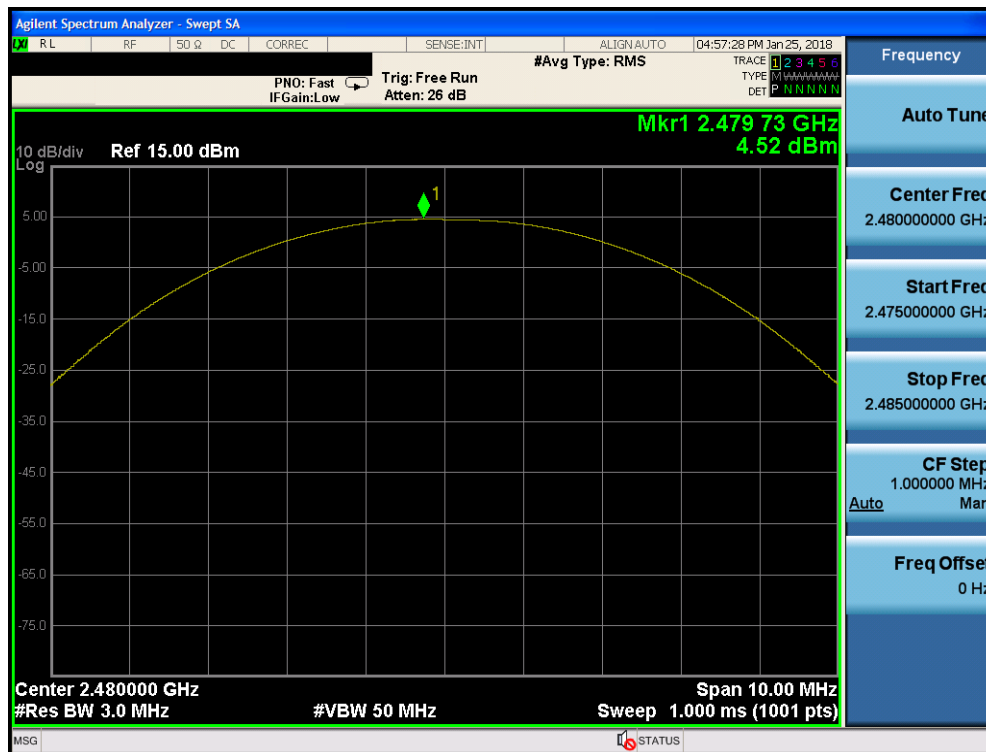
Plot 7-9. Peak Power Plot (Bluetooth (LE), 1Mbps – Ch. 39)
