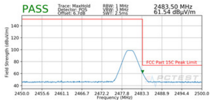
Plot 7-36. Radiated Restricted Upper Band Edge Measurement (Peak)
