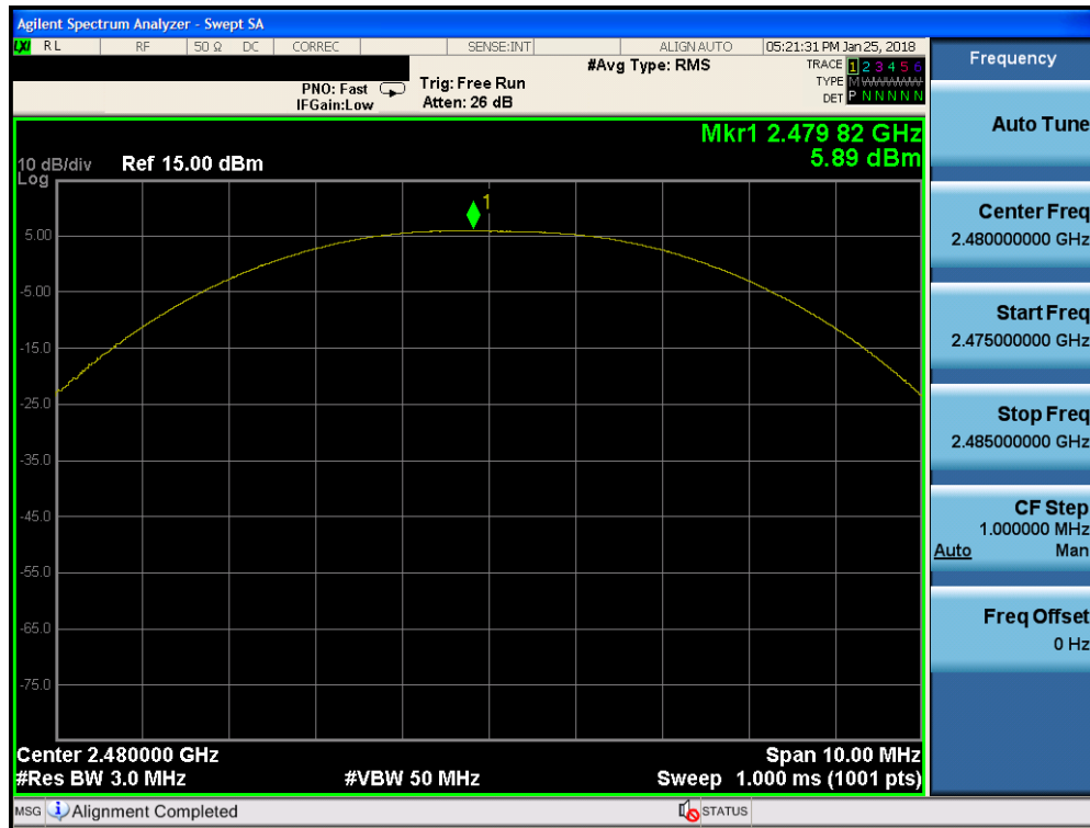
Plot 7-12. Peak Power Plot (Bluetooth (LE), 2Mbps – Ch. 39)
