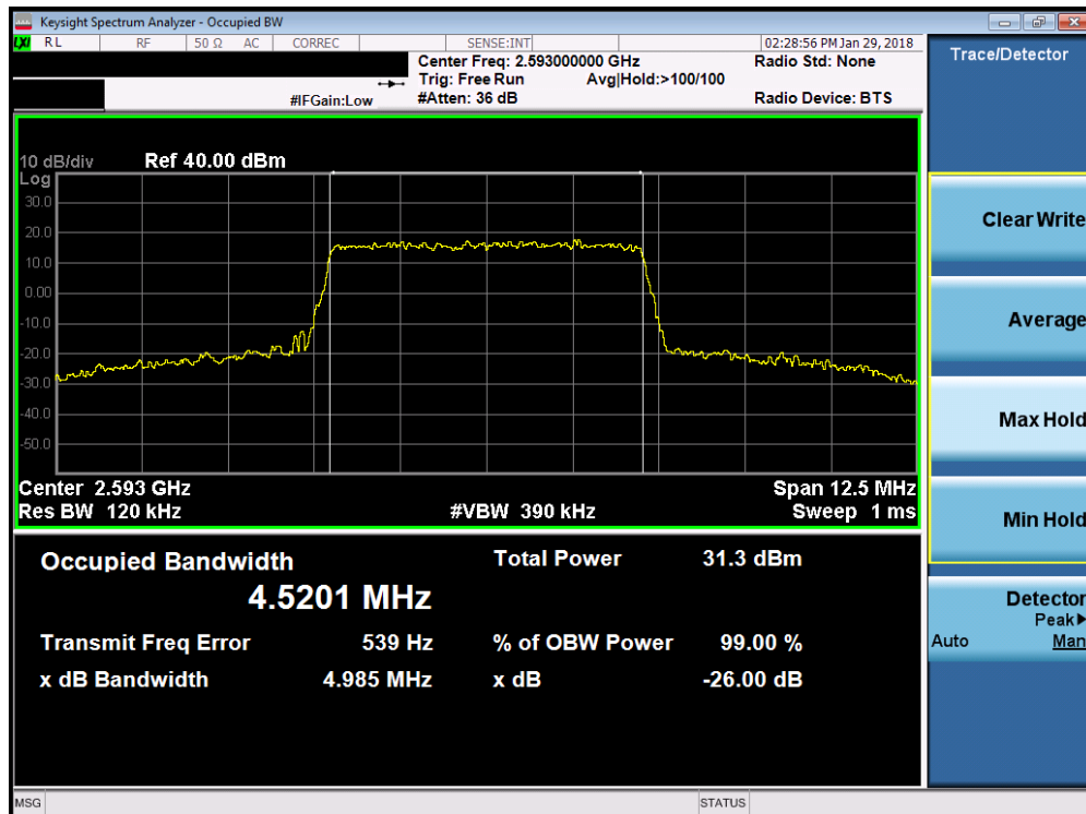
Plot 7-29. Occupied Bandwidth Plot (Band 41 - 5.0MHz 16-QAM - Full RB Configuration)
