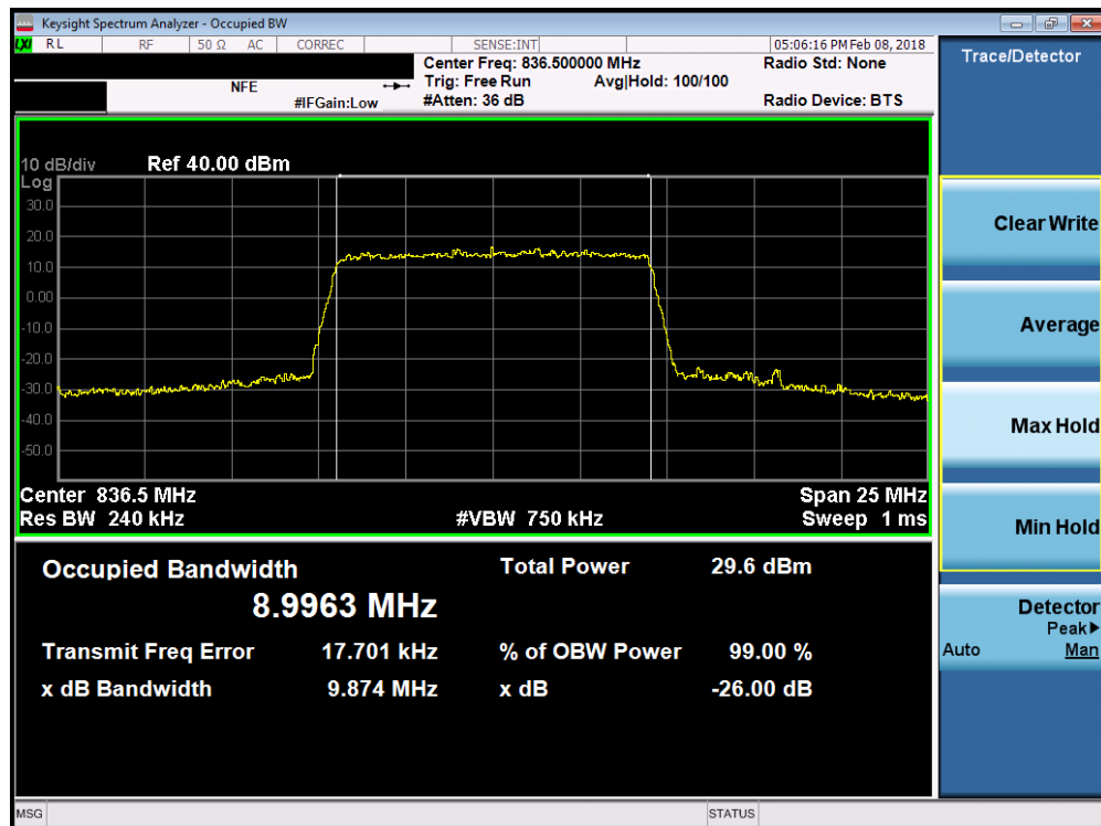
Plot 7-24. Occupied Bandwidth Plot (Band 5/26 - 10.0MHz 64-QAM - Full RB Configuration)
