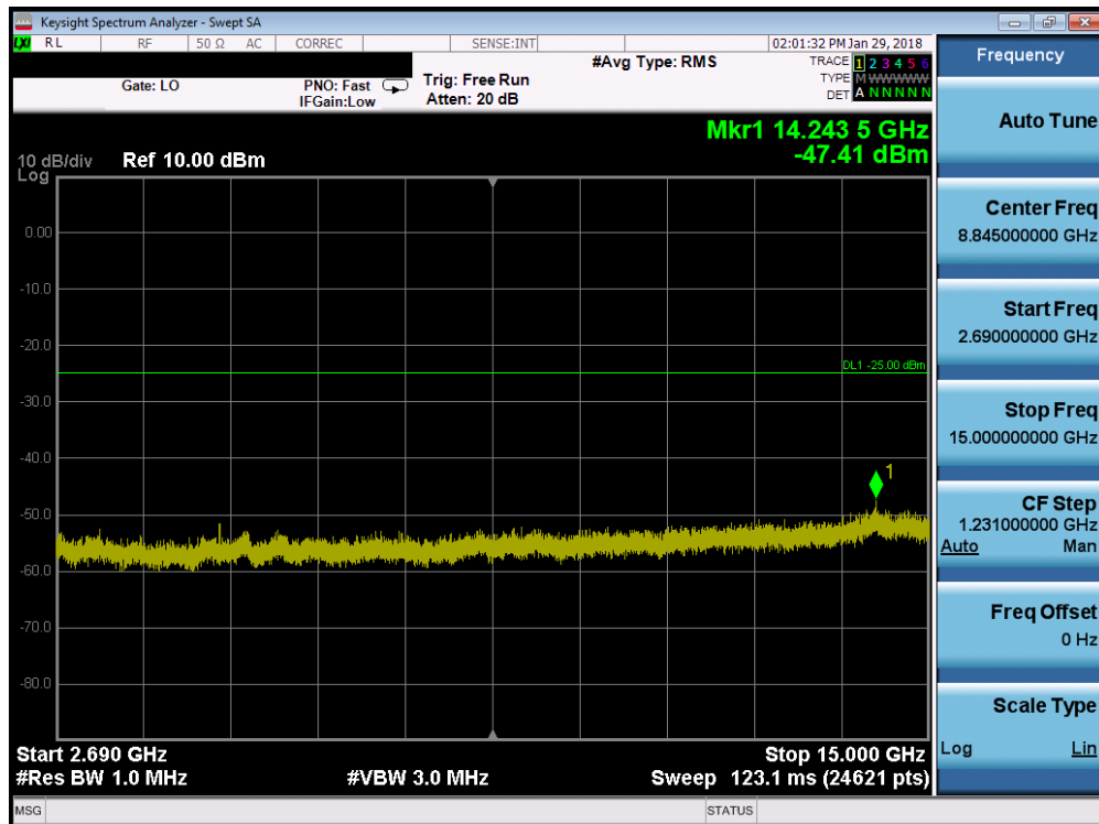
Plot 7-68. Conducted Spurious Plot (Band 41 - 20.0MHz QPSK - RB Size 1, RB Offset 0 - Low Channel)
