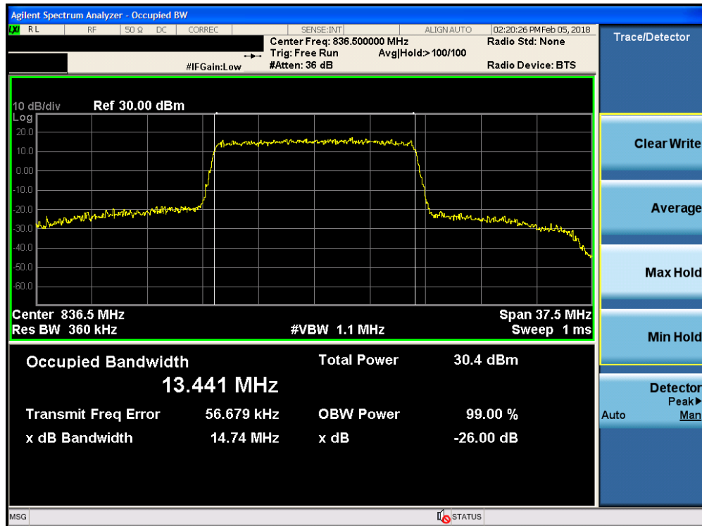
Plot 7-27. Occupied Bandwidth Plot (Band 26 - 15.0MHz 64-QAM - Full RB Configuration)
