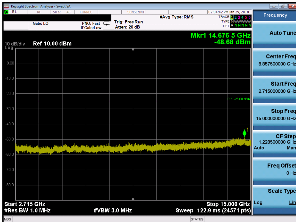
Plot 7-74. Conducted Spurious Plot (Band 41 - 20.0MHz QPSK - RB Size 1, RB Offset 0 - High Channel)
