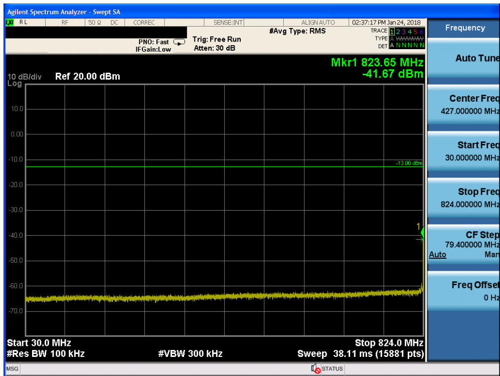
Plot 7-61. Conducted Spurious Plot (Band 5/26 - 10.0MHz QPSK - RB Size 1, RB Offset 0 - Mid Channel)
