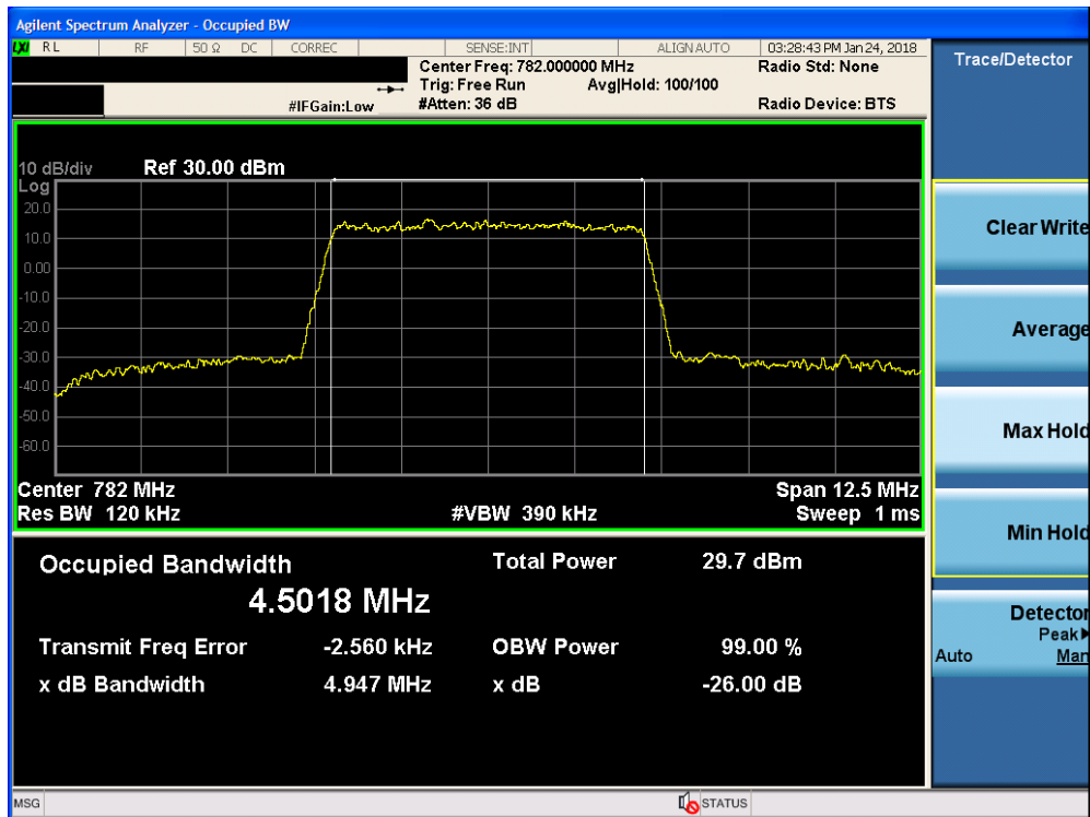
Plot 7-8. Occupied Bandwidth Plot (Band 13 - 5.0MHz 16-QAM - Full RB Configuration)
