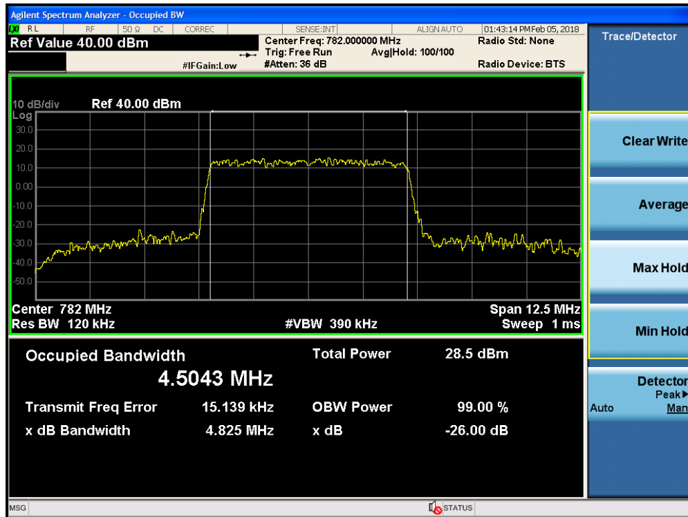
Plot 7-9. Occupied Bandwidth Plot (Band 13 - 5.0MHz 64-QAM - Full RB Configuration)
