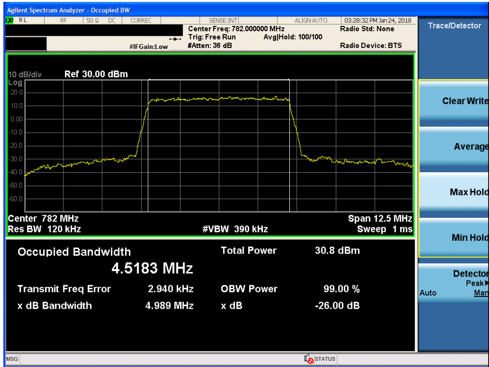
Plot 7-7. Occupied Bandwidth Plot (Band 13 - 5.0MHz QPSK - Full RB Configuration)
