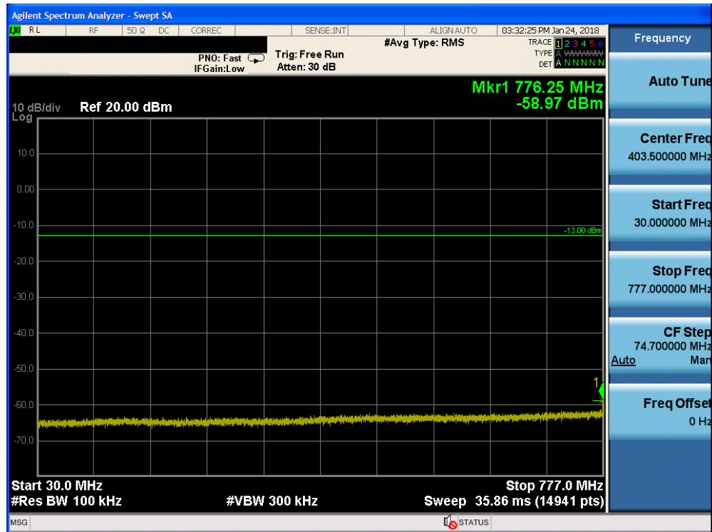
Plot 7-55. Conducted Spurious Plot (Band 13 - 5.0MHz QPSK - RB Size 1, RB Offset 0 - High Channel)
