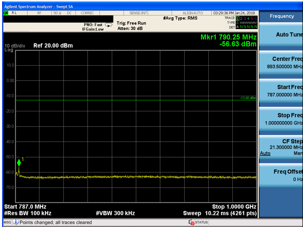
Plot 7-53. Conducted Spurious Plot (Band 13 - 5.0MHz QPSK - RB Size 1, RB Offset 0 - Mid Channel)
