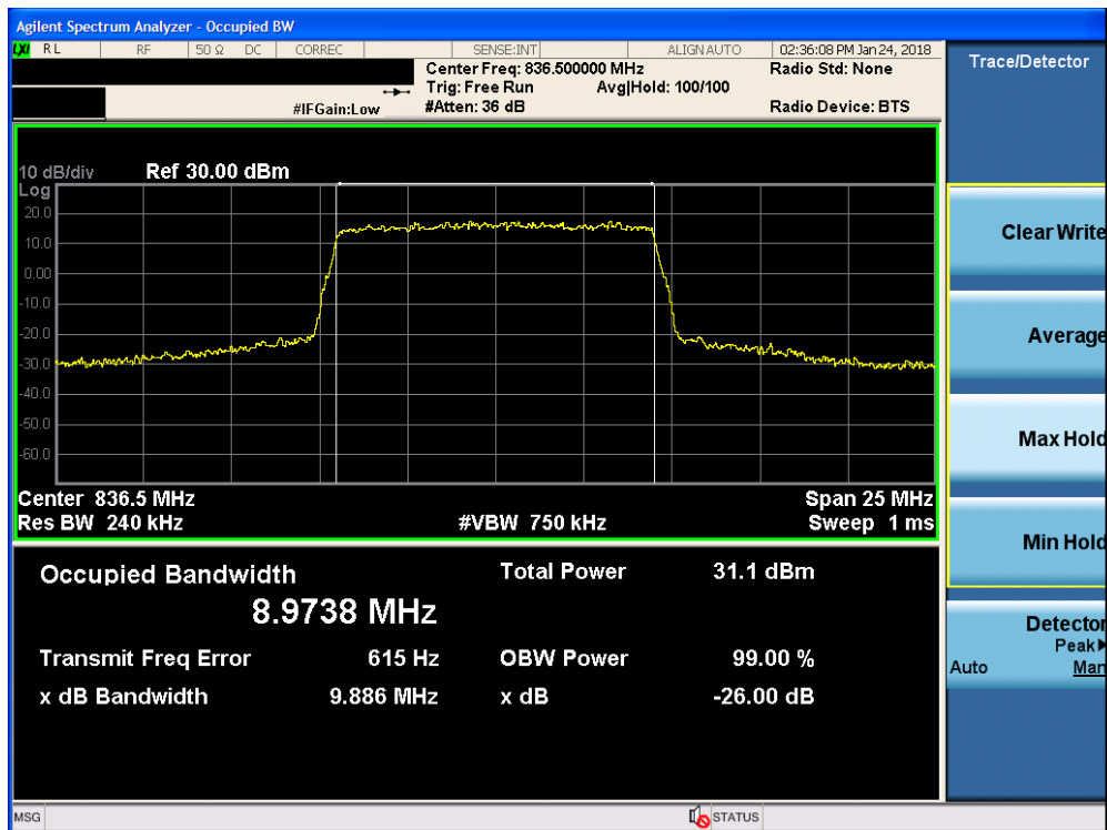
Plot 7-22. Occupied Bandwidth Plot (Band 5/26 - 10.0MHz QPSK - Full RB Configuration)
