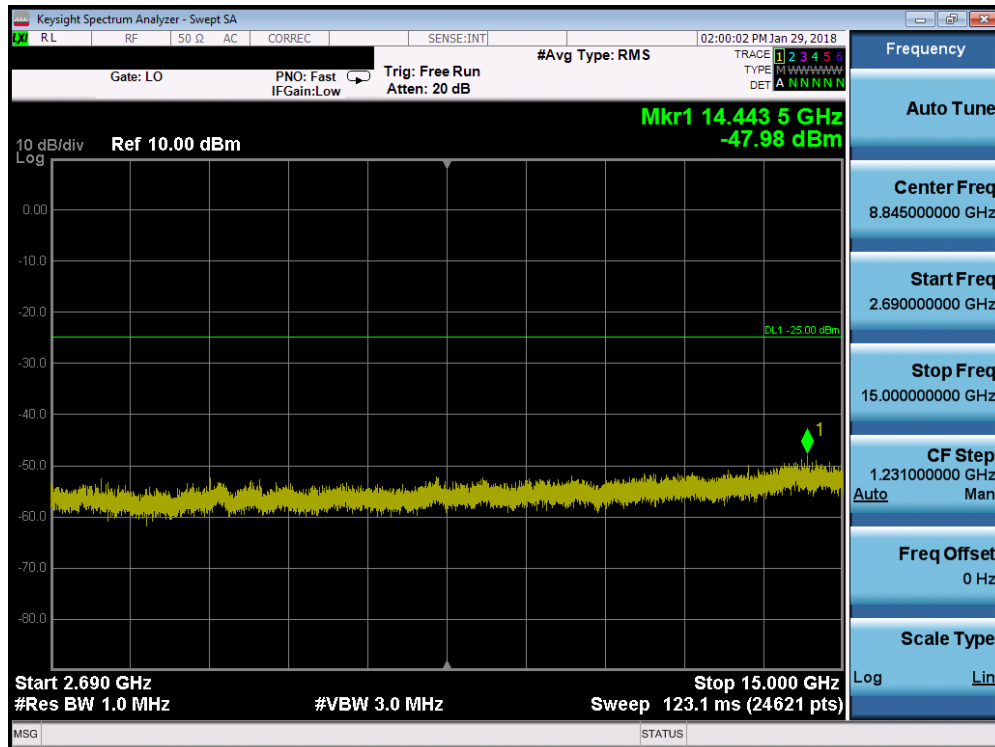
Plot 7-71. Conducted Spurious Plot (Band 41 - 20.0MHz QPSK - RB Size 1, RB Offset 0 - Mid Channel)
