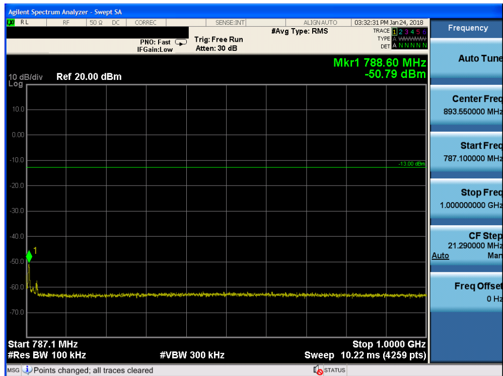
Plot 7-56. Conducted Spurious Plot (Band 13 - 5.0MHz QPSK - RB Size 1, RB Offset 0 - High Channel)
