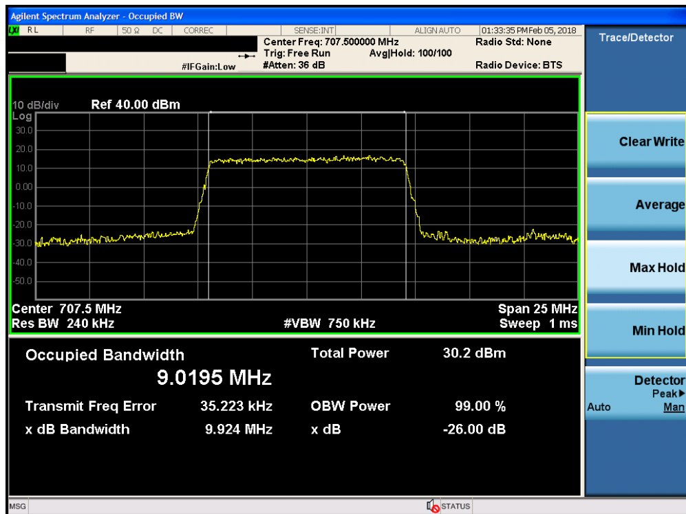
Plot 7-6. Occupied Bandwidth Plot (Band 17 - 10.0MHz 64-QAM - Full RB Configuration)
