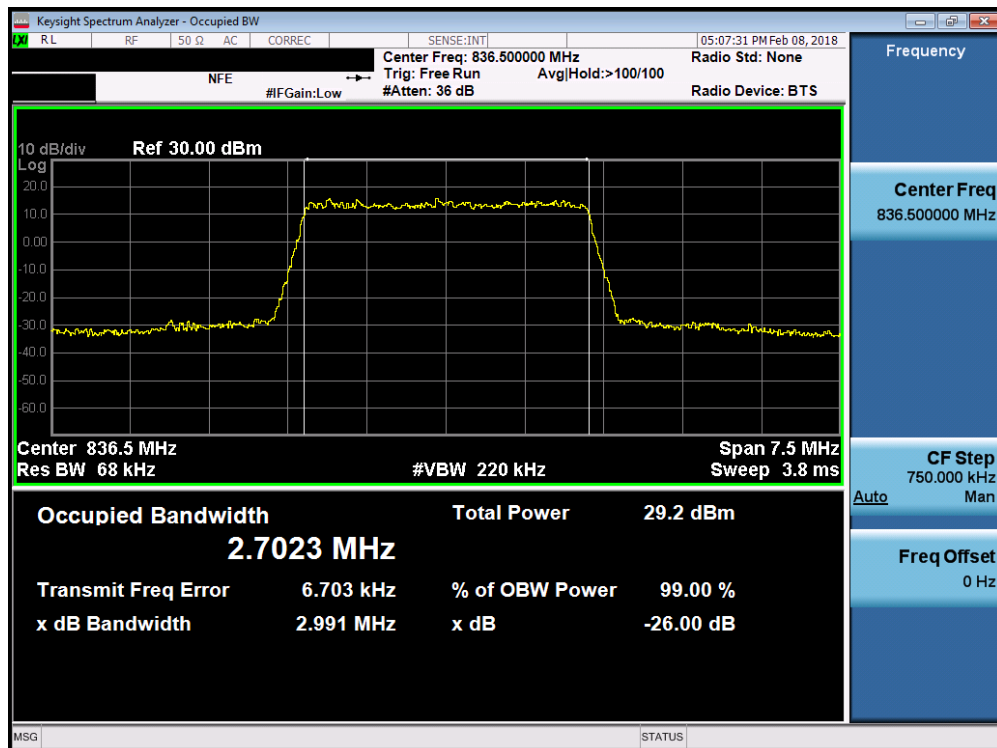
Plot 7-18. Occupied Bandwidth Plot (Band 5/26 - 3.0MHz 64-QAM - Full RB Configuration)
