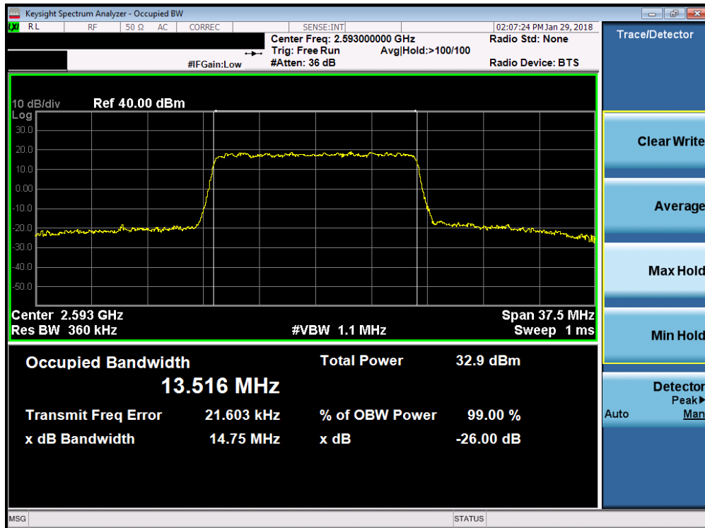
Plot 7-34. Occupied Bandwidth Plot (Band 41 - 15.0MHz QPSK - Full RB Configuration)
