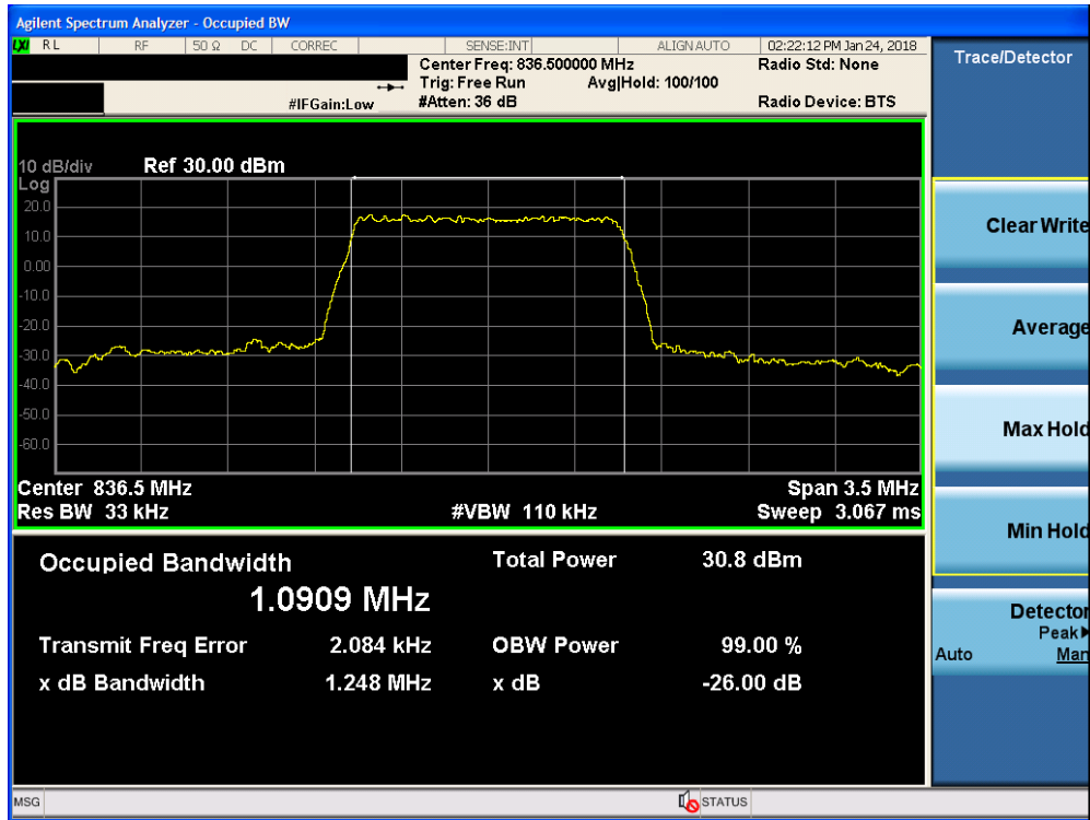
Plot 7-13. Occupied Bandwidth Plot (Band 5/26 - 1.4MHz QPSK - Full RB Configuration)
