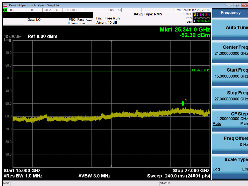
Plot 7-72. Conducted Spurious Plot (Band 41 - 20.0MHz QPSK - RB Size 1, RB Offset 0 - Mid Channel)
