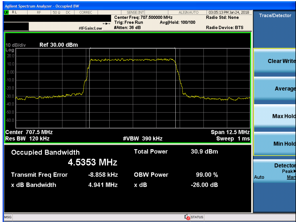
Plot 7-1. Occupied Bandwidth Plot (Band 17 - 5.0MHz QPSK - Full RB Configuration)
