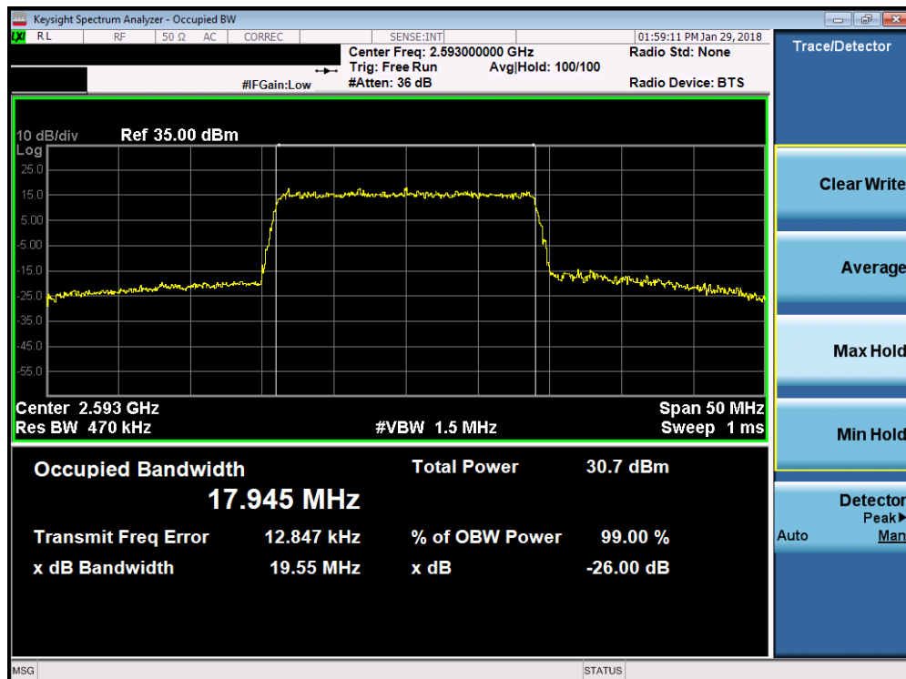
Plot 7-39. Occupied Bandwidth Plot (Band 41 - 20.0MHz 64-QAM - Full RB Configuration)
