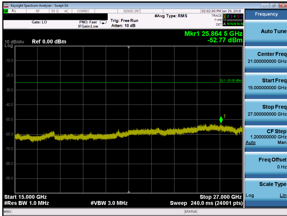
Plot 7-69. Conducted Spurious Plot (Band 41 - 20.0MHz QPSK - RB Size 1, RB Offset 0 - Low Channel)
