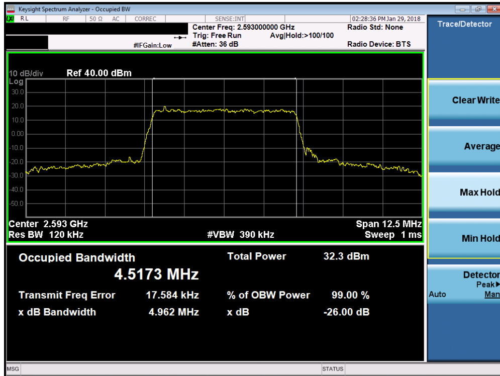
Plot 7-28. Occupied Bandwidth Plot (Band 41 - 5.0MHz QPSK - Full RB Configuration)
