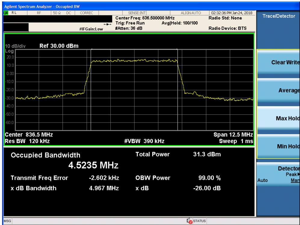
Plot 7-19. Occupied Bandwidth Plot (Band 5/26 - 5.0MHz QPSK - Full RB Configuration)
