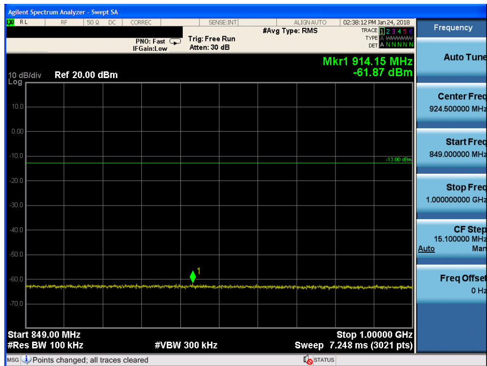
Plot 7-59. Conducted Spurious Plot (Band 5/26 - 10.0MHz QPSK - RB Size 1, RB Offset 0 - Low Channel)
