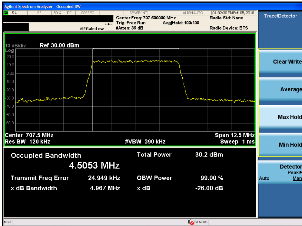
Plot 7-3. Occupied Bandwidth Plot (Band 17 - 5.0MHz 64-QAM - Full RB Configuration)
