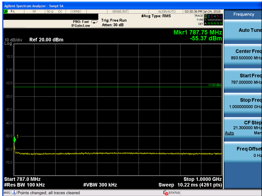
Plot 7-50. Conducted Spurious Plot (Band 13 - 5.0MHz QPSK - RB Size 1, RB Offset 0 - Low Channel)
