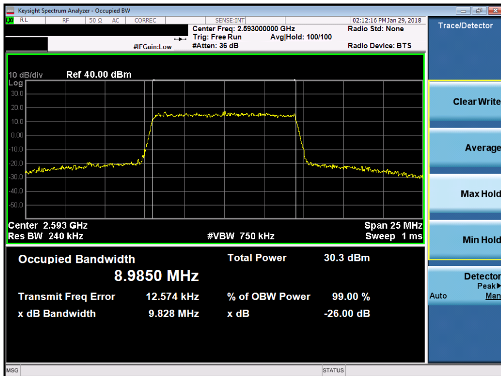
Plot 7-33. Occupied Bandwidth Plot (Band 41 - 10.0MHz 64-QAM - Full RB Configuration)
