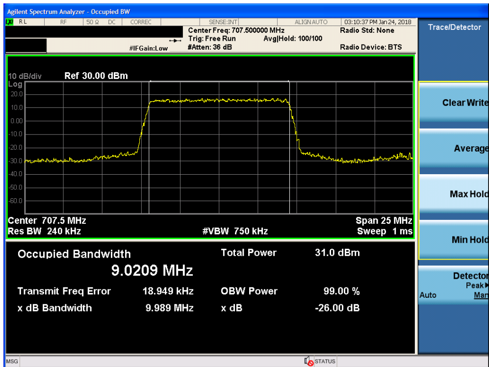
Plot 7-4. Occupied Bandwidth Plot (Band 17 - 10.0MHz QPSK - Full RB Configuration)
