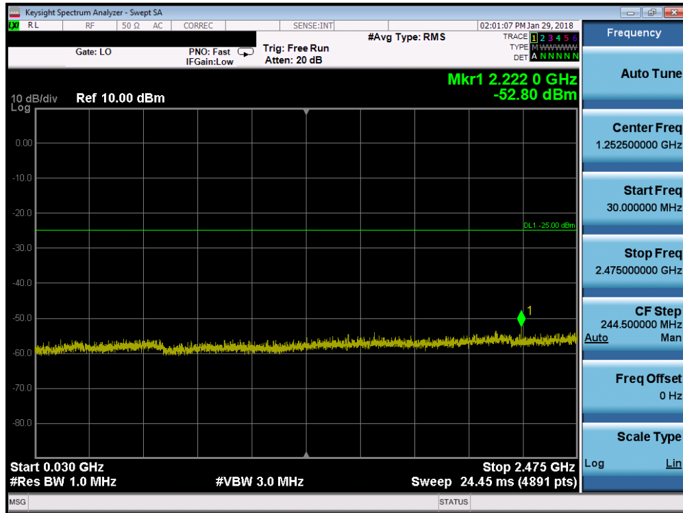
Plot 7-67. Conducted Spurious Plot (Band 41 - 20.0MHz QPSK - RB Size 1, RB Offset 0 - Low Channel)
