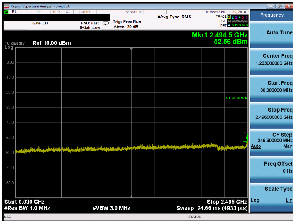
Plot 7-70. Conducted Spurious Plot (Band 41 - 20.0MHz QPSK - RB Size 1, RB Offset 0 - Mid Channel)
