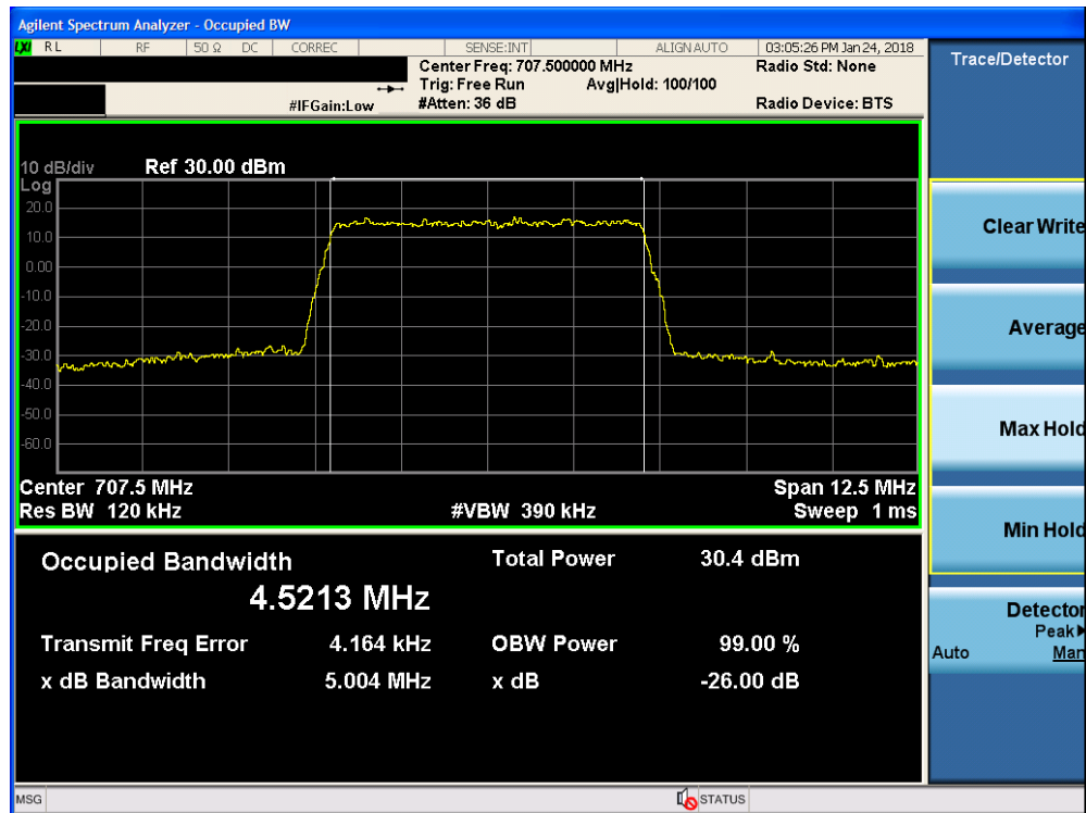
Plot 7-2. Occupied Bandwidth Plot (Band 17 - 5.0MHz 16-QAM - Full RB Configuration)
