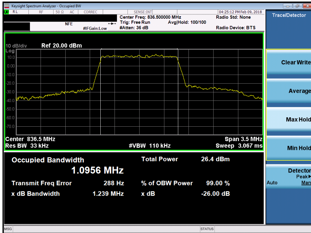
Plot 7-15. Occupied Bandwidth Plot (Band 5/26 - 1.4MHz 64-QAM - Full RB Configuration)
