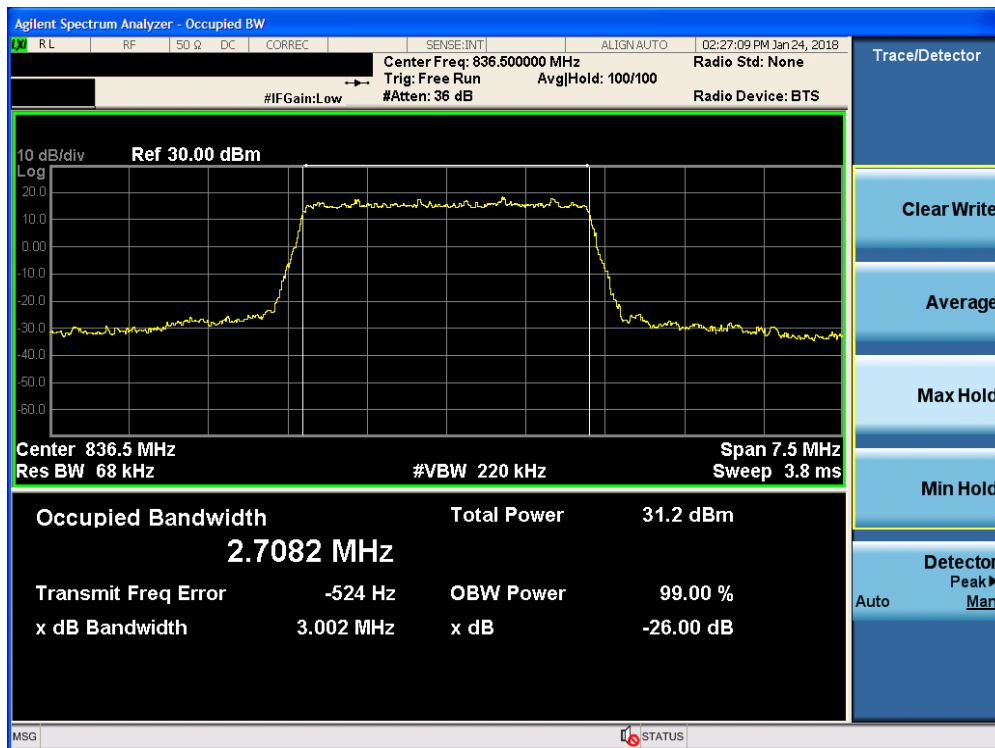
Plot 7-16. Occupied Bandwidth Plot (Band 5/26 - 3.0MHz QPSK - Full RB Configuration)
