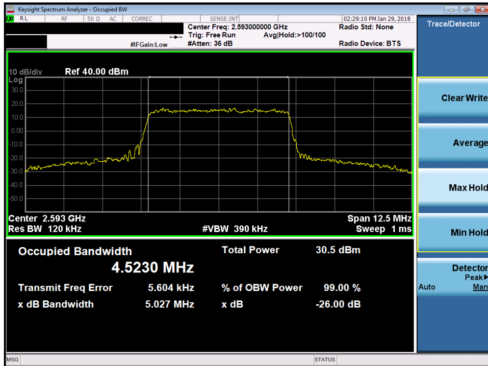
Plot 7-30. Occupied Bandwidth Plot (Band 41 - 5.0MHz 64-QAM - Full RB Configuration)
