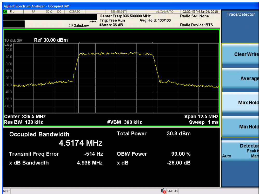
Plot 7-20. Occupied Bandwidth Plot (Band 5/26 - 5.0MHz 16-QAM - Full RB Configuration)
