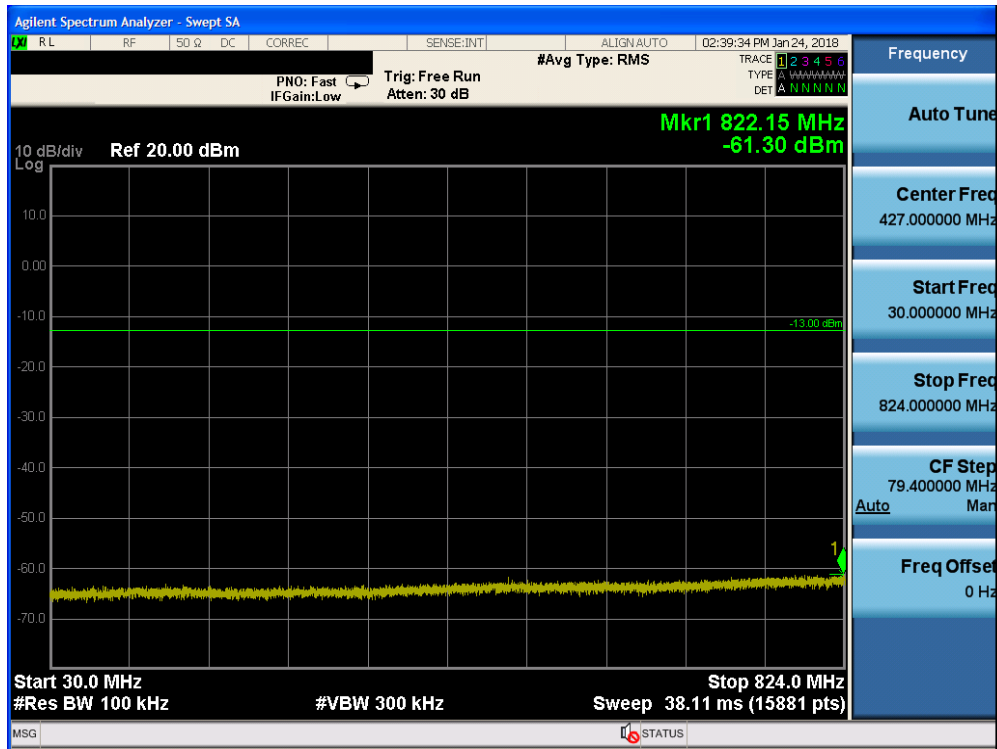
Plot 7-64. Conducted Spurious Plot (Band 5/26 - 10.0MHz QPSK - RB Size 1, RB Offset 0 - High Channel)
