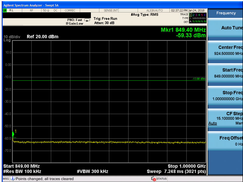
Plot 7-62. Conducted Spurious Plot (Band 5/26 - 10.0MHz QPSK - RB Size 1, RB Offset 0 - Mid Channel)
