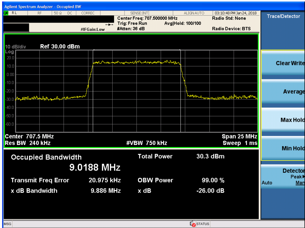
Plot 7-5. Occupied Bandwidth Plot (Band 17 - 10.0MHz 16-QAM - Full RB Configuration)
