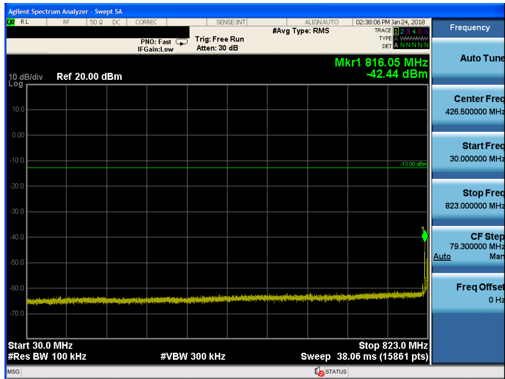
Plot 7-58. Conducted Spurious Plot (Band 5/26 - 10.0MHz QPSK - RB Size 1, RB Offset 0 - Low Channel)
