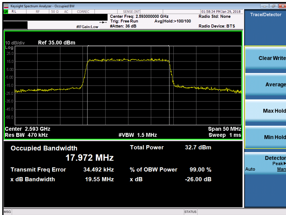
Plot 7-37. Occupied Bandwidth Plot (Band 41 - 20.0MHz QPSK - Full RB Configuration)
