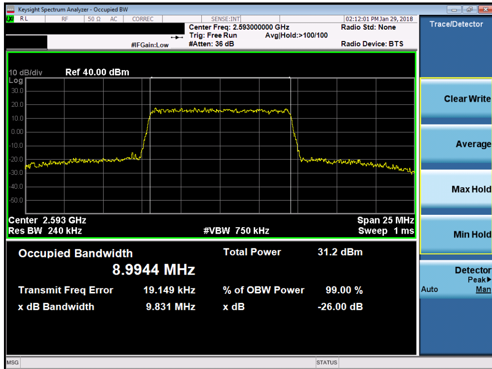
Plot 7-32. Occupied Bandwidth Plot (Band 41 - 10.0MHz 16-QAM - Full RB Configuration)
