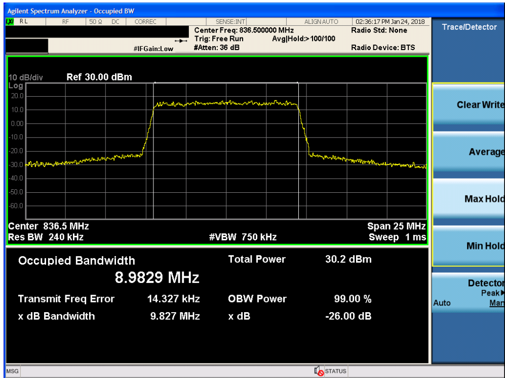
Plot 7-23. Occupied Bandwidth Plot (Band 5/26 - 10.0MHz 16-QAM - Full RB Configuration)
