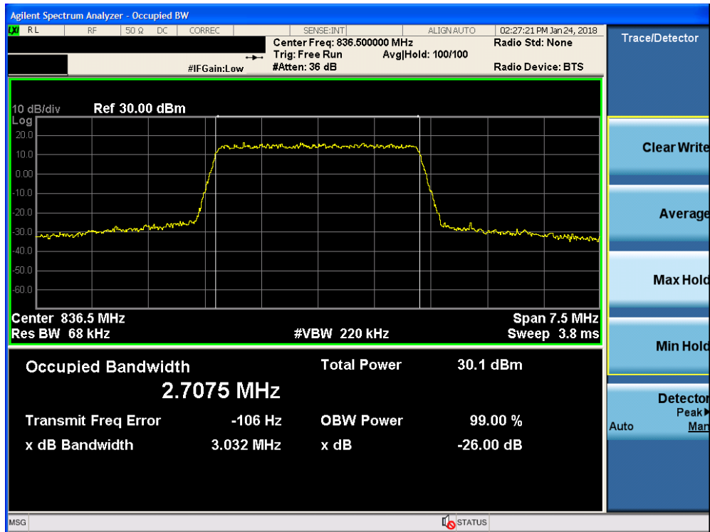
Plot 7-17. Occupied Bandwidth Plot (Band 5/26 - 3.0MHz 16-QAM - Full RB Configuration)
