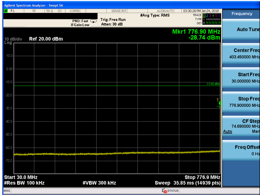
Plot 7-49. Conducted Spurious Plot (Band 13 - 5.0MHz QPSK - RB Size 1, RB Offset 0 - Low Channel)
