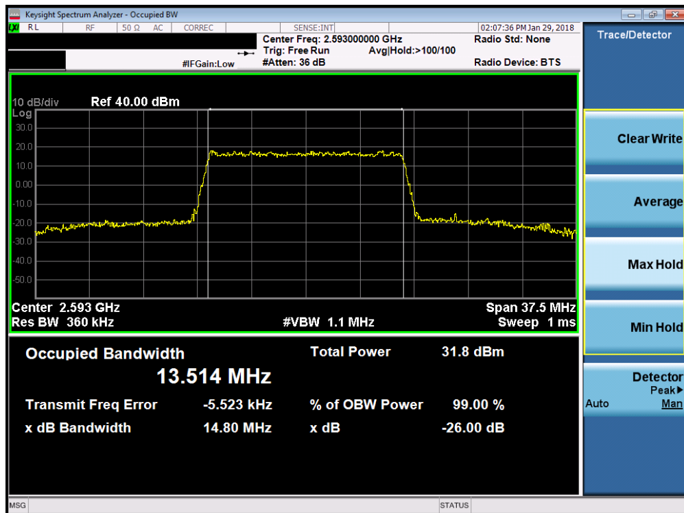
Plot 7-35. Occupied Bandwidth Plot (Band 41 - 15.0MHz 16-QAM - Full RB Configuration)
