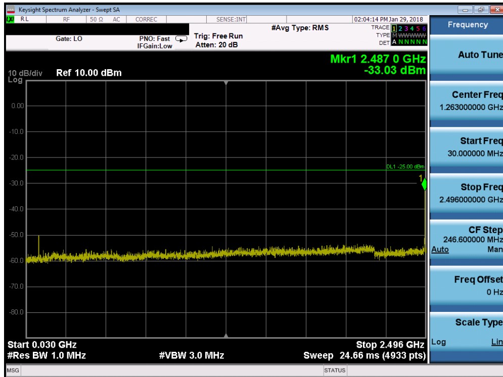
Plot 7-73. Conducted Spurious Plot (Band 41 - 20.0MHz QPSK - RB Size 1, RB Offset 0 - High Channel)
