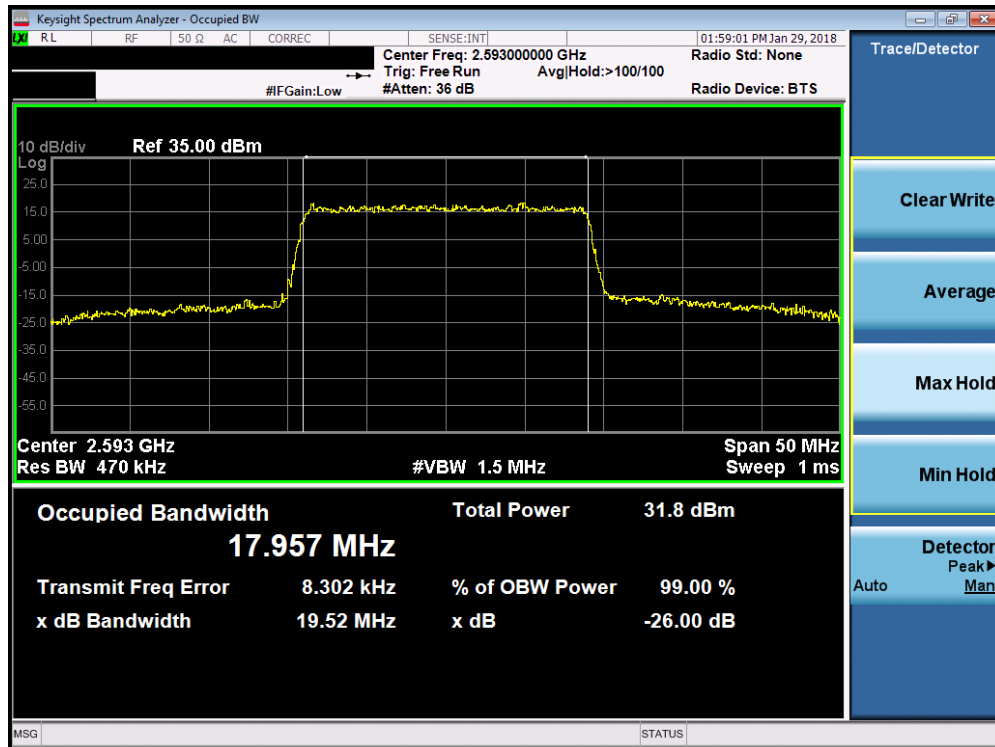
Plot 7-38. Occupied Bandwidth Plot (Band 41 - 20.0MHz 16-QAM - Full RB Configuration)
