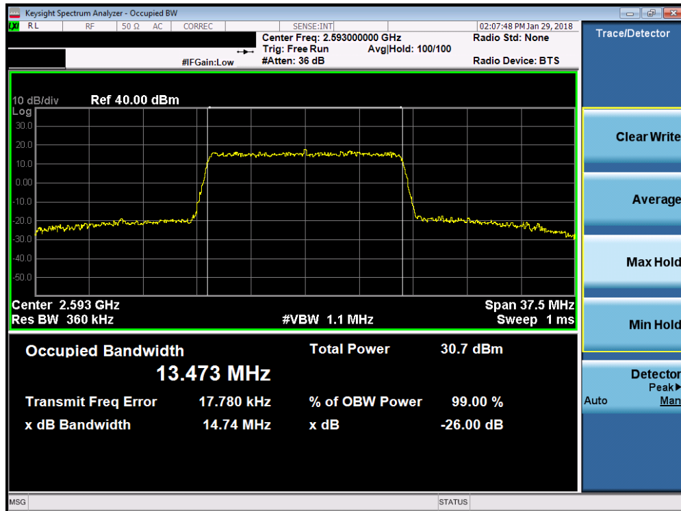
Plot 7-36. Occupied Bandwidth Plot (Band 41 - 15.0MHz 64-QAM - Full RB Configuration)
