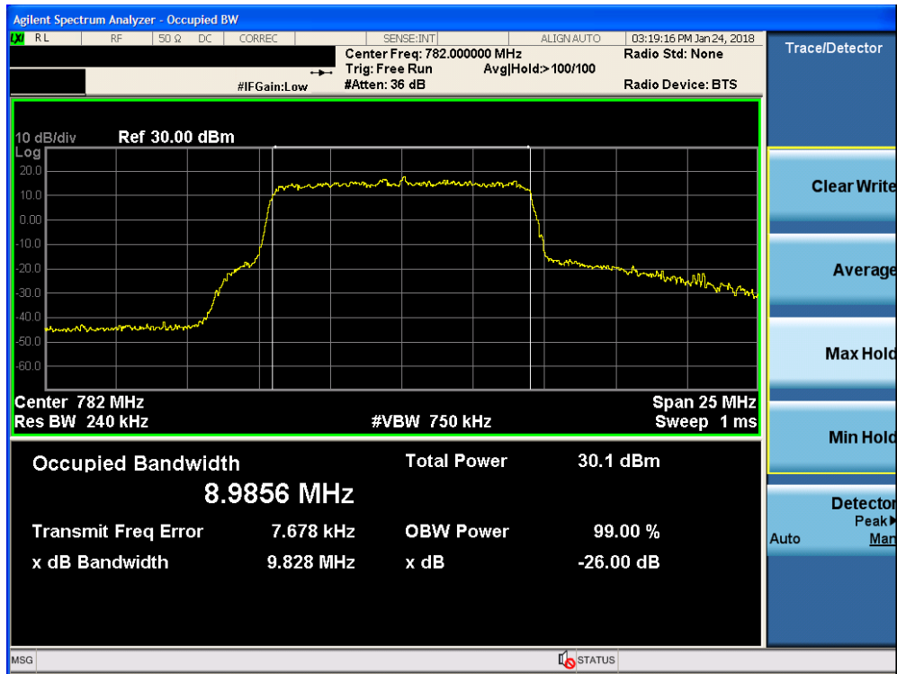
Plot 7-11. Occupied Bandwidth Plot (Band 13 - 10.0MHz 16-QAM - Full RB Configuration)
