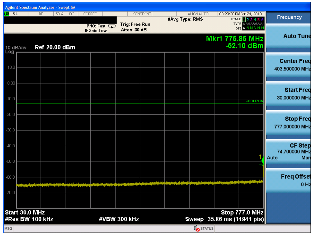
Plot 7-52. Conducted Spurious Plot (Band 13 - 5.0MHz QPSK - RB Size 1, RB Offset 0 - Mid Channel)
