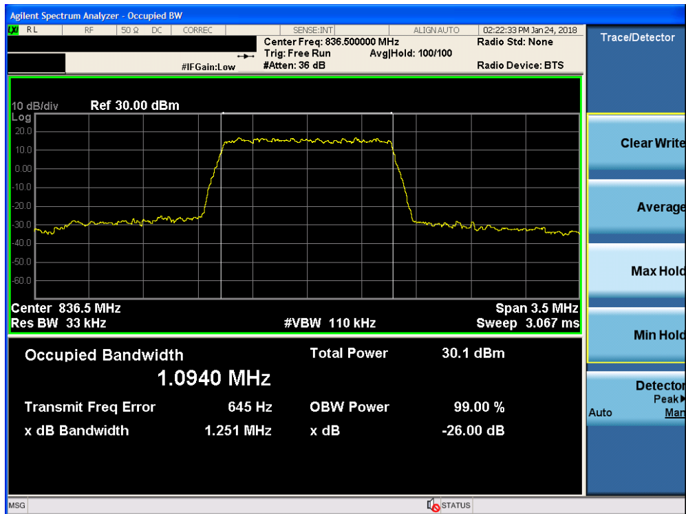
Plot 7-14. Occupied Bandwidth Plot (Band 5/26 - 1.4MHz 16-QAM - Full RB Configuration)
