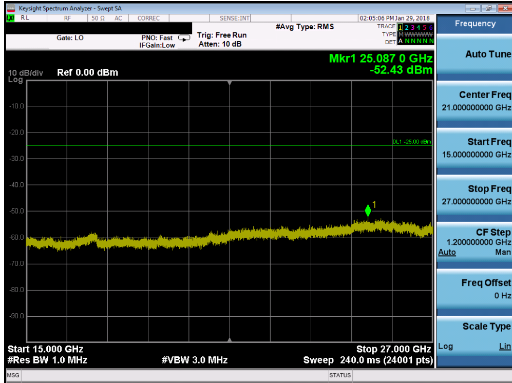
Plot 7-75. Conducted Spurious Plot (Band 41 - 20.0MHz QPSK - RB Size 1, RB Offset 0 - High Channel)
