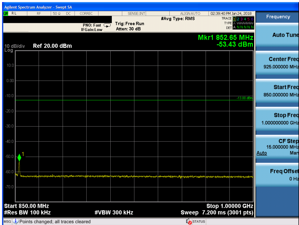
Plot 7-65. Conducted Spurious Plot (Band 5/26 - 10.0MHz QPSK - RB Size 1, RB Offset 0 - High Channel)
