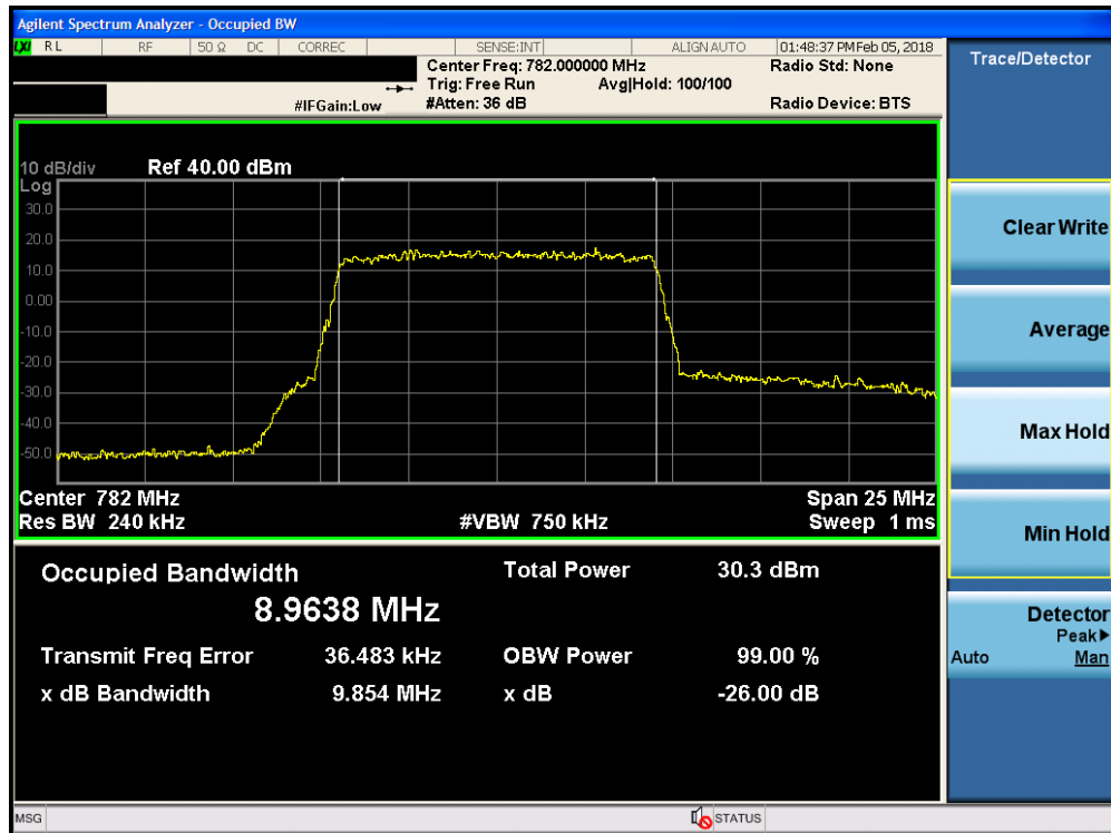
Plot 7-12. Occupied Bandwidth Plot (Band 13 - 10.0MHz 64-QAM - Full RB Configuration)
