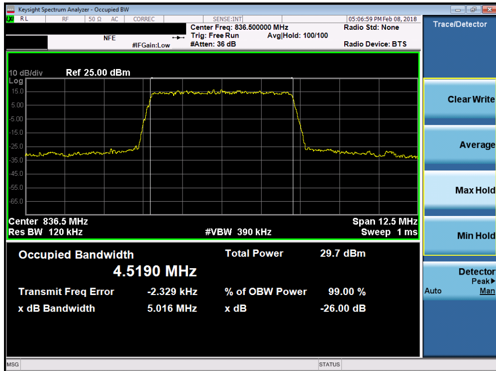
Plot 7-21. Occupied Bandwidth Plot (Band 5/26 - 5.0MHz 64-QAM - Full RB Configuration)
