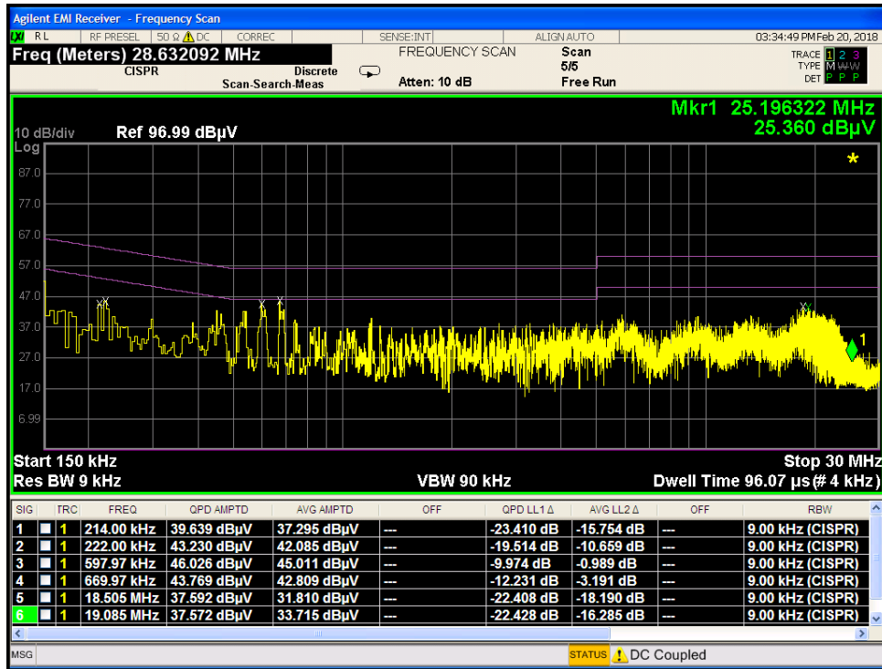
Plot 7-10. Line-Conducted Test Plot (L1) with WCP - Terminated in 50Ω
