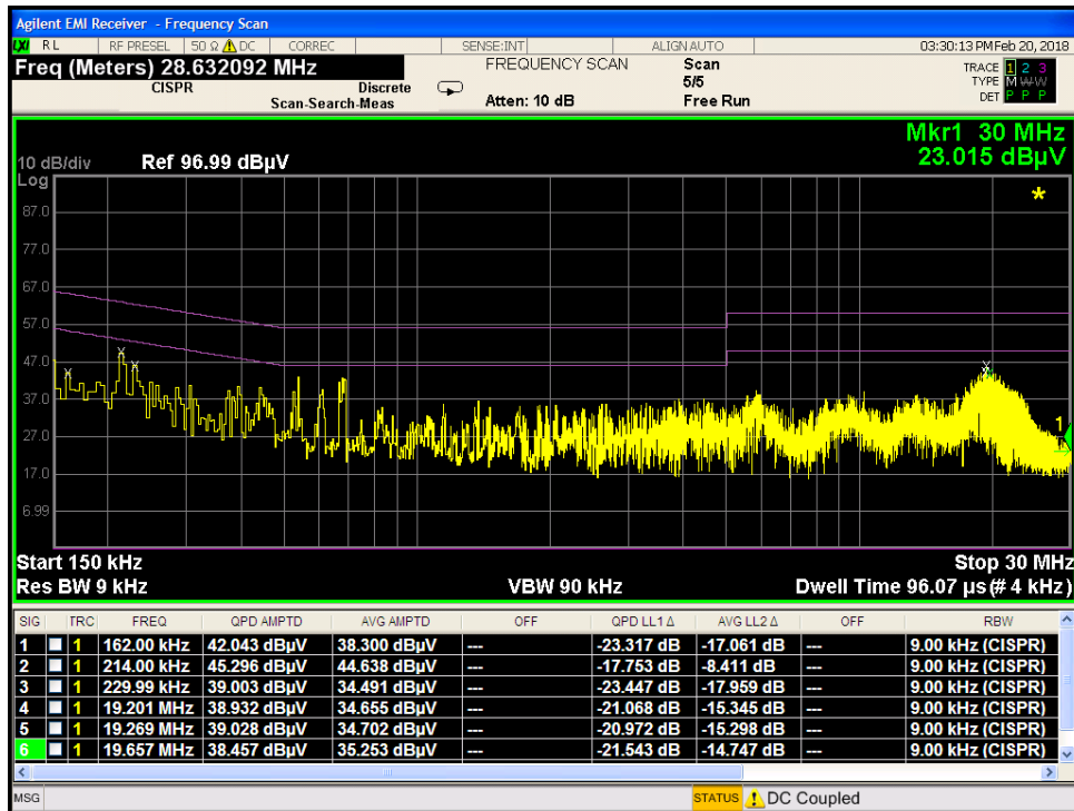
Plot 7-11. Line-Conducted Test Plot (N) with WCP - Terminated in 50Ω
