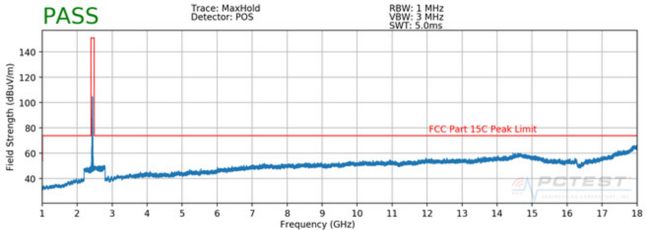
Plot 7-78. Radiated Spurious Plot above 1GHz (802.11b – Ch. 6) H
