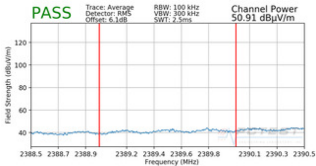
Plot 7-91. Radiated Restricted Lower Band Edge Measurement (Average)
