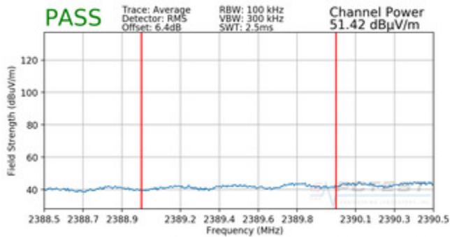
Plot 7-109. Radiated Restricted Band Edge Measurement with WCP (Average)
