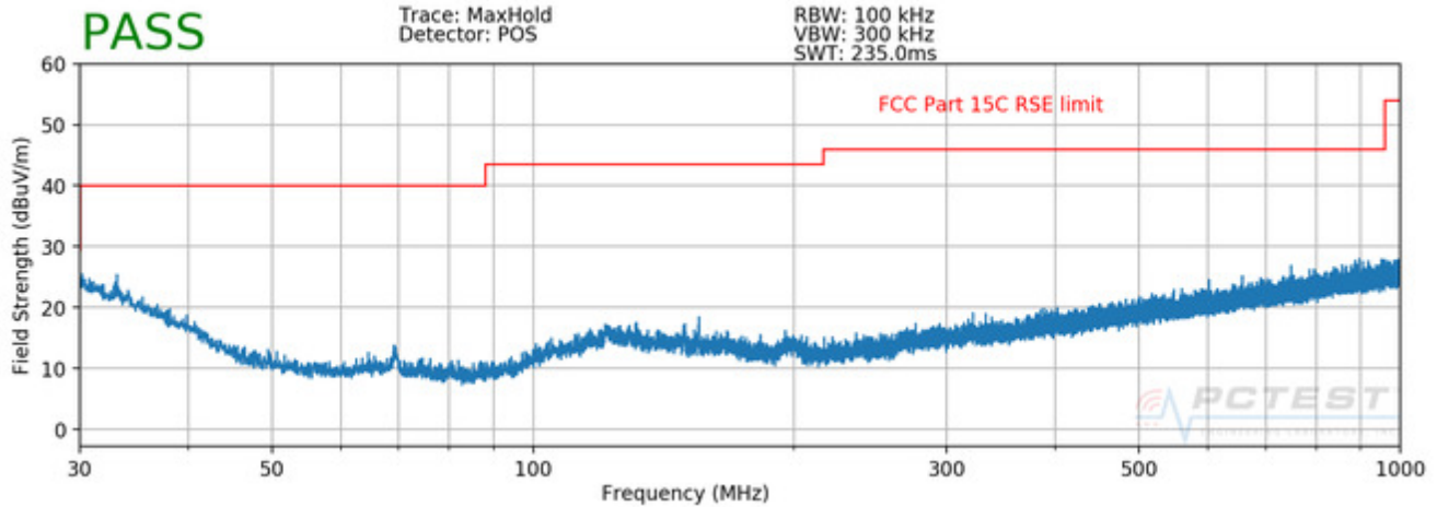
Plot 7-112. Radiated Spurious Plot below 1GHz V
