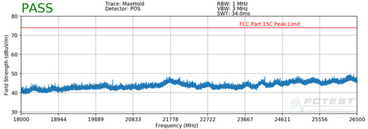
Plot 7-76. Radiated Spurious Plot above 18GHz H
