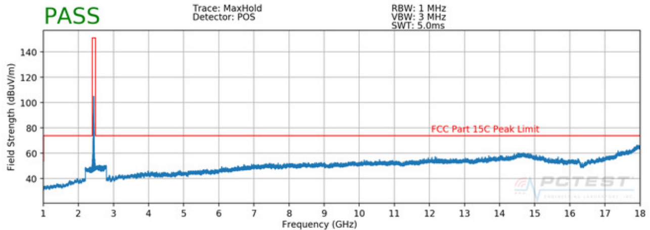
Plot 7-74. Radiated Spurious Plot above 1GHz (802.11b – Ch. 6) H
