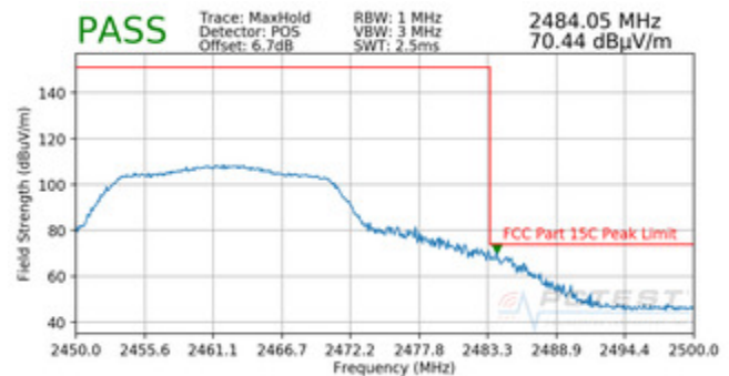
Plot 7-104. Radiated Restricted Upper Band Edge Measurement (Peak)
