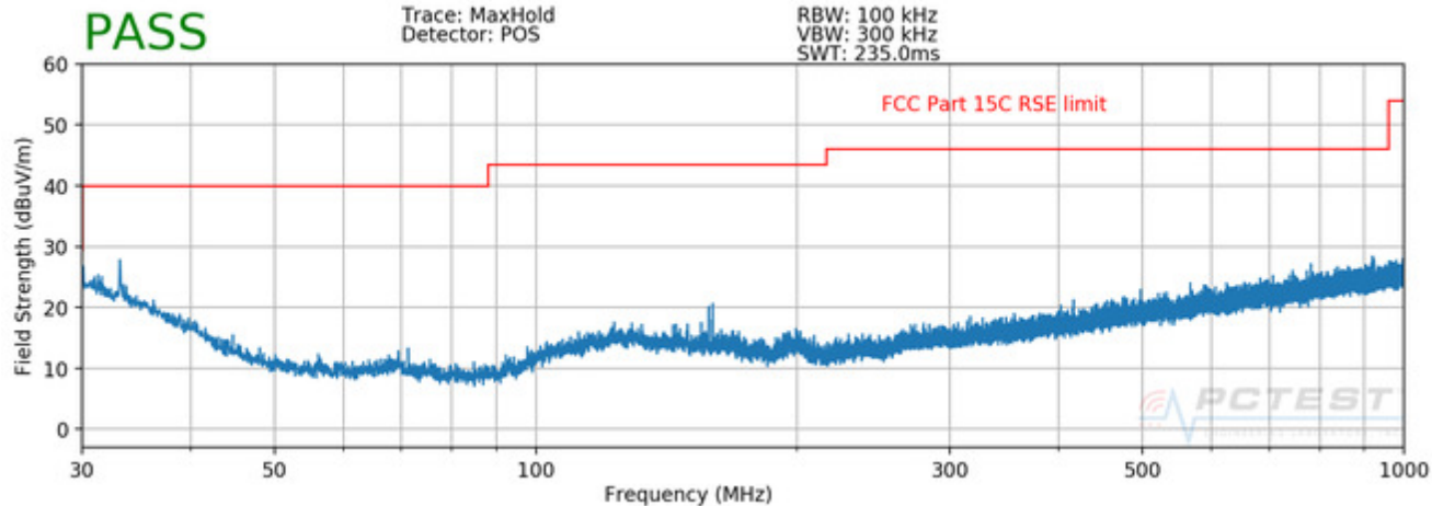
Plot 7-111. Radiated Spurious Plot below 1GHz V
