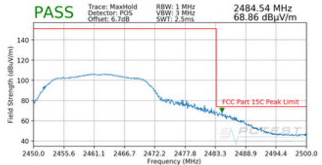
Plot 7-94. Radiated Restricted Upper Band Edge Measurement (Peak)
