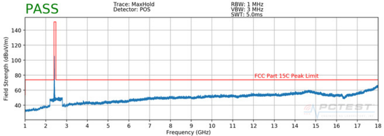
Plot 7-77. Radiated Spurious Plot above 1GHz (802.11b – Ch. 1) H
