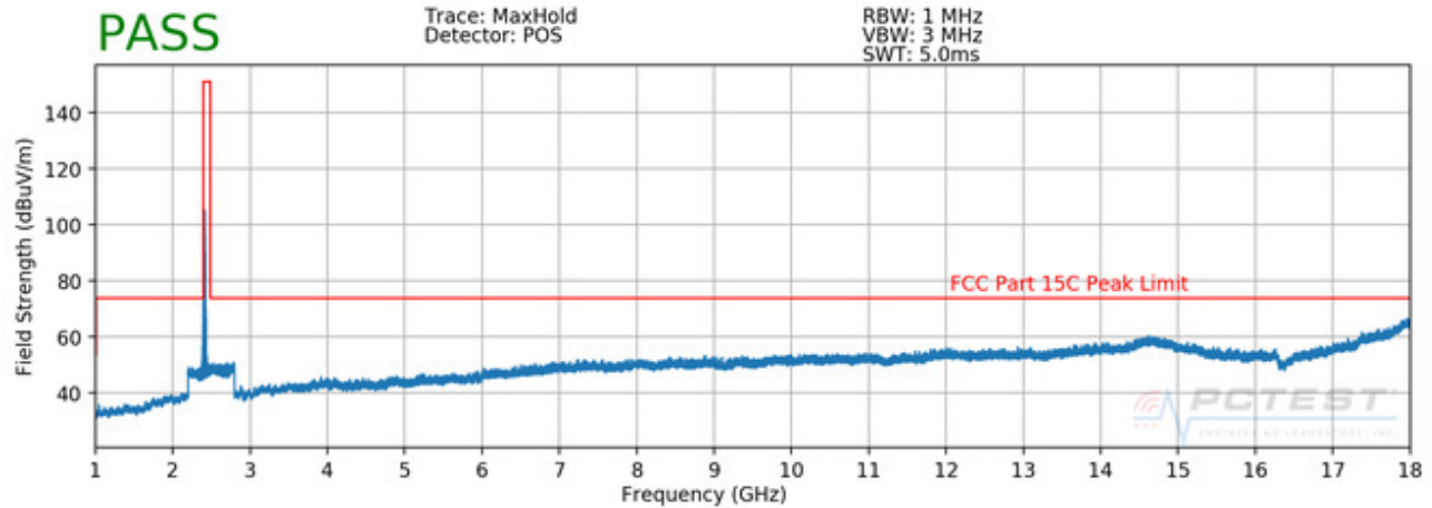
Plot 7-73. Radiated Spurious Plot above 1GHz (802.11b – Ch. 1) H
