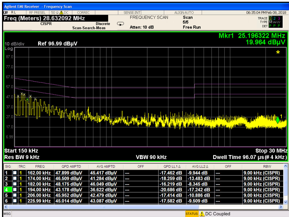
Plot 7-116. Line Conducted Plot 802.11b with WCP (N)
