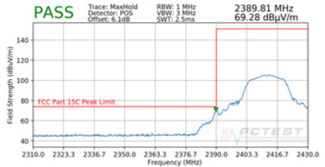
Plot 7-90. Radiated Restricted Band Edge Measurement with WCP (Peak)
