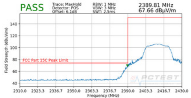
Plot 7-92. Radiated Restricted Lower Band Edge Measurement (Peak)
