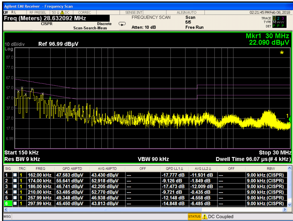
Plot 7-113. Line Conducted Plot 802.11b (L1)
