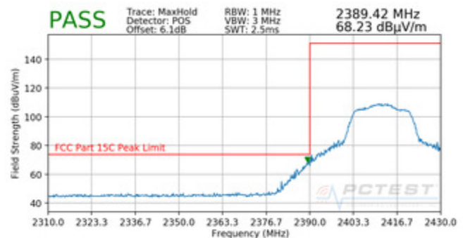
Plot 7-102. Radiated Restricted Lower Band Edge Measurement (Peak)
