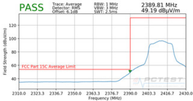
Plot 7-89. Radiated Restricted Band Edge Measurement with WCP (Average)
