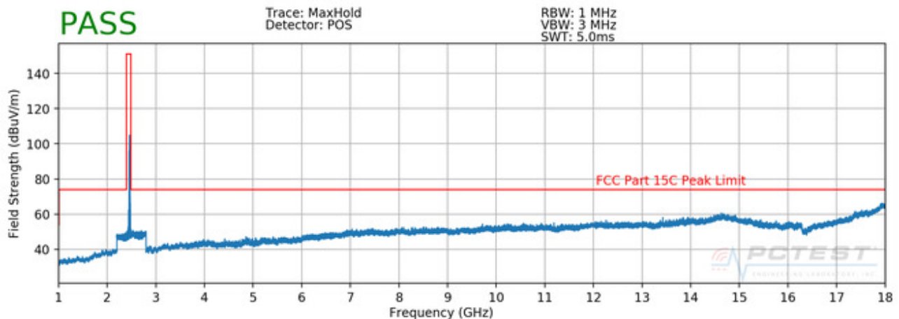
Plot 7-79. Radiated Spurious Plot above 1GHz (802.11b – Ch. 11) H
