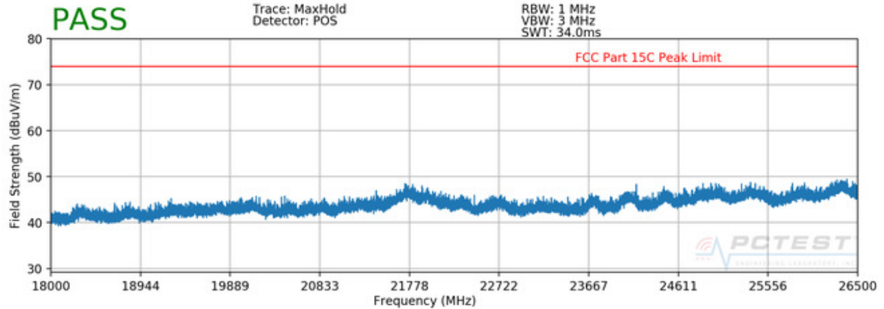
Plot 7-80. Radiated Spurious Plot above 18GHz H
