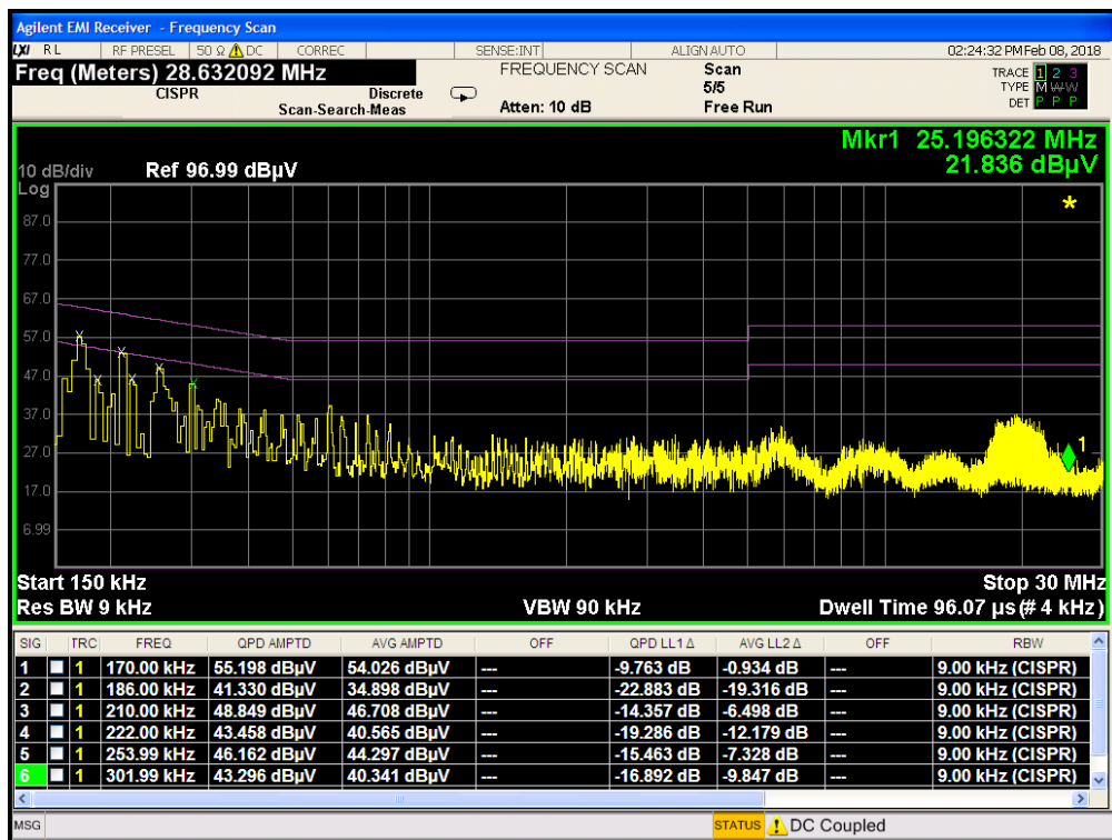
Plot 7-114. Line Conducted Plot 802.11b (N)
