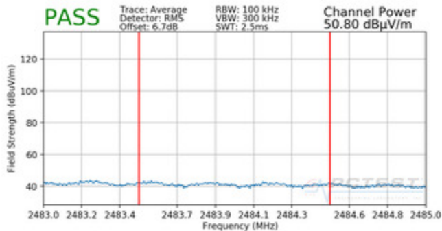
Plot 7-93. Radiated Restricted Upper Band Edge Measurement (Average)
