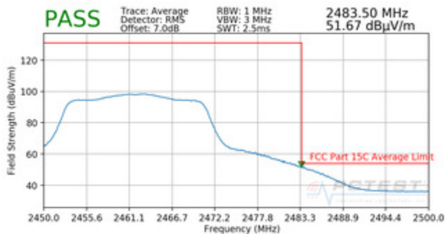
Plot 7-103. Radiated Restricted Upper Band Edge Measurement (Average)
