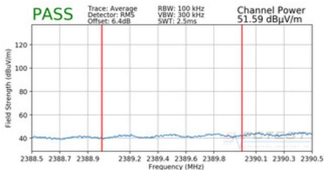
Plot 7-101. Radiated Restricted Lower Band Edge Measurement (Average)
