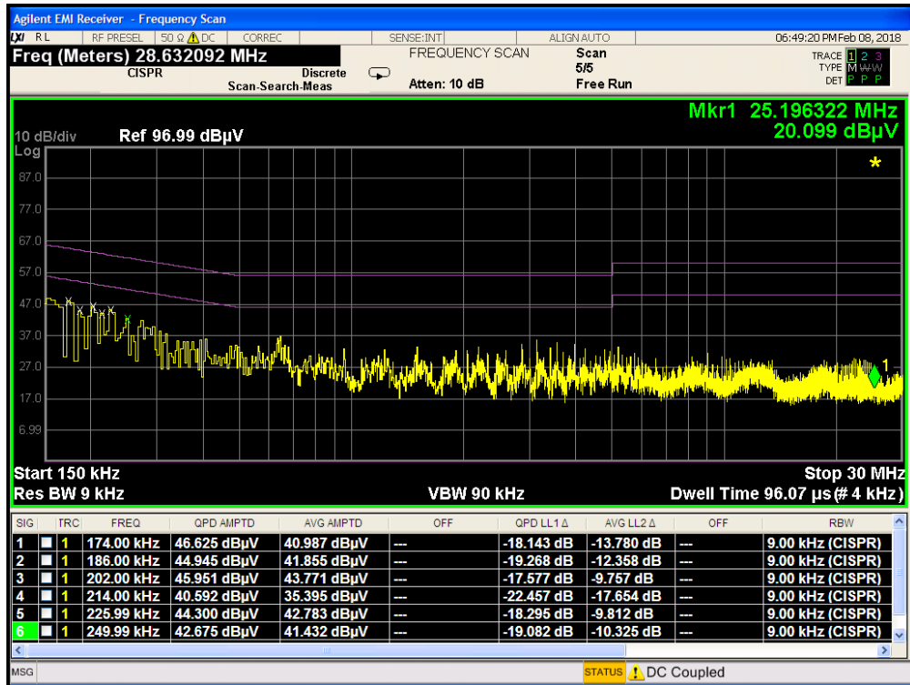
Plot 7-115. Line Conducted Plot 802.11b with WCP (L1)
