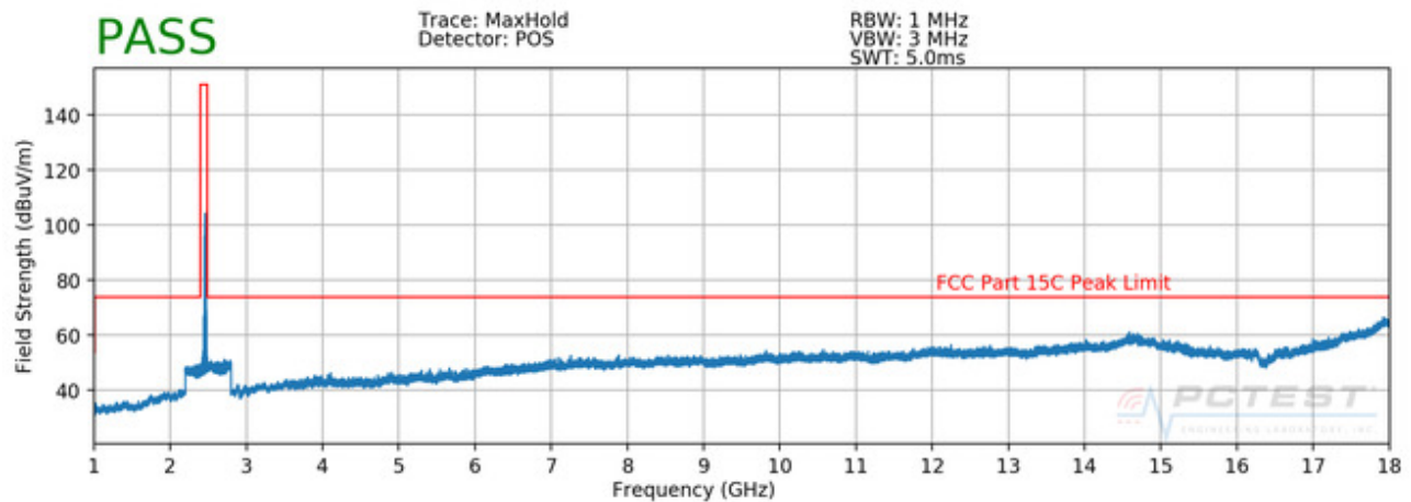
Plot 7-75. Radiated Spurious Plot above 1GHz (802.11b – Ch. 11) H
