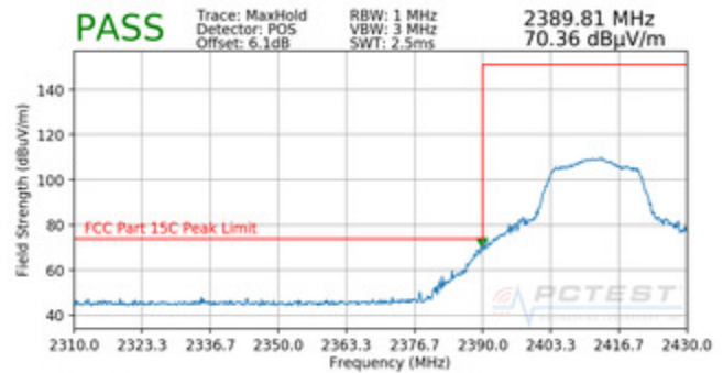
Plot 7-110. Radiated Restricted Band Edge Measurement with WCP (Peak)
