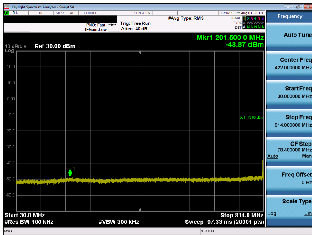
Plot 7-16. Conducted Spurious Plot (LTE Band 26, 15.0MHz QPSK – RB Size 1, RB Offset 0)
