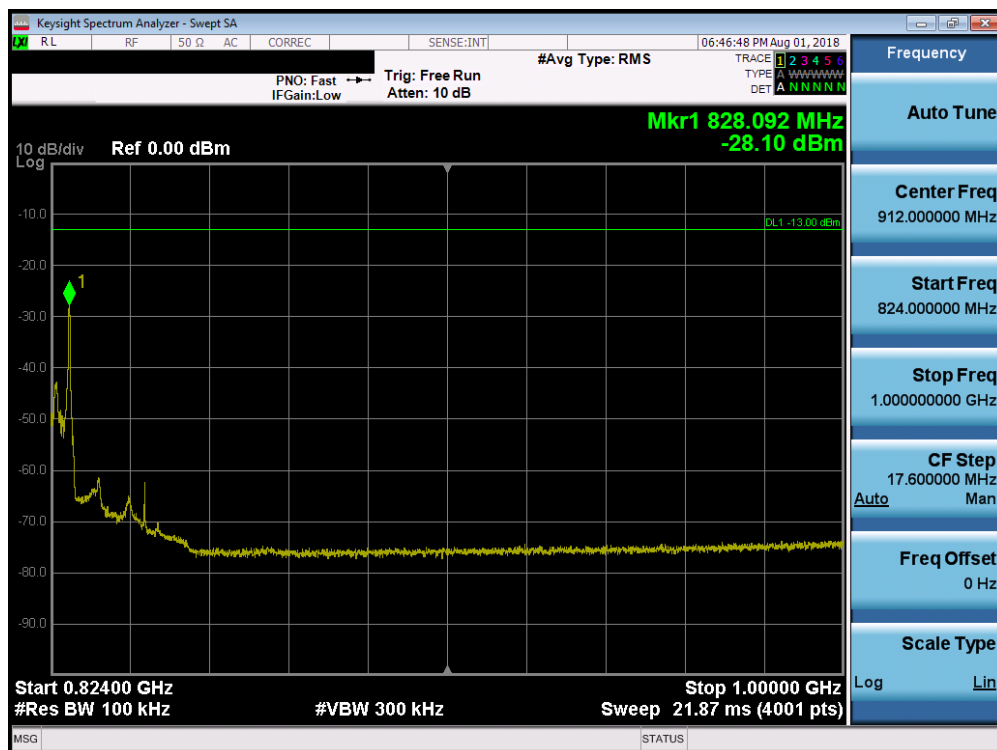
Plot 7-17. Conducted Spurious Plot (LTE Band 26, 15.0MHz QPSK – RB Size 1, RB Offset 0)
