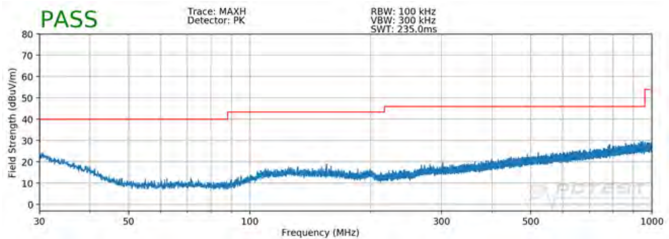
Plot 7-137. Radiated Spurious Plot below 1GHz SISO ANT1
