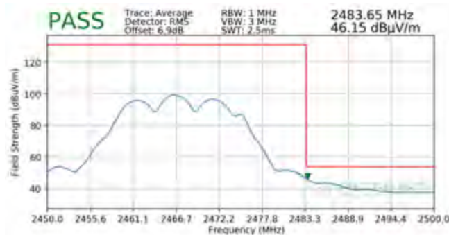
Plot 7-117. Radiated Restricted Upper Band Edge Measurement CDD (Average)
