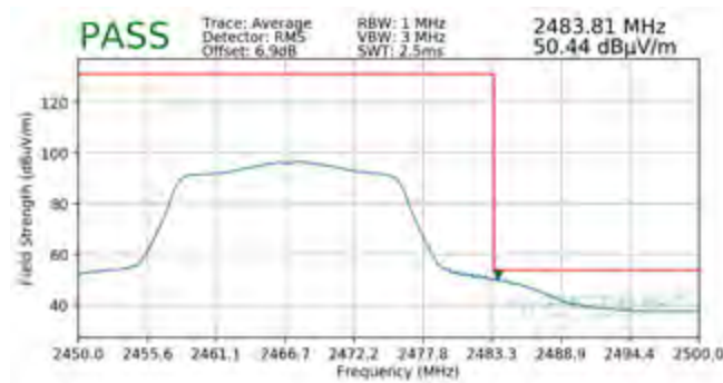
Plot 7-107. Radiated Restricted Band Edge Measurement SISO ANT2 with WCP (Average)
