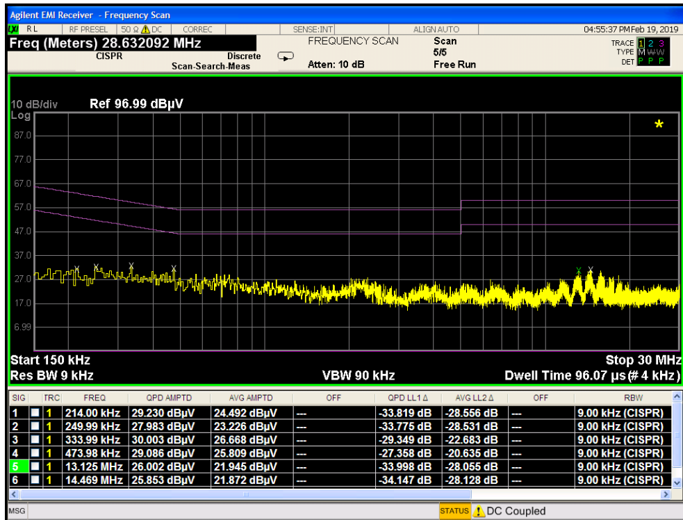
Plot 7-9. Line-Conducted Test Plot (N) – with Antenna Terminated in 50Ω
