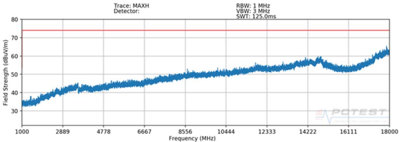
Plot 7-11. Radiated Spurious Plot above 1GHz (Configuration 3 - H)
