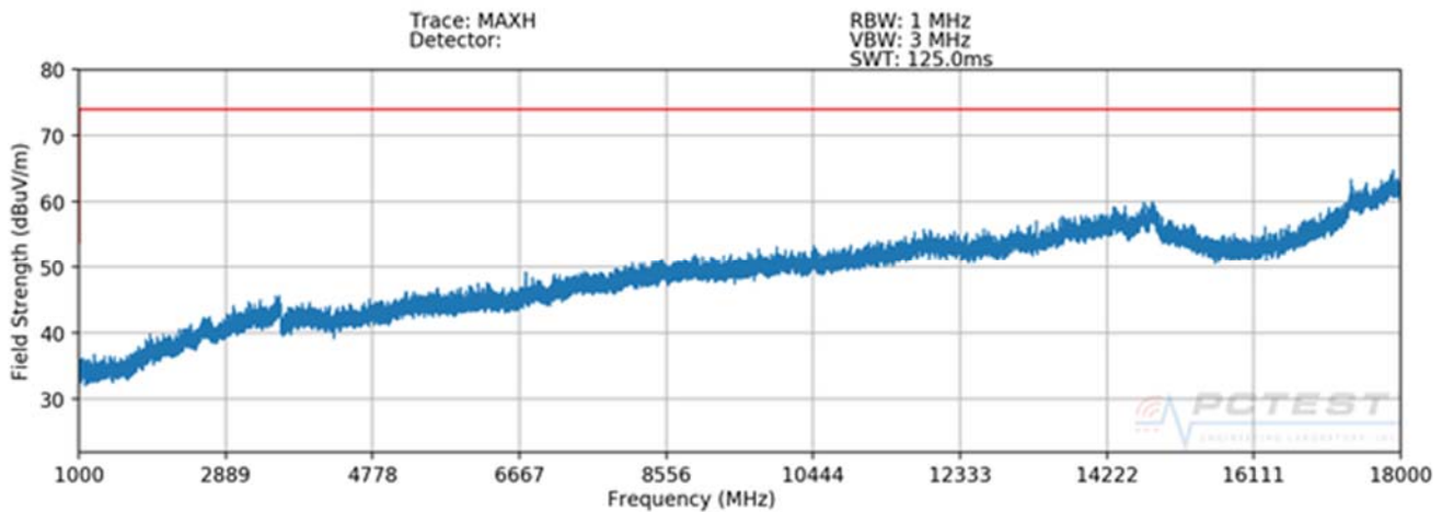
Plot 7-3. Radiated Spurious Plot above 1GHz (Configuration 1 - H)
