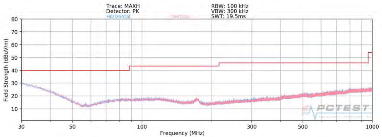
Plot 7-370. Radiated Spurious Plot below 1GHz (5GHz – 2.4 GHz)
