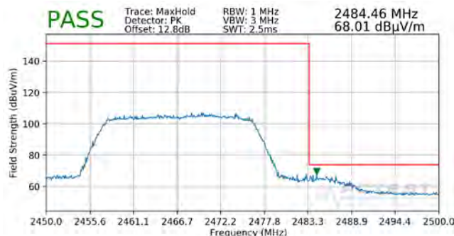
Plot 7-202. Radiated Restricted Upper Band Edge Measurement MIMO (Peak - 242 Tones)
