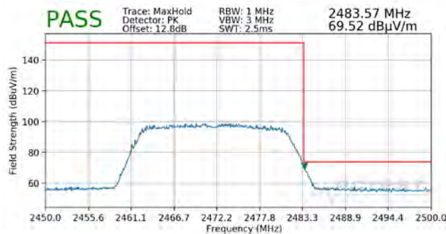
Plot 7-168. Radiated Restricted Upper Band Edge Measurement SISO ANT1 (Peak - 242 Tones)
