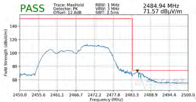
Plot 7-194. Radiated Restricted Upper Band Edge Measurement MIMO (Peak - 106 Tones)
