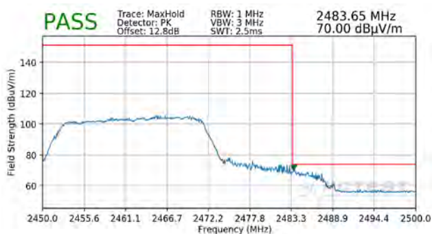
Plot 7-188. Radiated Restricted Band Edge Measurement SISO ANT2 with WCP (Peak – 242 Tones)
