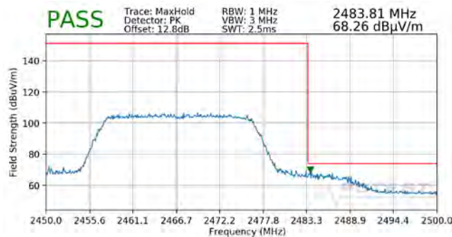
Plot 7-166. Radiated Restricted Upper Band Edge Measurement SISO ANT1 (Peak - 242 Tones)
