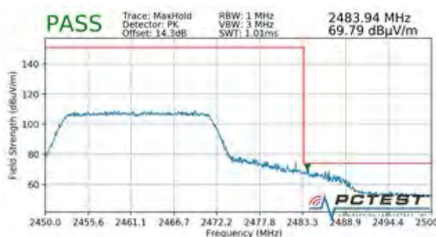
Plot 7-164. Radiated Restricted Upper Band Edge Measurement SISO ANT1 (Peak - 242 Tones)
