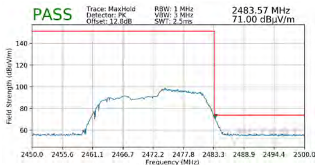
Plot 7-178. Radiated Restricted Upper Band Edge Measurement SISO ANT1 (Peak - 106 Tones)
