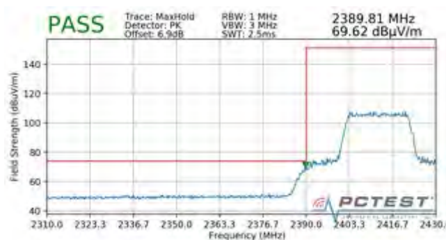
Plot 7-162. Radiated Restricted Lower Band Edge Measurement SISO ANT1 (Peak - 242 Tones)
