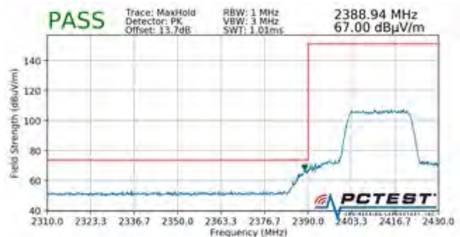
Plot 7-198. Radiated Restricted Lower Band Edge Measurement MIMO (Peak - 242 Tones)
