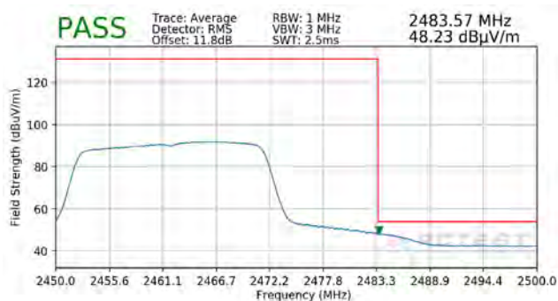
Plot 7-187. Radiated Restricted Band Edge Measurement SISO ANT2 with WCP (Average – 242 Tones)
