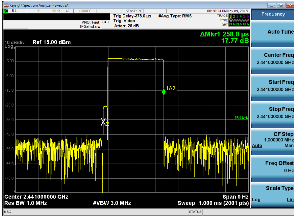
Plot 7-2. Pulse Width Measurement
