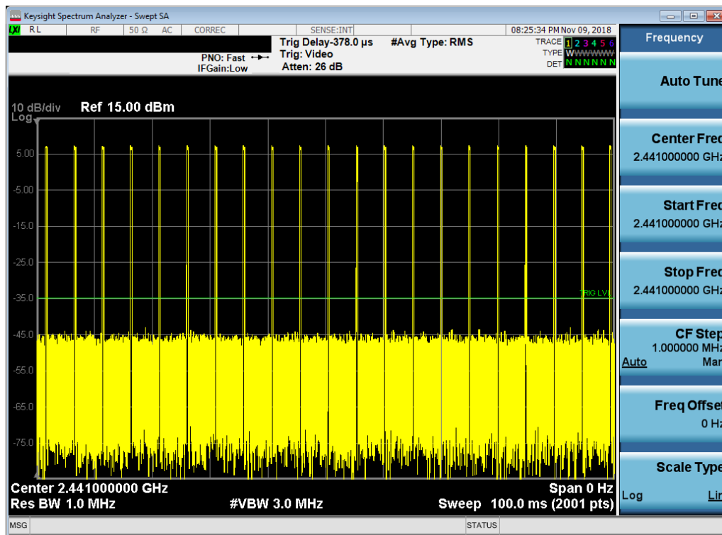
Plot 7-3. Worst Case 100ms Operation
