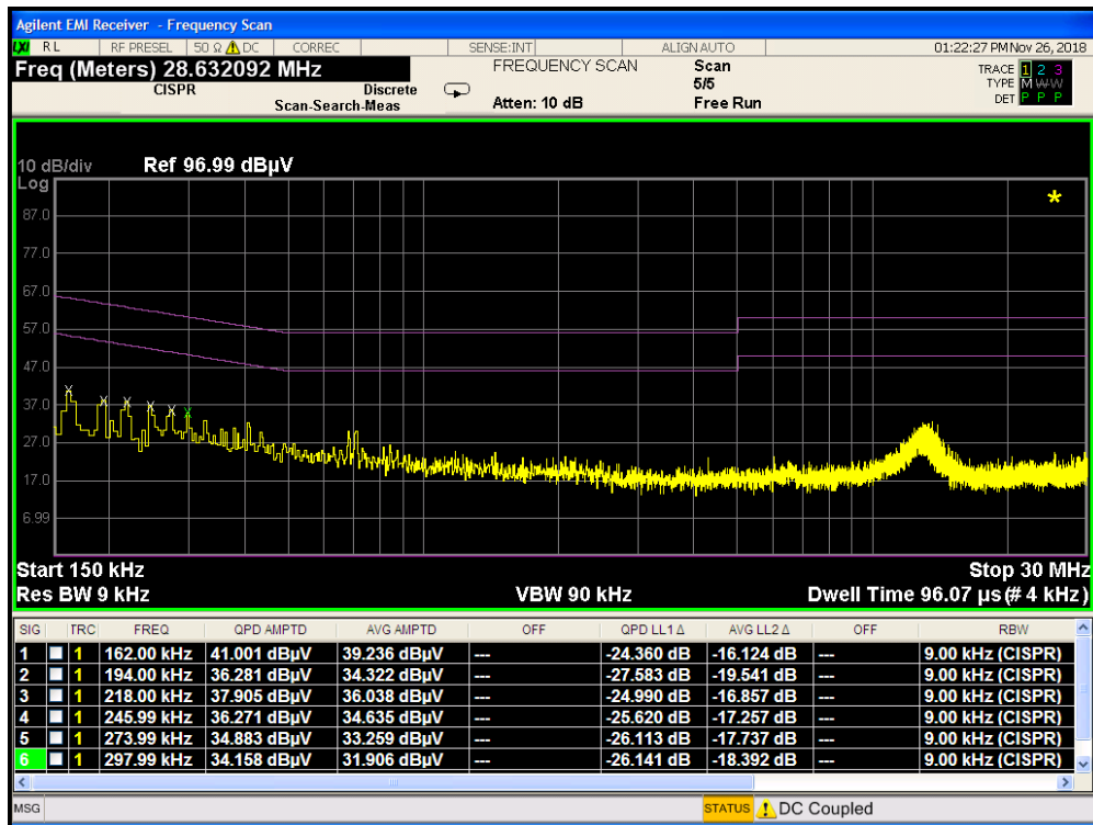
Plot 7-56. Line Conducted Plot with Bluetooth LE (N)
