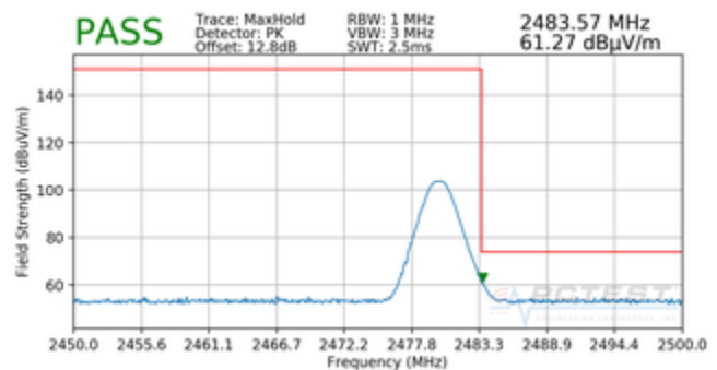
Plot 7-52. Radiated Restricted Upper Band Edge Measurement (Peak)
