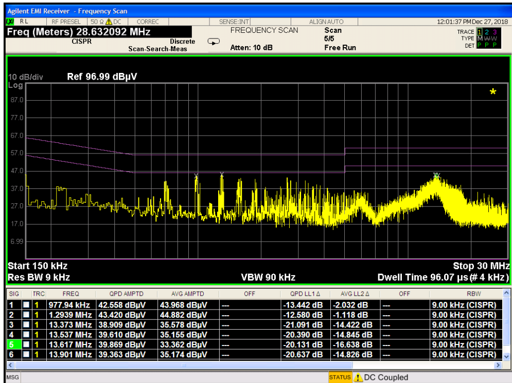
Plot 7-58. Line Conducted Plot with Bluetooth LE (N) with Wireless Charging Pad
