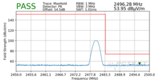
Plot 7-54. Radiated Restricted Upper Band Edge Measurement with WCP (Peak)
