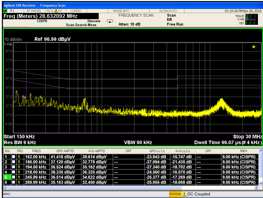
Plot 7-55. Line Conducted Plot with Bluetooth LE (L1)
