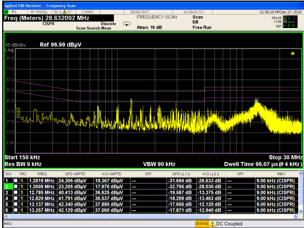
Plot 7-57. Line Conducted Plot with Bluetooth LE (L1) with Wireless Charging Pad
