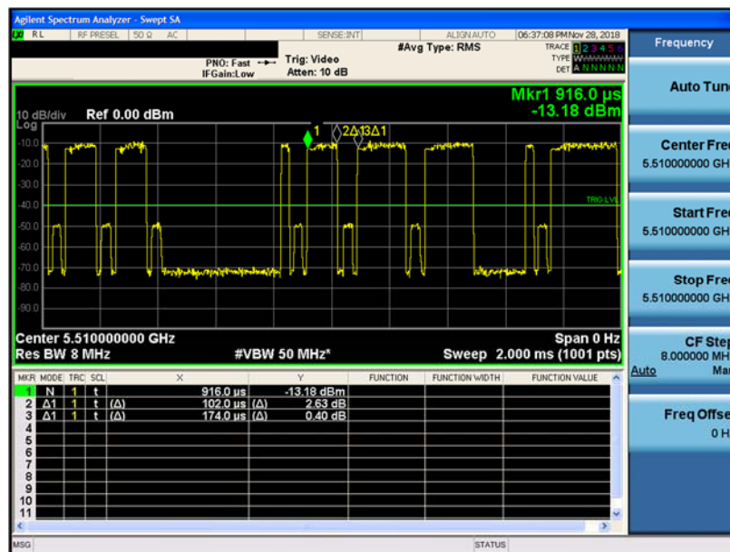
Figure 5-2. Band 2C Pulse Width
