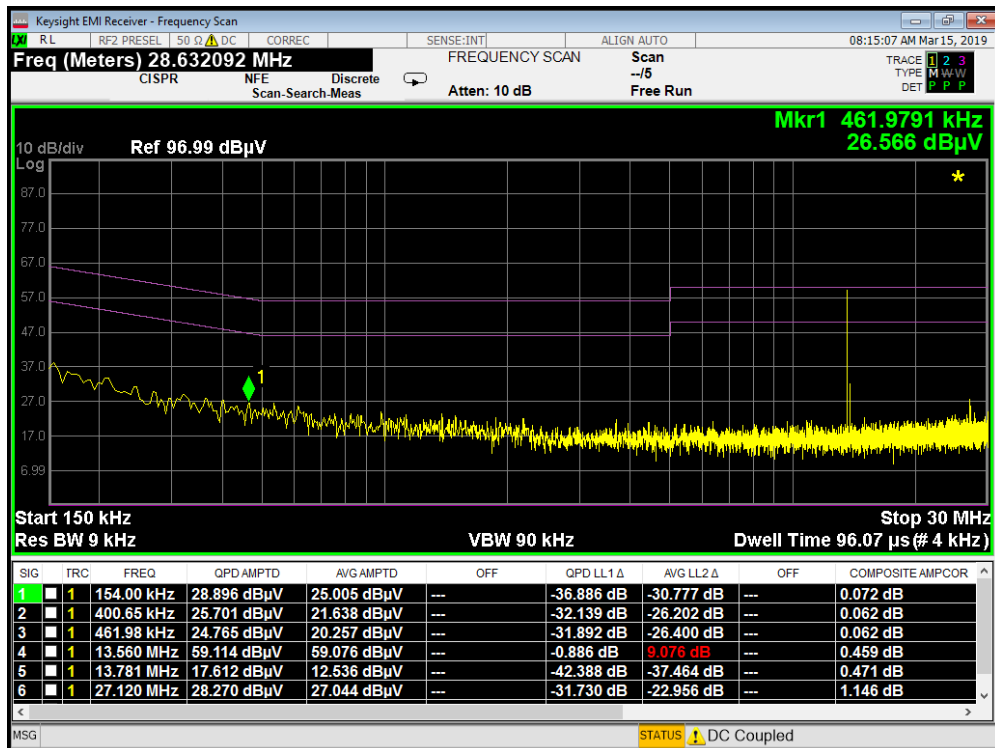
Plot 7-7. Line-Conducted Test Plot with Antenna (N)
