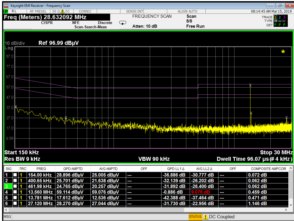
Plot 7-6. Line-Conducted Test Plot with Antenna (L1)
