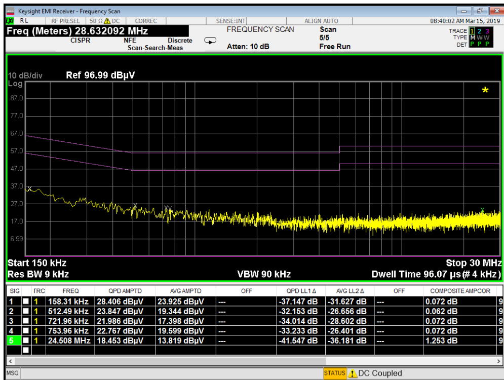
Plot 7-9. Line-Conducted Test Plot with Antenna Terminated in 50Ω (N)
