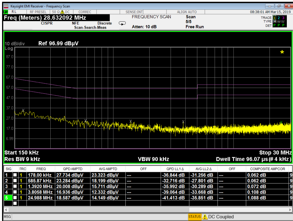
Plot 7-8. Line-Conducted Test Plot with Antenna Terminated in 50Ω (L1)
