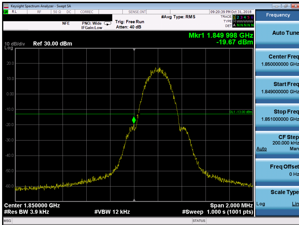
Plot 7-35. Band Edge Plot (PCS GSM Mode - Low Channel)
