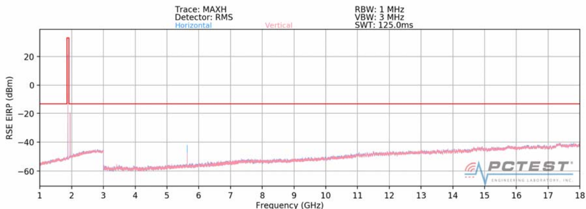
Plot 7-48. Radiated Spurious Plot above 1GHz (PCS GPRS)
