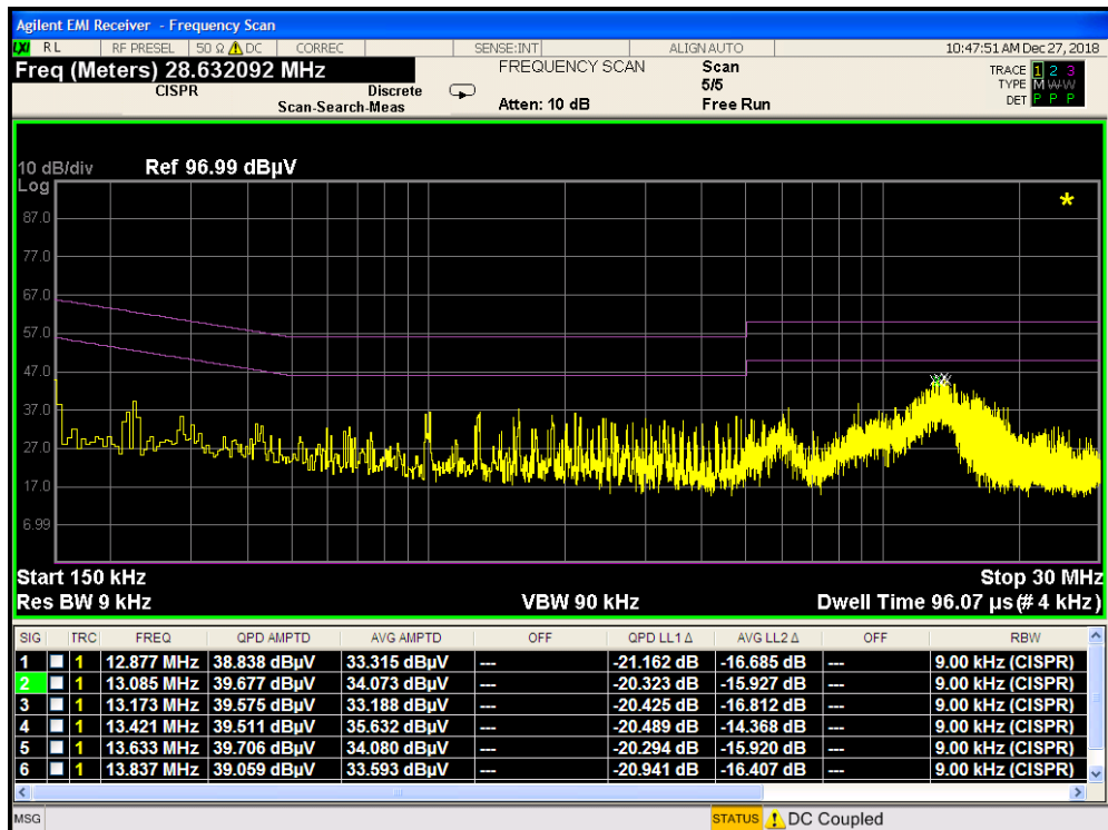
Plot 7-54. Line-Conducted Test Plot (N) with Wireless Charging Pad
