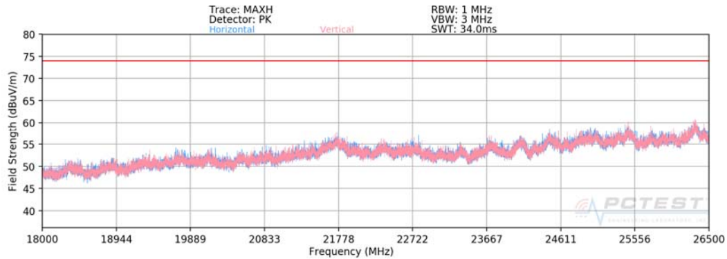
Plot 7-45. Radiated Spurious Plot above 18GHz
