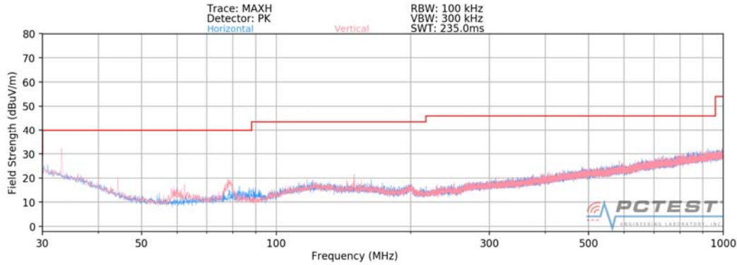
Plot 7-50. Radiated Spurious Plot below 1GHz
