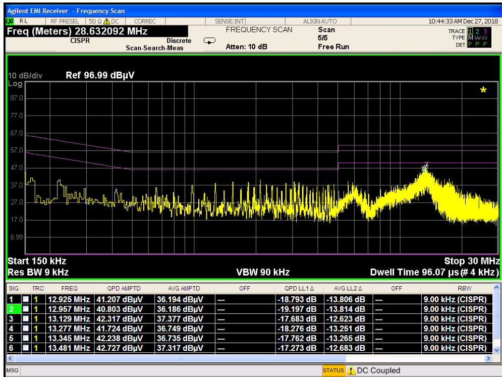
Plot 7-53. Line-Conducted Test Plot (L1) with Wireless Charging Pad
