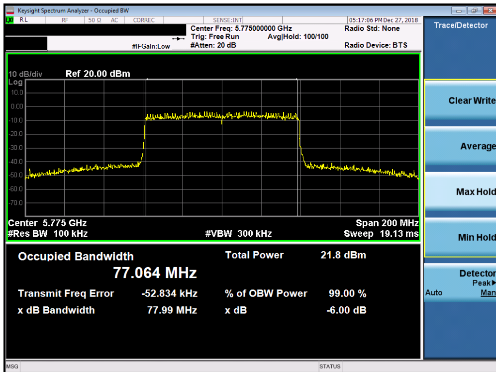
Plot 7-117. 6dB Bandwidth Plot SISO ANT1 (80MHz BW 802.11aax (UNII Band 3) – Ch. 155)
