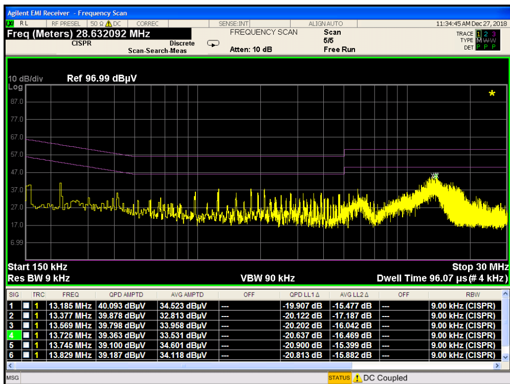
Plot 7-398. Line Conducted Plot with 802.11a UNII Band 2A with WCP (N)
