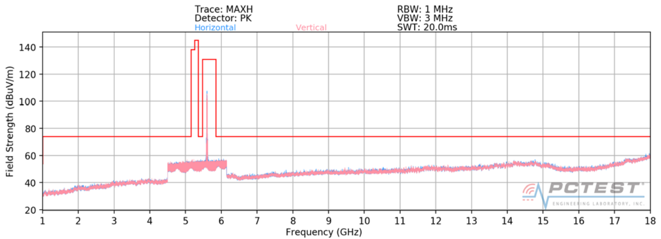
Plot 7-279. Radiated Spurious Plot above 1GHz MIMO/CDD (802.11a – U2C Ch. 120)
