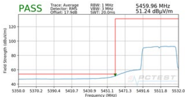
Plot 7-305. Radiated Lower Band Edge Plot SISO ANT1 (Average – UNII Band 2C)
