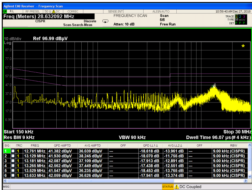
Plot 7-397. Line Conducted Plot with 802.11a UNII Band 2A with WCP (L1)
