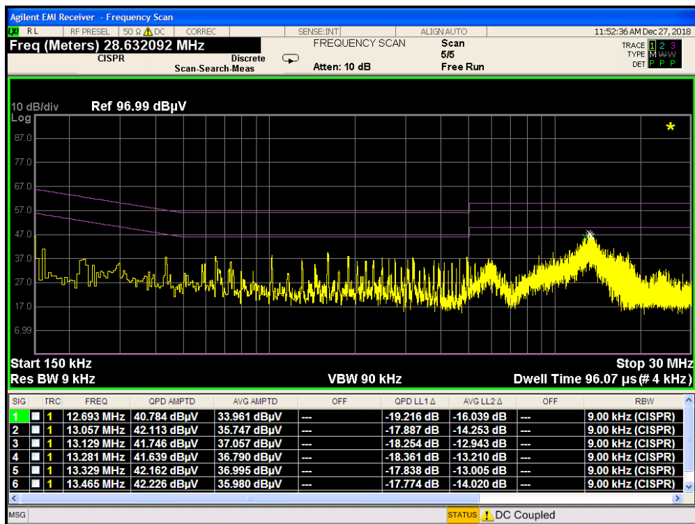
Plot 7-401. Line Conducted Plot with 802.11a UNII Band 3 with WCP (L1)
