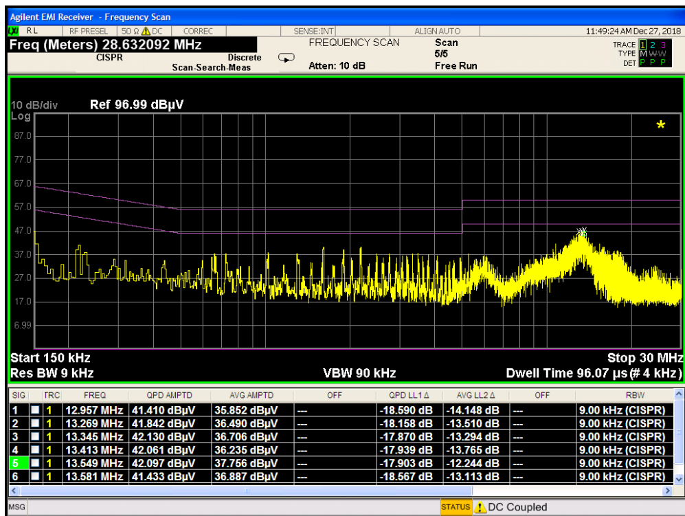
Plot 7-399. Line Conducted Plot with 802.11a UNII Band 2C with WCP (L1)
