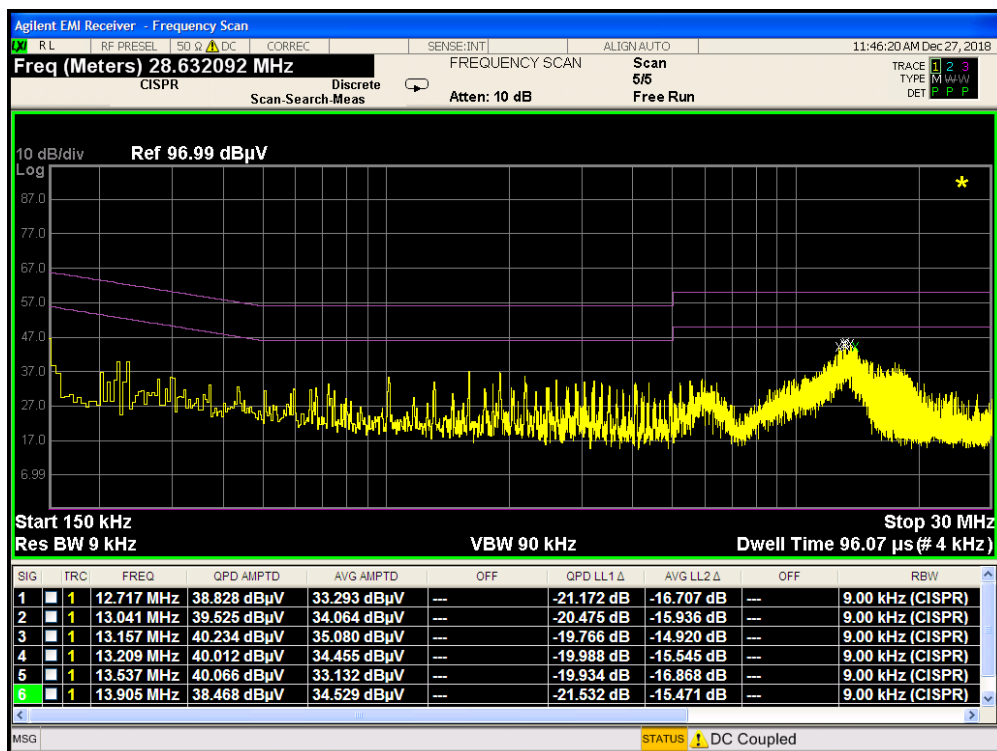
Plot 7-400. Line Conducted Plot with 802.11a UNII Band 2C with WCP (N)
