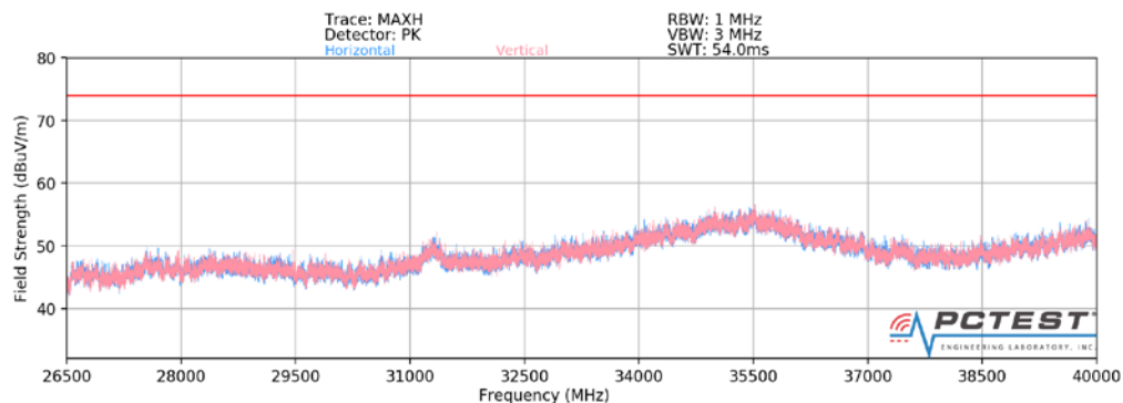
Plot 7-291. Radiated Spurious Plot above 26.5GHz (Dual Band Simult. Tx)
