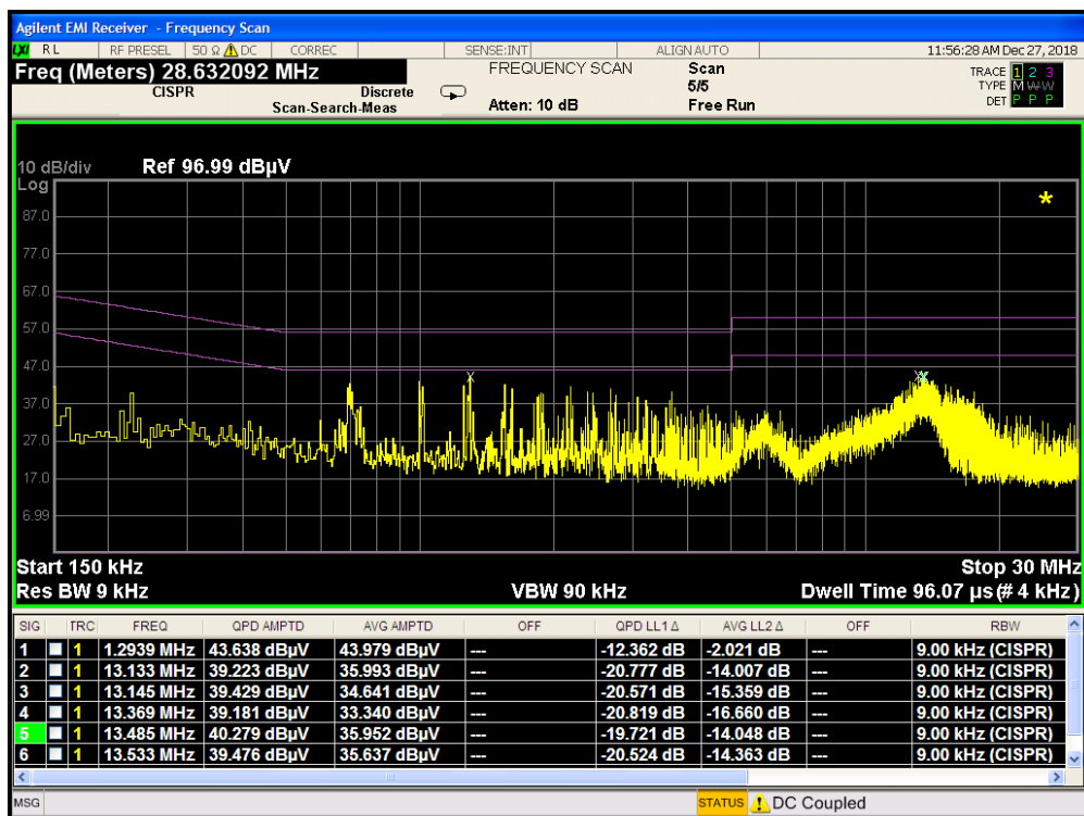
Plot 7-402. Line Conducted Plot with 802.11a UNII Band 3 with WCP (N)
