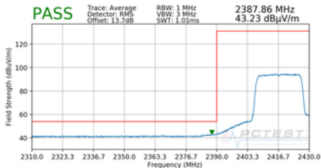
Plot 7-171. Radiated Restricted Lower Band Edge Measurement SISO ANT1 (Average – 242 Tones)
