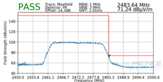
Plot 7-180. Radiated Restricted Upper Band Edge Measurement SISO ANT1 (Peak - 242 Tones)
