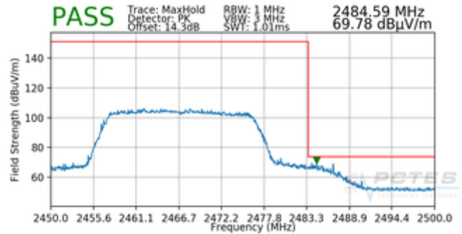
Plot 7-178. Radiated Restricted Upper Band Edge Measurement SISO ANT1 (Peak - 242 Tones)
