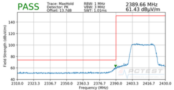
Plot 7-214. Radiated Restricted Lower Band Edge Measurement MIMO (Peak – 242 Tones)
