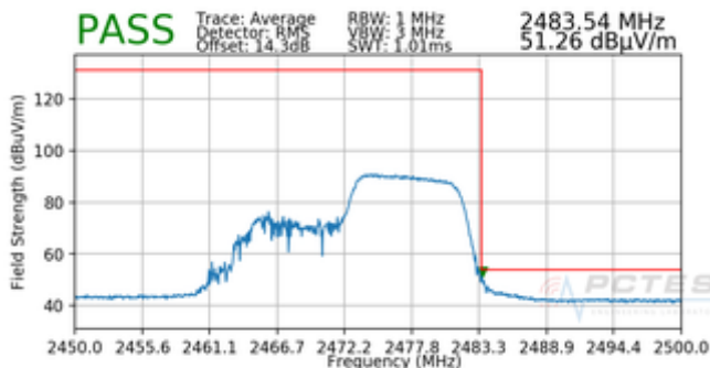
Plot 7-211. Radiated Restricted Upper Band Edge Measurement MIMO (Average – 106 Tones)
