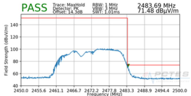
Plot 7-212. Radiated Restricted Upper Band Edge Measurement MIMO (Peak – 106 Tones)
