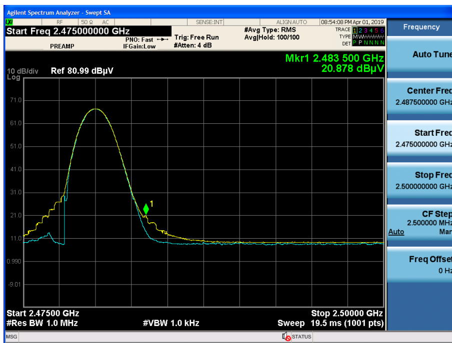
Radiated Restricted Band Edges plot – Average Reading (8DPSK, Ch.78)
