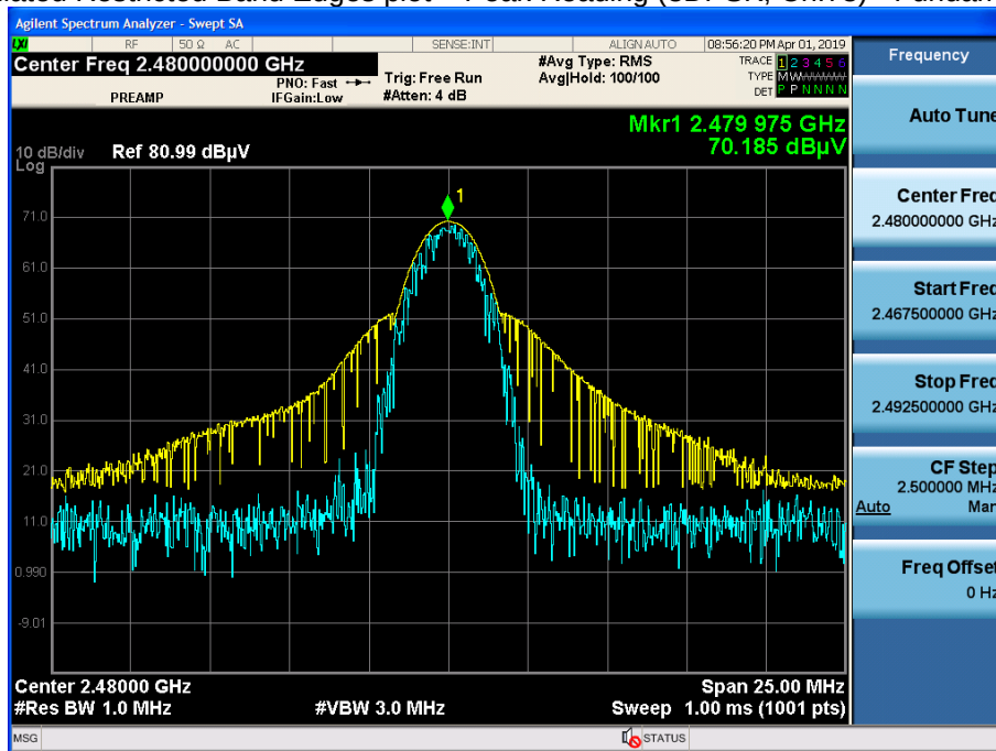
Radiated Restricted Band Edges plot – Peak Reading (8DPSK, Ch.78) - Fundamental
