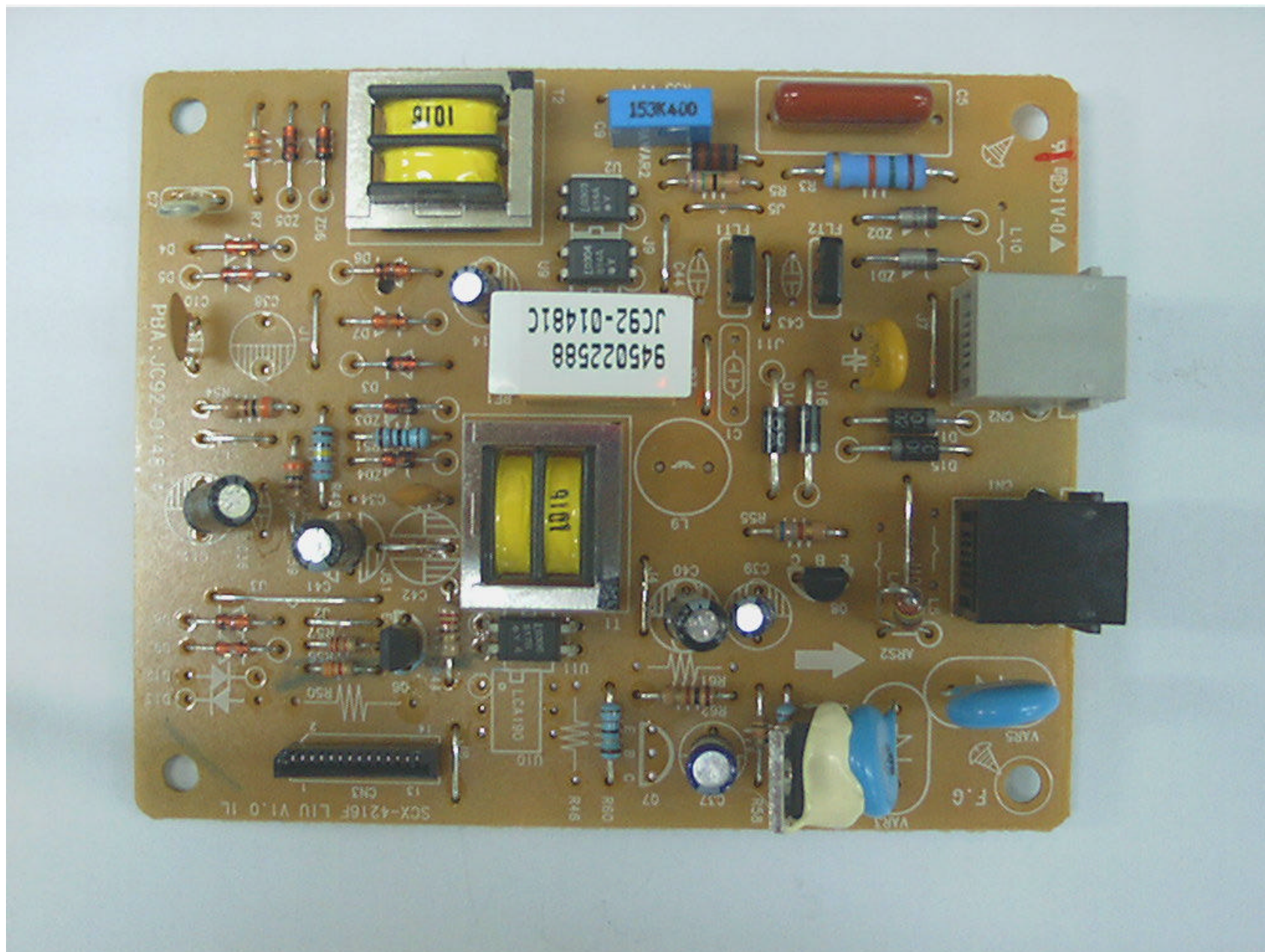
Top view of LIU [NEW]
